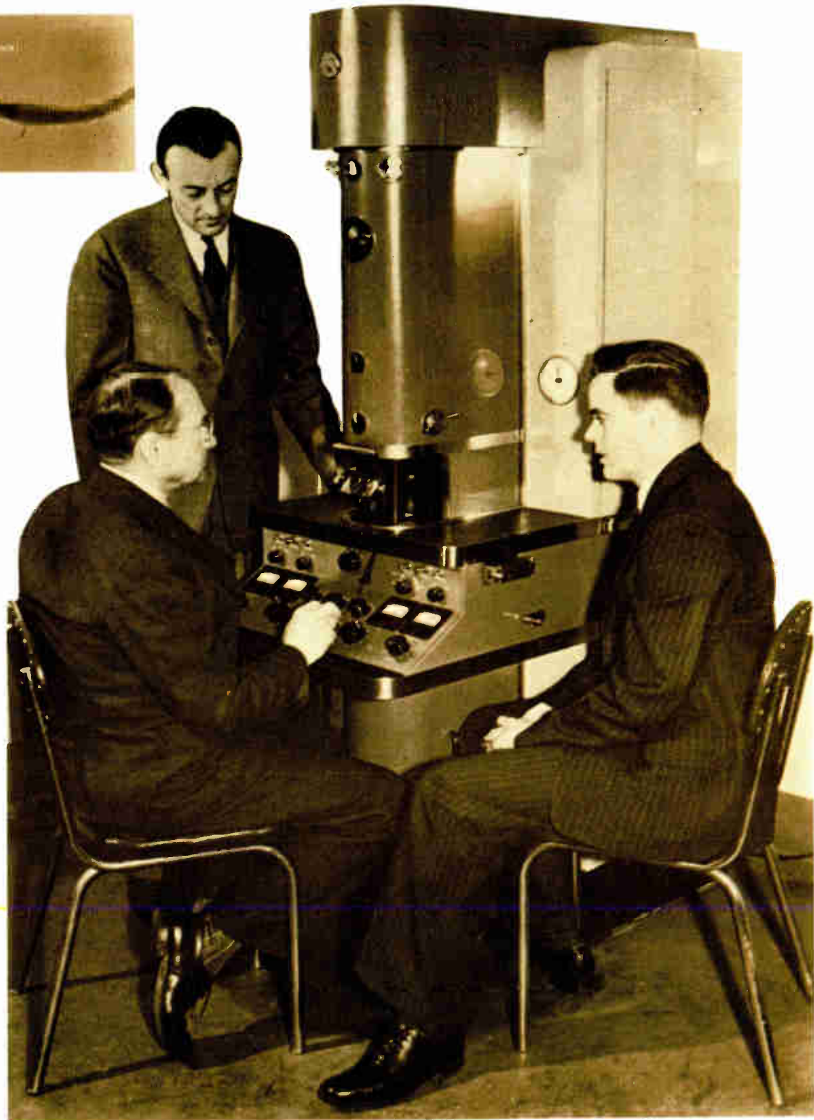
The RCA electron microscope — one of the most revolutionary scientific instruments of the 20th Century — magnifies infinitesimal objects of the submicroscopic world and permits photographic enlargements up to 100,000 diameters.
