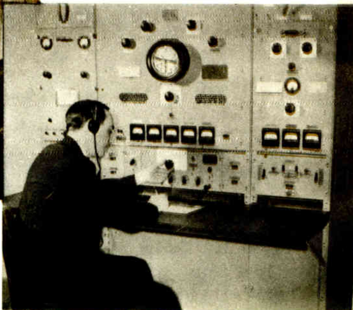
BELOW: New console radio equipment designed by Radiomarine for shipboard installation combines three transmitters, three receivers and an automatic SOS alarm.
