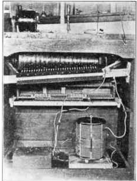
Music was broadcast by Father Desilets, Nicolet, Que., in 1913-'14. Each of the rotary spark dischargers was operated by pressure of its key on the keyboard of the organ which was thus converted into a wireless transmitter.
