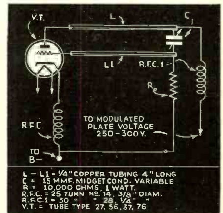
Schematic diagram and list of parts used in constructing the 1-meter oscillator, utilizing standard receiving tubes.
