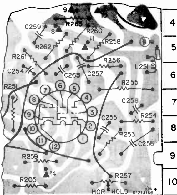
Partial sweep Board for 23" Receivers w/stamping EN118A
