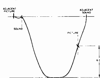
Figure 13 - RF-IF Response
