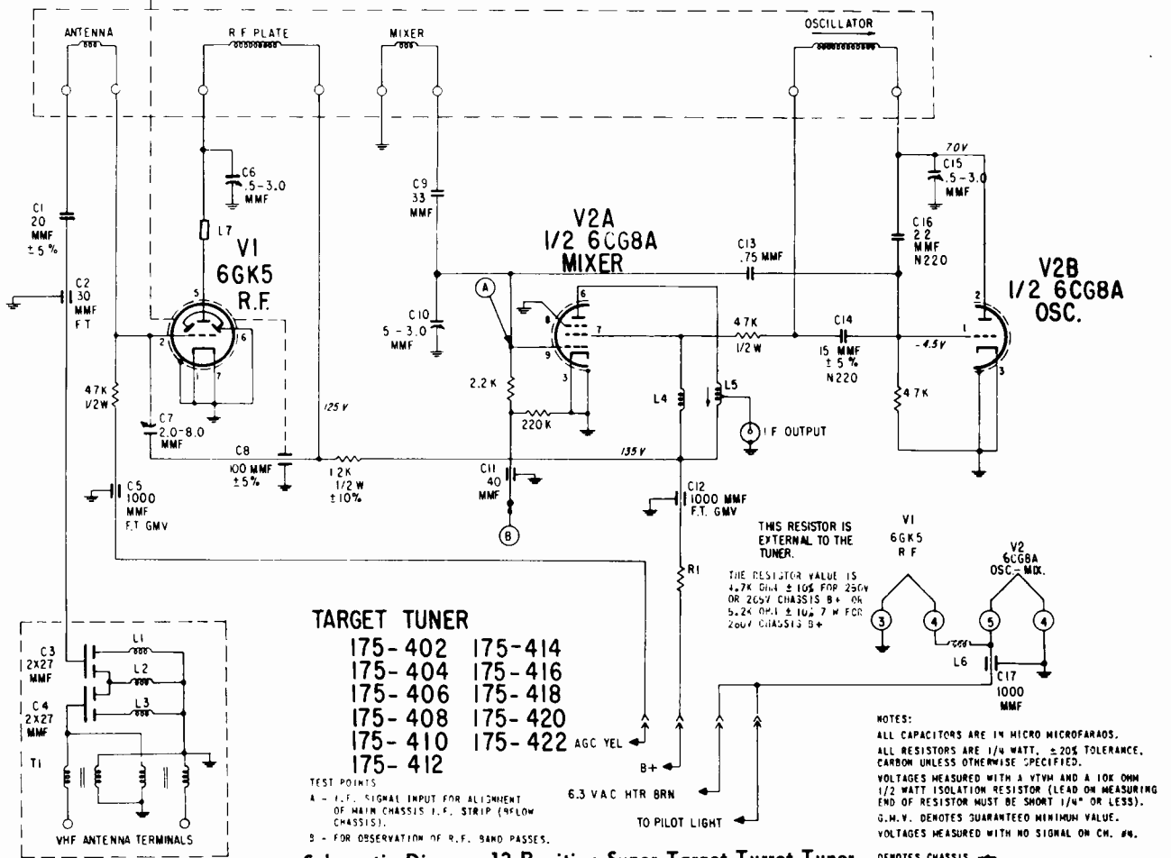
Schematic Diagram 12 Position Super Target Turret Tuner.
