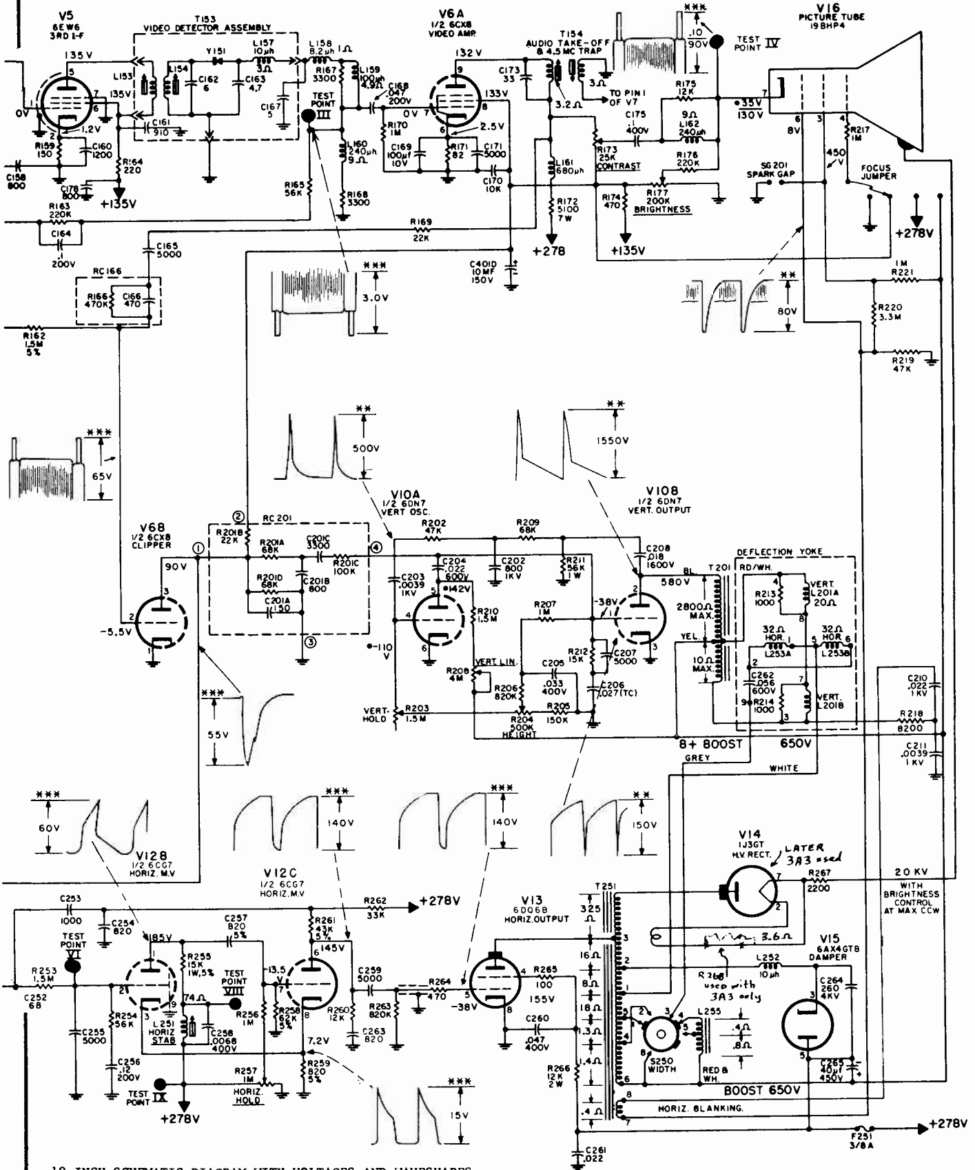
19 INCH SCHEMATIC DIAGRAM WITH VOLTAGES AND WAVESHAPES
