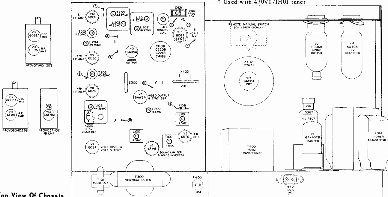
Top View Of Chassis.
