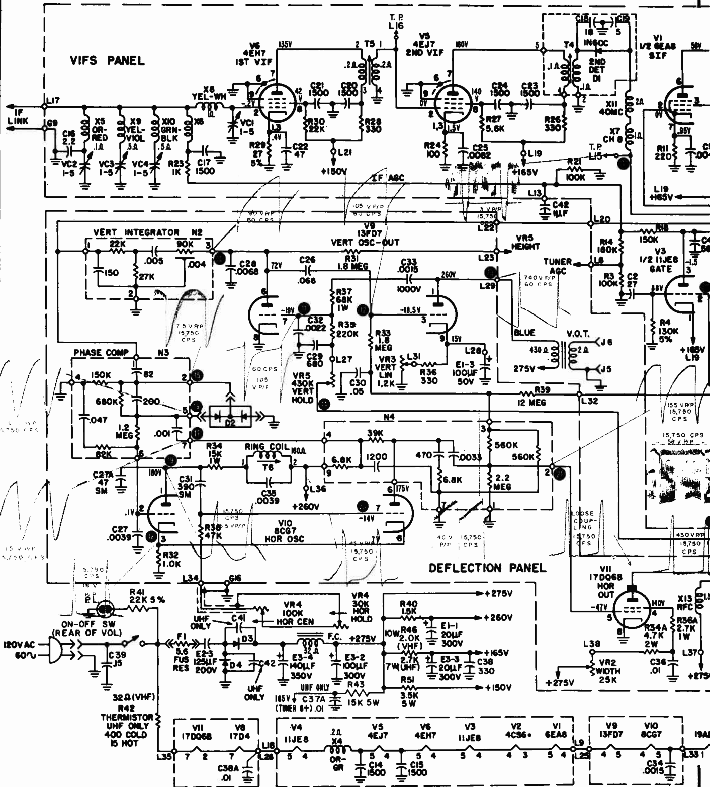
SCHEMATIC DIAGRAMS AND OSCILLOSCOPE WAVEFORMS 12J28
