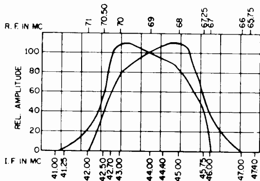
OVERALL R.F., I.F. RESPONSE
