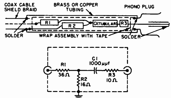
FIG. 1. IF INJECTION NETWORK
