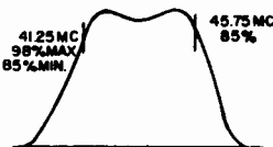
Figure 9—T208 3rd Pix I-F Response
