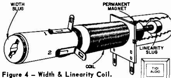
Figure 4 - Width & Linearity Coil.
