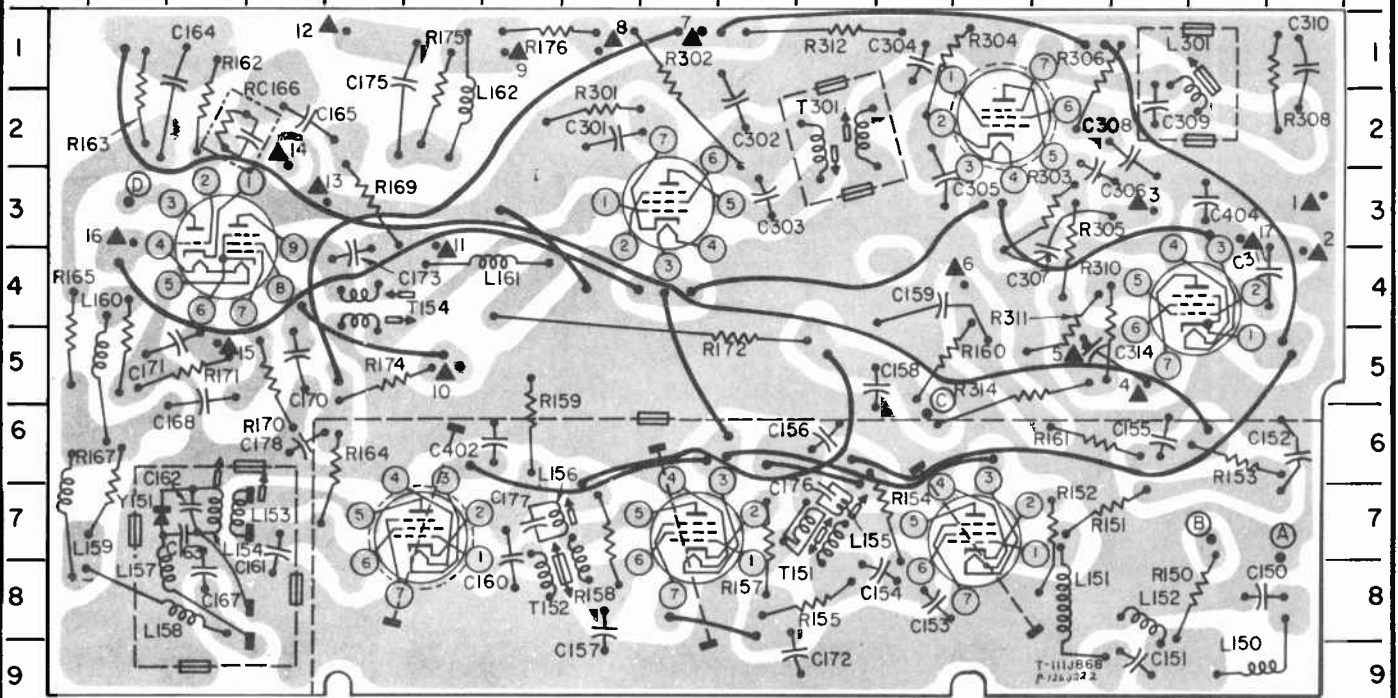
I-F BOARD COMPONENT LOCATIONS AS VIEWED FROM THE CONDUCTOR SIDE
