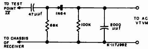
FIG. 3 DETECTOR NETWORK
