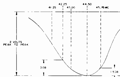
Figure 11 - IF Response: 1st IF amp grid to 2nd detector.
