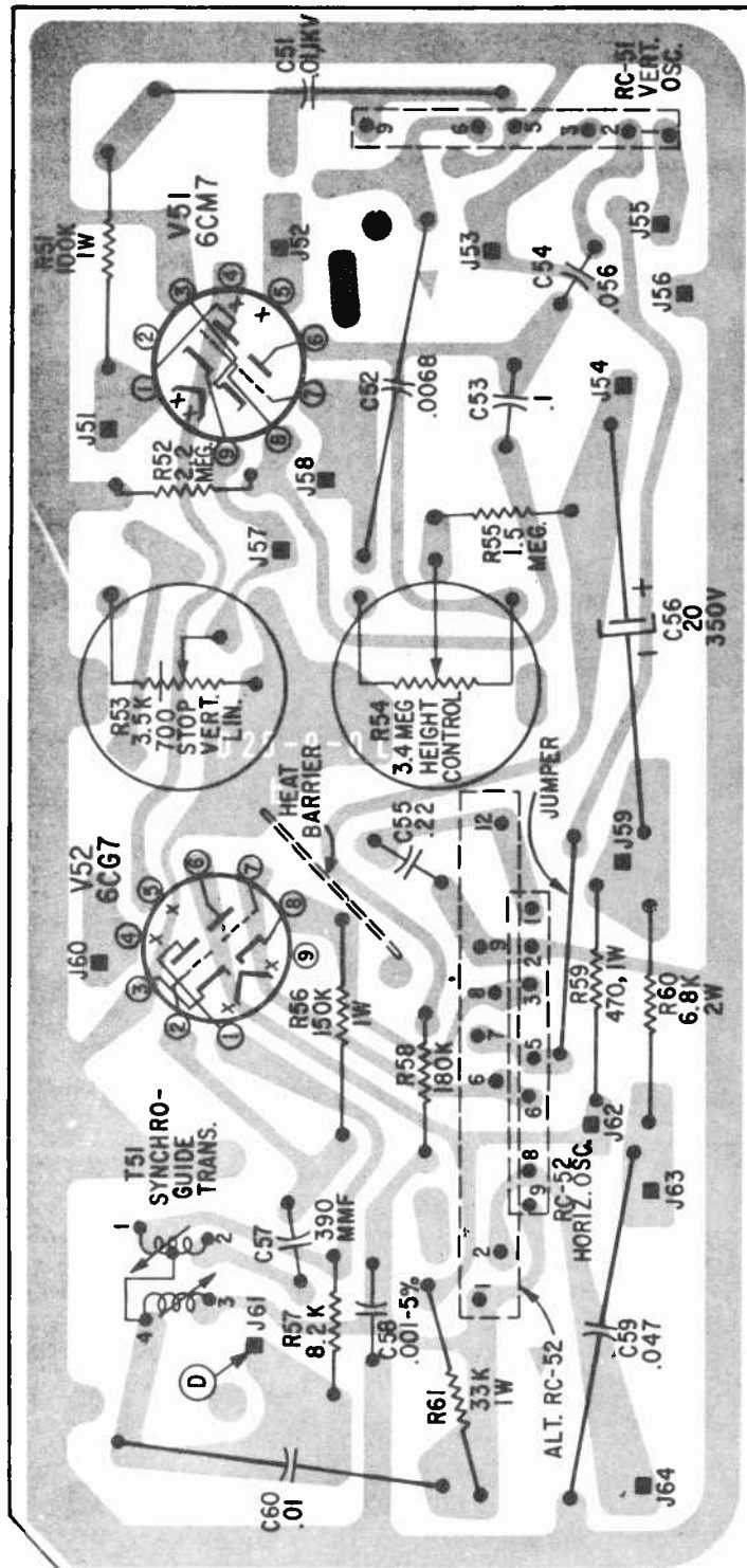
NOTE: WIRING DIAGRAM SHOWN FROM CIRCUIT SIDE VERTICAL-HORIZONTAL OSCILLATOR BOARD, 84-7905-1
