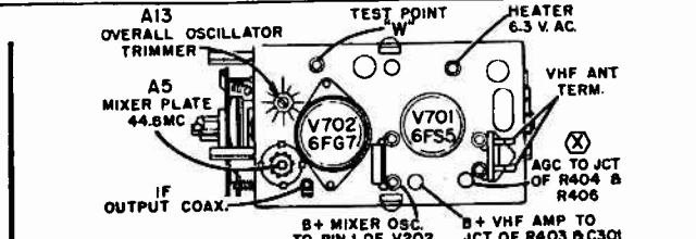
Figure G. Top View of VHF Tuner 94E203-6.
