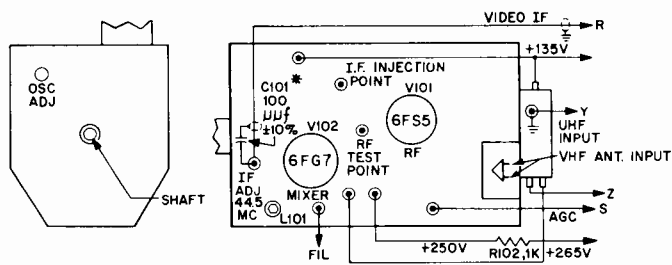
TUNER PART NO. CL28516 (VHF) USED WITH CL28517 (UHF)
