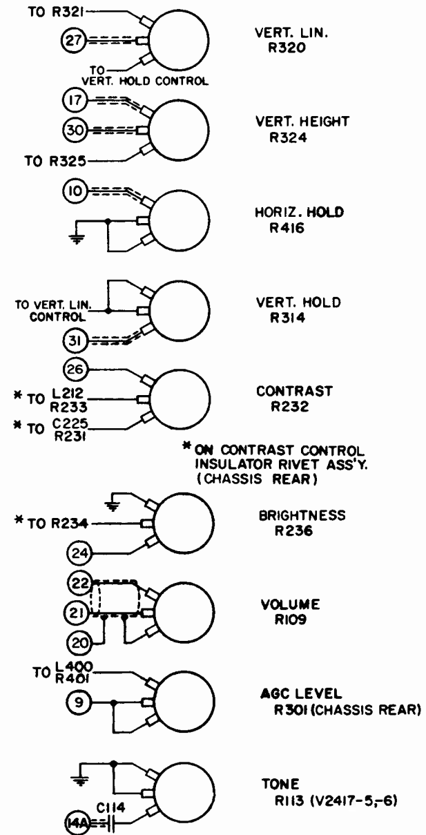
Figure 8 - Control Wiring Diagram All views seen from rear.
