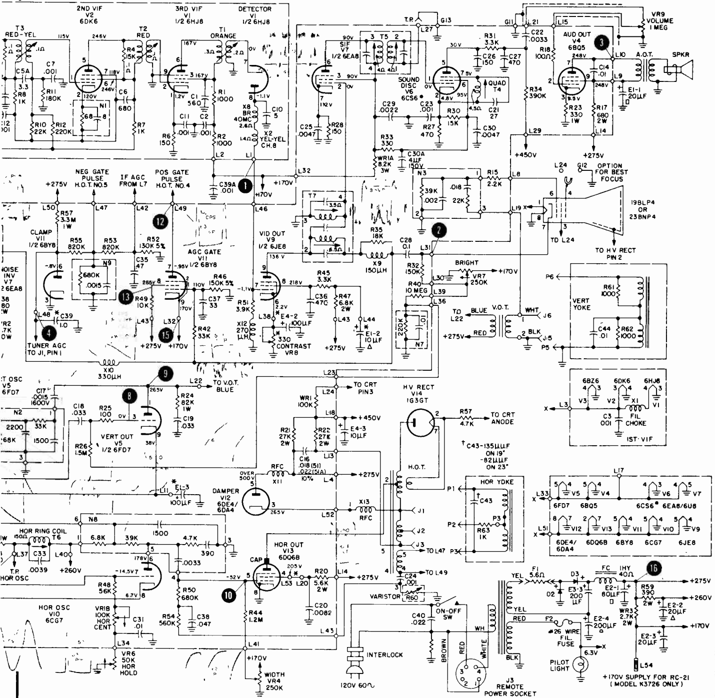
Schematic Diagram - Television Chassis 12N52
