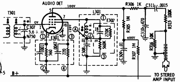
TV CHASSIS AUDIO CIRCUIT FOR STEREO-TV MODELS (CHASSIS QTS & RTS-579)
