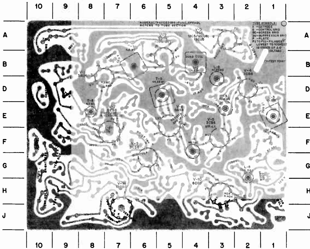
FIG. 3 - ETCHED PRINTED CIRCUIT BOARD CHASSIS (BOTTOM VIEW)
