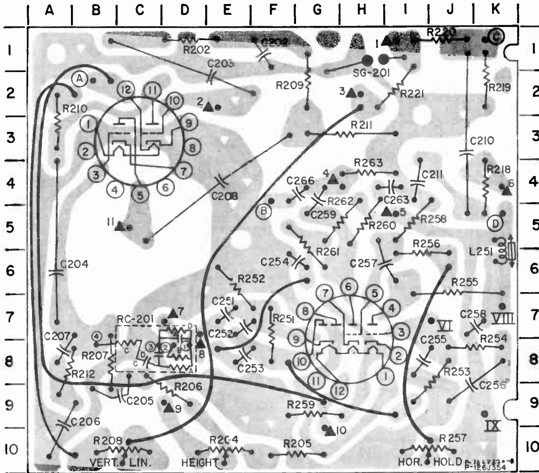
Component view of 19" sweep board w/COMPACTRONS
