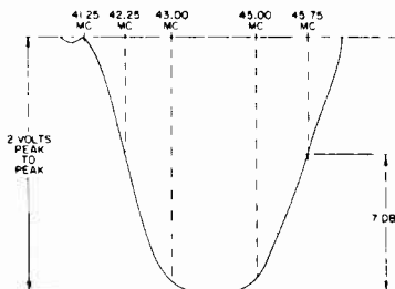
Figure 12 - IF Response: mixer grid to 2nd detector.
