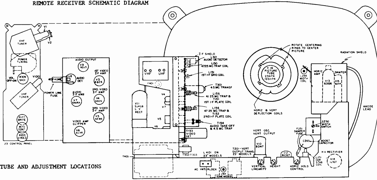
REMOTE RECEIVER SCHEMATIC DIAGRAM
