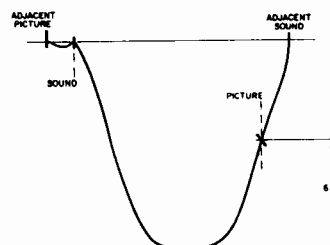
Figure 16 - Typical RF-IF Response.
