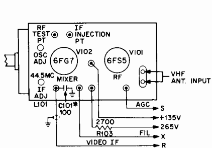
TUNER PART NO. CL28515 (VHF)
