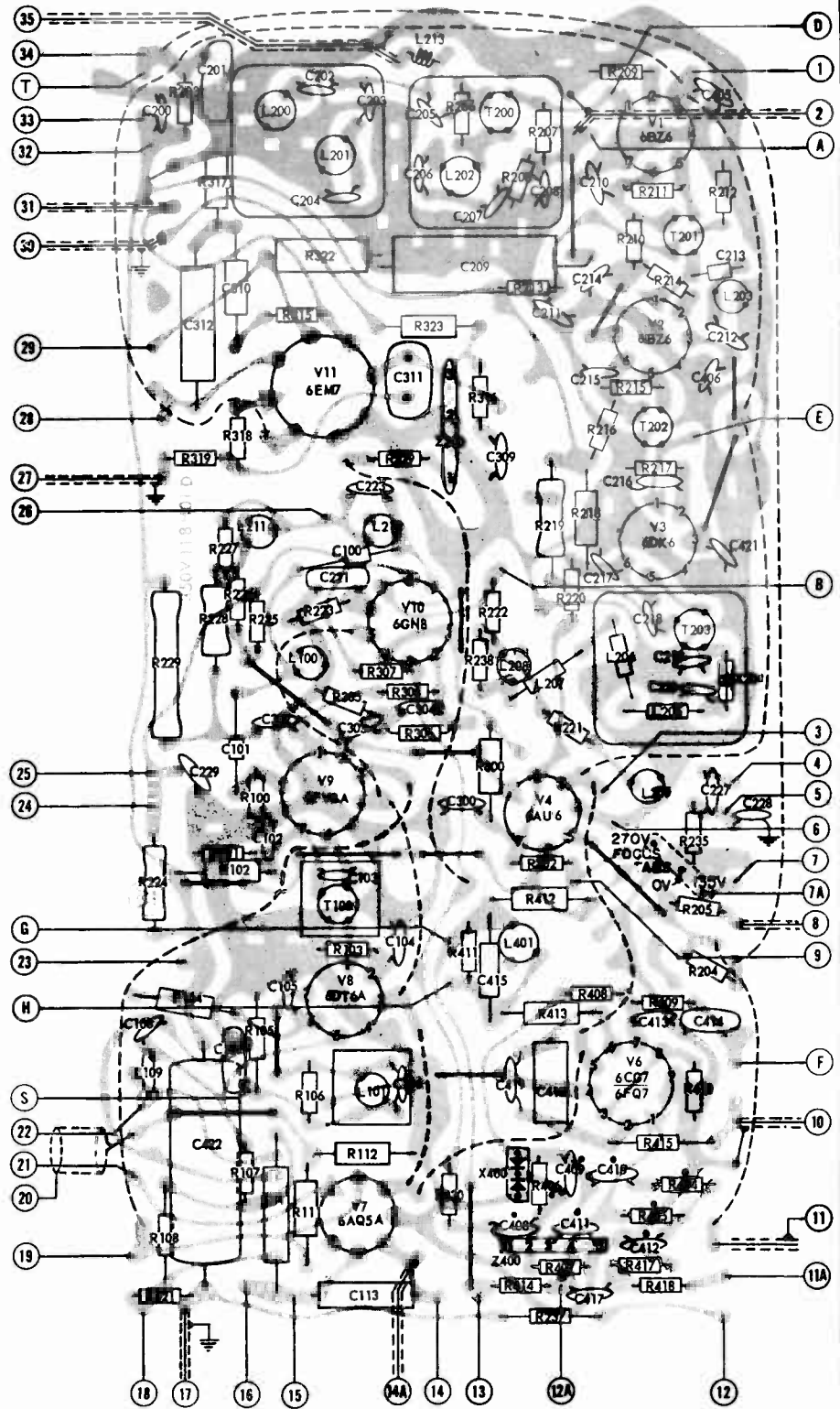
Figure 6 - Bottom view of PC board showing location of top components in solid outlines. Tube pin numbering is for bottom of socket.
