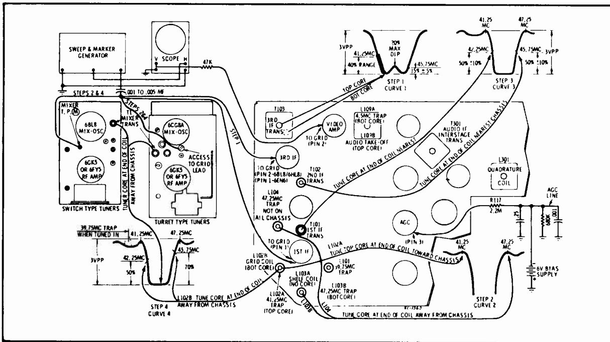
FIGURE 10. VIDEO IF & SOUND ALIGNMENT DETAIL
