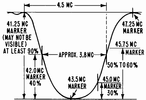
Figure C. Ideal IF Response Curve.
