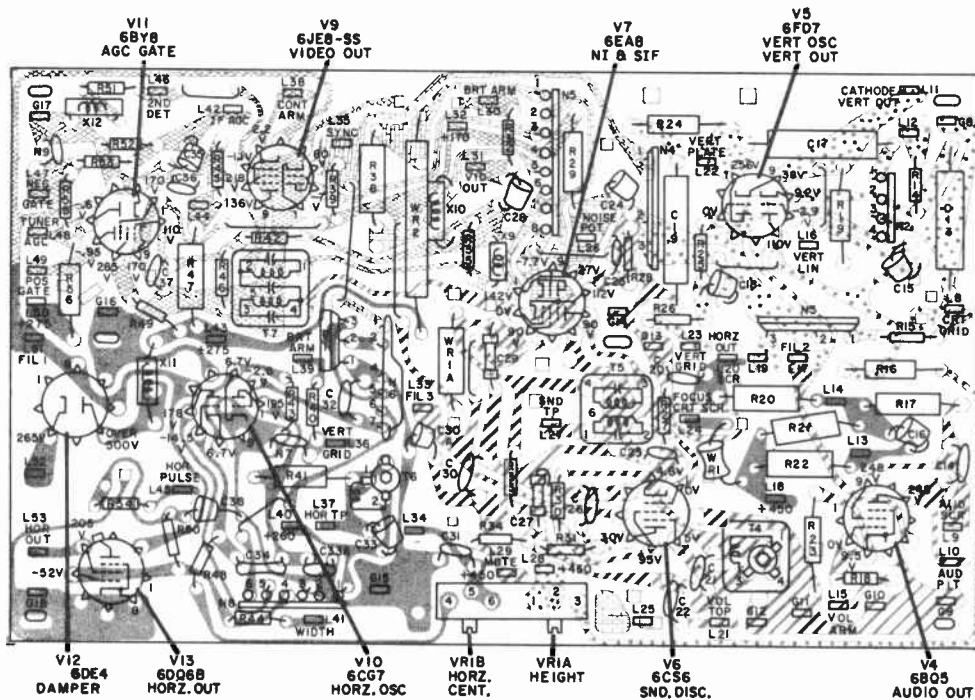
Video IF Perma-Circuit Panel - Top View
