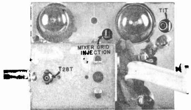
FIGURE 1-3b ALIGNMENT POINTS OF T106 TUNER, TOP VIEW
