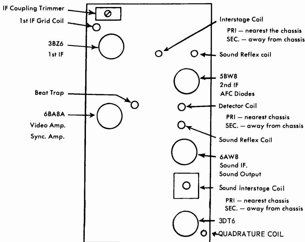
The above diagram represents a top view of the vertical portion of the slimline chassis.
