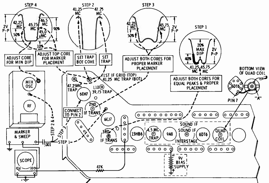
VIDEO IF & SOUND ALIGNMENT DETAIL
