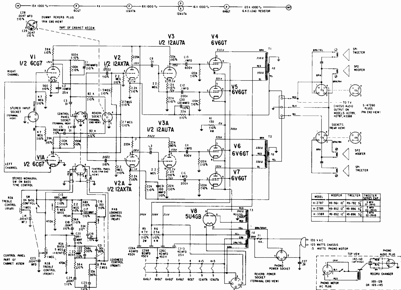
Schematic Diagram 8H30 Chassis.
