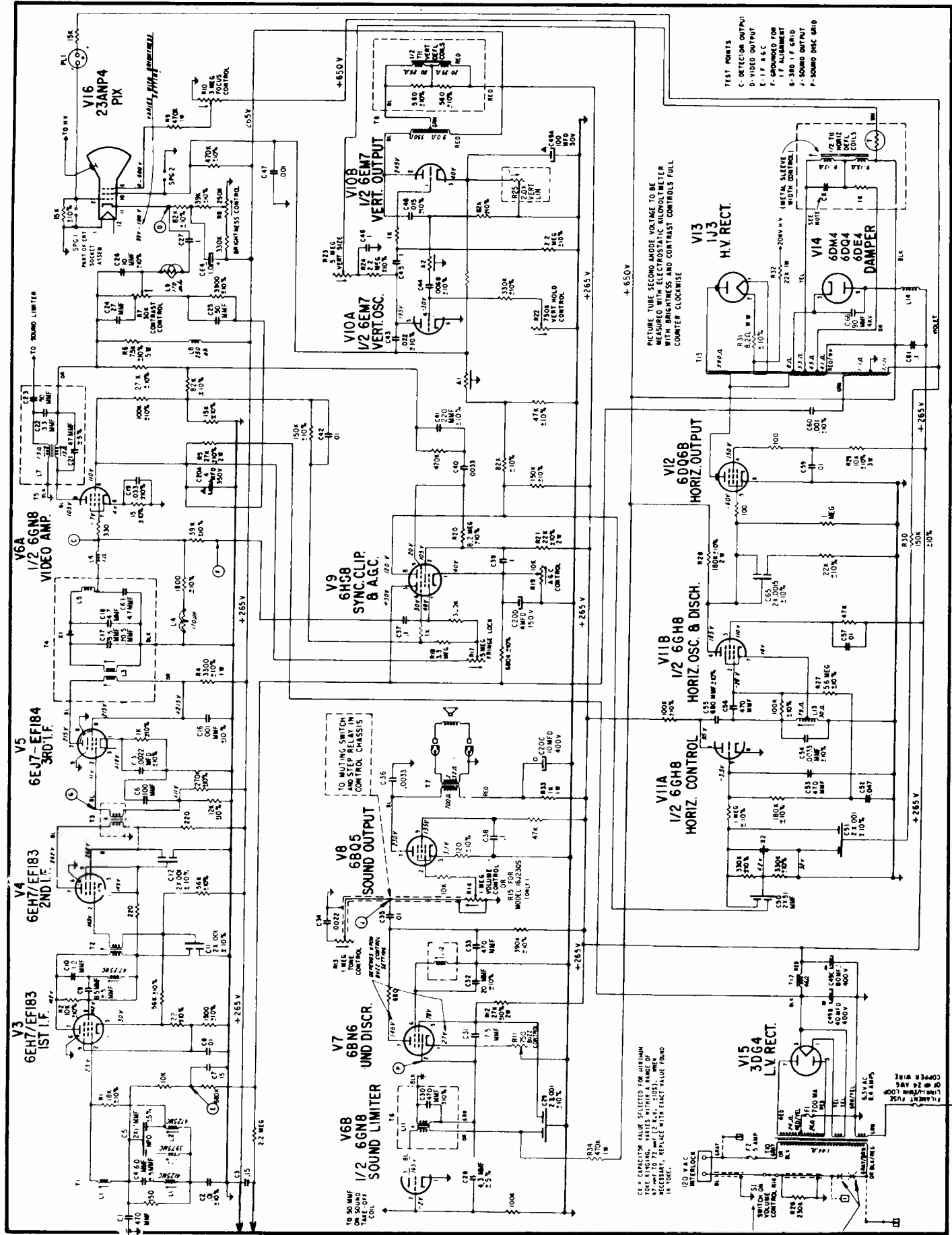
Schematic Diagram, Tube and Trimmer Layout 16J23, 16J23Q and 16J23QS Chassis.
