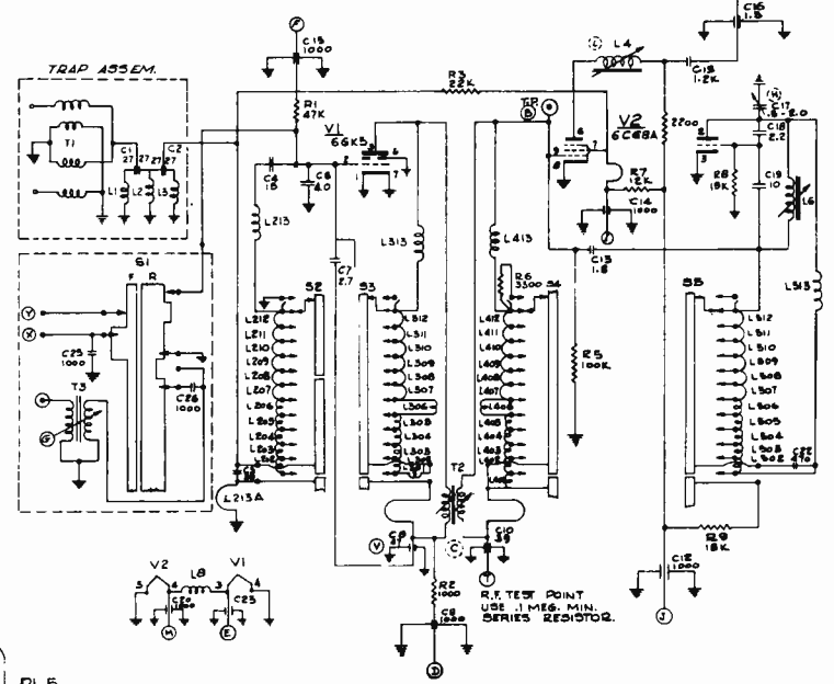
RF TUNER 10711, SCHEMATIC
