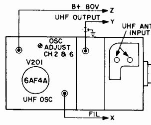
TUNER PART NO. CL28517 (UHF)
