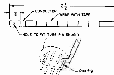
Figure 10 - Mixer coupling gimmick.
