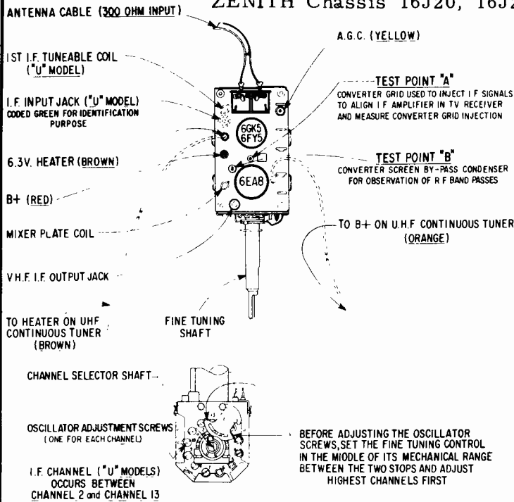
Tube and Trimmer Layout, Bandswitch Tuner.
