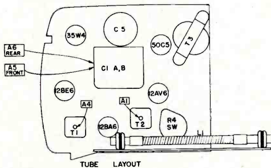
TUBE LAYOUT
