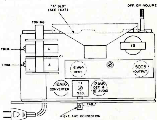
FIG 2 Chassis Layout
