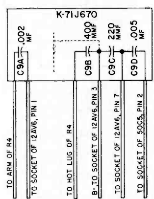
Bulbplate Connections
