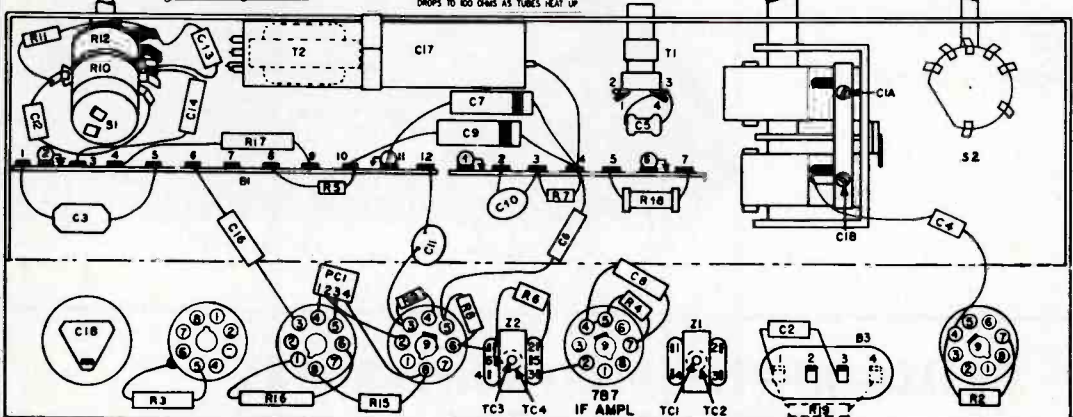
50Y7GT RECTIFIER 35L6GT OUTPUT 7C6 DET. AVC 1ST AUDIO ALIGNMENT CHART 7A8 CONVERTER
