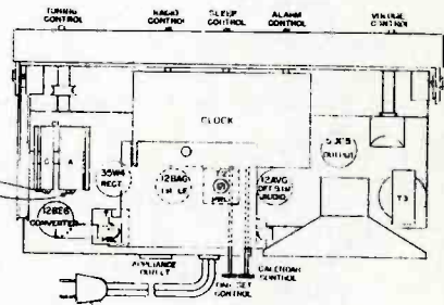
Chassis Layout
