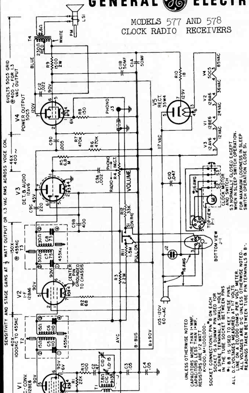
Schematic Diagram, Models 577 and 578
