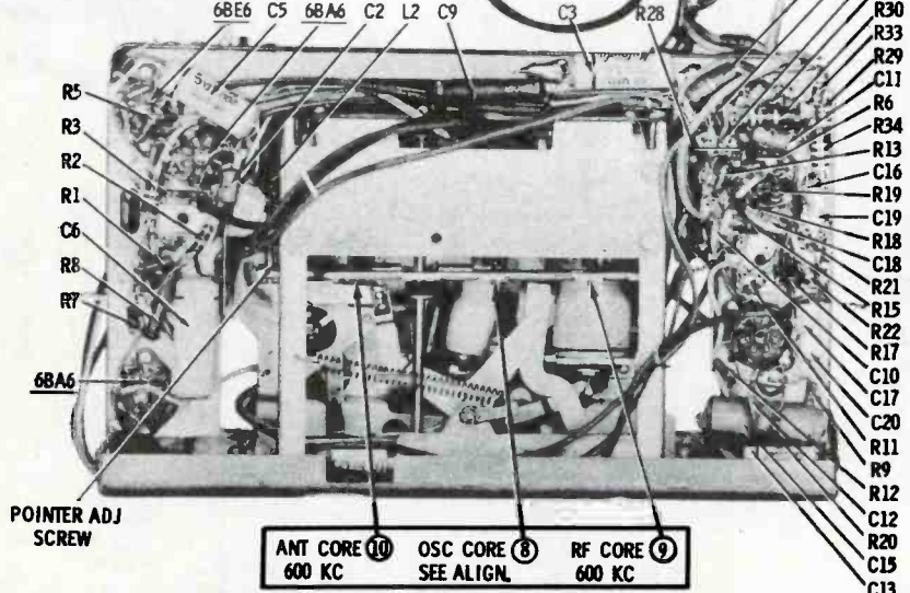
ALIGNMENT ADJUSTMENTS & PARTS LOCATIONS.
