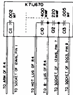
Complete Unit, C10, 11, 12, 13
