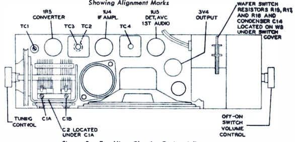
Figure 2. Top View, Showing Tuning Adjustments
