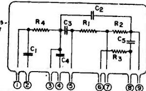
PC-165 WIRING DIAGRAM
