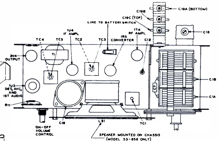
Top View, Showing Trimmer Locations
