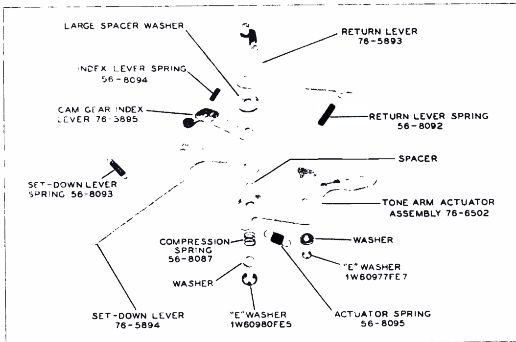
Figure 8. Actuator Assembly
