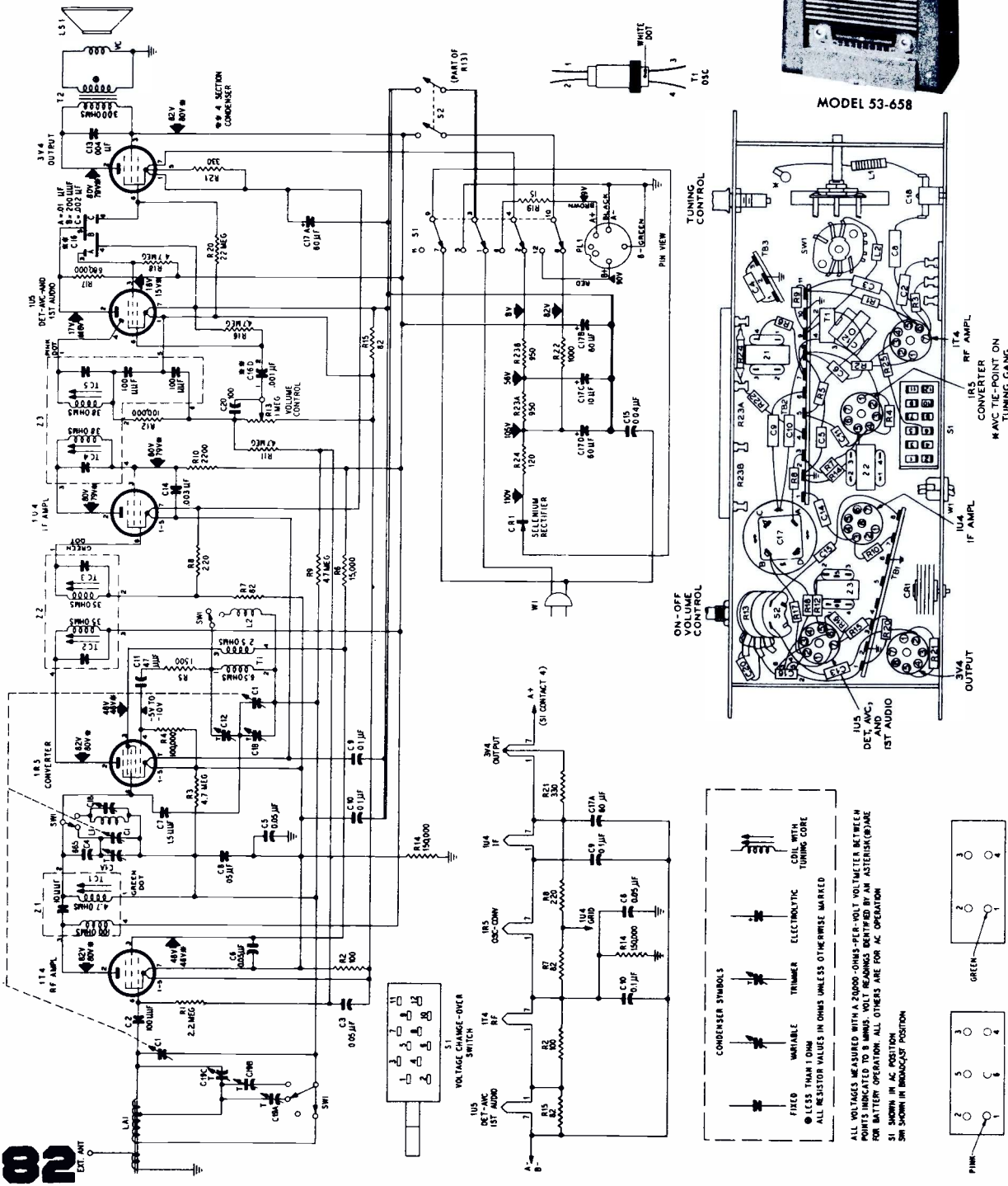
Bottom View, Showing Symbolized Chassis
