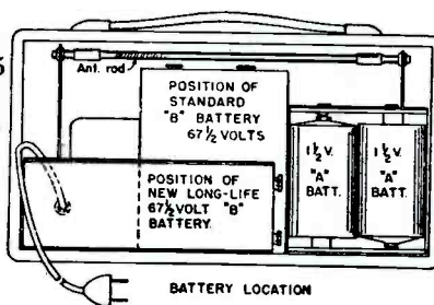
BATTERY LOCATION
