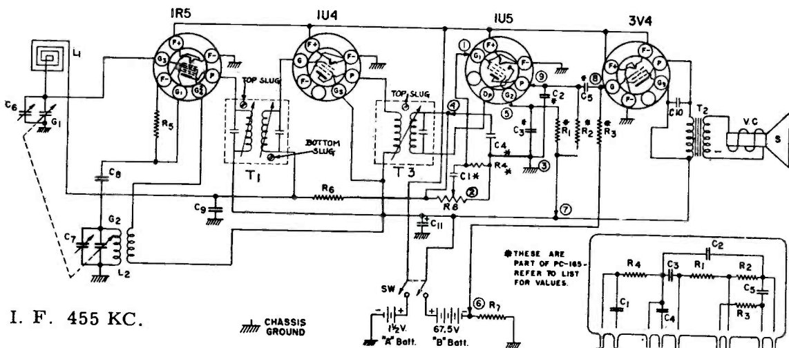
PC-165 WIRING DIAGRAM
