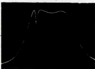
Figure 15-T Video IF response curve: Wobbulator to the grid of V12 and the travelling detector to the oscillograph at the plate of V13. L31 and L32 properly tuned (birdie at 26.4 mc.).
