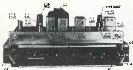
Figure 9. RF-IF Chassis
