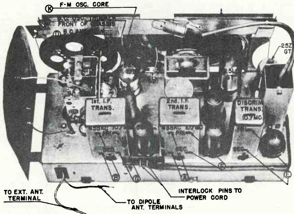
CHASSIS TOP VIEW SHOWING ALIGNMENT ADJUSTMENTS
