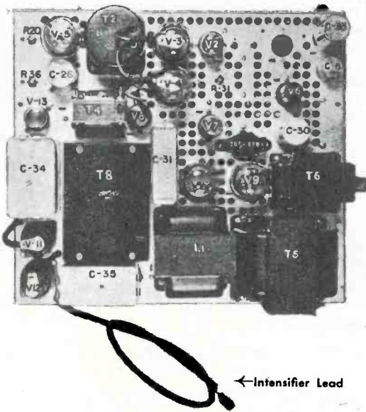
Figure 6. Sweep Chassis
