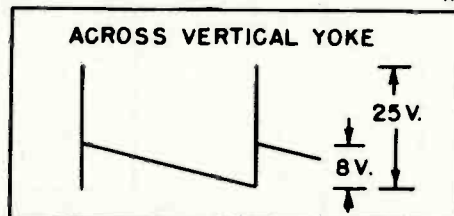
Fig. 55. Vert. Yoke Input (Osc. Synced at Half of Vert. Sweep Speed)
