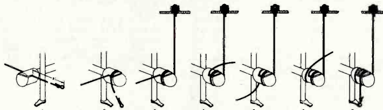
Figure 2—Elevator Windless Stringing Procedure
