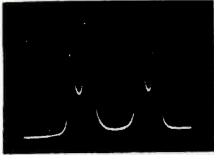
Figure 15-A Oscilloscope of the dual sound IF curve (untuned).
