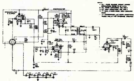
Sync Stabilizer Schematic
