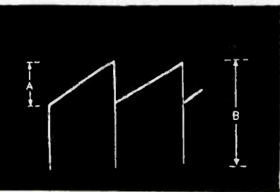
Vertical Deflection Amp Grid Tube V8 Pin 4 A=60 volts B=85 volts
