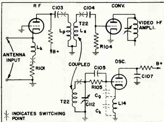
Fig. 2. R-f Amplifier, Converter & Oscillator
