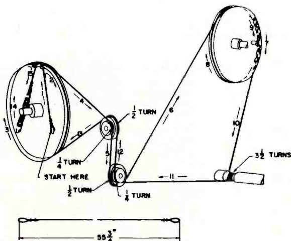
Fig. 15. Radio Tuning, Dial Drive Stringing
