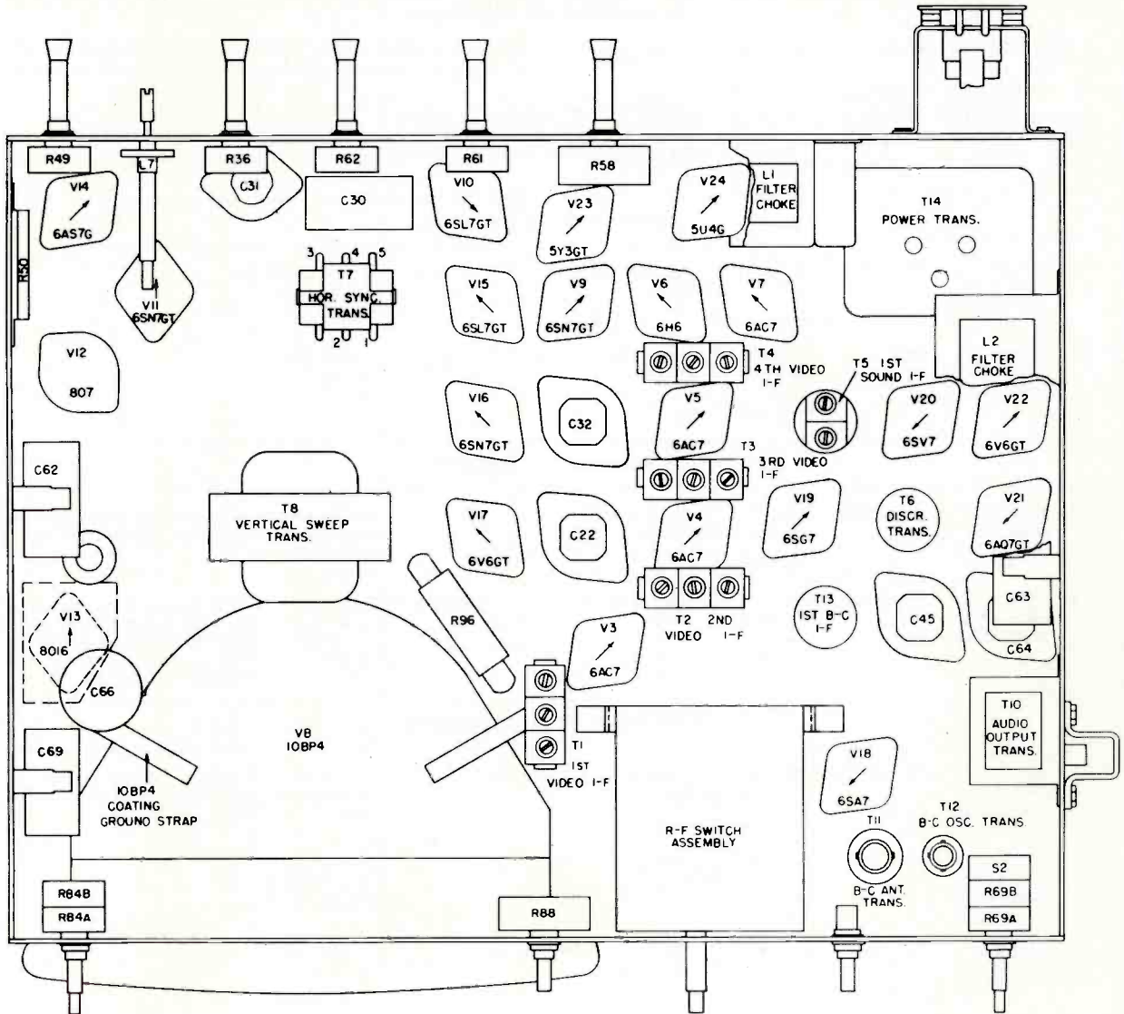
Fig. 14. Component Location, Bottom View of Chassis
