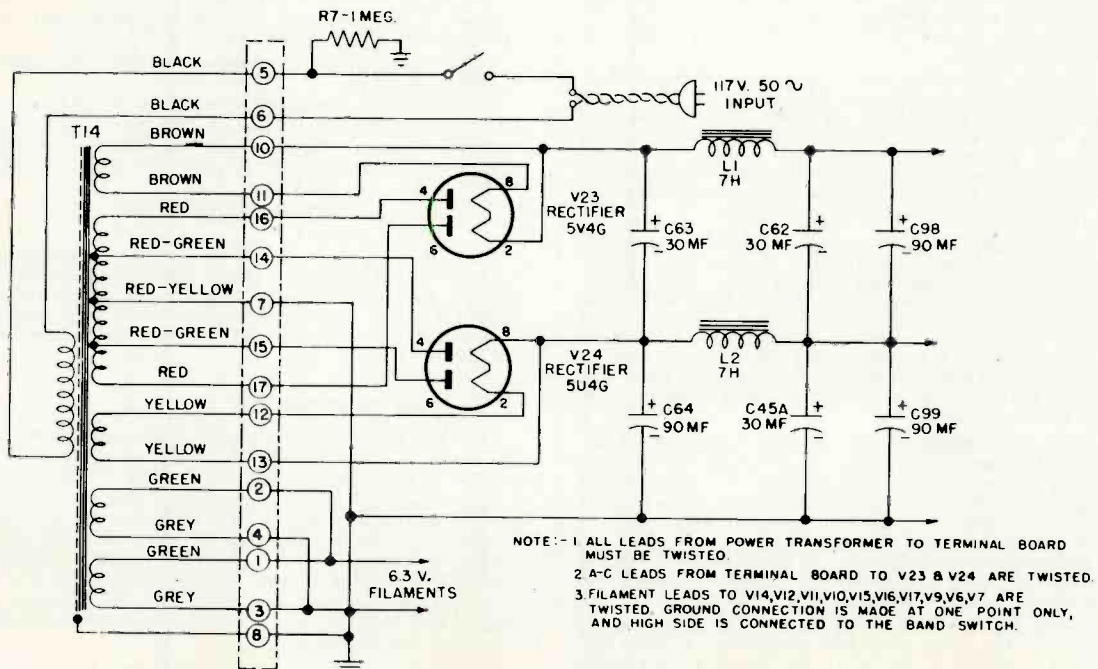
Fig. 18. Schematic Changes for 50-cycle Operation
