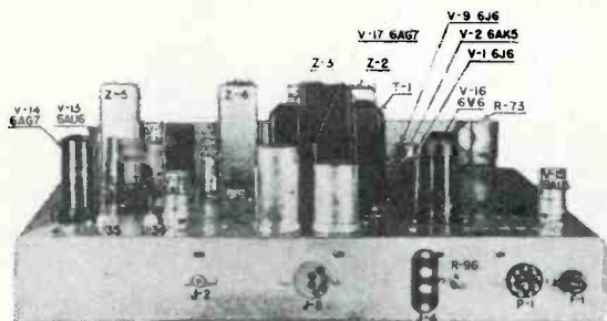
Figure 8. RF-IF Chassis
