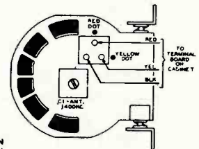
Fig. 9 Loop antenna
