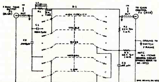
Tone Selector Schematic
