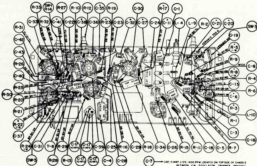
Bottom View — Parts Layout
