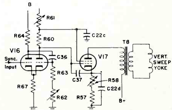
Fig. 7. Vertical Sweep Output
