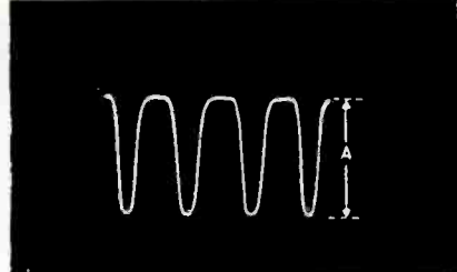
Oscillator Plate Tube V3 Pin 3 A=52 volts
