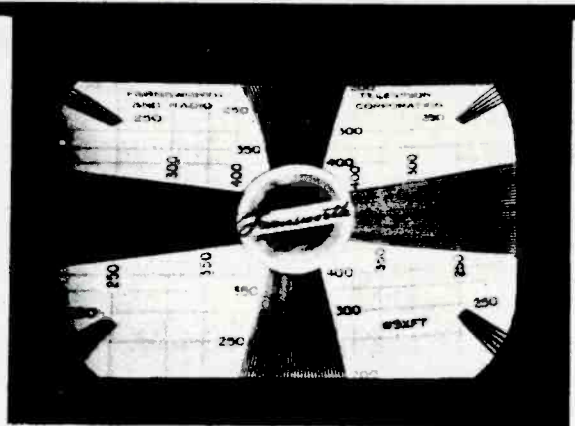
32f Height control too low
