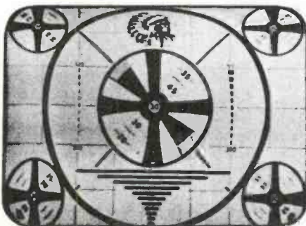
Fig. 26. Vertical Linearity Control Misadjusted
