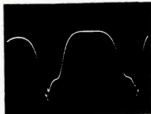
Figure 15-M Video IF response curve: Wobbulated signal generator at the grid of V14. Oscilloscope at the cathode of V16. Birdie at 26.4 mc.
