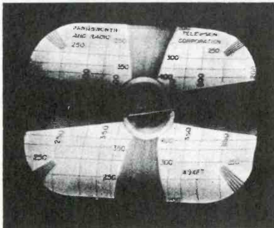
32c 120 cycle hum in video and in H. scan
