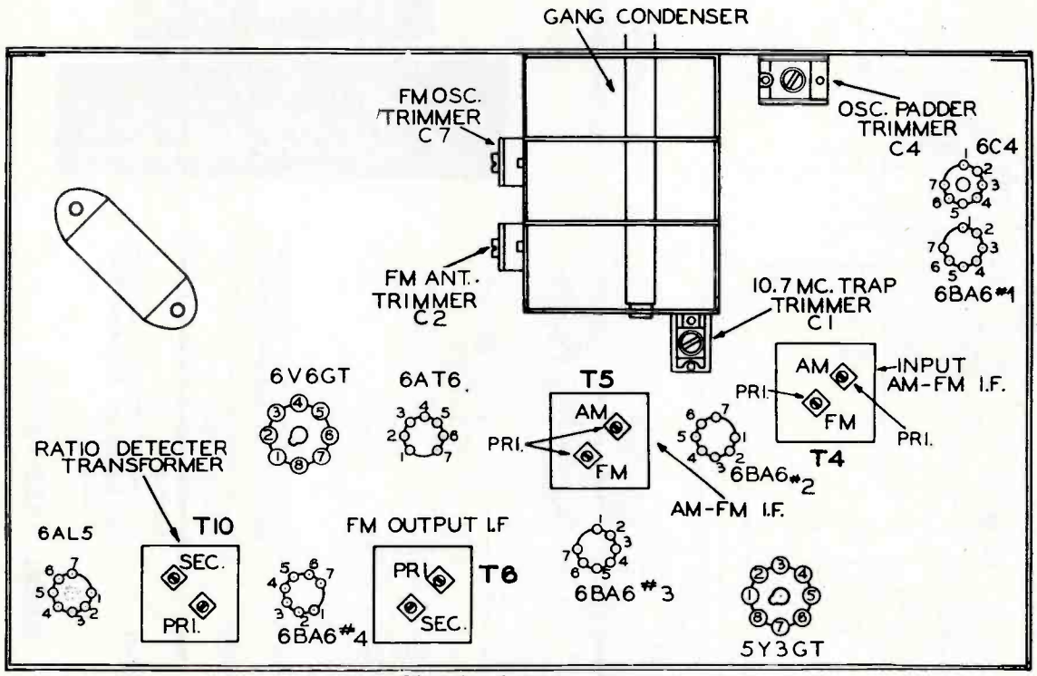
Chassis—bottom view
