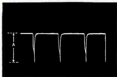
Damping Tube Plate Tube V5 Pin 2 A=450 volts
