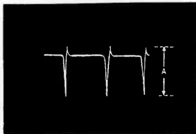
Sync Amplifier Grid Tube V2 Pin 1 A=4.5 volts
