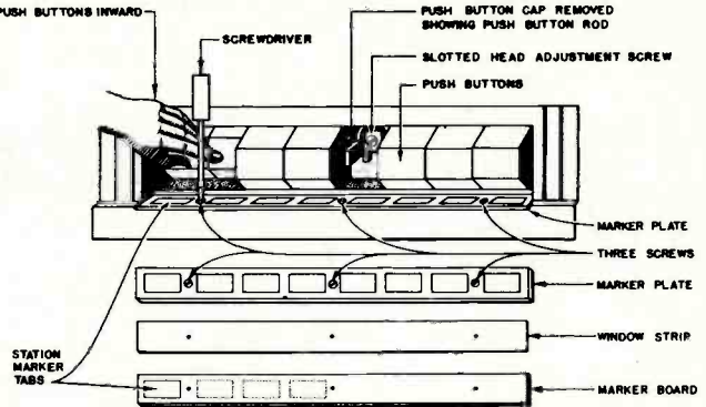
Fig. 15 Push-Button set-up
