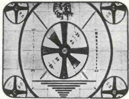
Fig. 29. Vertical Height Control Misadjusted
