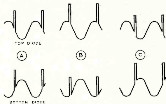
Figure 8—Sync Discriminator Waveforms
