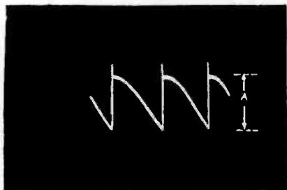
Vertical Amp Plate Tube V8 Pin 2 Sweep Non-Linear Due to Extreme Position of Controls A=125 volts
