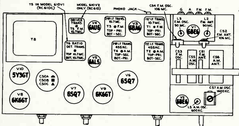
Top View Chassis
