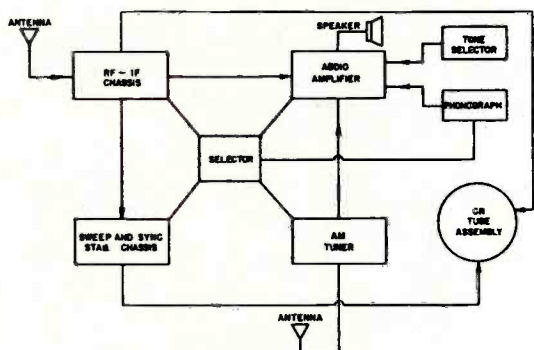
Figure 1. Block Diagram of RA-101 Receiver
