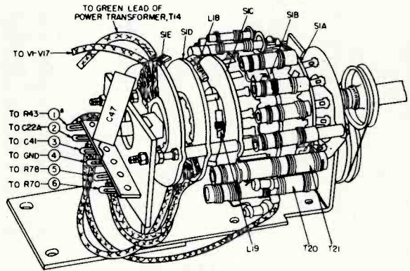
Fig. 12. R-F Coil & Switch Assembly
