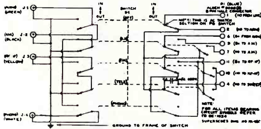
Service Selector Schematic
