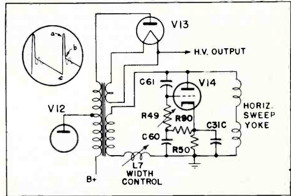
Fig. 6. Horizontal Sweep Output
