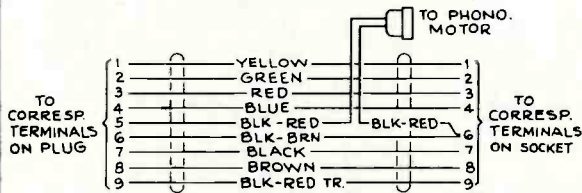
Fig. 15 Power Cable
