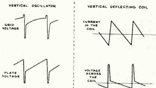
Figure 7—Vertical Sweep Waveforms
