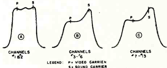
Fig. 11. R-F Alignment Curves
