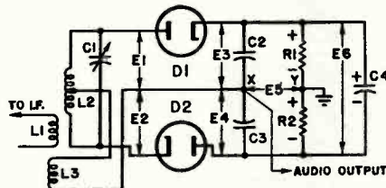
Fig. 4. Ratio Detector Circuit
