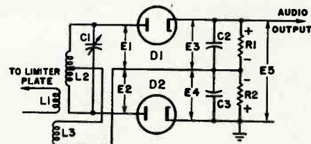
Fig. 3. Discriminator Circuit
