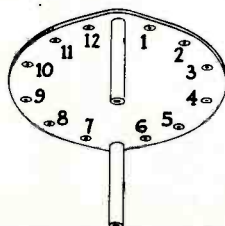
Figure 5—Identification of Switch Wafers —Set Inverted and Viewed from Panel
