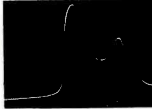
Figure 15-H Oscilloscope showing a slight amount of overload caused by too much signal from the wobbulated signal generator.
