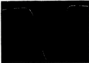
Figure 15-G Oscilloscope of overall sound IF response. (The improper alignment is due to the different amplitude of the signal now being applied to the grids of each stage.) (Birdie at 21.9 mc.)
