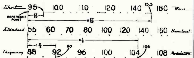
Fig. 10 Dial scale drawing
