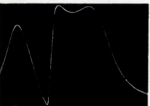
Figure 15-Y Sound trap too low.
