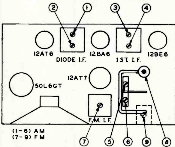
TRIMMER LOCATION CHART
