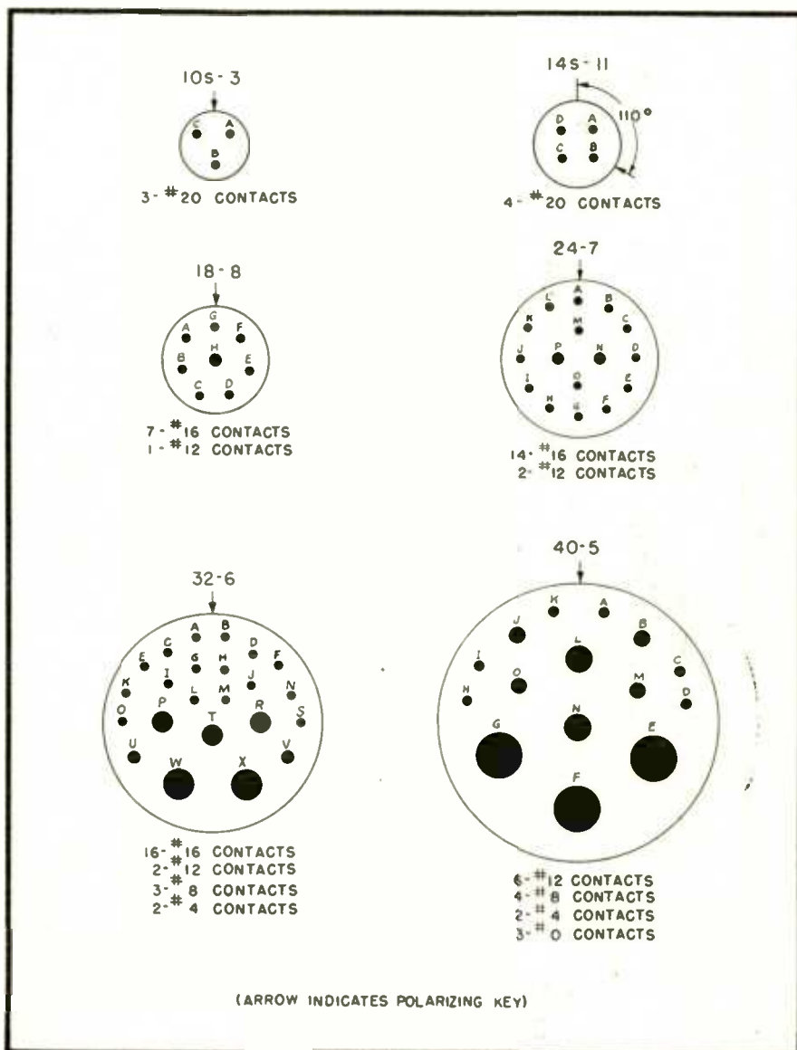
Fig. 4. Typical insert arrangements
