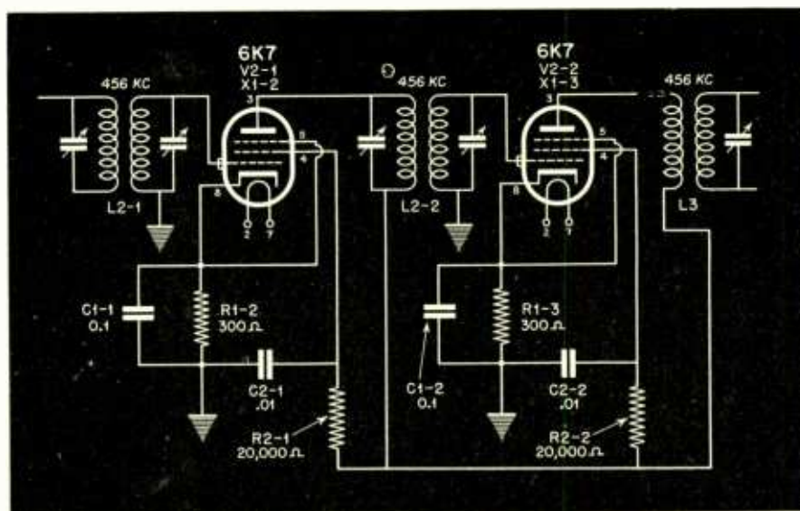
Fig. 5. Schematic diagram with component values and reference numbers as used in instruction manual
