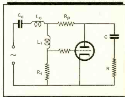
Fig. 4. Harmonic generator
