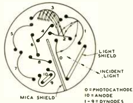
Structure of 1P21 Phototube
