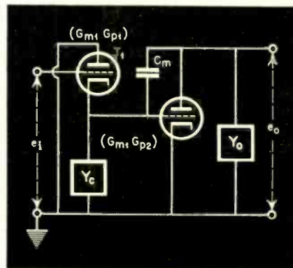
Fig. 2. Equivalent circuit for r-f driver and amplifier stages
