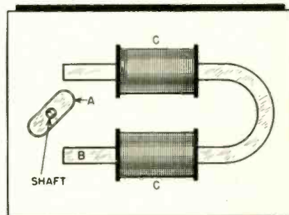
Fig. 2. Inductor-type alternator
