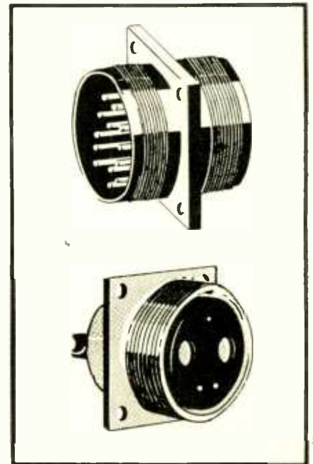
Fig. 2. Above, Type RA (AN 3100) and, below, Type RB (AN 3102) receptacles
