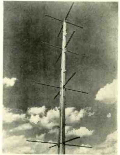
FM Turnstile Antenna
