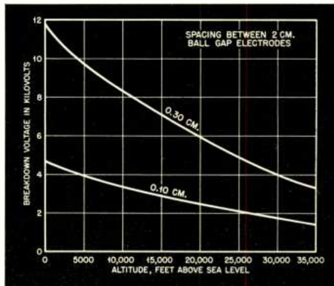
Fig. 2. Breakdown voltage and altitude relation
