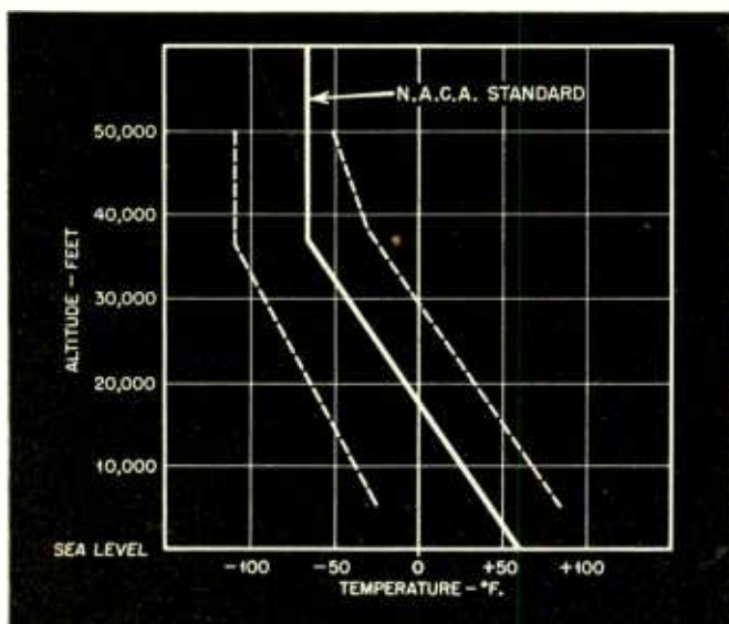
Fig. 1. Variation in temperature with altitude
