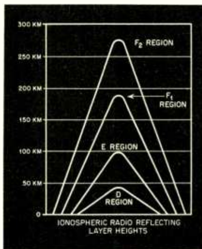
Fig. 3. Ionospheric radio reflecting layer heights
