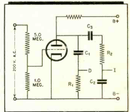
Fig. 3. Differentiating circuit
