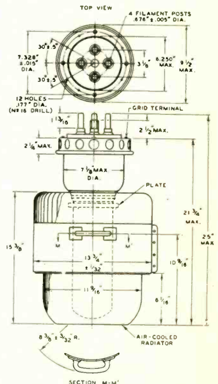
The 9C22 High-Power Triode
