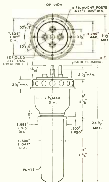
The 9C21 High-Power Triode
