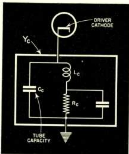
Fig. 6. Elements of driver cathode circuit
