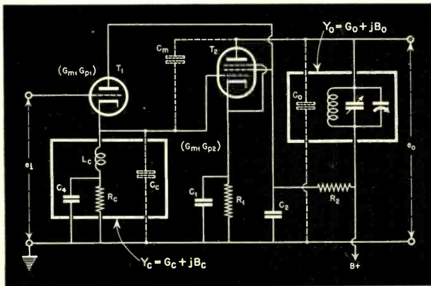
Fig. 1. High transconductance tube with driver
