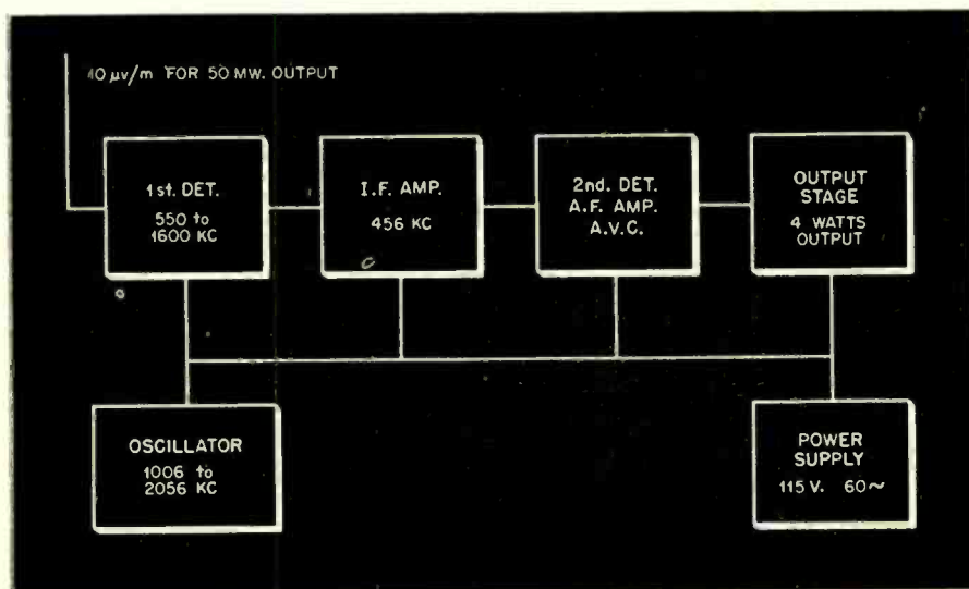
Fig. 4. Block diagram of typical receiver with data for selecting tube types
