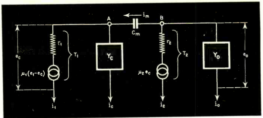
Fig. 3. Equivalent circuit for small r-f voltages
