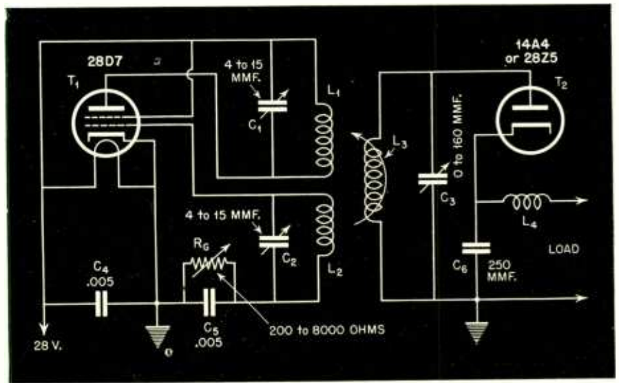
Fig. 1. Schematic of rectified power oscillator. L_1 and L_2 are wound on thin form, 1\frac{1}{8} " diameter. L_1 consists of 10 turns of No. 14 wire, winding length 1\frac{1}{8} ". L_2 —14 turns of No. 14, 1\frac{1}{2} " long. L_3 —various (see curves), 1" diameter, close-wound enameled wire. L_4 —20 turns of No. 20, \frac{1}{4} " diameter, 1" long.
