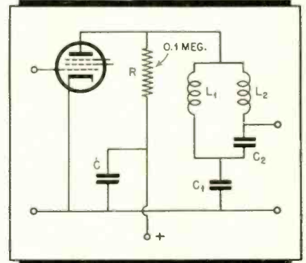
Fig. 1. Wide-band i-f circuit
