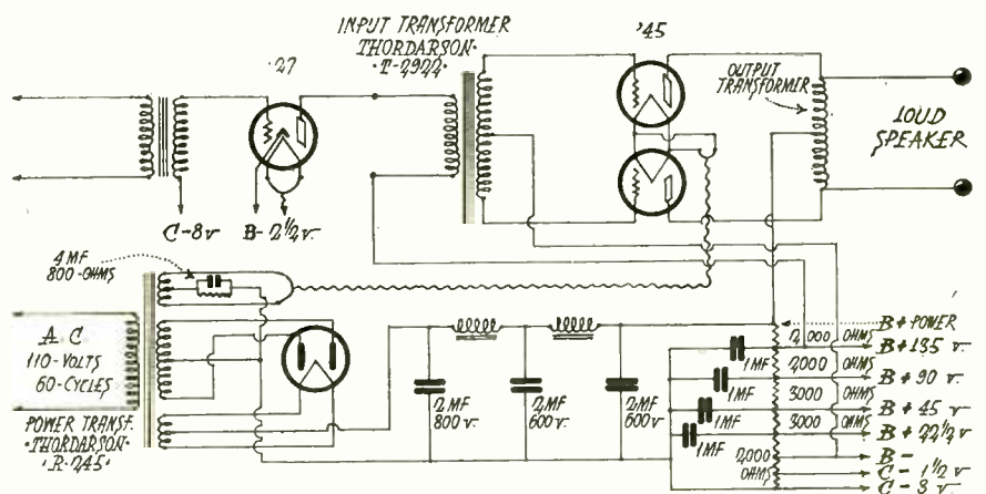
Circuit Diagram of Thordarson R-245 Amplifier
