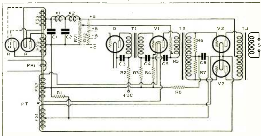
Fig. 1. Push-Pull Power Amplifier Employing Resistance-Capacity Filter
