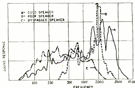
Examples of Loudspeaker Characteristics
