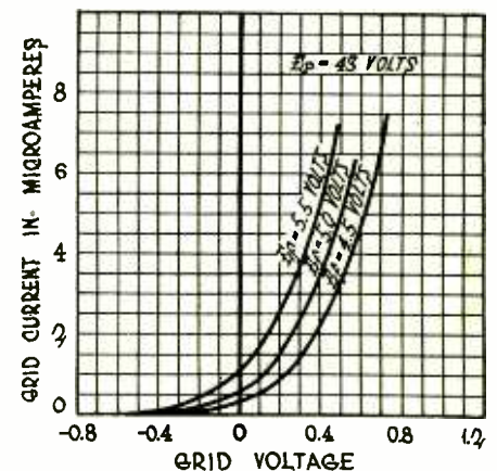
Fig. 3. Effect of Filament Temperature Upon the Grid Current of an '01-A Tube
