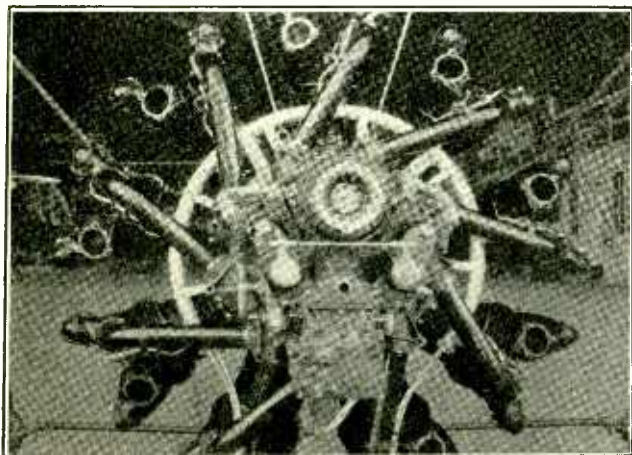
Complete Harness for Motor, Showing Flexible Terminals to Magnetos
