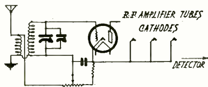
Fig. 3. A Satisfactory Circuit for Manual Control of Volume
