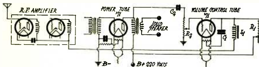
Fig. 1. Williamson's Form of Automatic Volume Control
