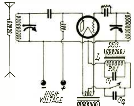
Circuit for Preventing Key Click
