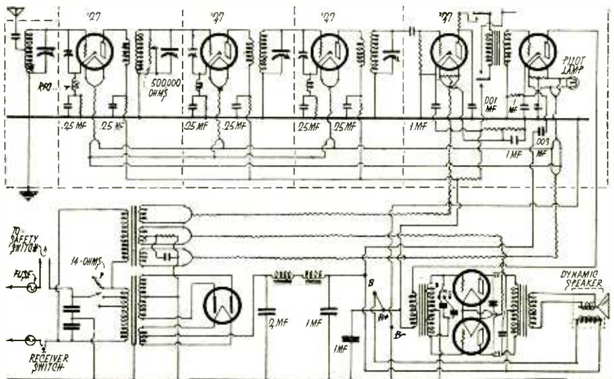
Circuit Diagram Federal Type "M" Receiver
