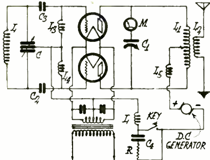
Fig. 2. Push-Pull Transmitter for D.C. Operation
