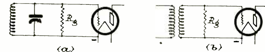
Fig. 2. Effective Shunted Resistance Caused by Grid Current in R.F. and A.F. Amplification Circuits
