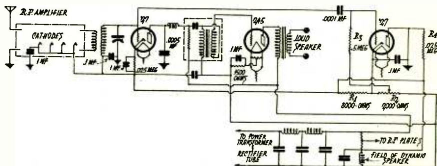
Fig. 2. Automatic Volume Control, Depending Upon Strength of R.F. Carrier Signal
