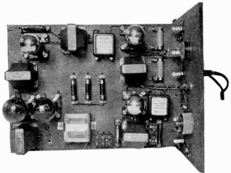
Audio Amplifier Section of System
