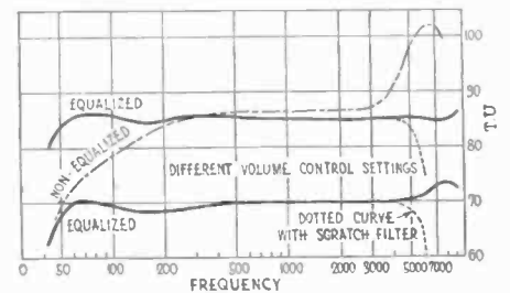
Fig. 2. Frequency Characteristics of System
