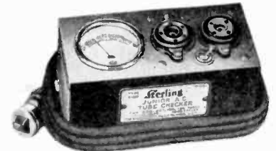
Sterling Junior A.C. Tube Checker.
