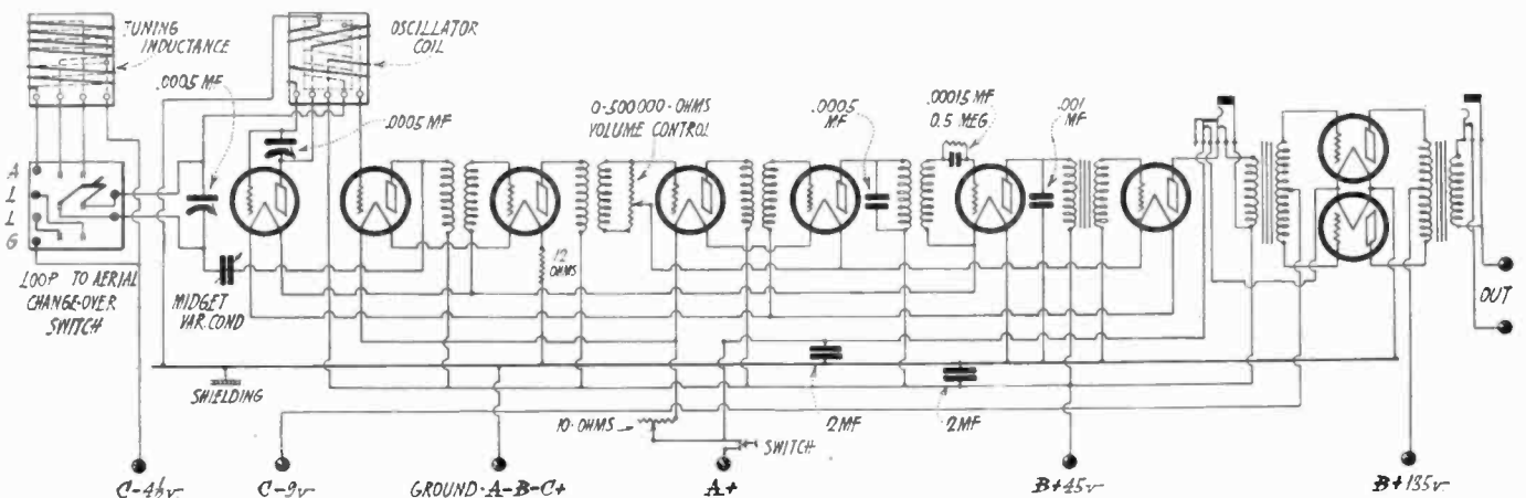
Fig. 2. Circuit of Northern Electric 9-Tube Superheterodyne
