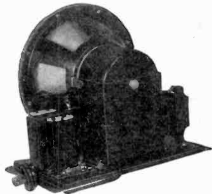
Model NH-3 Dynamic Cone Chassis.
