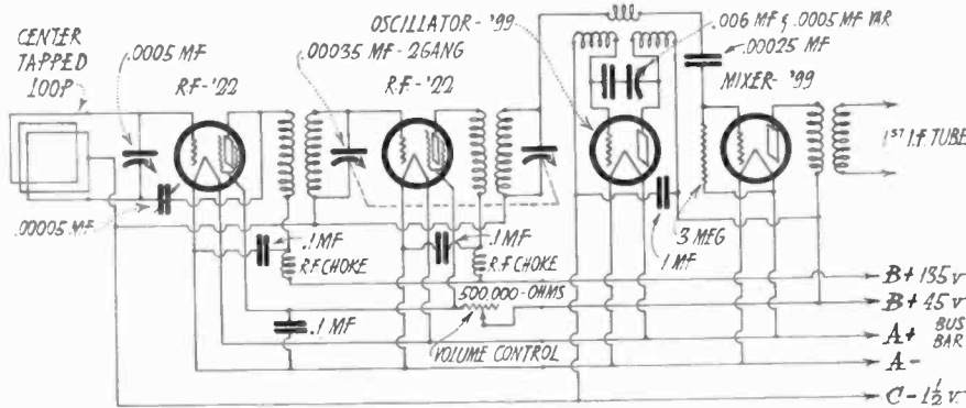
Fig. 1. Circuit of R.F. Amplifier for 45-Kilocycle Superheterodyne
