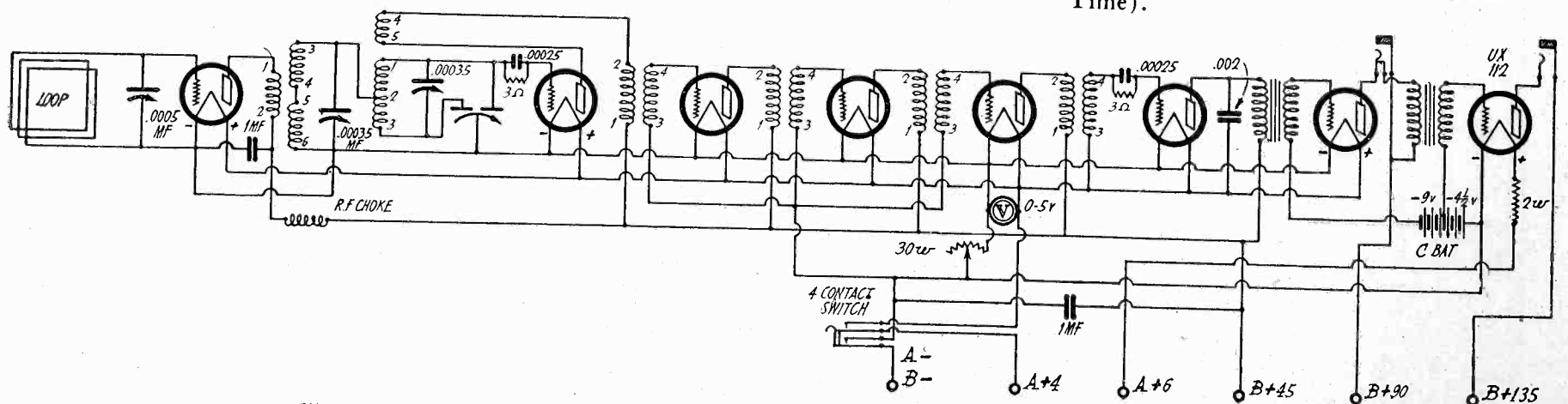
Fig. 2. The Pressley Superheterodyne With Stage of R.F. Amplification Added.
