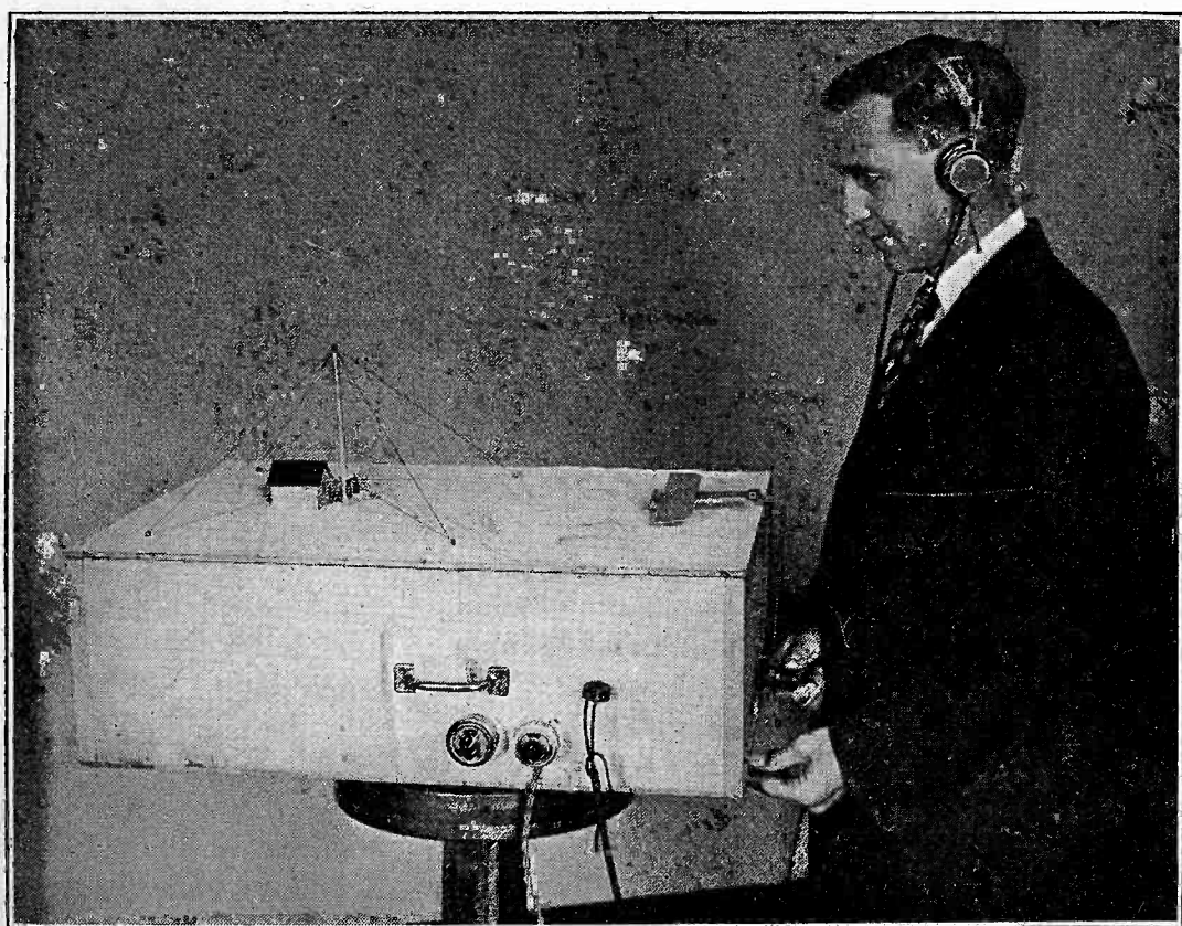
Model of Double Beam Radio Beacon for Guiding Aircraft.
