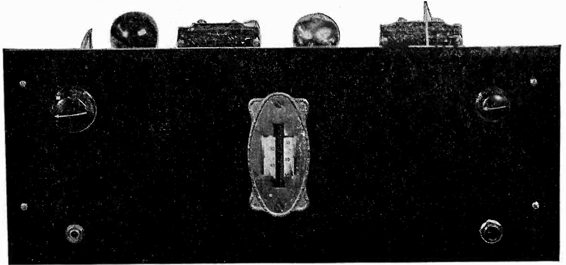
Panel View, Showing Drum Type Dials.
