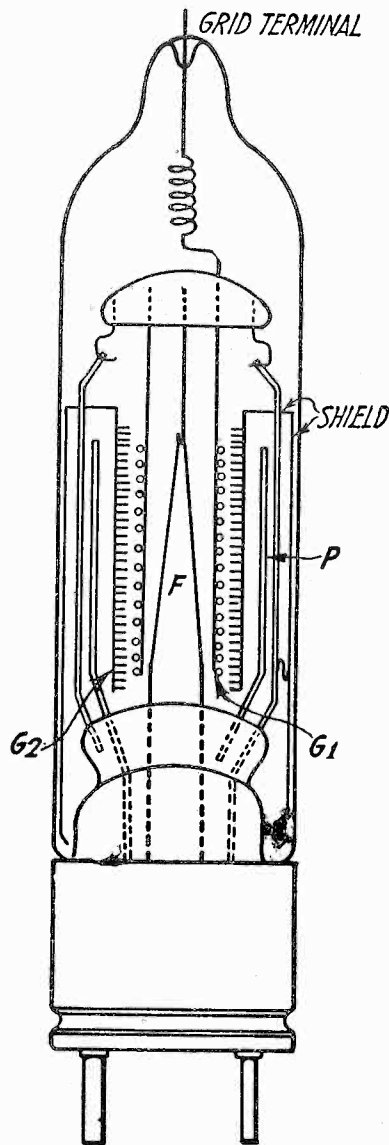
Fig. 1. Structural Details of the Shielded Grid Tube.
