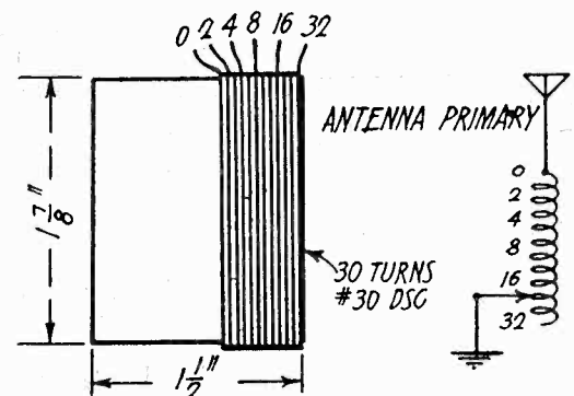
Fig. 3. Antenna Coil.
