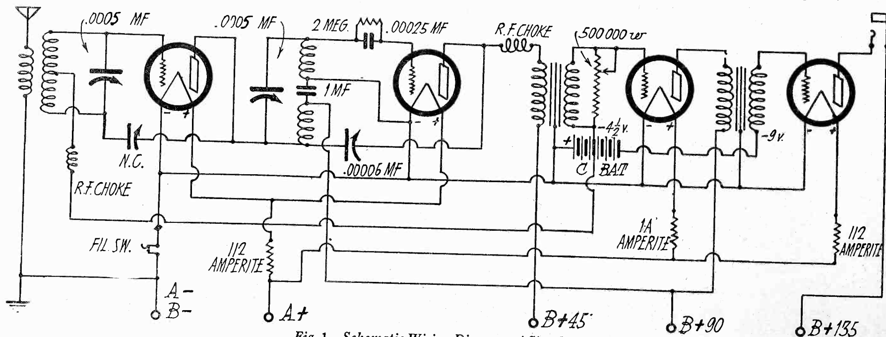
Fig. 1. Schematic Wiring Diagram of Simplicity Receiver.
