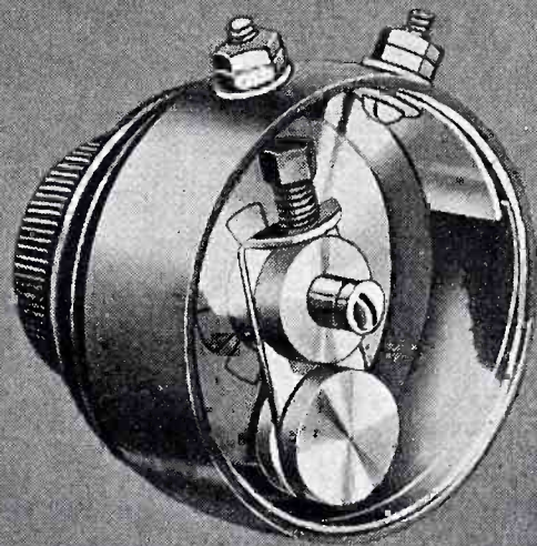
FROST-RADIO Type 886 Super-Variable High Resistance Price $1.50
