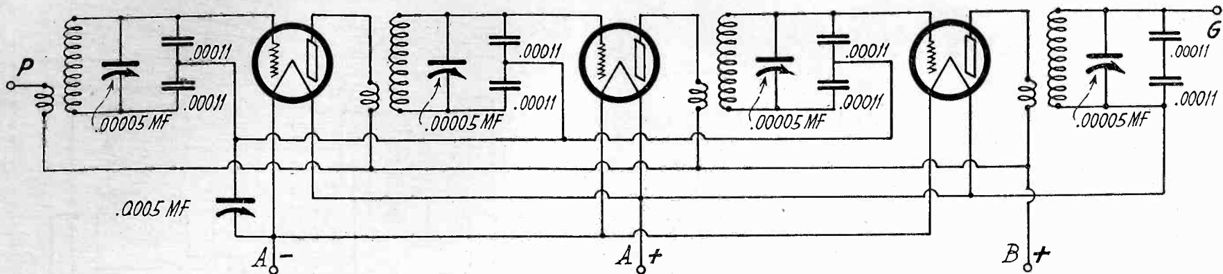
Fig. 4. Circuit Diagram of Infradyne Amplifier Unit.
