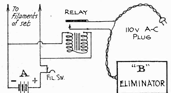
Fig. 4. Circuit Connections for Shunt Relay.
