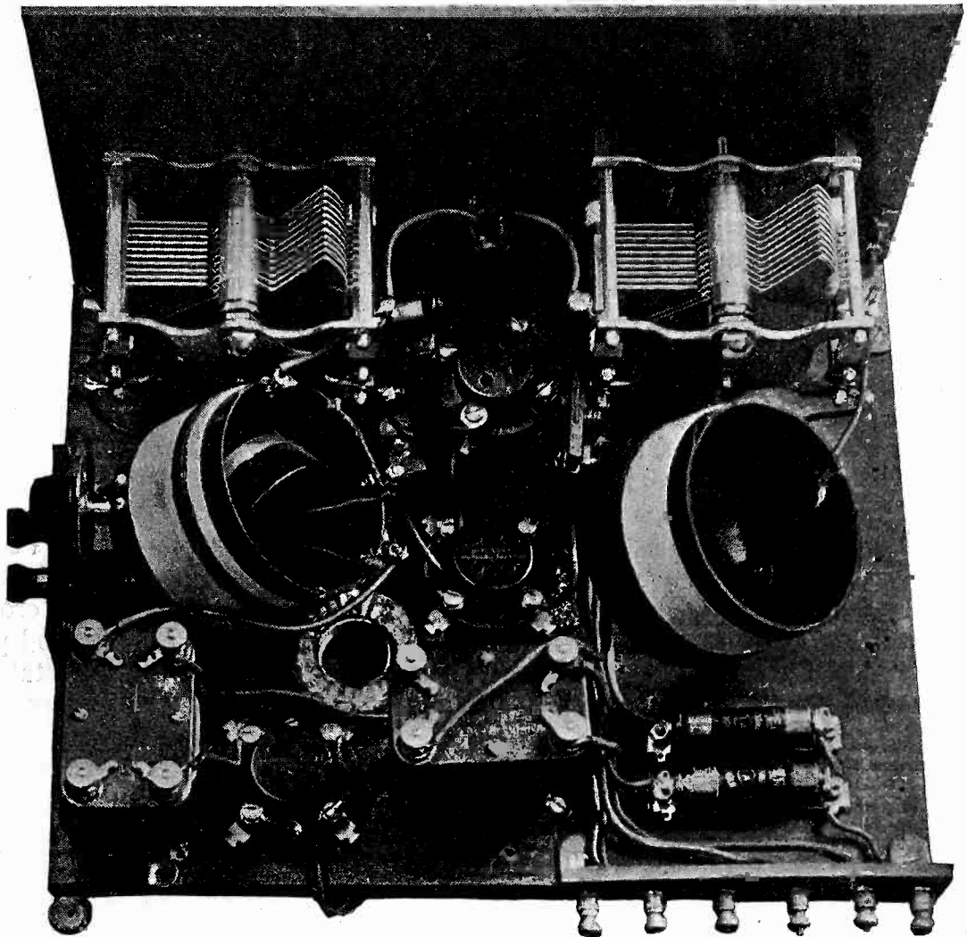
Rear View of Three-Tube Experimental Set.
