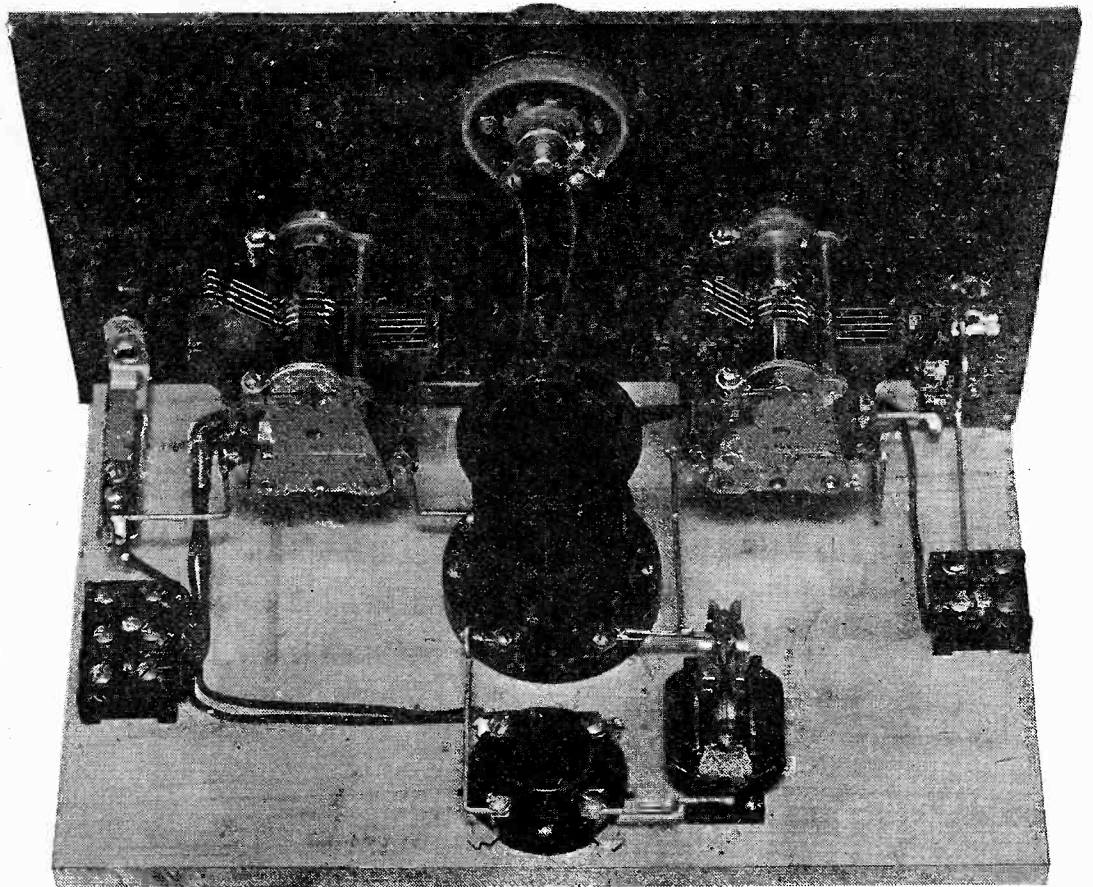
Completed Short Wave Receiver.
