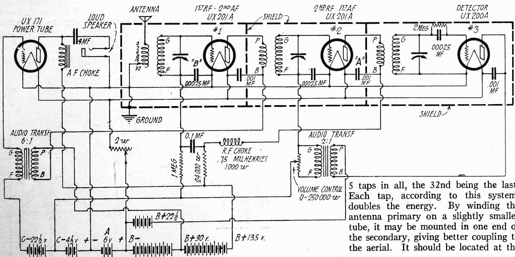
Fig. 1. Circuit Diagram of New Grimes Inverse Duplex.
