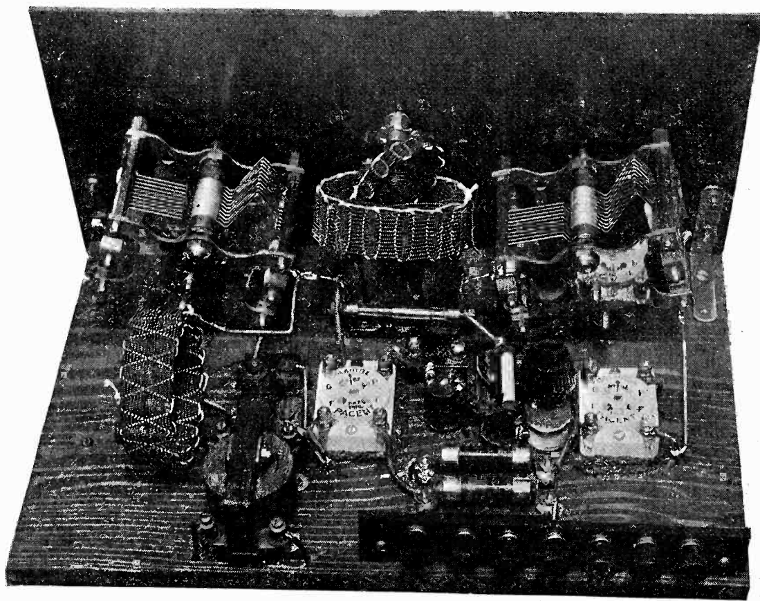
Rear View of Two-Tube Experimental Set.
