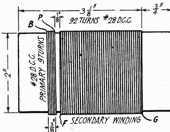
Fig. 4. Intermediate Tuning Coil.
