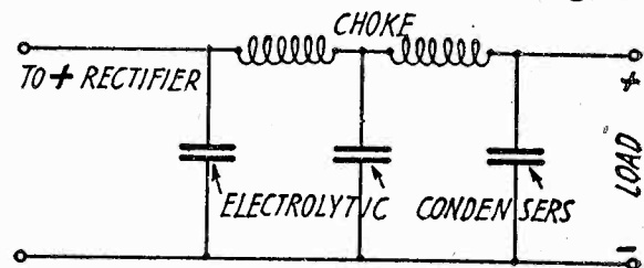
Fig. 3. Arrangement Using Condensers.
