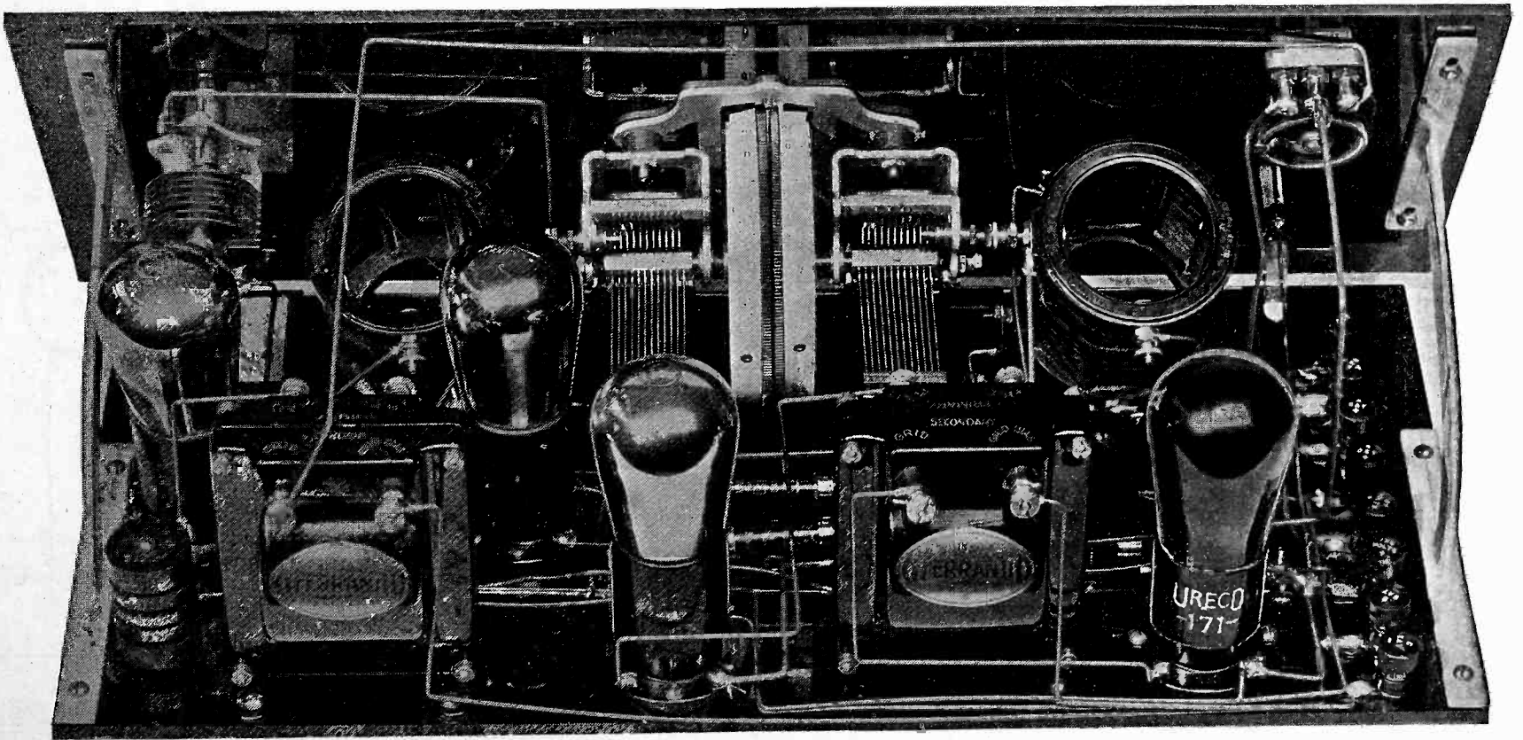
Rear View of Completed Receiver.
