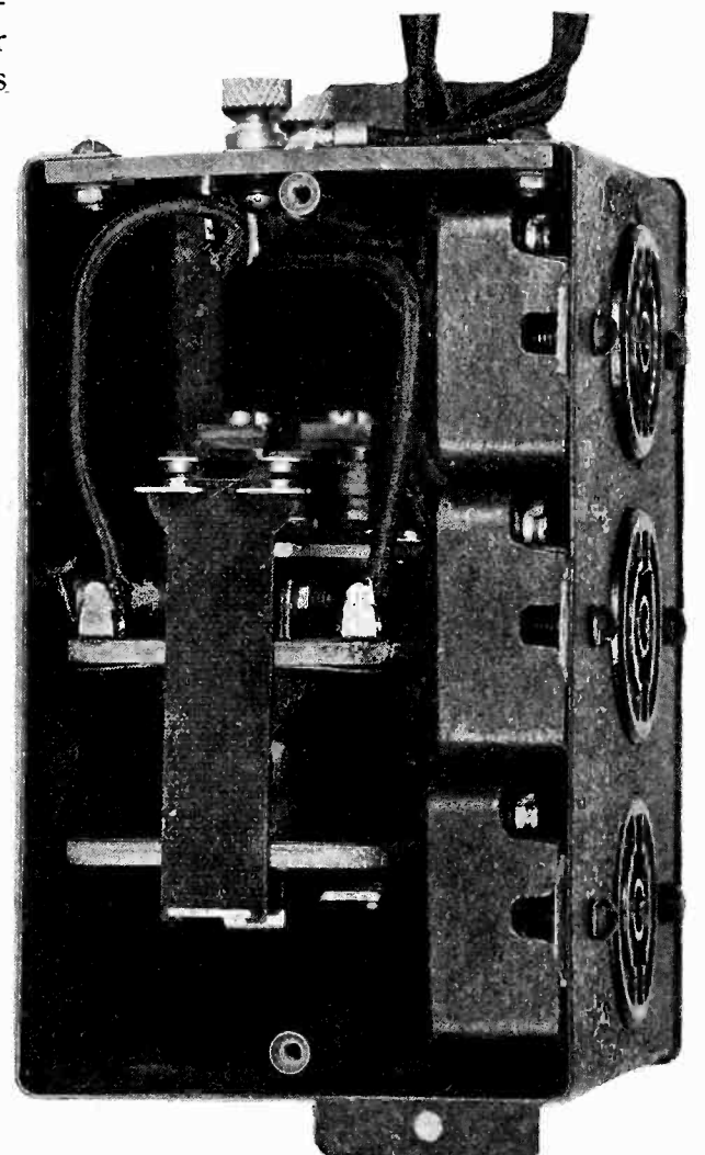
Fig. 3. Shunt Relay, with Three Power Circuit Contacts.
