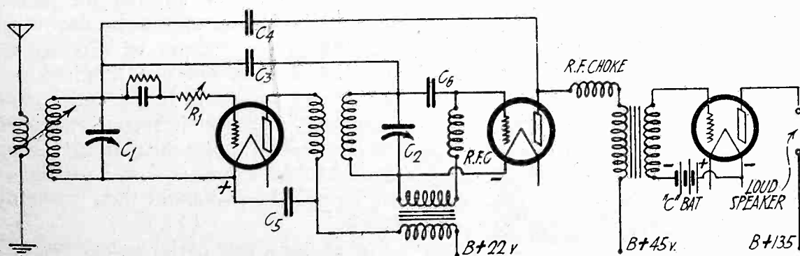
Fig. 1. Circuit Diagram of Stabilized Regenerative Receiver.
