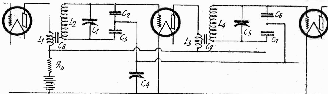
Fig. 7b. Equivalent of Portion of Infradyne Amplifier.
