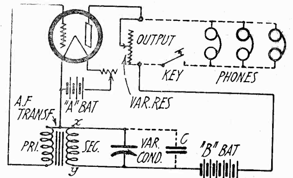
Fig. 1. Circuit Diagram of A. F. Oscillator.
