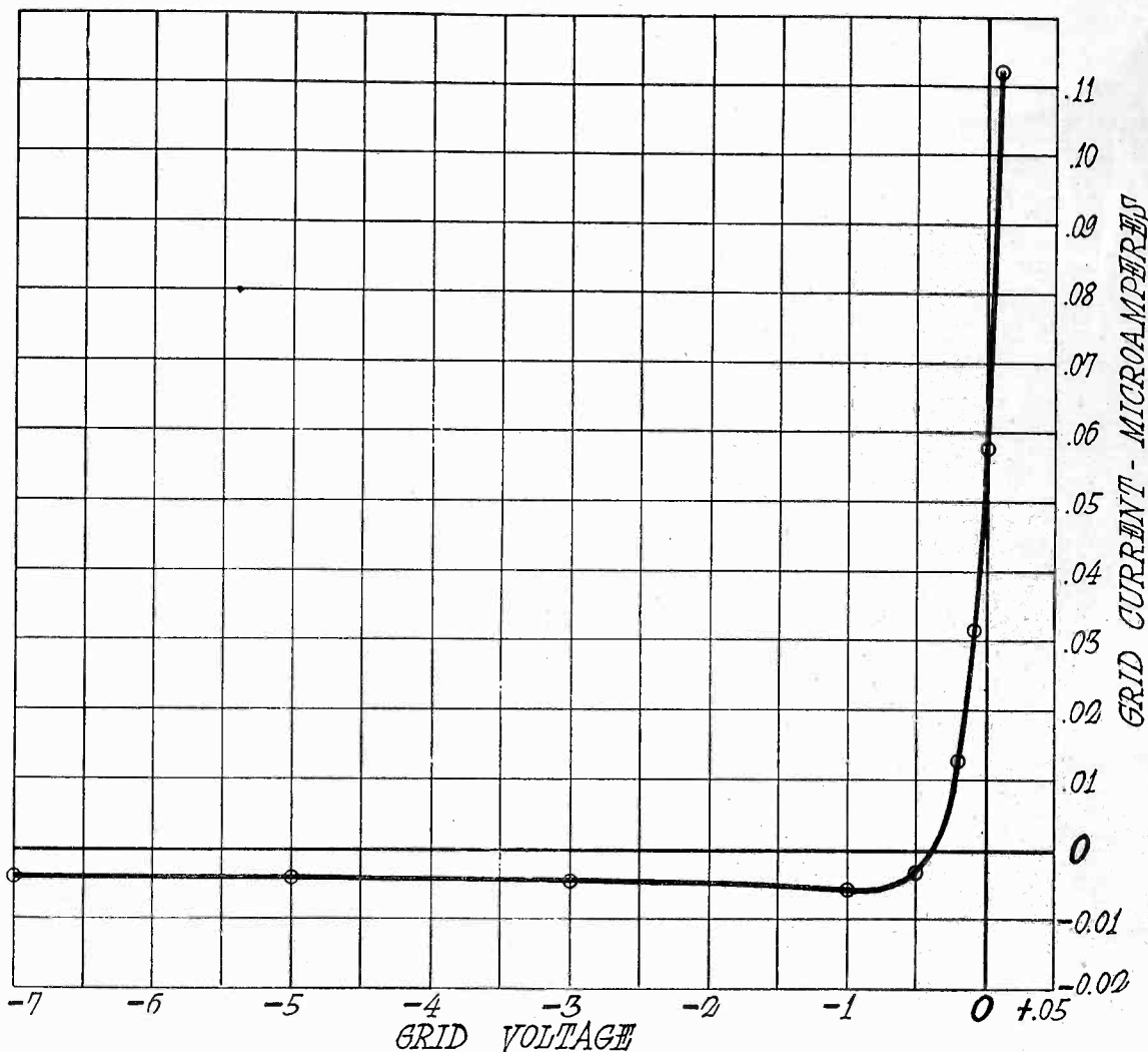
Fig. 5. Variation of Grid Current with Grid Potential.
