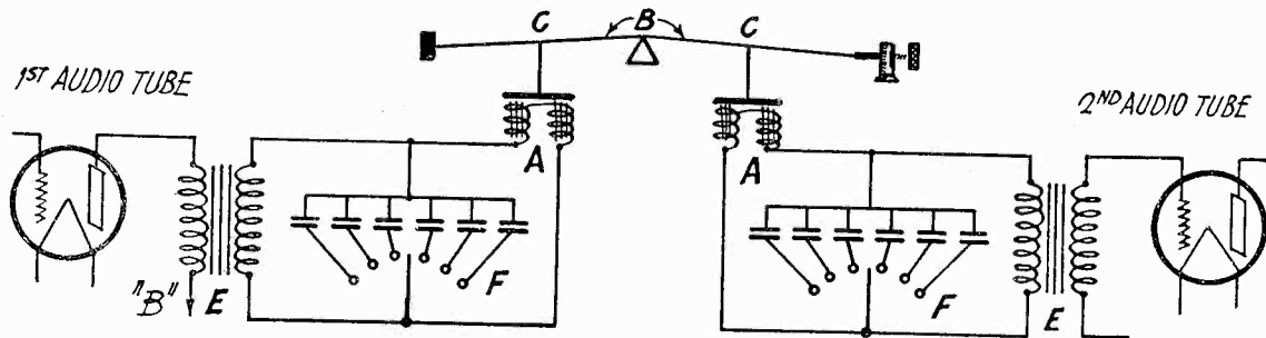
Circuit Diagram of McCaa Band Eliminator.
