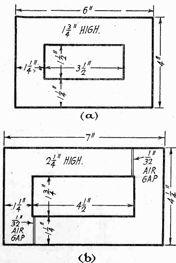
Fig. 1. Core Dimensions: (a) Transformer, (b) Choke.
