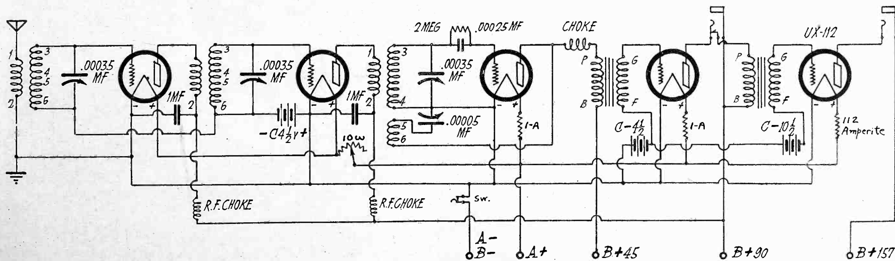
Fig. 1. Five Tube Receiver With Regenerative Detector.
