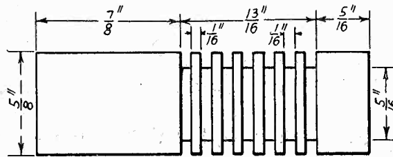
Fig. 2. Choke Coil Form.
