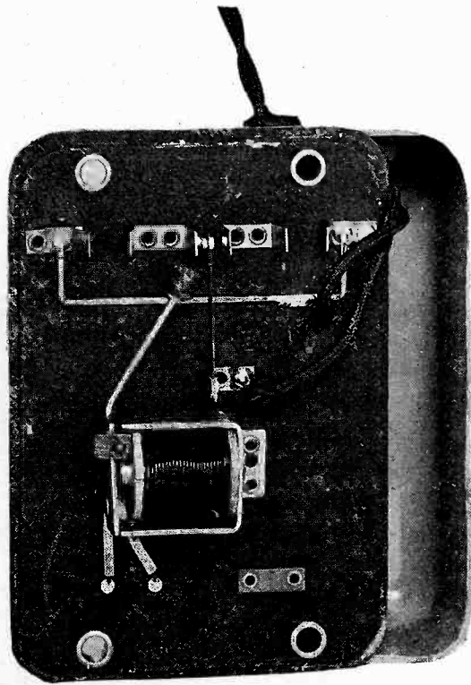
Fig. 1.—Series Type Relay, for Two Power Circuits.
