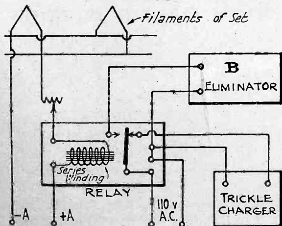
Fig. 2. Circuit of Series Relay.
