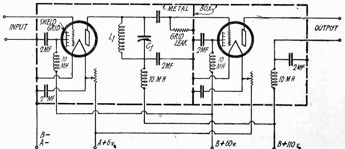
Fig. 2. Circuit Diagram of Two Stage Amplifier Using Shielded Grid Tube.
