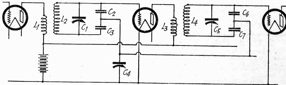
Fig. 7a. Portion of Infradyne Amplifier.
