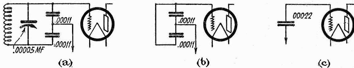
Fig. 6. Input Circuit and Its Equivalents.
