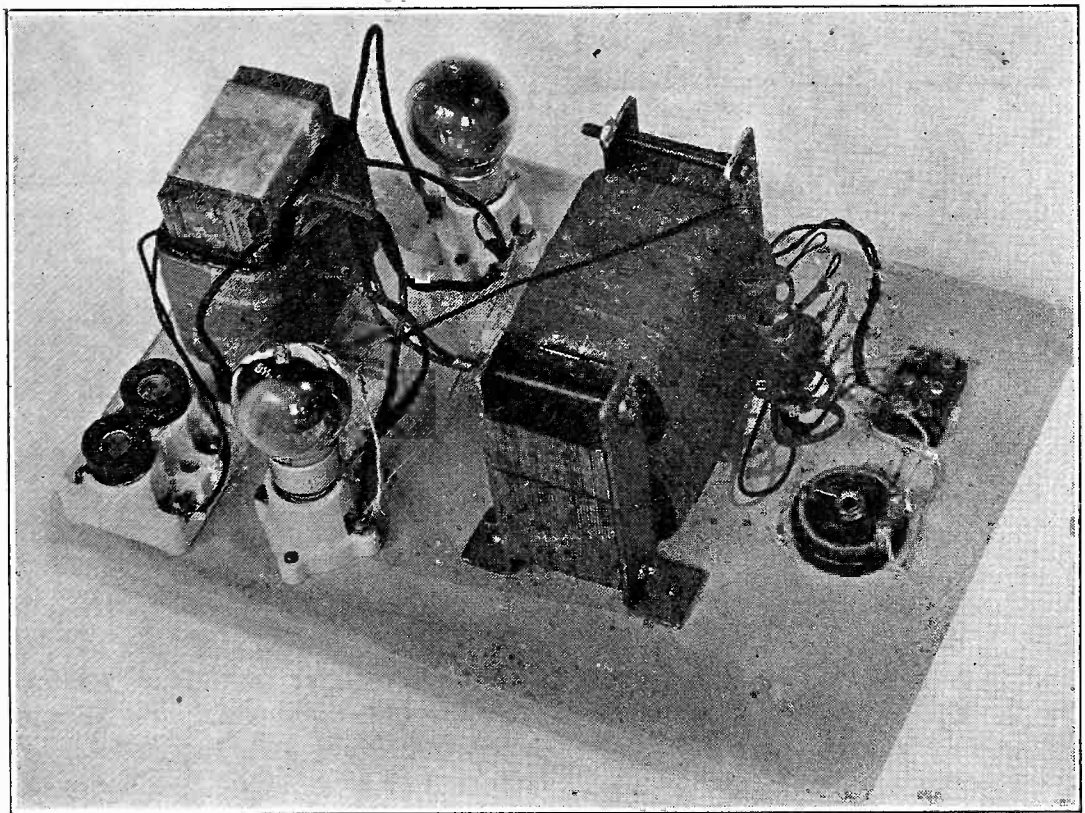
Complete "A" Eliminator.
