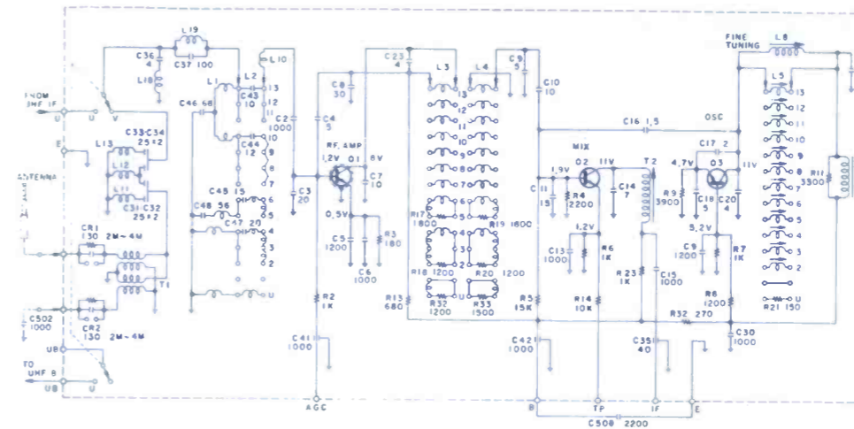
VHF TUNER
