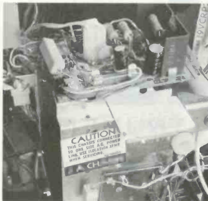
The power supply panel is located on the top of the high-voltage cage.
