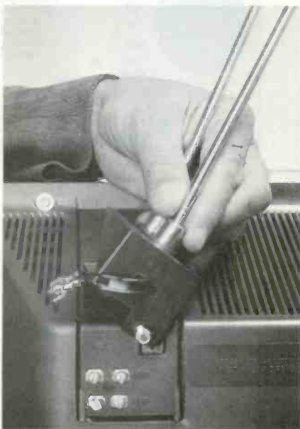
The antenna assembly can be replaced by removing one screw and the antenna terminals, eliminating the need to remove the back cover of the TV set.
