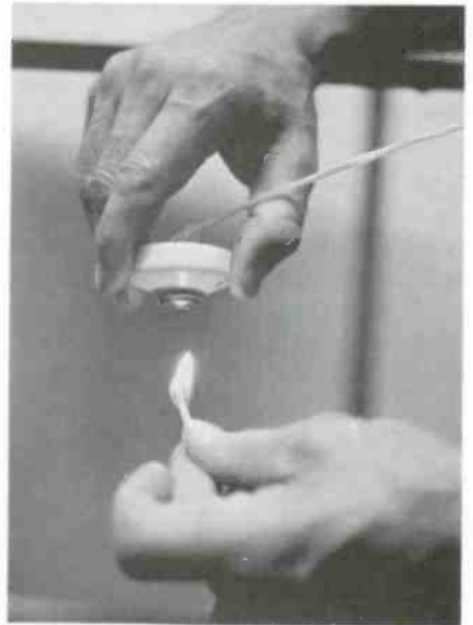
A lighted match was used to test an EICO 135°F heat detector that could be attached to the alarm system to add fire protection.
