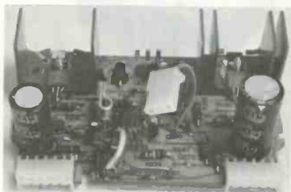
One of the vertical modules which is plugged into the common signal board to compensate for the different screen sizes.
