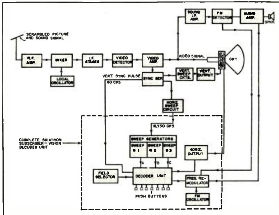
Fig. 5. Block diagram of the S-V decoder installed in a standard television set.
