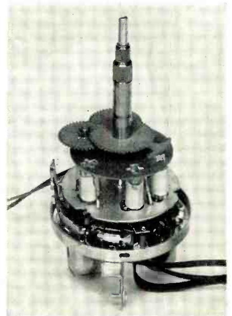
Fig. 11. The G-E "U.H.F. 70" converter shown with the shield can removed. Note that the crystal is held by spring clips.
