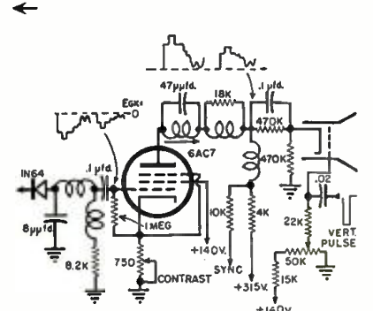
Fig. 6. White clamping type of automatic brightness control circuit used by Stewart Warner in their model 9202-C TV receiver.
