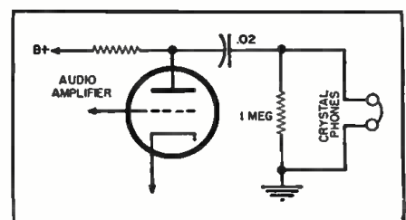
Recommended phone connection circuit.
