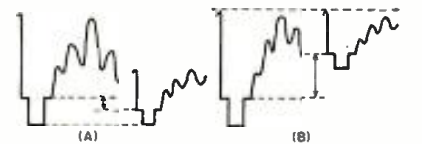
Fig. 7. Effect of a change in signal level on the black level for circuit using (A) sync pulse clamping; (B) white clamping.
