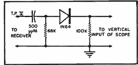
Fig. 8. Detector circuit for step 4. Table 1.
