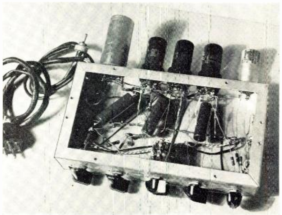
Fig. 4. Modification of the Williamson circuit to obtain 150 ma. d.c. heater current.
