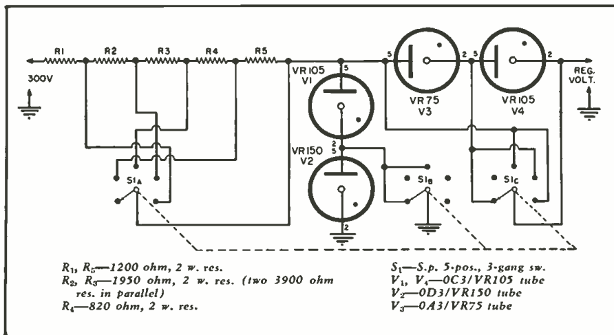
Fig. 2. Schematic of circuit which provides adjustable feature for power supply.
