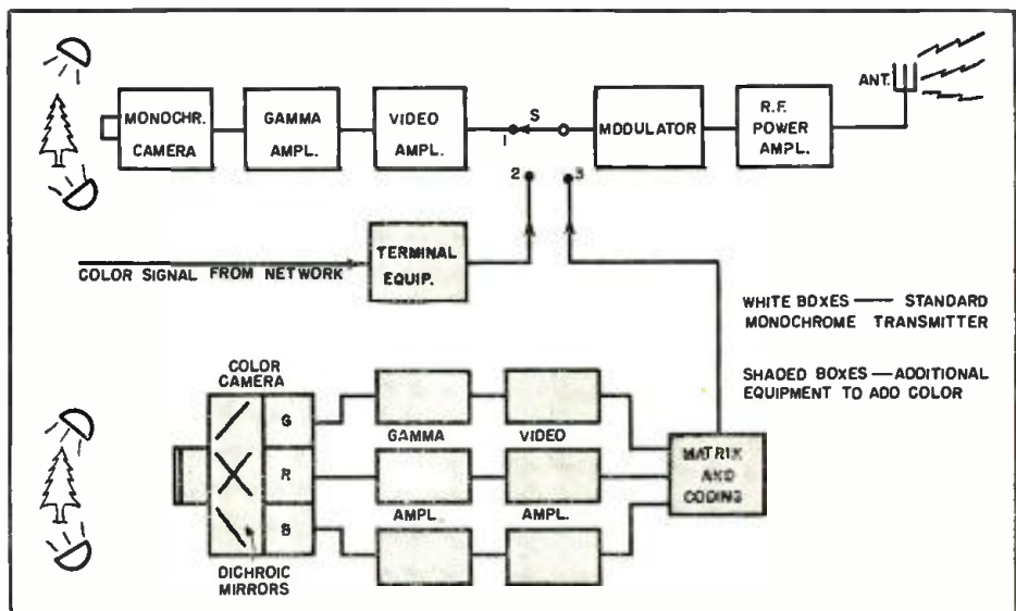
Fig. 3. Simplified block diagram of a typical color television transmitter.
