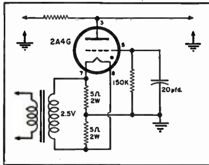
Fig. 3. Alternate circuit using a 2A4G.
