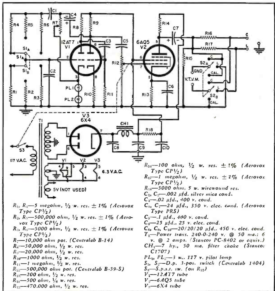
Fig. 3. Complete schematic diagram and parts list for the "Con-VI."
