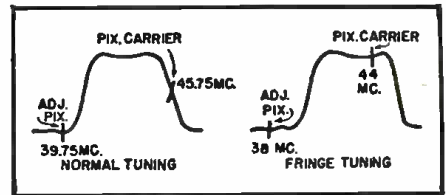
Fig. 7. Response curves for both normal and fringe areas to provide best tuning.
