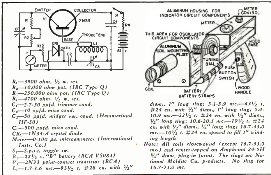
Fig. 1. Complete schematic of the "Transdipper" and an experimental "breadboard" layout which still affords operating convenience. The metering circuit measures changes of r.f. voltage, which is more effective than measuring d.c. current dips.
