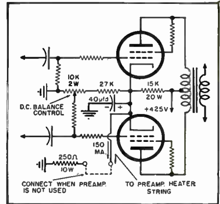
Fig. 4. Modification of the Williamson circuit to obtain 150 ma. d.c. heater current.
