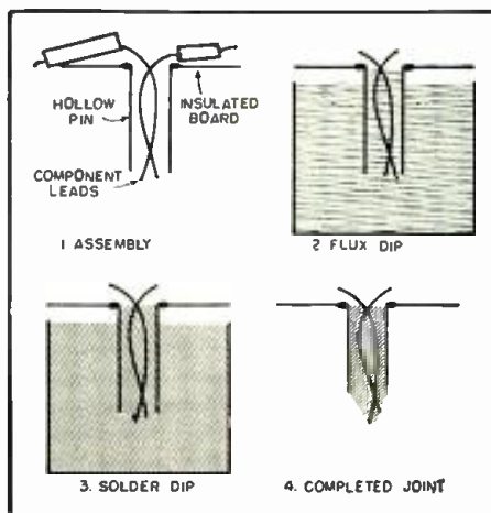
Fig. 2. The four basic dip-solder steps.
