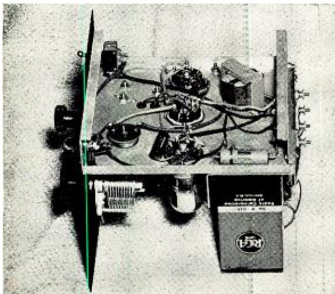
Bottom view of chassis, showing neat and roomy layout of parts. The round object at left is the 7.5 mhy. plate-circuit choke.
