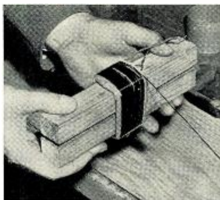
Fig. 1. Winding the new secondary. The block of wood prevents damage to wire.
