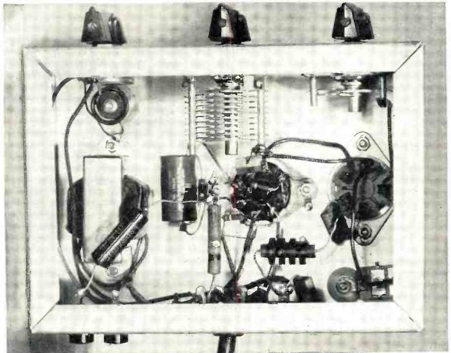
Under-chassis view of the Novice station receiver. The audio transformer is seen at left, below the regeneration control. Phone tip jacks and power cable can be seen along rear edge of chassis. Coil socket is at extreme right. Note roomy layout.
