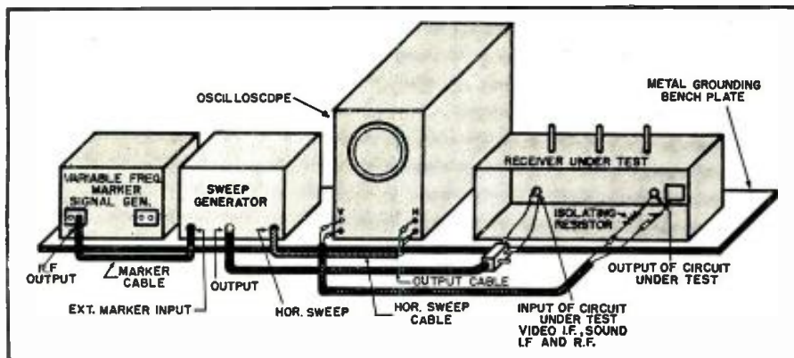
Fig. 5. Service bench setup showing how sweep generator is connected to receiver.
