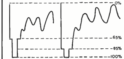
Fig. 3. Effect on black level of a change in blanking pulse amplitude percentage.
