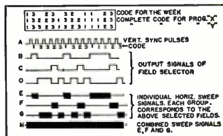
Fig. 4. Signals at field selector and coding and switching circuit of Figs. 2 and 5. See text for details on these patterns.
