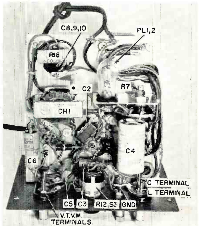
Fig. 5. Under chassis view of unit with major parts identified.
