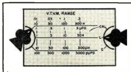
Fig. 6. Detail of the scale used on "Con-VI."
