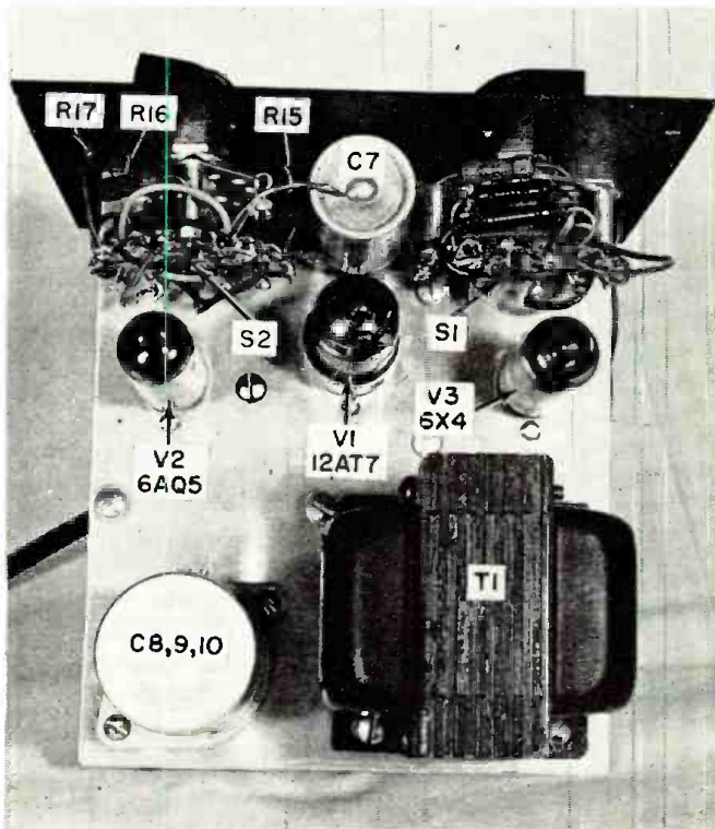
Fig. 4. Top chassis view of the "Con-VI" showing parts layout.
