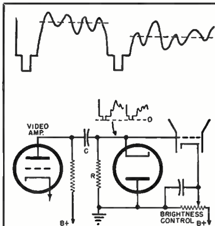
Fig. 2. Diode sync pulse clamping circuit.
