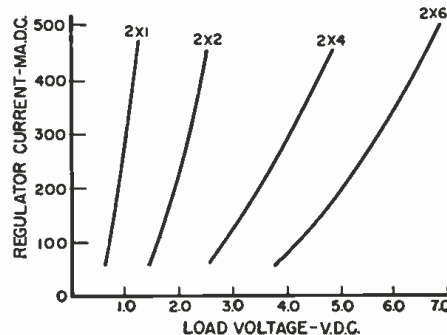
Fig. 2. Regulation characteristics for various regulators. See text for discussion.
