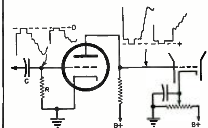
Fig. 5. Grid leak bias sync pulse clamping automatic brightness control circuit.
