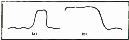
Fig. 3. When the sweep is too wide, the pattern will tend to crowd together (A). When too little sweep is used, the full pattern may not be obtained as shown in curve (B).
