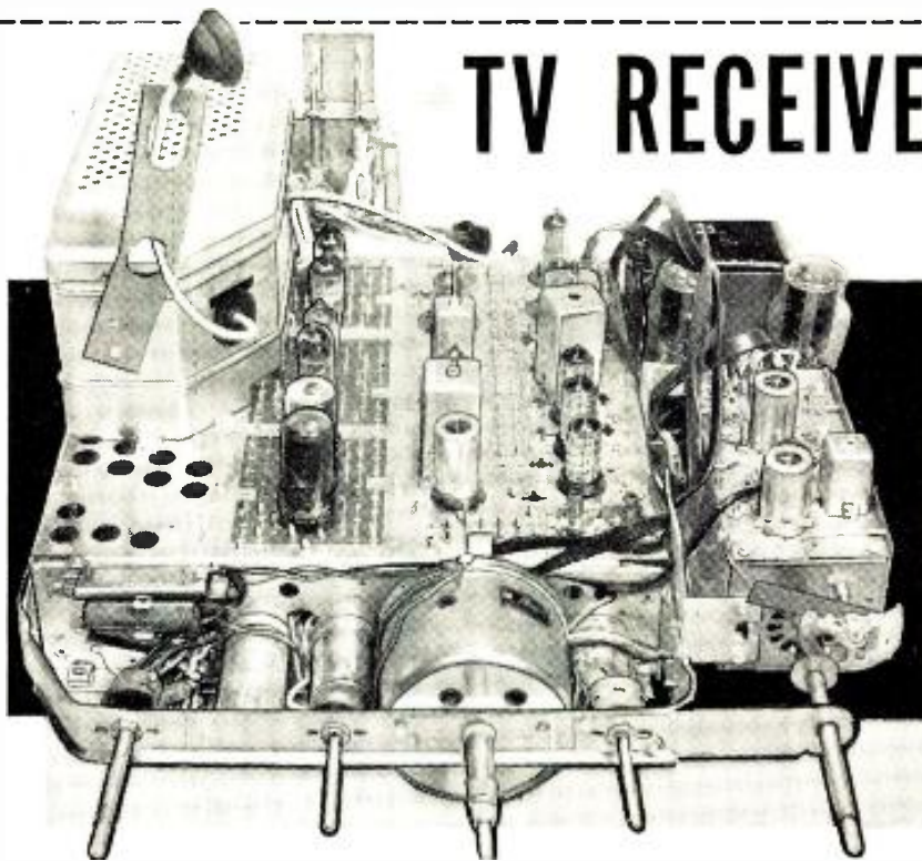
Fig. 1. The G-E dip-soldered "EE" chassis, used in its new TV line.
