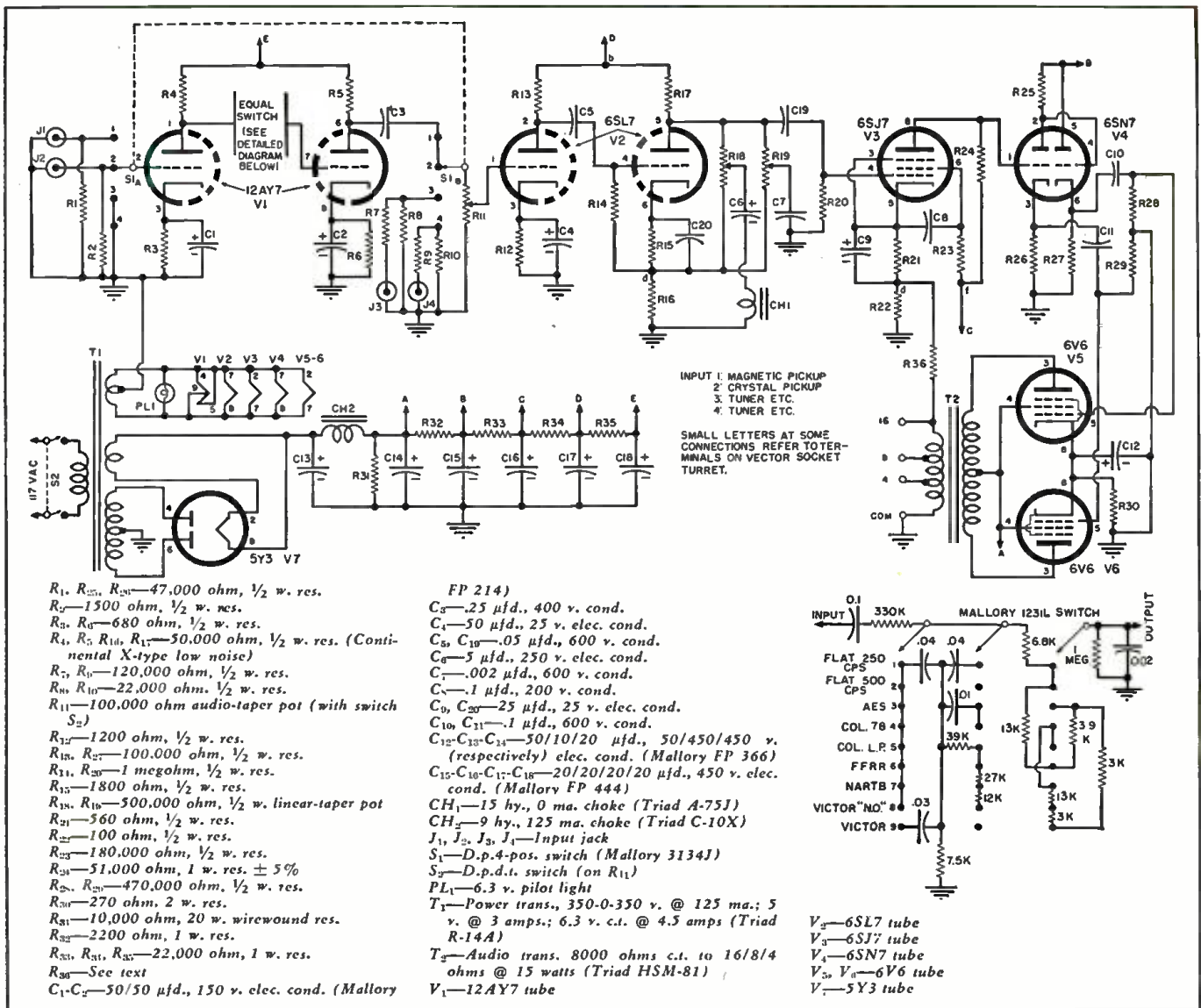
Fig. 4. Complete schematic of improved Kappler amplifier. Equalizer circuit is shown in the inset diagram above.
