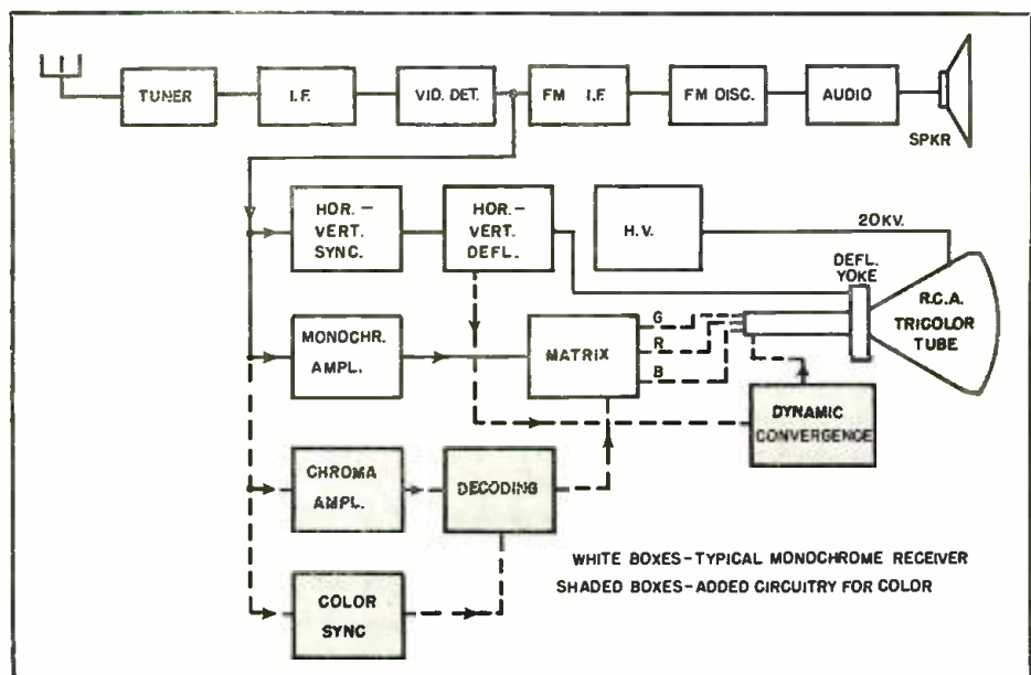
Fig. 4. Simplified block diagram of a typical color television receiver.
