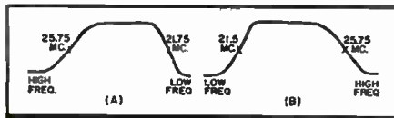
Fig. 8. A sweep phase reversal switch can reverse pattern obtained on screen. See text.
