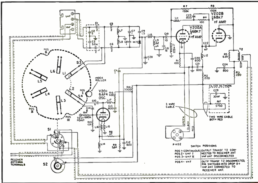
Fig. 5. Schematic of the G-E "U.H.F. 70" converter used with the "EE" chassis.
