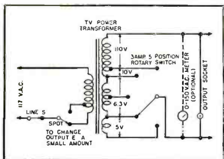
Fig. 4. Circuit diagram of junk-box supply.
