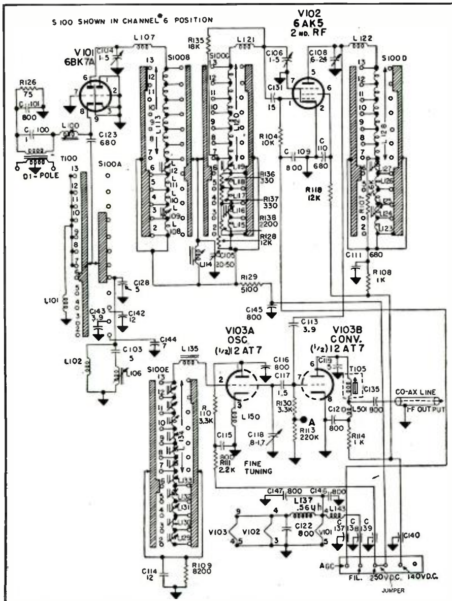
Fig. 6. Schematic diagram of the v.h.f. tuner of the General Electric "EE" chassis.
