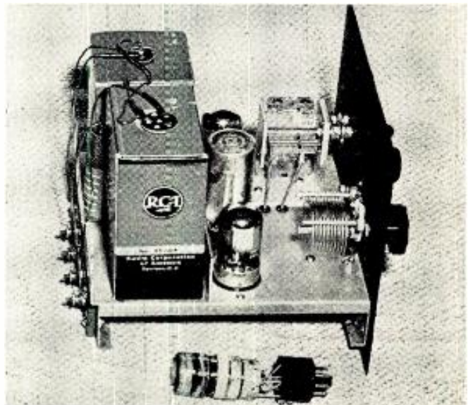
Top view. Short-wave coil is in place, covered by a Millen shield which is part of coil form. Broadcast coil is in front.
