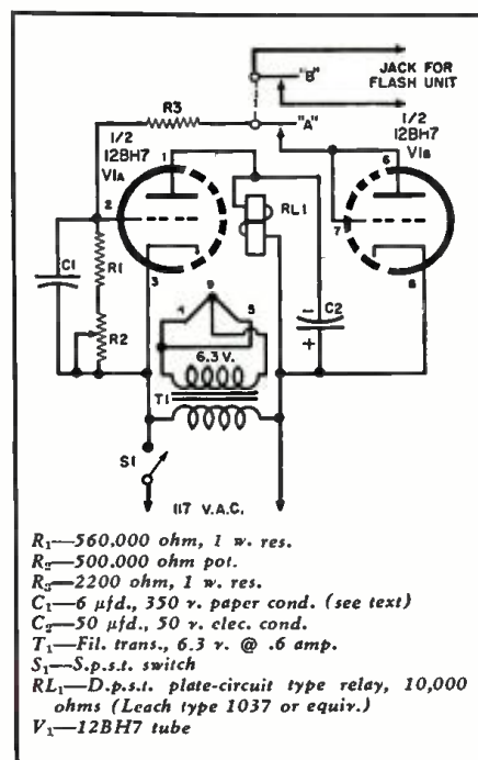
Complete schematic of compact tester unit.
