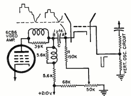
Fig. 8. Automatic brightness control circuit of the Magnavox 104 series sets.
