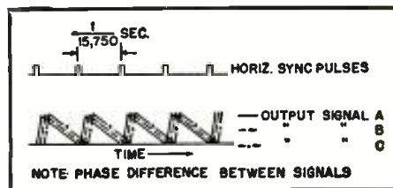
Fig. 3. Output signals of sweep generators #1, #2, #3 of S-V transmission system.
