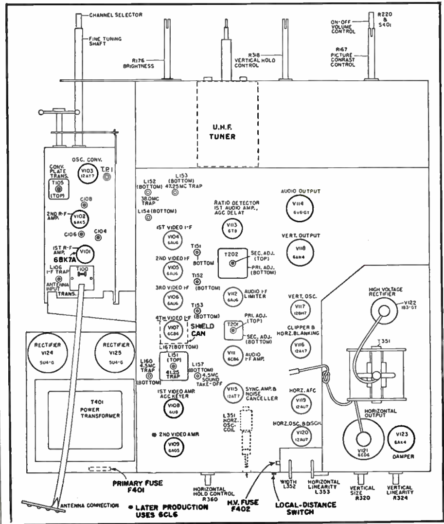
Fig. 10. Top view of the G-E "EE" chassis showing the tube and parts layout.
