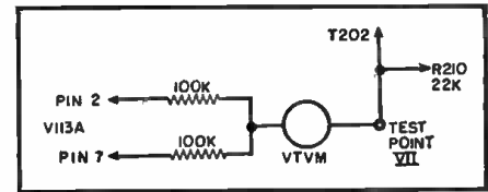
Fig. 9. Resistor network used in step 9. Table 1. The resistors are equal within 5%.
