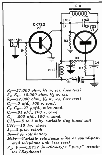
"Wireless mike" using CK722 transistors.
