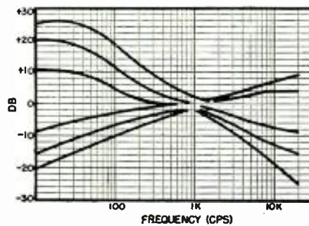
Fig. 3. Over-all preamp response curves.
