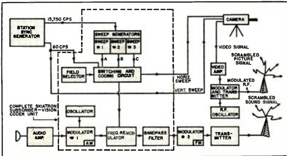
Fig. 2. Block diagram of transmitter adapted to handle S-V coded transmissions.
