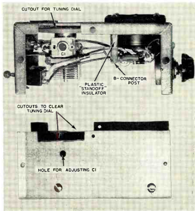
Fig. 4. Side views of the box sections, showing cuts necessary to clear the tuning dial. As the rotor of C_1 is grounded, C_1 may be mounted directly on the side of the box with the dial outside, eliminating cutting. C_1 , the emitter condenser, is visible in this view. Its adjusting hole is on other cover.
