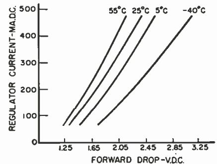
Fig. 3. Variation of regulation characteristics with temperature. Refer to text.
