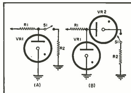
Fig. 1. (A) Basic voltage regulator circuit. (B) Another version of a voltage regulator.
