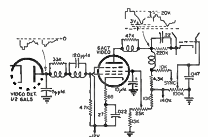
Fig. 9. Arvin's white clamping circuit.
