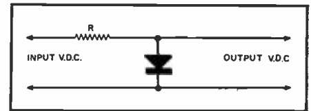
Fig. 1. A basic d.c. regulator circuit.
