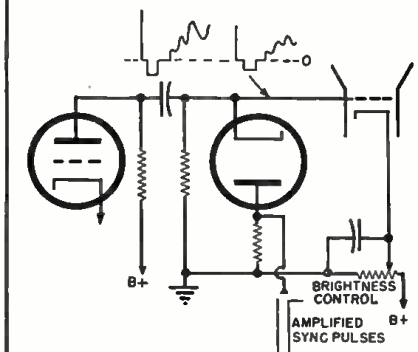
Fig. 4. Diode blanking pulse clamping.
