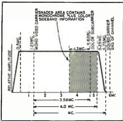
Fig. 2. Color signal characteristics.
