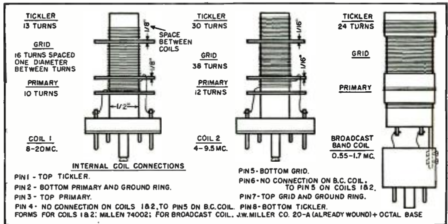
Coil diagram of the student receiver. The Millen forms have octal bases. Looking at the bottom of a form, with the octal key pointing down, pin 1 is to the lower left of key; other pins are counted clockwise from pin 1. The broadcast coil is ready-made (J. W. Miller Co. No. 20-A) and is attached to an old octal tube base.
