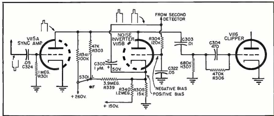
Fig. 4. Partial schematic diagram of the noise inverter circuit used in the G-E "EE" chassis. As shown here, sync pulses are fed to the inverter from two sources.
