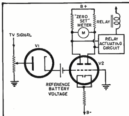
Fig. 2. Simplified basic circuit of one test channel of the intermittent recorder.
