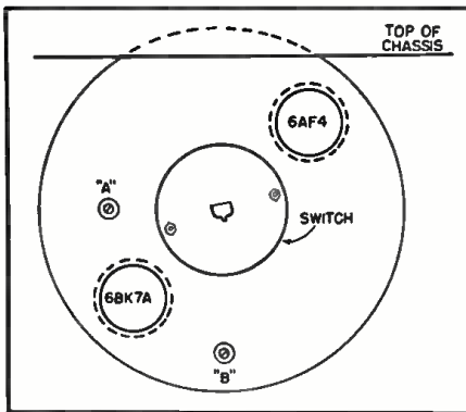
Fig. 12. Rear view of "U.H.F. 70" tuner showing location of i.f. adjustments.
