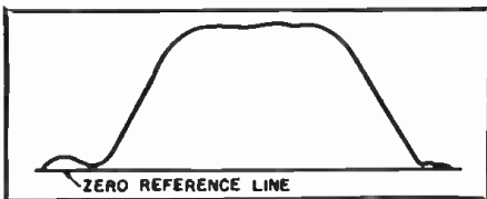
Fig. 7. A blanking circuit in a sweep generator produces a zero reference line on the screen of the service oscilloscope.
