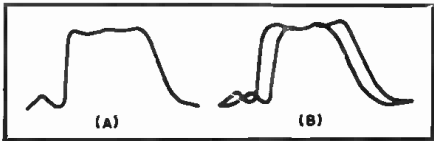
Fig. 4. (A) Desired single pattern response curve. (B) Double trace pattern obtained before phase control adjustment.
