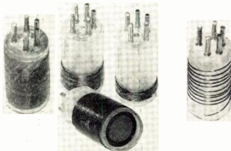
Fig. 2. The plug-in coils for the "Transdipper." Left to right, coils for 1.7-3.6 mc., 5.4-10.9 mc., 3.1-5.9 mc., 10.6-20.5 mc., 16.7-33.0 mc. The four lowest-frequency coils have slugs to adjust the "Q" of the coils to obtain reliable "dipping" action.
