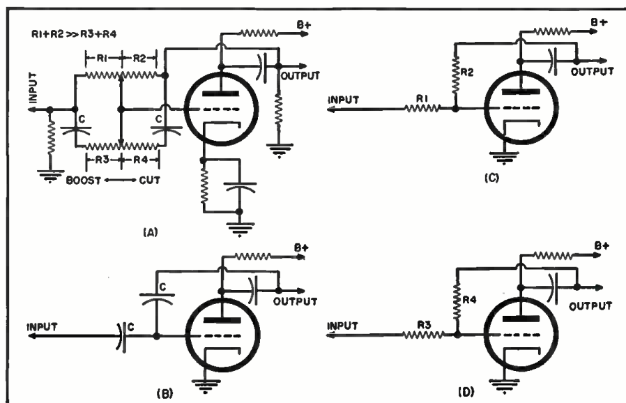
Fig. 1. Tone control-record compensation circuits. (A) Continuous tone control. (B) Mid-frequency equivalent. (C) Low-frequency and (D) high-frequency equivalent circuits.
