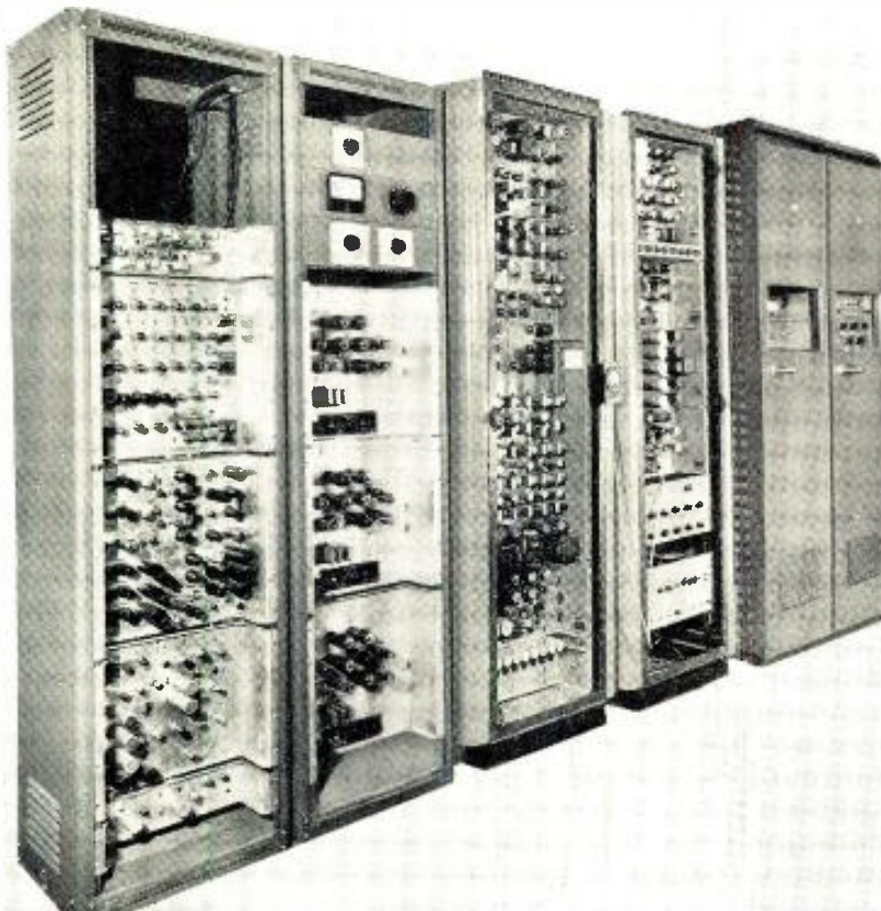
Color TV signal generating equipment used by Emerson for the design and testing of color TV receivers. Included is a monoscope and flying-spot scanner.
