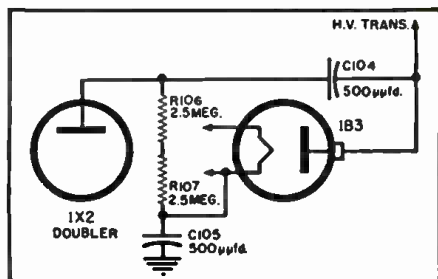
Portion of the Philco D-1 chassis circuit showing source of possible service fault.
