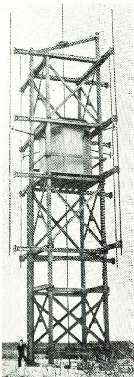
Fig. 1. High-frequency direction finder antenna system consisting of vertical doublets.
