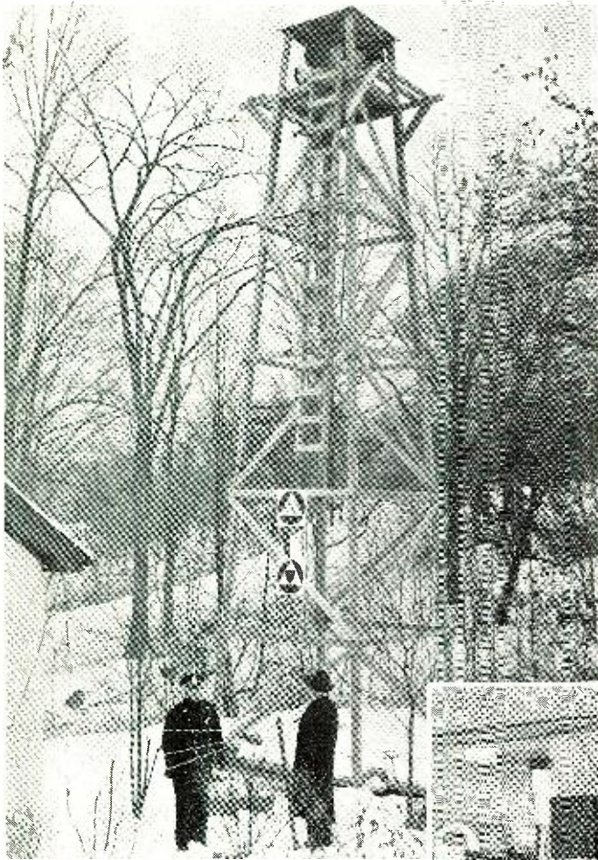
A 34' air raid tower showing the speakers mounted on a platform.
