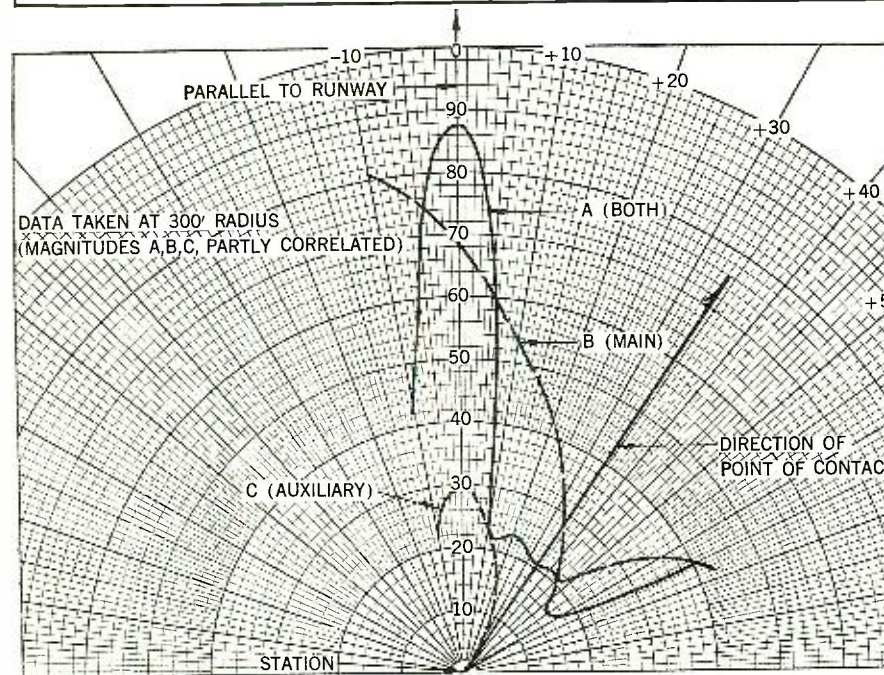
Fig. 14. Left: Field Pattern of Glide Path Antenna System installation.
