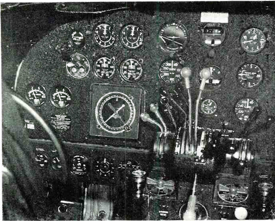
Nerve center of the modern airliner is the radio compass.
