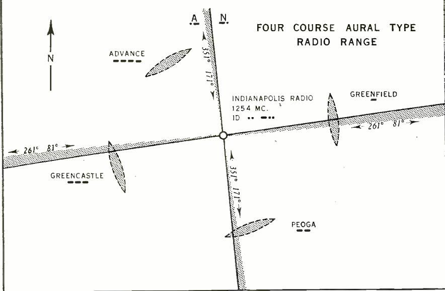
Fig. 12. Above: UHF Two-course units. Fig. 13. Left: Orientation of 4-course.
