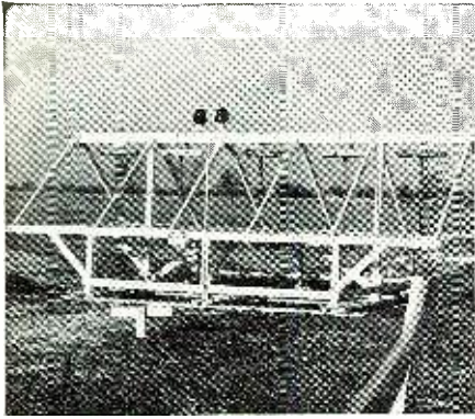
Fig. 1. Experimental 5-loop system.
