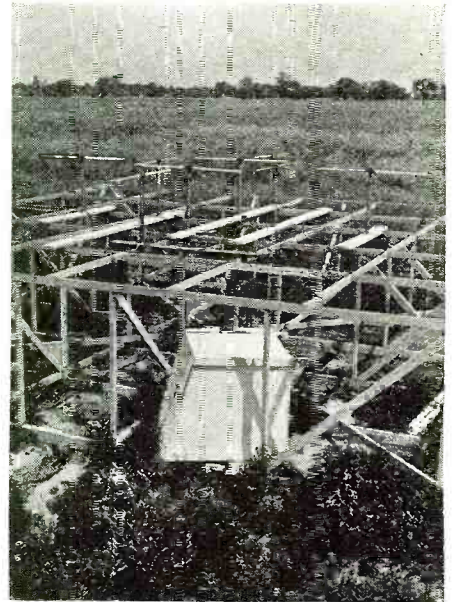
Fig. 8. An 8-element Z marker system.
