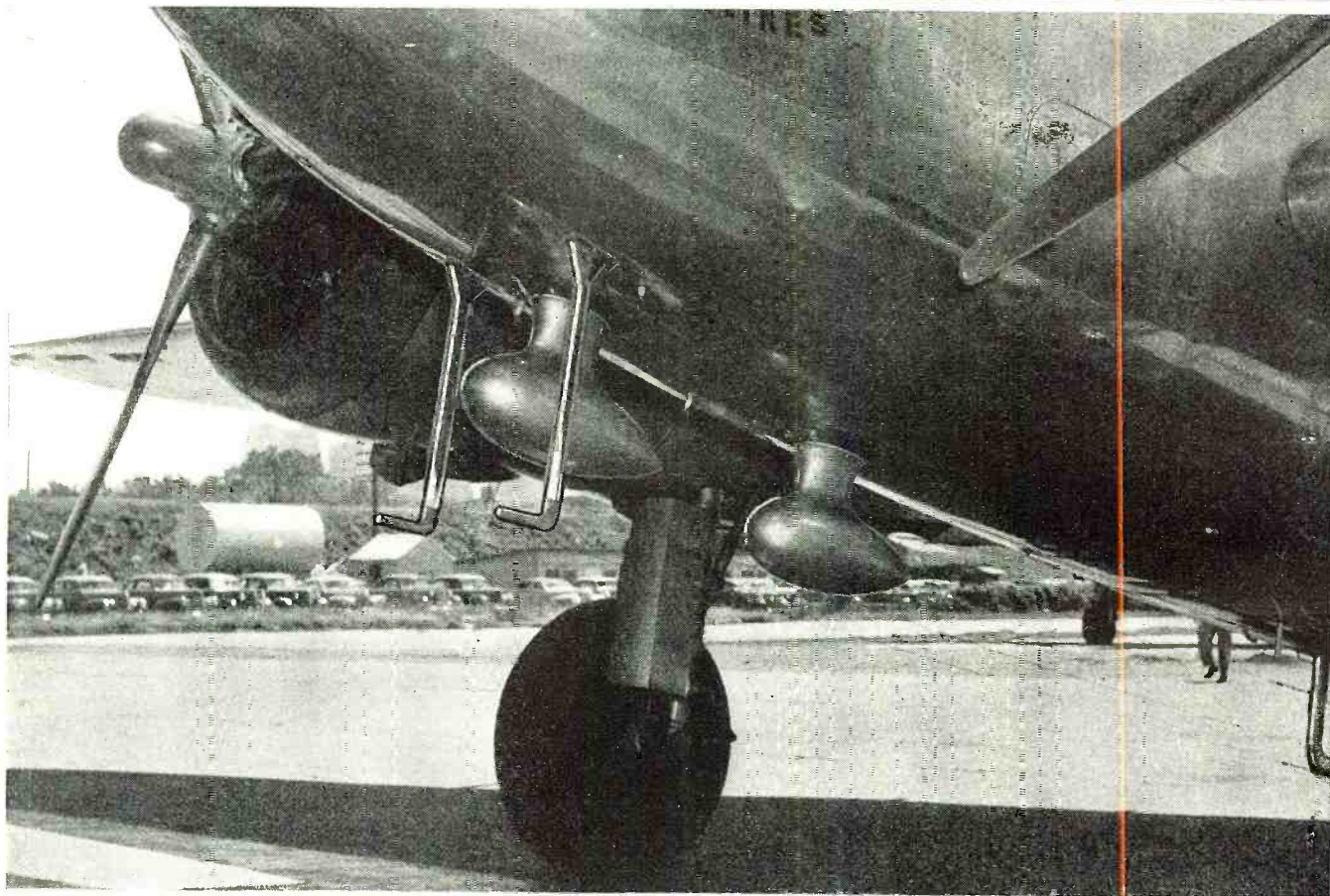
Dual loops installed on Mid-Continent Lockheed Lodestar plane.
