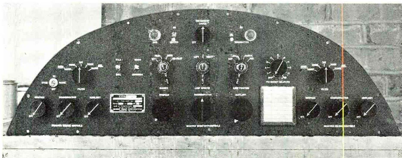
Radio remote-control panel installed in a Lockheed Lodestar airplane. Note the special knobs which are designed for easy handling when wearing gloves.
