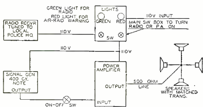
Block diagram of complete system.
