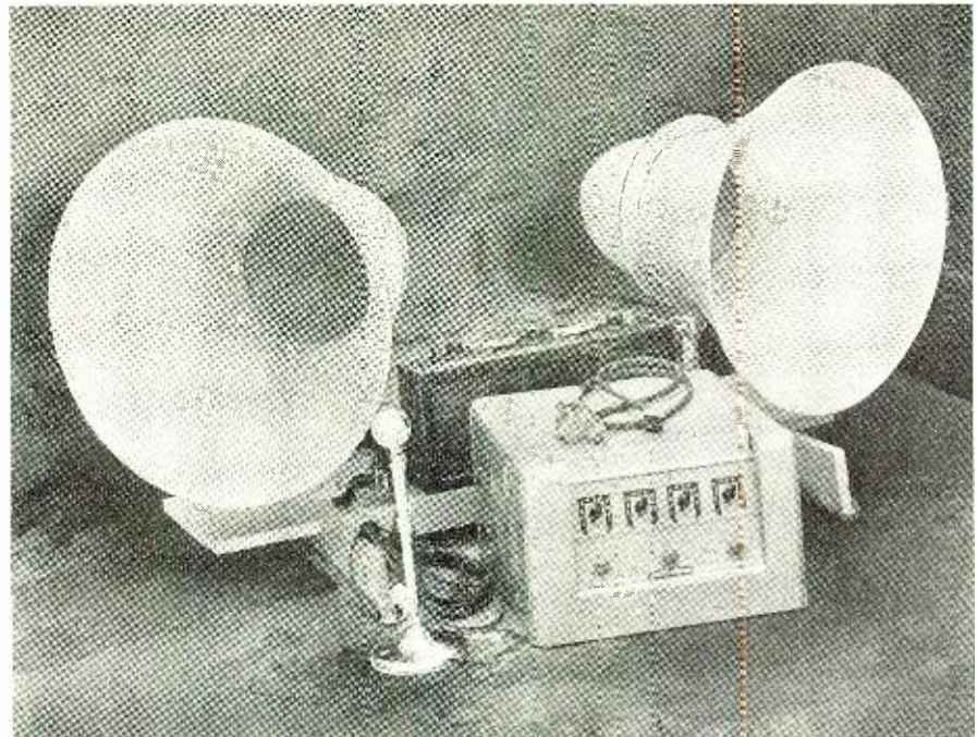
Traffic control car equipment includes 30 watt amplifier, mike and speakers.
