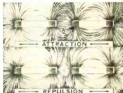
Figure 6. At A is shown attraction between two magnets placed so that opposite poles react on each other. B shows the repulsion effect between two similar poles
