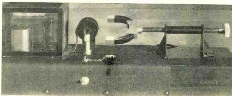
Figure 7. This is a replica of the original Barkhausen apparatus for demonstrating the theory of magnetism. By rotating the magnet, sounds of tiny molecular particles can be heard changing polarity
