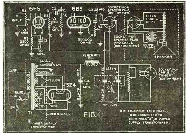
FIG. 1. THE COMPLETE SCHEMATIC DIAGRAM The lower portion shows the power supply. The amplifier and loudspeaker are shown above
