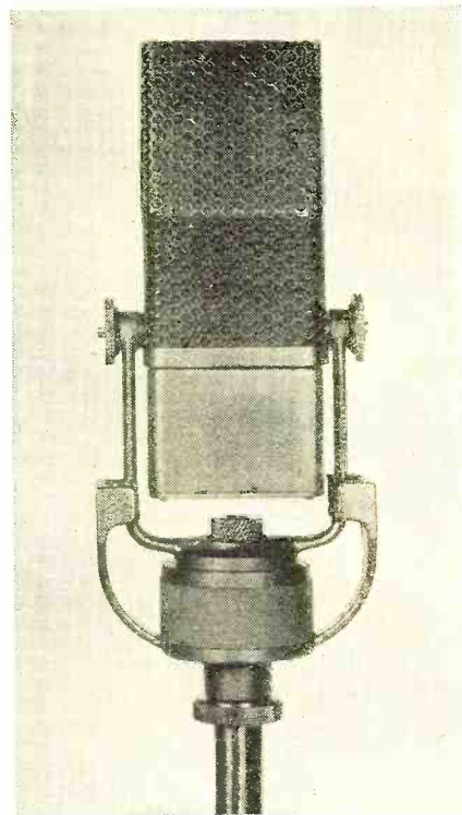
Figure 4. The velocity microphone built upon the principle of interaction between electric currents flowing in a ribbon and a magnetic field
