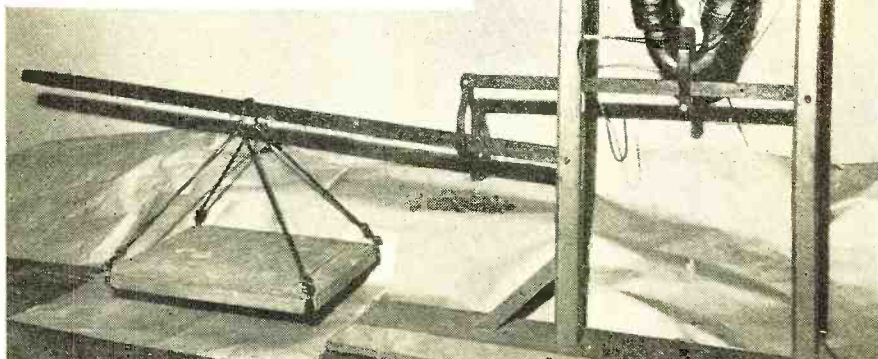
Figure 8. A replica of the great Henry's largest magnet, which was made by winding silk-wrapped wire on an iron frame. It operated by passing heavy currents of low voltage through the winding and could lift a large weight
