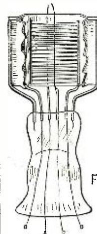
The skeleton view of the elements of a vacuum tube shown here with will give the reader a clearer idea of the relation between the various parts.
