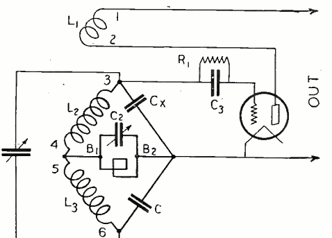
Fig. 2. The autodyne frequency changer, part of the circuit which oscillates at one frequency and detects at another.
