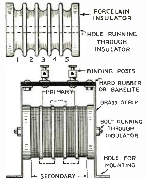
A porcelain insulator makes an excellent form on which to build a transformer, the grooves making natural slots for the wire.
