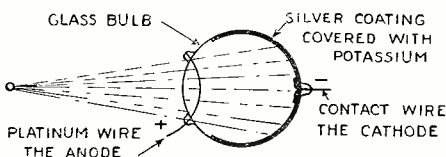
ORIGINAL ELSTER AND GEITEL PHOTO ELECTRIC CELL
