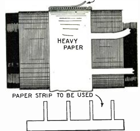
One of the best methods yet devised for fastening a primary coil that is wound over a secondary.
