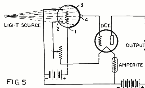
Circuit of the apparatus shown in the photograph at the left.
