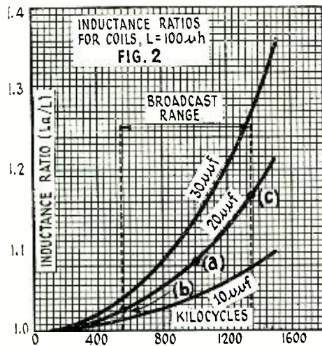
FIG. 2 How the apparent inductance of a coil depends on the coil capacity is shown in this chart.
