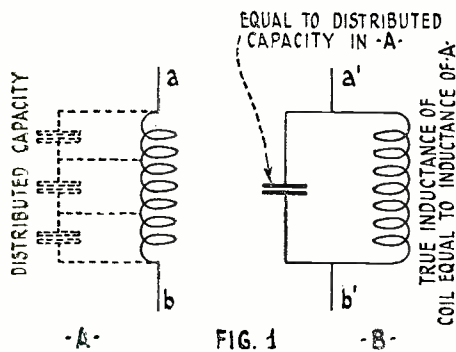
FIG. 1 A coil having capacity as shown in (A) is equivalent to the circuit in (B), the inductance of (B) equal to the true inductance in (A) and the capacity in (B) equal to the coil capacity in (A).
