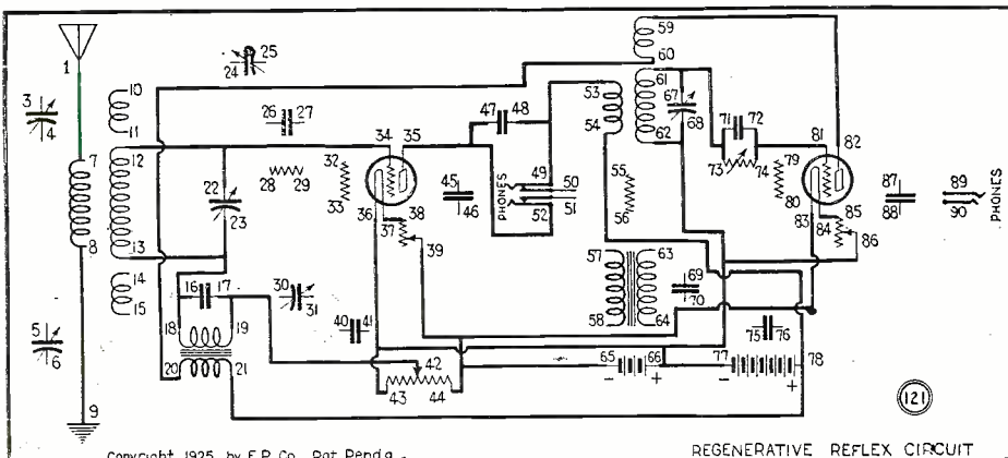
REGENERATIVE REFLEX CIRCUIT (121)
