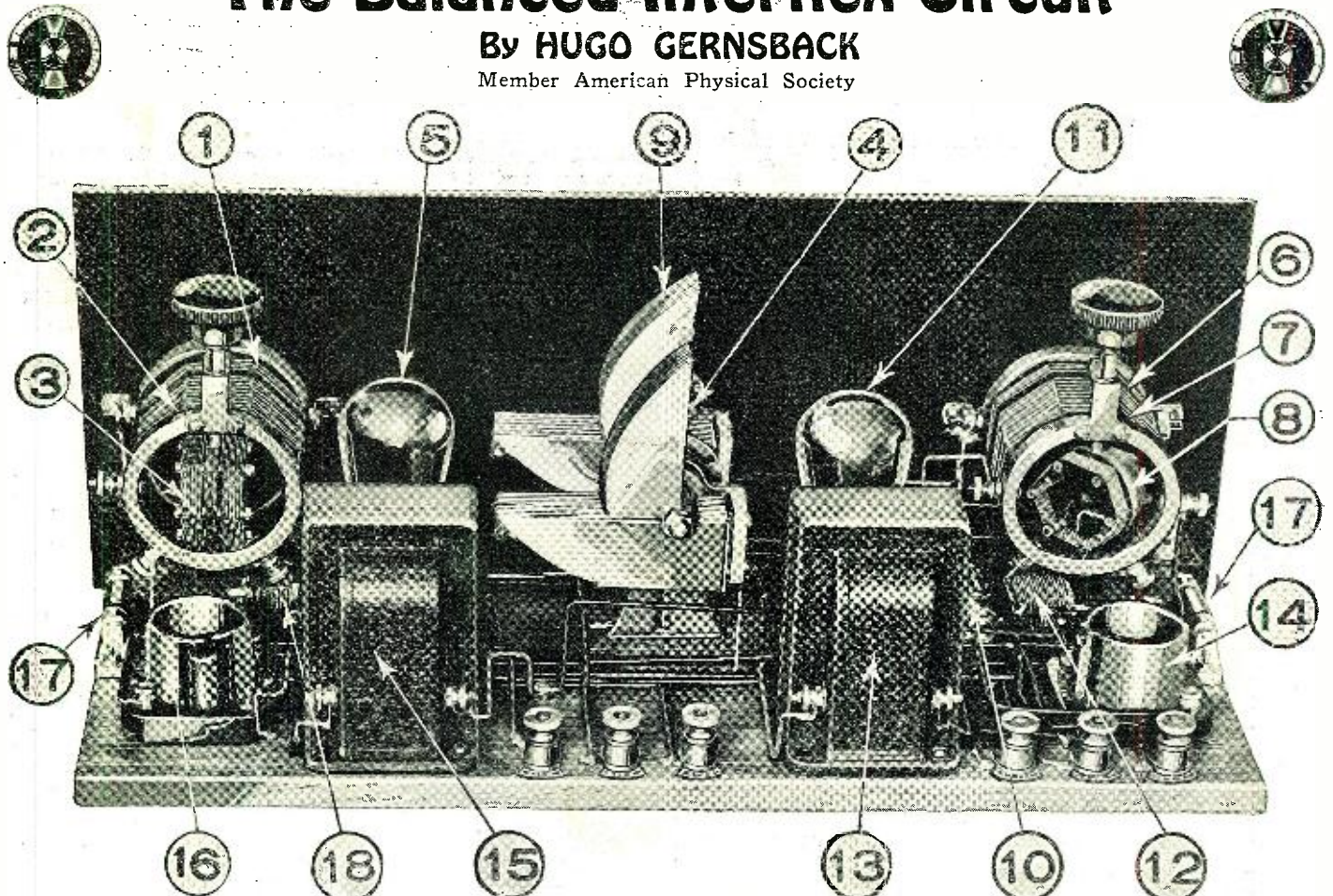
Rear view of the Balanced Interflex. (1) and (6), aperiodic primary; (2) and (7), secondaries of main inductances; (3) and (8), adjustable losses; (5), (11), (14), and (16), tubes and sockets; (17) automatic resistances; (12) and (18), automatic filament control jacks; (10) crystal detector; (13) and (15), audio frequency transformers; (4) and (9), straight-line frequency condensers, linked.
