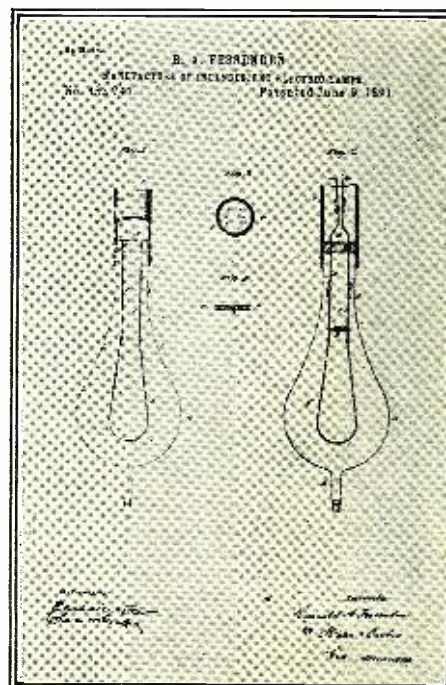
One of Fessenden's important inventions is the use of silicon iron wire for leading-in conductors in incandescent bulbs. The illustration is a reproduction of the drawing for this patent.
