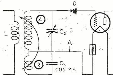
Fig. 1. Theoretical circuit of the Balanced Interflex. L 4 and 2 constitute variocoupler. 2 and C-3 represents the adjustable lossor grounded to the filament. Crystal detector D is in the grid circuit, making the first tube a detector-coupled amplifier. Tuning is accomplished by condenser C-2.
