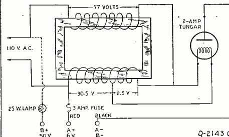
Charging "B" batteries by means of an "A" battery-charger of the regular 2-ampere or 5-ampere type.
