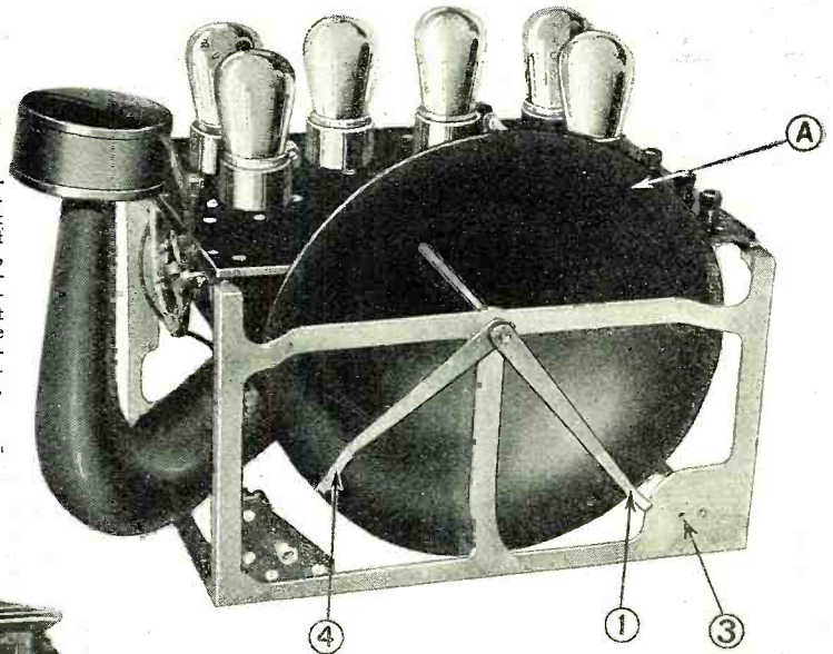
Front view of the receiver. The loud speaker unit on the left leads to the bell of horn, A. The levers, 1 and 4 are shown connected to the shaft carrying the gears that operate the variable condensers. The position of the volume control is indicated at 3.
