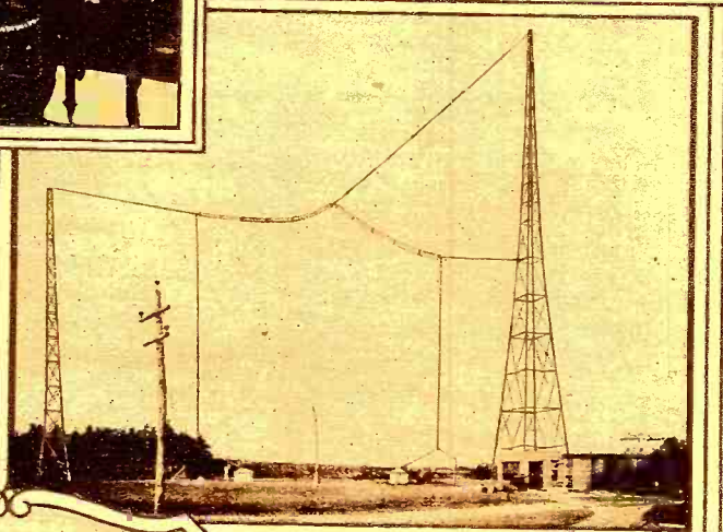
THE SUPERPOWER ANTENNA SYSTEM. Several miles from the studio is erected this antenna system, under which may be seen the buildings that house the transmitting equipment.
