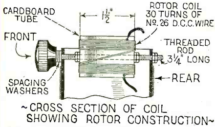
Fig. 4. Constructional details of the adjustable losser described in the article which can be readily made by any constructor.
