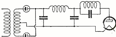
Fig. 17. To the circuit of Fig. 16 a parallel resonant circuit has been added in order to suppress any ripple that might get through to it.
