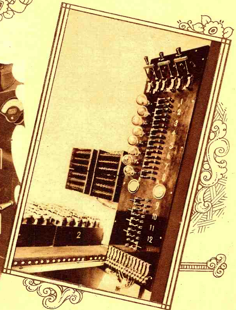
BATTERY-CHARGING PANEL. This panel, which was built by the station's staff of engineers, controls the charging of any or all of the storage batteries used in transmitting.
