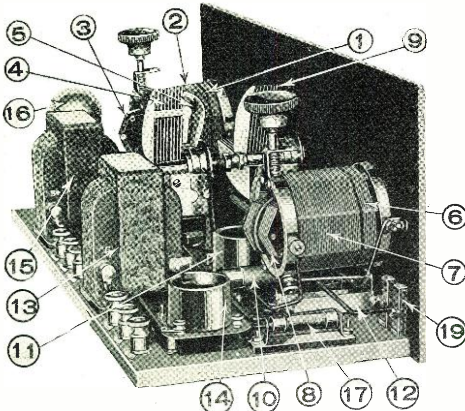
This is a side view of the Balanced Interflex Circuit, giving a good idea of the mounting of the variocouplers and the adjustable lossors. The figures used are the same for all illustrations. (19) here is the condenser C-3 shown above in Fig. 1.
