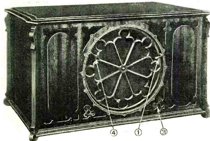
Front view of the six-tube receiver that has but two tuning controls, indicated at 1 and 4. These levers move along the periphery of the grill work, on which is engraved a scale to be used for logging. The number 3 indicates the volume control. Photos on this page Courtesy of Phenix Radio Corp.
