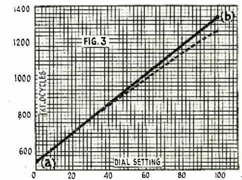
FIG. 3 The calibration curve of an S. L. F. condenser is bent slightly by the circuit capacity.
