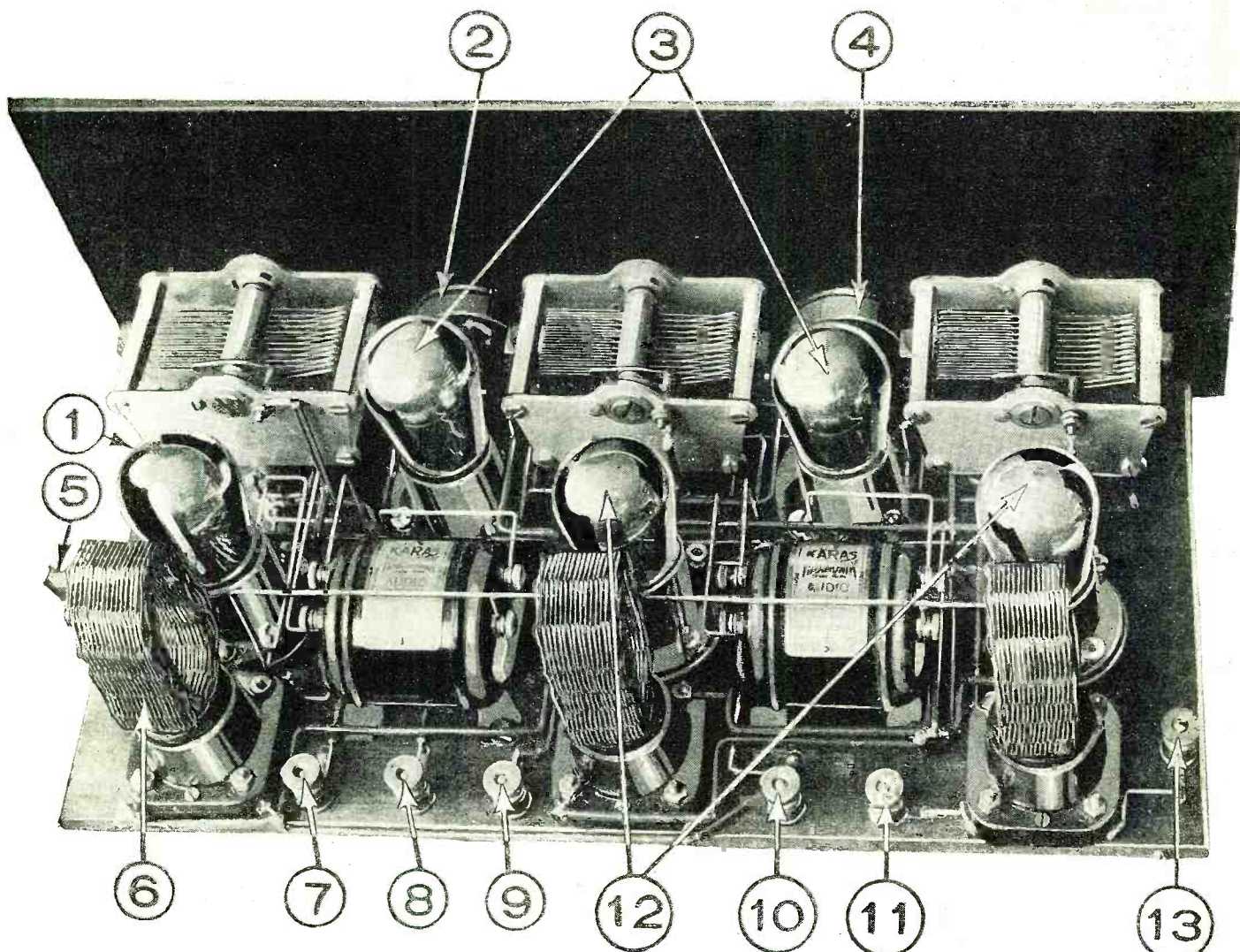
Rear view of the three-range receiver. 1 is the detector tube; 2, a potentiometer; 3, radio frequency amplifier tubes; 4, a rheostat; 5, the gridleak; 6, removable coil for different wave-lengths; 7, +45 volts; 8, +“A” and —“B”; 9, —“A”; 10, +90 volts; 11, antenna binding post; 12, audio frequency amplifier tubes; 13, the ground binding post.
