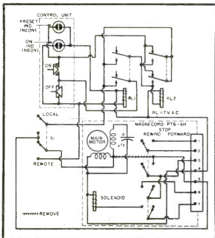
Fig. 4. Remote control system circuitry.
