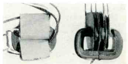
Fig. 3. Common pulse transformer (left) and equivalent wafer construction (right).
