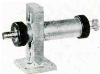
Fig. 1. Ridge wave guide crystal detector.
