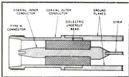
Fig. 1. Butt transition from coax to double-ground-plane strip line.
