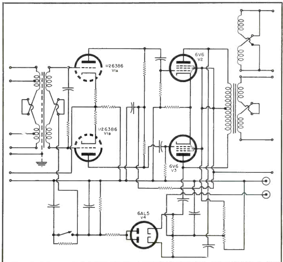
Fig. 7. Over-all schematic diagram of the Type BA-9-A “uni-level” amplifier.
