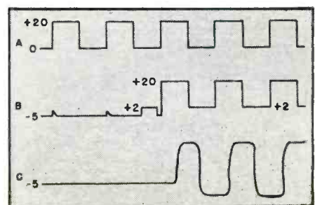
Fig. 7. Waveforms of the current-doubler flip-flop of Fig. 6, right.
