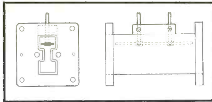
Fig. 2. Ridge wave guide attenuator.
