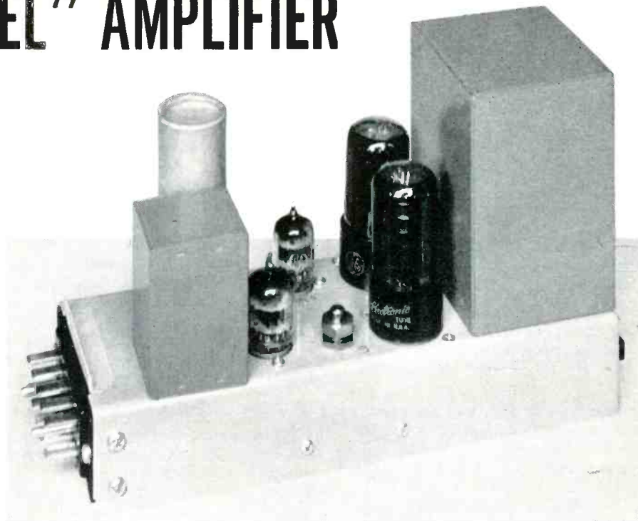
Fig. 1. Over-all view of Type BA-9-A "uni-level" plug-in amplifier.
