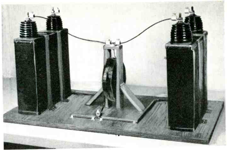
Fig. 5. Wave trap for operation at a single frequency only.
