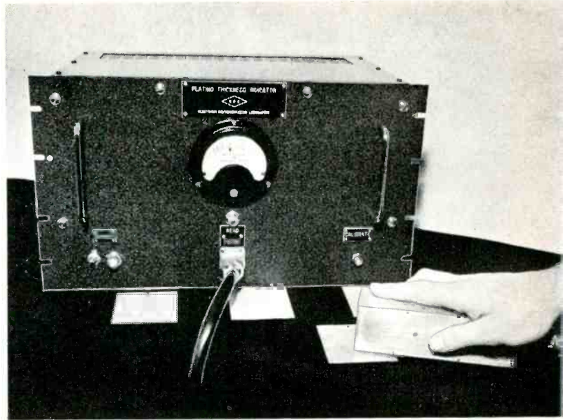
Fig. 4. Phase-angle thickness gage is insensitive to any variations in the probe-to-sample spacing.
