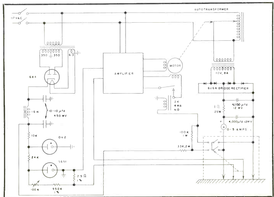
Fig. 5. Schematic diagram of the wave guide plating indicator.
