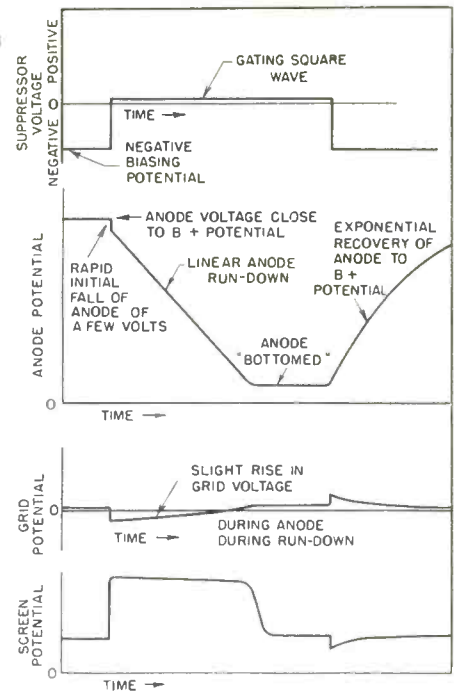
Fig. 4. Typical waveforms which can be obtained with gated Miller circuit.
