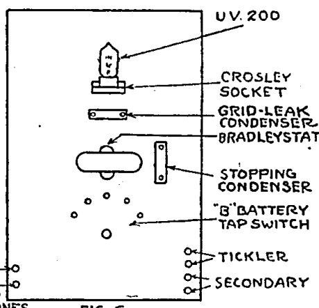
FIG. 6 BACK VIEW
