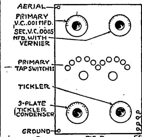
FIG. 3 FRONT VIEW
