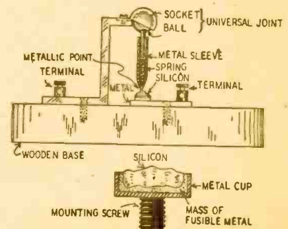
Fig. 3—The first patented mineral detector.
