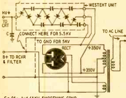
C-05-.1μf/6KV SMOOTHING COND Novel h.v. supply for scopes and televisers.
