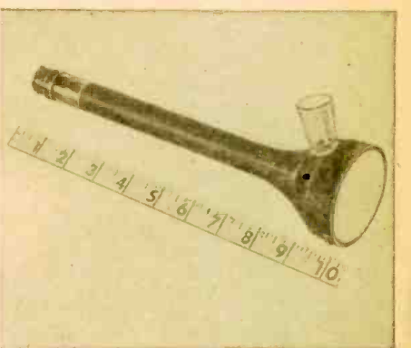
The tube. Cup insulates accelerating anode.
