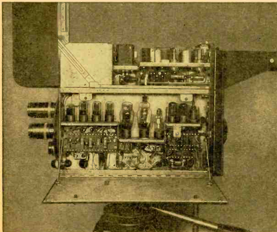
The preamplifier is in the lower section of this RCA image orthicon camera unit.
