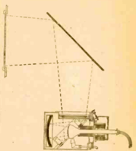
A multi-reflection optical system is used.
