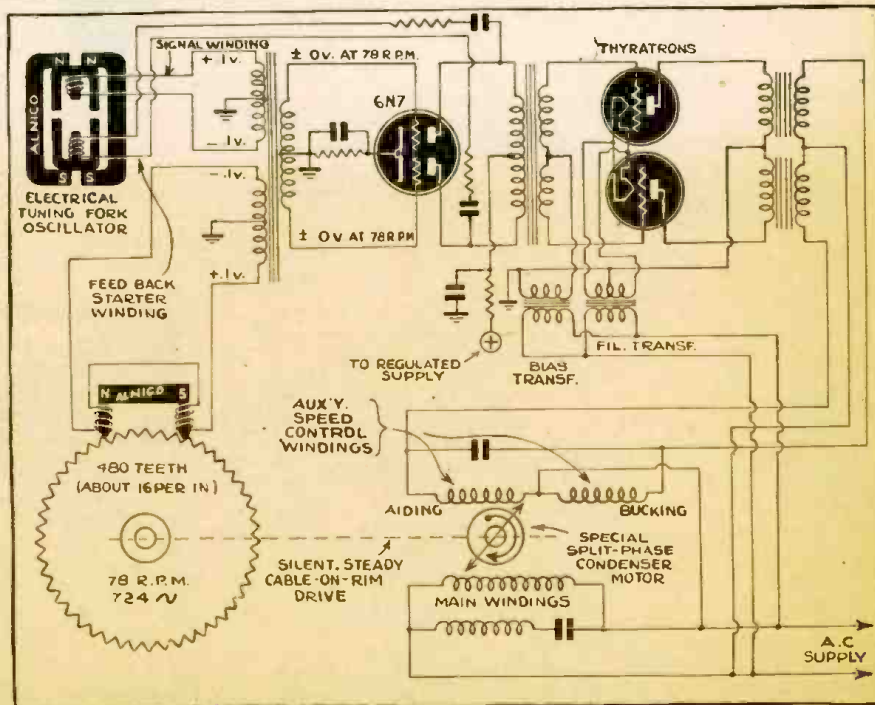
Fig. 2.—A proposed electronic speed-control system, using thyatrons to prevent speed changes.
