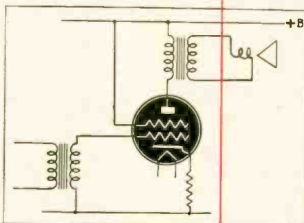
Fig. 7.—A degenerative current-feedback system.
