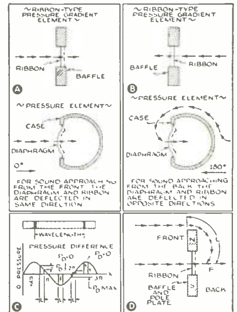
At A and B, above, principle of operation of the Cardioid directional microphone; at C and D, principles of operation of the ribbon-type mike. As shown at A and B, the diaphragm of the pressure element, because sound flows around corners always moves in the same direction regardless of direction of the sound; while, the ribbon of the pressure-gradient element reverses its direction of motion with reversal of sound direction. As shown at C, a pressure difference exists between 2 points in a sound wave. (NOTE that this difference will be zero at maximum and minimum pressure, and largest half-way in between, i.e., Pd is 90° OUT OF PHASE WITH THE PRESSURE); at D, a baffle is seen to introduce an acoustic-path difference, L, between front and back of ribbon (Pressure gradient = rate of change of pressure with distance = \frac{Pd}{L} approx., if L is small compared with wavelength.).
