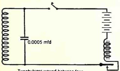
Twenty turns wound between four screws in panel to form loop 7 by 10 inches
