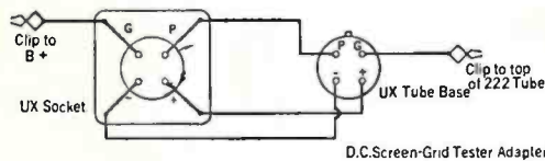
Fig. 2—The a.c. screen-grid tester adapter.
