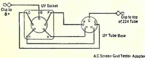
Fig. 1—The d.c. screen-grid tester adapter.
