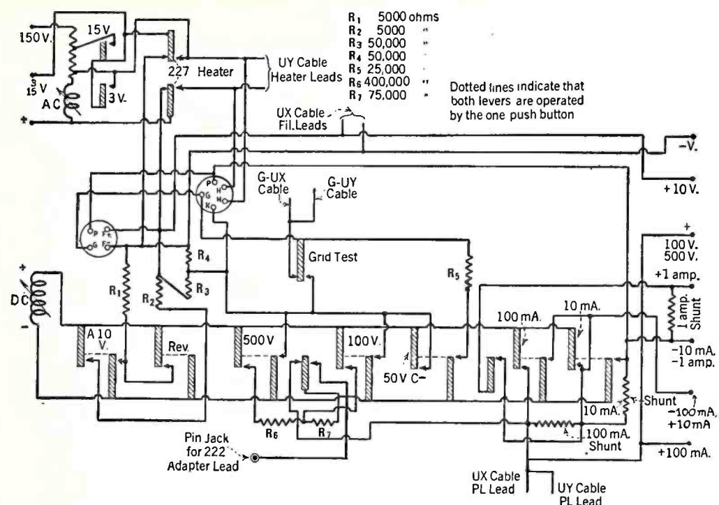
Fig. 1—Schematic of Diagnoser.
