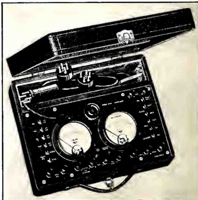
The New Jewell set analyzer tests a. c. screen-grid tubes.
