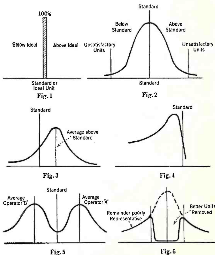
Curves indicating efficiency of production
