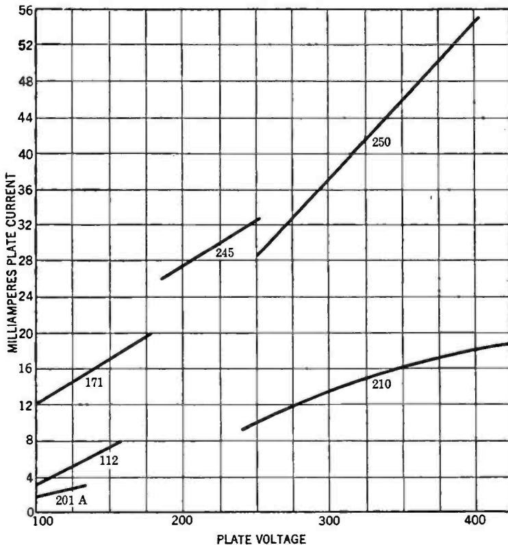
This graph indicates the correct plate currents for six popular types of tubes at various plate voltages, assuming a consistently correct C bias. These data should be pasted to the cover of your tube- and set-tester.
