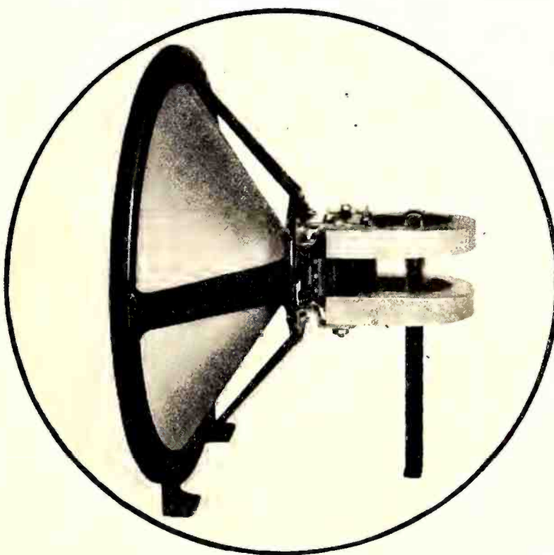
View of an inductor loud speaker motor with a paper cone attached. This loud speaker, of course, must be placed behind a baffleboard for best results.
