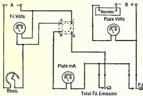
Fig. 6—D. C. tube-tester circuit.
