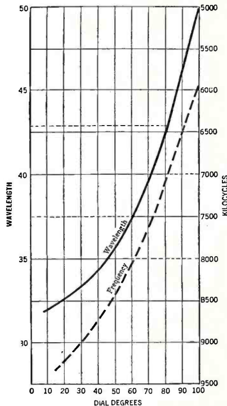
Fig. 3—Calibration curves of Mr. Leuck's oscillator.
