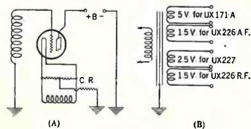
Fig. 8—(A) Method of obtaining negative C bias; (B) usual system of securing filament voltages in an a.c.-operated receiver.
