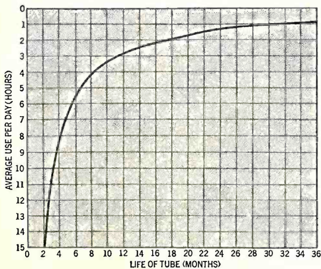
Showing how tube life varies with use.
