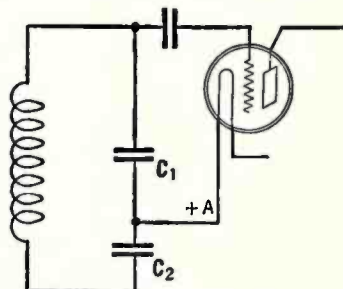
Fig. 3—The circuit used in problem No. 3.
