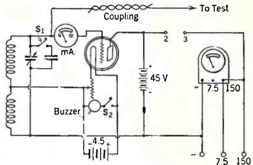
Fig. 3—Oscillator-voltmeter test combinations.
