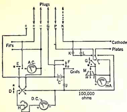
Schematic diagram of Mr. Howard's test set.
