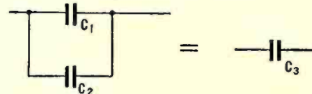
Fig. 5—Capacity formula for condensers in parallel.
