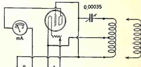
Fig. 4—Diagram of the oscillator tester shown in Fig. 5.
