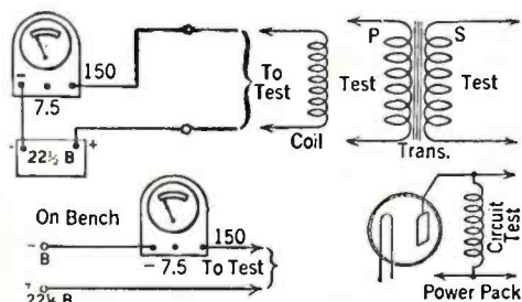
Fig. 2—Voltmeter continuity testing.
