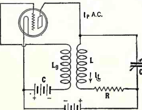
Fig. 3—A standard grid-tickler transmitting circuit.
