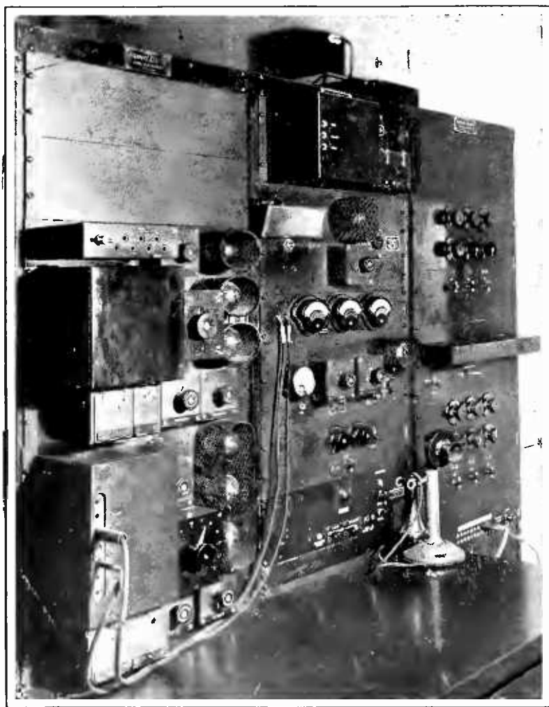
THE MIXING PANEL AT WBAL
