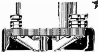
When the tube is inserted each prong is gripped the full length on two sides and held in a vice-like grip. Dirt cannot remain on the springs or prongs here.
