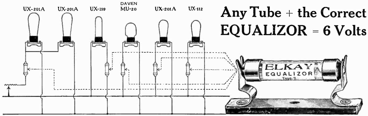
Filament Line of Standard Two-Stage Tuned R.F. Circuit
