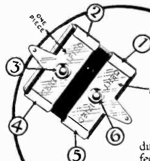
Electrad "Six-Point Pressure" Condenser
