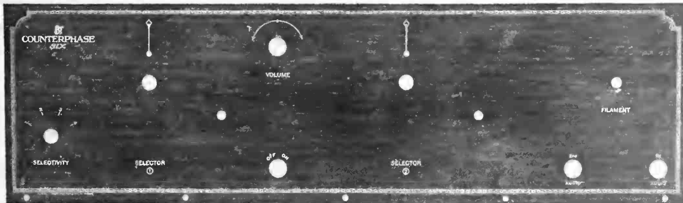
Crowe Panel for B-T Counterphase-Six, Size 7 x 24, Accurately Pierced, Ready for Use. (Packed in Individual Containers, with Insulation and Directions)
