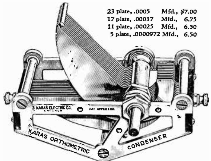
THE KARAS ORTHOMETRIC (STRAIGHT FREQUENCY LINE) CONDENSER
