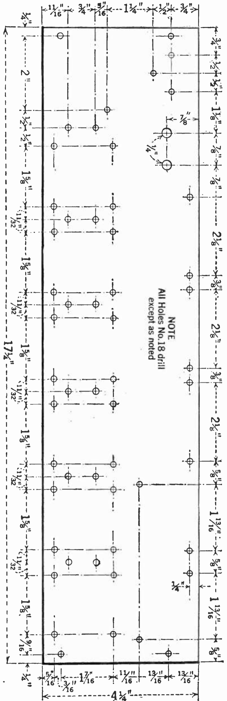
FIG. 7 Drilling dimensions for the sub-panel
