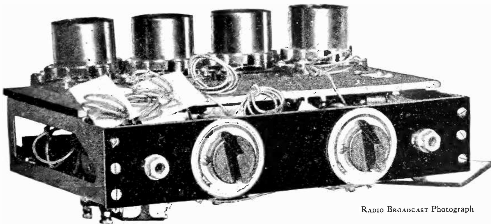
FIG. 1. SUB-PANEL ASSEMBLY
