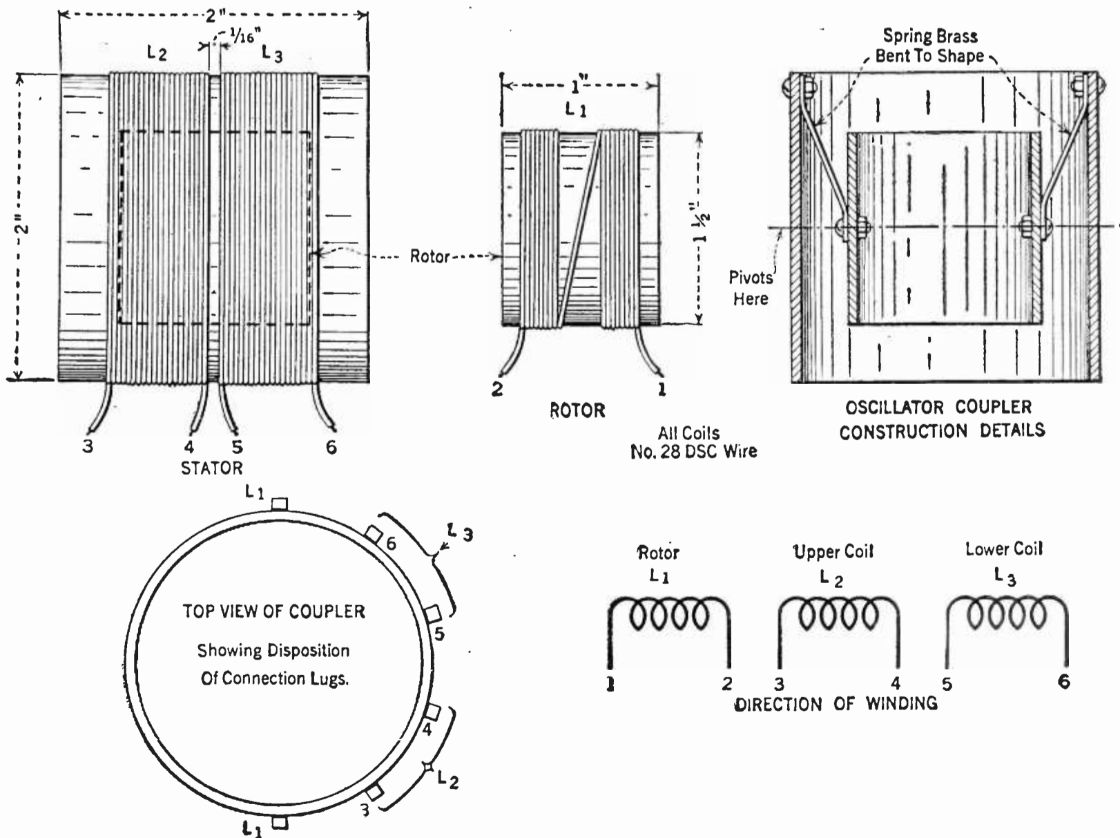
DETAILS OF CONSTRUCTION OF THE OSCILLATOR COUPLER
