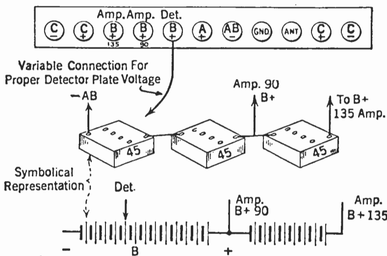
FIG. 9. TESTING PLATE VOLTAGE
