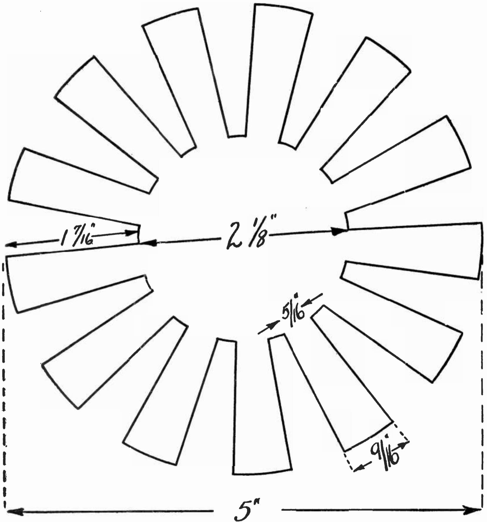
FIG. 2. A TEMPLATE FOR THE SPIDER WEB COILS
