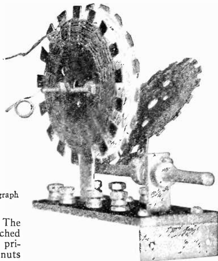
FIG. 3A-B. A HOME MADE COIL UNIT
