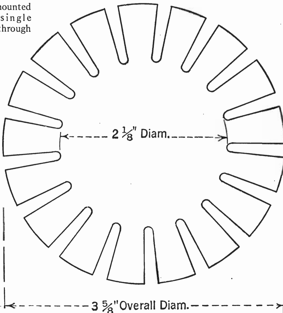
FIG. 4 A pattern for the coil form. This may be cut out and pasted on cardboard so that it can be duplicated exactly
