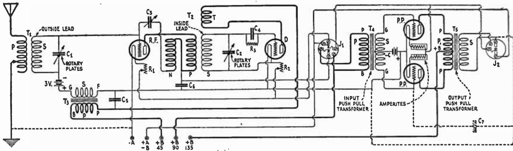
FIG. 8. THE WIRING ARRANGEMENT
