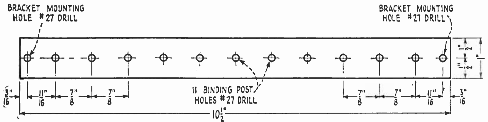
FIG. 21. THE BAKELITE BINDING POST LAYOUT
