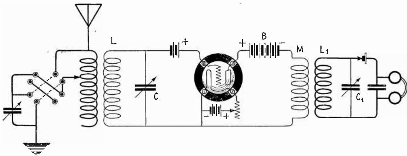
A VACUUM TUBE AND CRYSTAL COMBINATION
