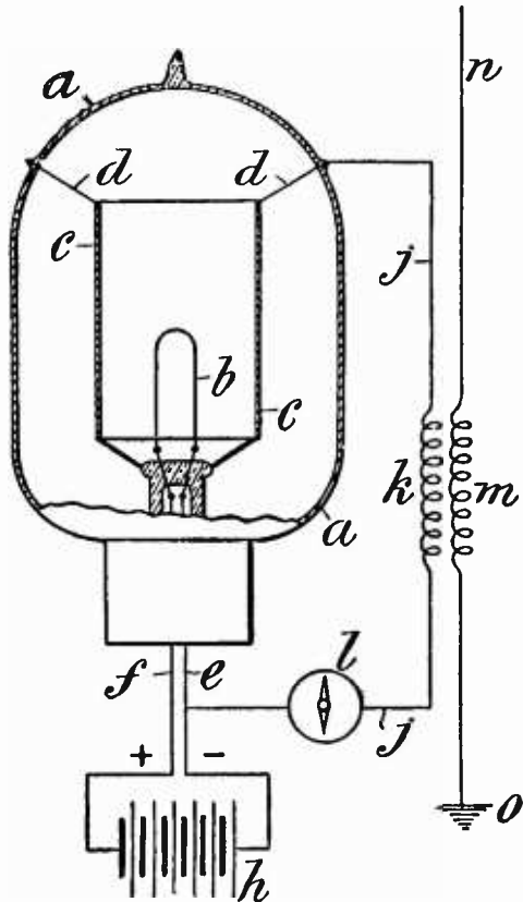
FIG. 1 The original Fleming valve arrangement
