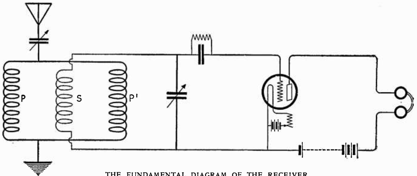
THE FUNDAMENTAL DIAGRAM OF THE RECEIVER
