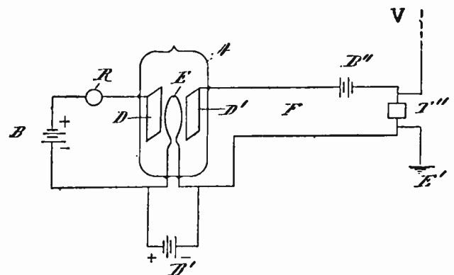
FIG. 2 One form of the De Forest patent No. 841,387
