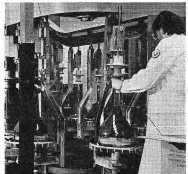
After the tube has passed all tests it is given its final washing before paint is applied to the outside.
