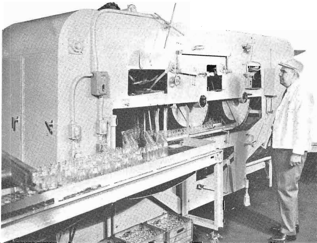
In this machine, bottles are removed automatically from their cases and placed on conveyors leading to the washer-loader unit at the left.
