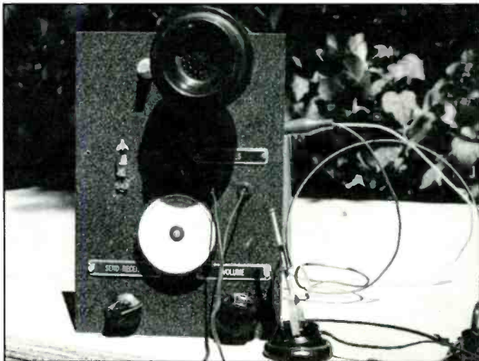
Don Aprin is all set to hear DX, and to talk to them at the same time using his novel regenerative transceiver. Note the tiny pencil tube on the left side of the front panel.
