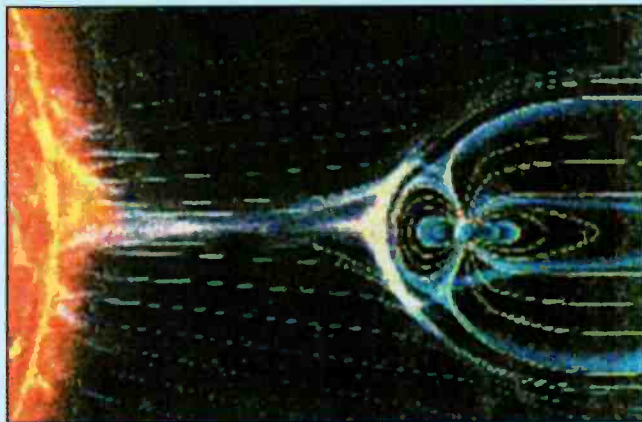
Solar activity affects the Earth's magnetic field.
