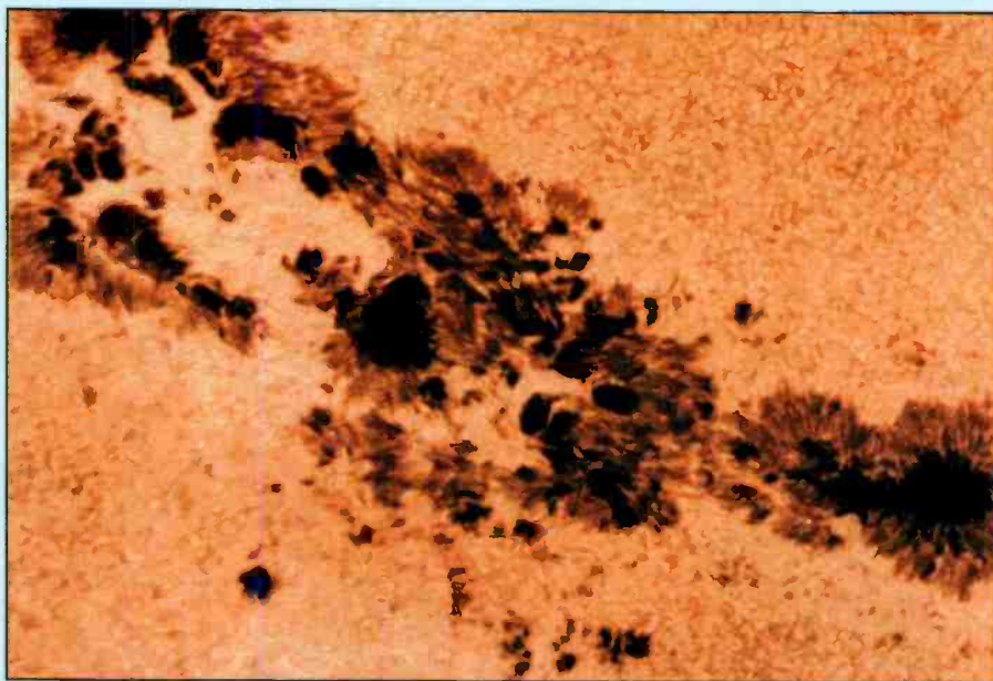
This photo of the Sun shows several sunspots.
