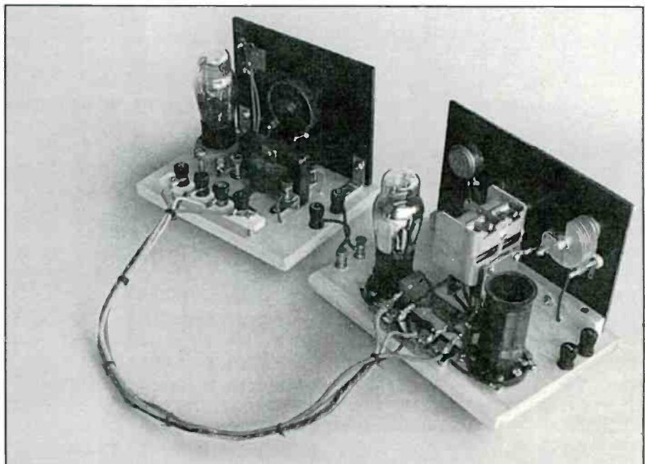
The rear view of the receiver and companion amplifier. Note how the layout is kept clean and uncluttered; even the interconnecting cable harness is laced to keep it orderly.
