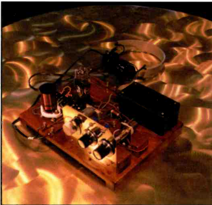
Jim's eclectic radio. A sharp contrast in vintage meets "new," to produce this unique receiver.
