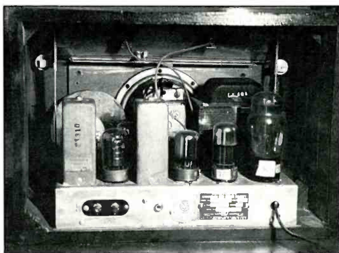
Rear view of the Canadian Red Cross receiver. The set is transformer-powered, making it unlikely that the set was a low-end mass produced unit intended for mass consumption.
