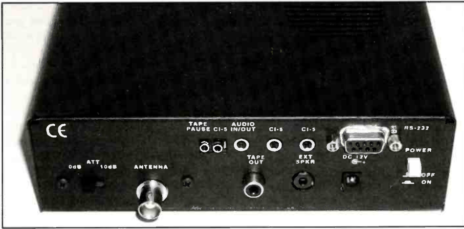
Some receivers, like this Optocom receiver, have an attenuator built right in. It's the switch at the far left on the back panel. Try that first, if you have one, before adding outboard accessories.
