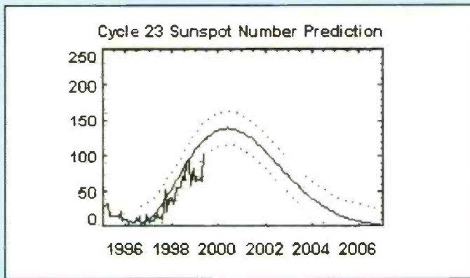
The current Solar Cycle — No. 23 — is expected to peak in mid-2000. By combining data about geomagnetic activity during the previous solar cycle with sunspot counts for the current cycle, David Hathaway and collaborators are able to predict when the next sunspot maximum will occur. The dotted lines above and below the solid curved line indicate the prediction curve's range of error.
