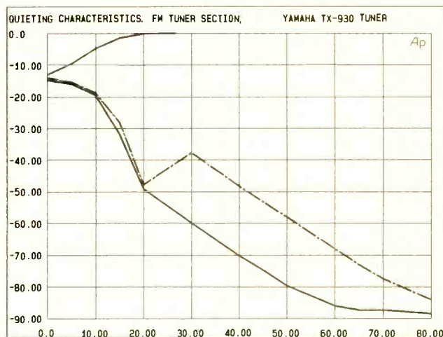
This plot shows the quieting characteristics in mono (lower solid line) and stereo (dashed line) as a function of signal strength at the antenna input. The upper solid line is the audio output reference level.
