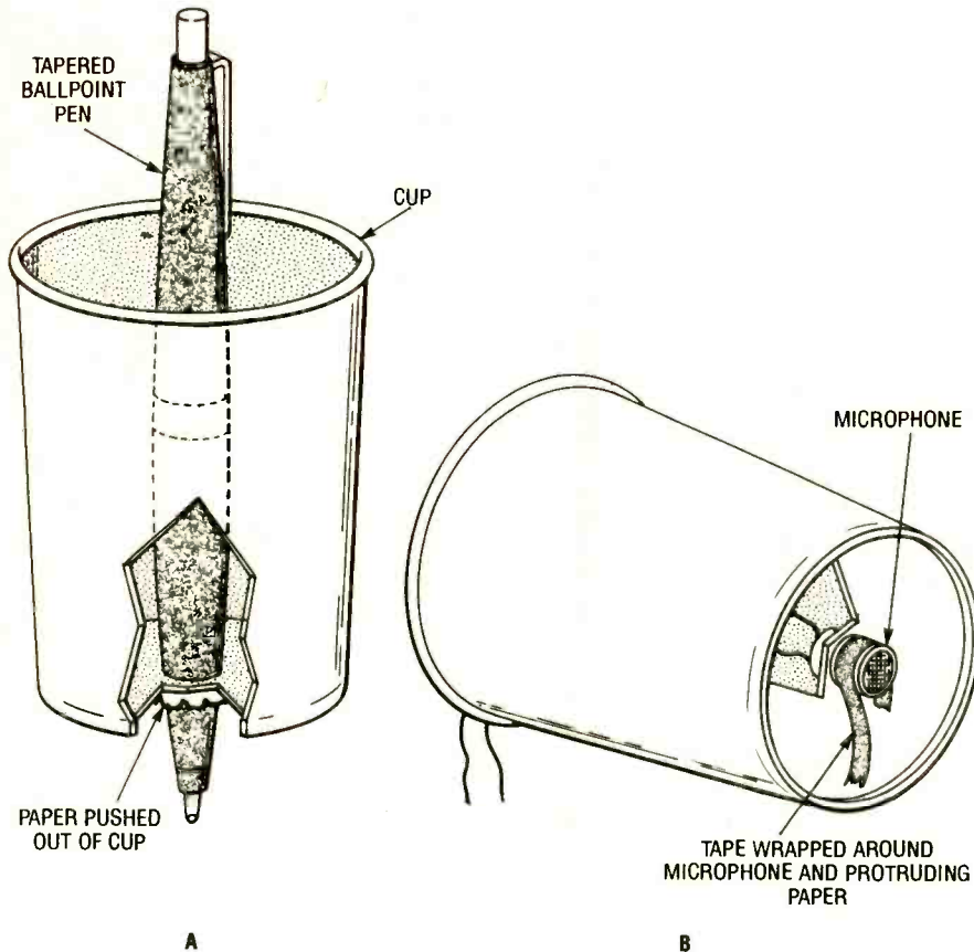
Fig. 4. Enlarge the hole in small increments, testing the fit of the microphone as you go (A). Wrap a narrow piece of tape around the microphone to hold it in place (B).
