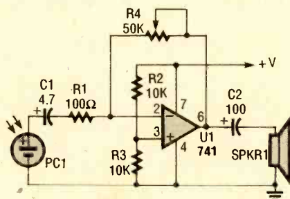
Fig. 2. The receiver portion of the communicator is just as simple as the transmitter: A solar cell picks up light emitted by the transmitter and converts it into a varying DC voltage.
