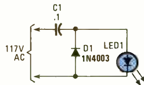
Fig. 1. This simple pilot light can be used to indicate the presence of 117 volts in AC-operated equipment.
