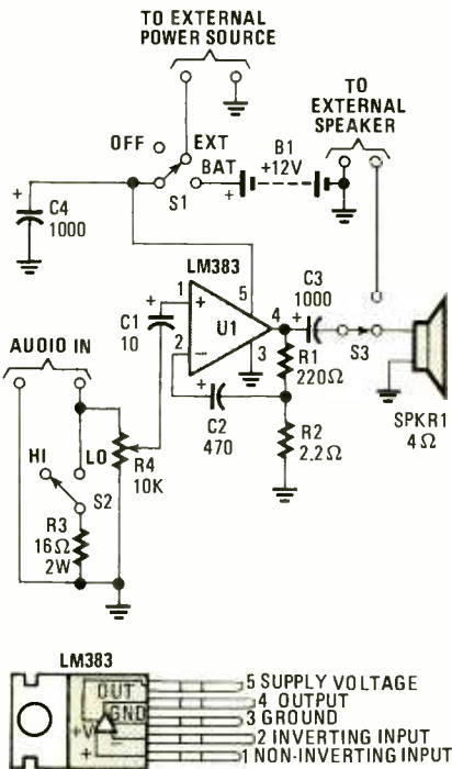
Fig. 3. This Audio Power Amp—built around an LM383 8-watt, audio power amplifier—can be used to boost an audio signal to a sufficient level so that it can be heard in a high-noise environment.
