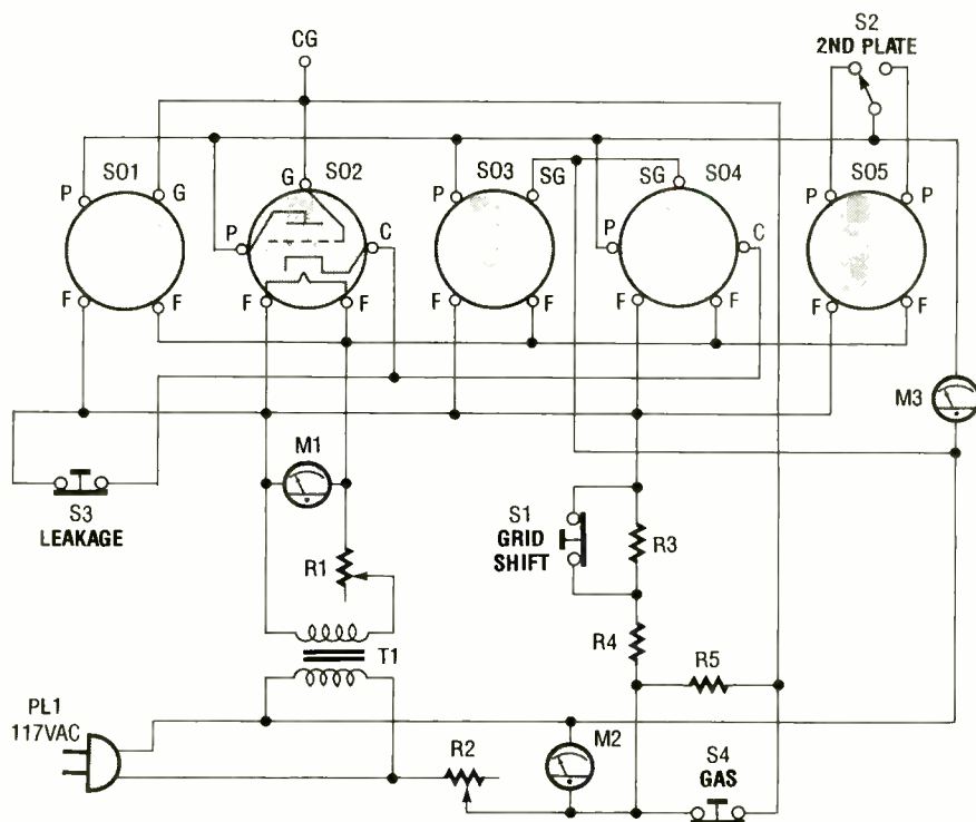
Fig. 1. Our basic late-1920's tube-tester circuit. It needs more refinements (to be added next month) before being construction-ready, so don't get out your soldering irons yet!
