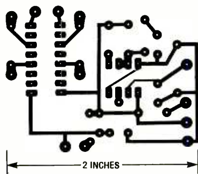
Fig. 2. The full-scale foil pattern for the Silencer's printed-circuit board is shown here. When etching the board, be sure that you do not over or under etch the board. After etching your board, check it against the pattern shown here for opens and shorts.
