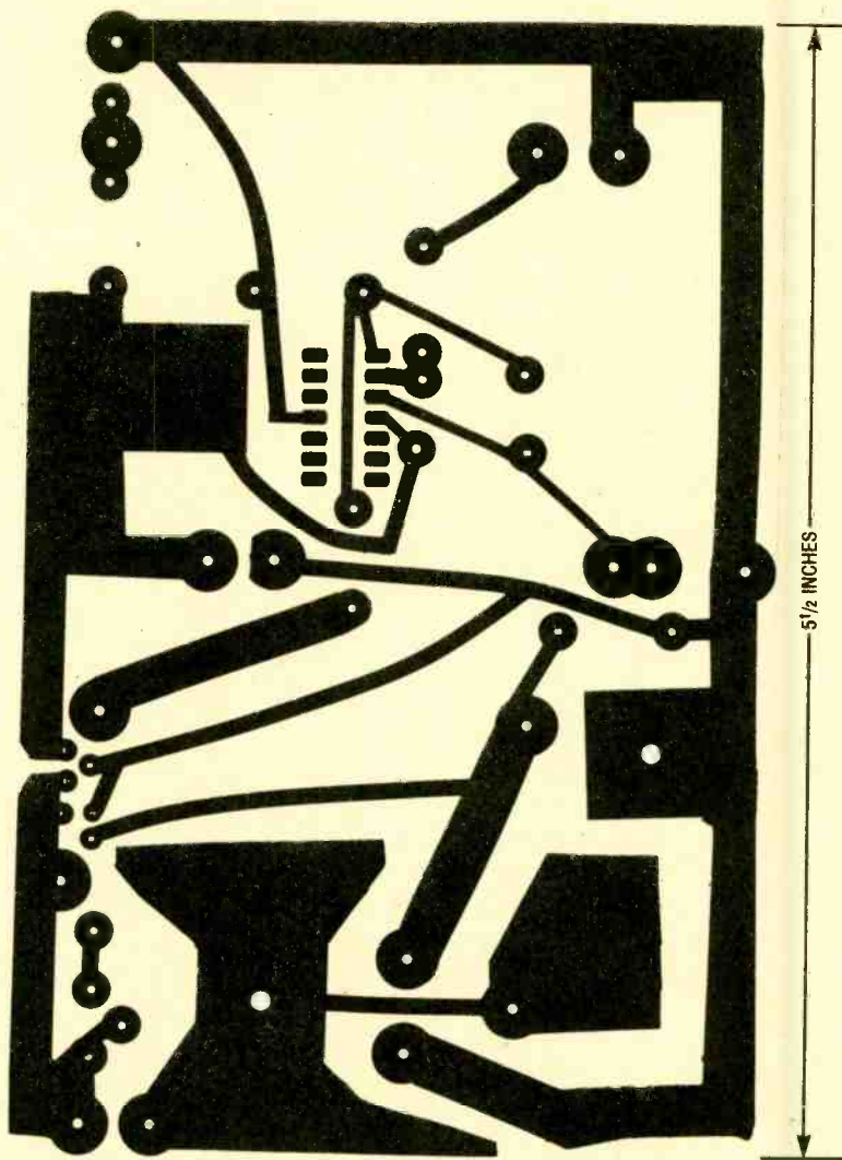
Fig. 2. Although there is nothing to prevent you from assembling the circuit on experimenter's or perfboard, printed-circuit assembly makes the job much easier and helps to reduce the common errors that find their way into hobby-electronics construction projects. Here's the foil pattern used by the author for his prototype.
