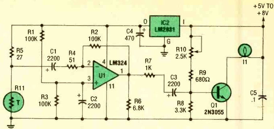
Fig. 1. The Lepton Candle is built around relatively few components; its main elements are 1/4 of a quad op-amp (U1) and a thermistor (R11). Thermistor temperature changes, producing proportional voltage changes, are presented to the op-amp and used to control lamp I1 through transistor Q1.
