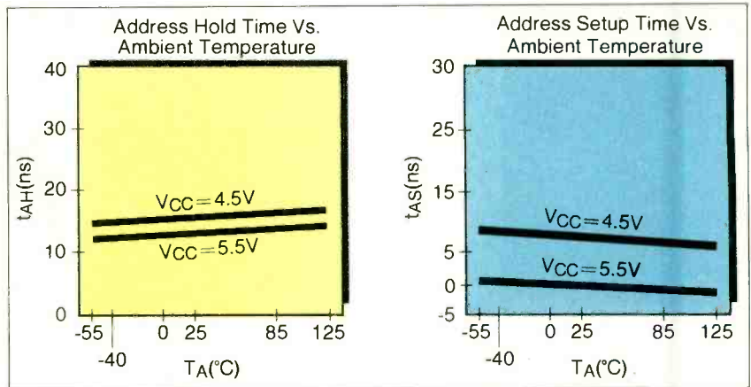
Fig. 2. Time of operation plotted against temperature.
