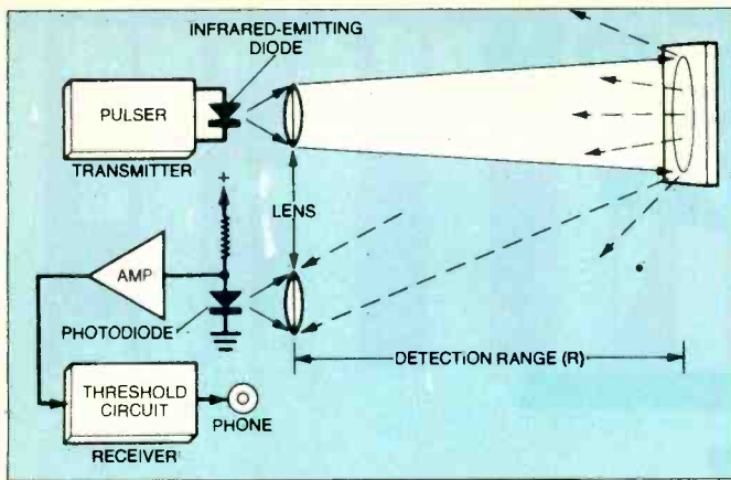
Fig. 2. An infrared travel aid for the blind.
