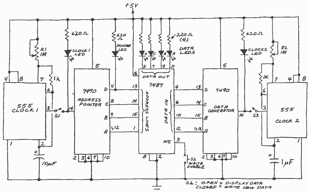
Fig. 3. Automated RAM demonstrator with pseudo-random data generator.
