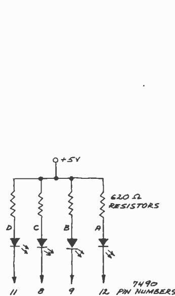
Fig. 1. Circuit indicates address pointer output.
