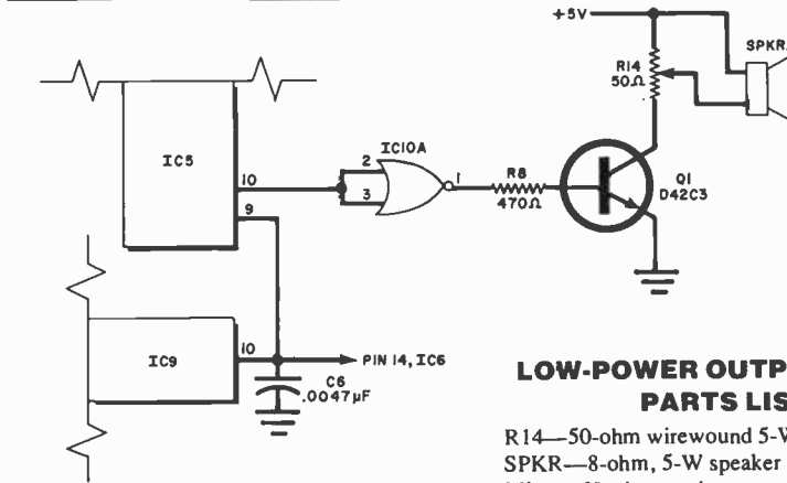
Fig. 2. Output stage for the low-power version.
