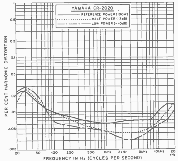
Total harmonic distortion at rated (100 W), half, and low power.
