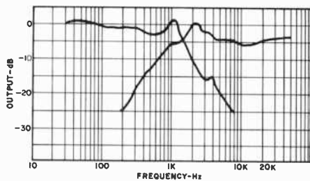
Fig. 3. Idealized response of Fig. 1 may actually be like this.
