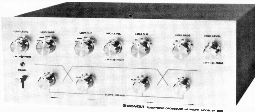
U.S. Pioneer Electronics Model SF-850 crossover network provides for selection of 6-, 12-, or 18-dB/octave slopes.
