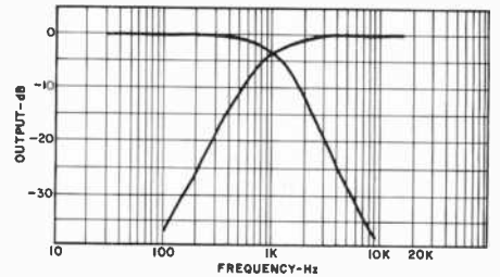
Fig. 1. (A) L/C crossover networks (12 dB/octave) and (B) response.
