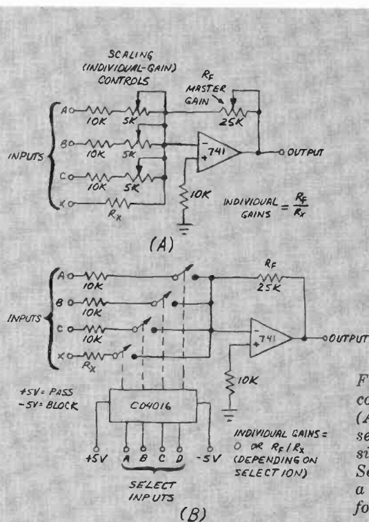
Fig. 1. Synthesis circuits: (A) strings, (B) single-resonance horn, (C) double-resonance horn, (D) woodwind, (E) flute or piccolo.
