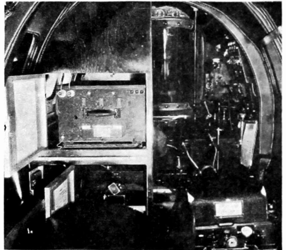
Interior of the "Early Bird," showing the Western Electric Radio transmitter and receiver.
