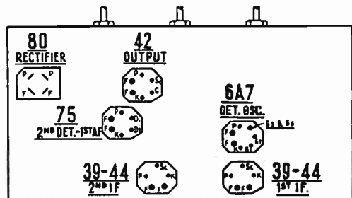
Tube layout (underside)
