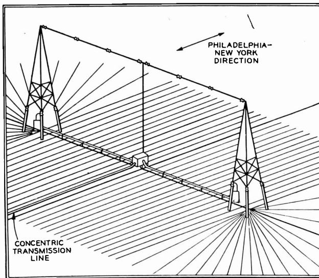
Directional Characteristics of WOR's New Station
