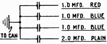
(46) BY-PASS CONDENSER CONNECTIONS
