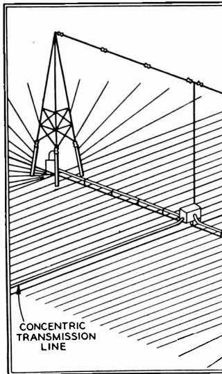
Directional Characteristics
