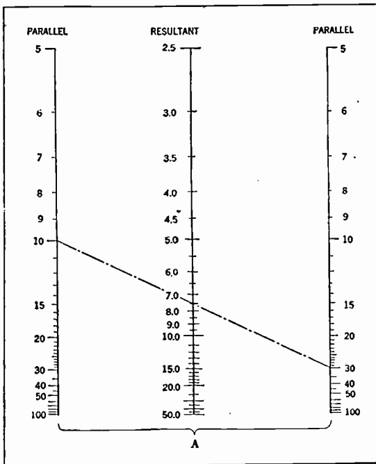
Resistances in Parallel (in ohms)
