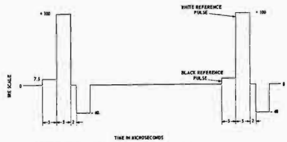
Fig. 33. Typical vertical interval reference signal.
