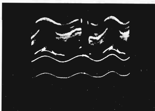
Fig. 114. Interference—120 Hz—vertical.
