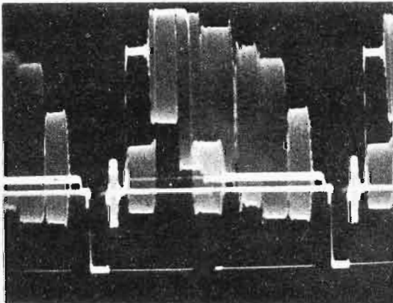
Fig. 36. Color bar signal—horizontal—wideband.
