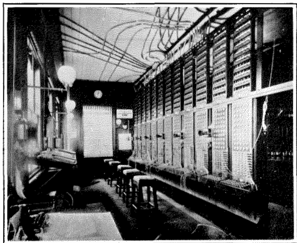
Figure 3—Interior of Wellington Exchange in 1887
