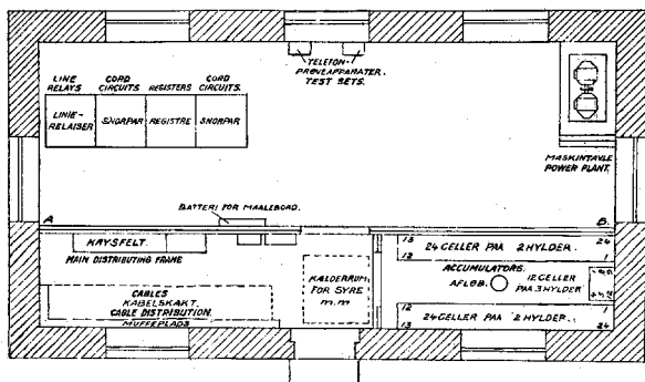
Figure 7—Floor Plan of Rural Exchange
