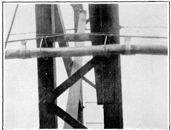
Figure 9—Cable Lifted from Rings by Wire Ties at a Through Strand Position
