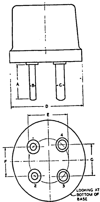
SMALL FOUR-PIN BASE
