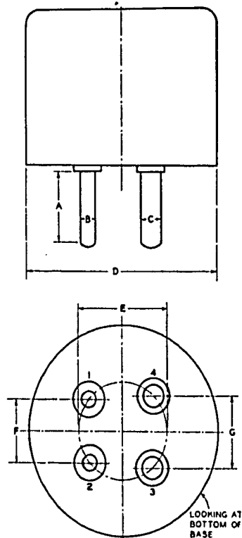
LARGE FOUR-PIN BASE, WITHOUT BAYONET PIN
