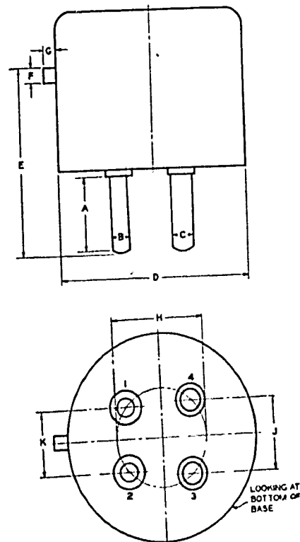
LARGE FOUR-PIN BASE WITH BAYONET PIN
