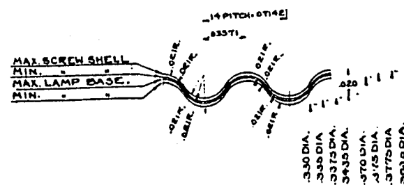
STANDARD FOR MINIATURE SCREW SHELL AND LAMP BASE.
