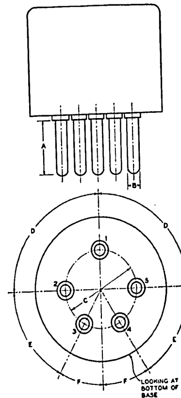
LARGE FIVE-PIN BASE
