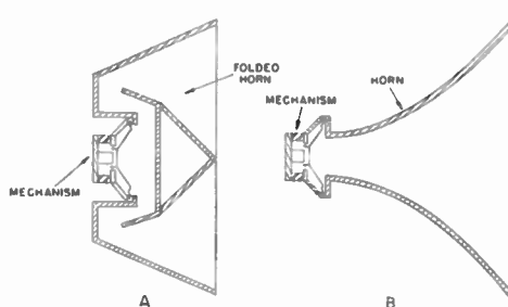
Fig. 12—Large-throat horns for horn loudspeakers. A) Folded horn. B) Straight-axis horn.
