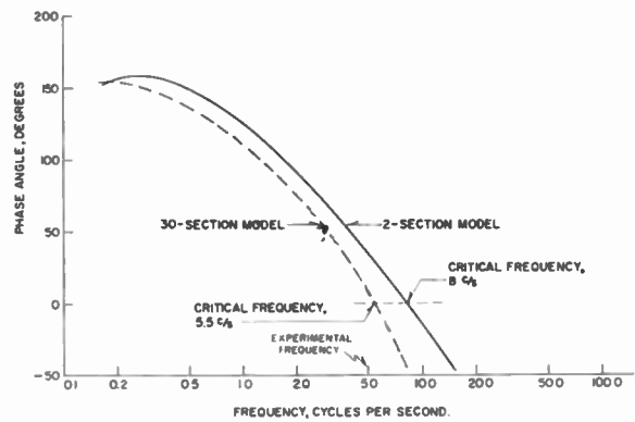
Fig. 11—Phase shift. Boiling reactor reactivity feedback loop.
