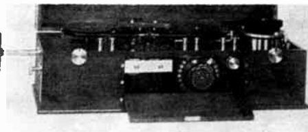
Fig. 4—English Marconi magnetic detector, this assembly being specially designed for receiving time signals. Used until after World War I, when tube receivers became standard. These detectors had to be wound up periodically, a clock-spring motor supplying power to the rotating iron-wire endless cable.
