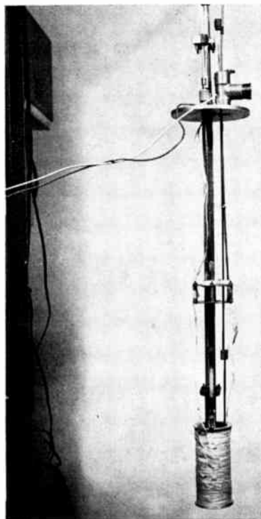
Fig. 10—Tunable L-band maser using superconducting solenoid to provide the magnetic field. This particular solenoid can supply up to 6500 gauss with a 1\frac{1}{2} -volt dry cell and a variable resistor. A closed superconducting circuit may be set up, after which a persistent current maintains the magnetic field and the dry cell may be removed. [After S. H. Autler, M.I.T. Lincoln Laboratory, Lexington, Mass., private communication.]
