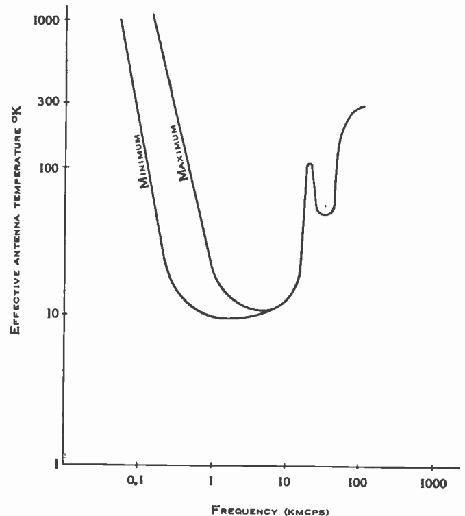
Fig. 6—Space noise from galactic, corona and atmospheric contributions (after [12]).
