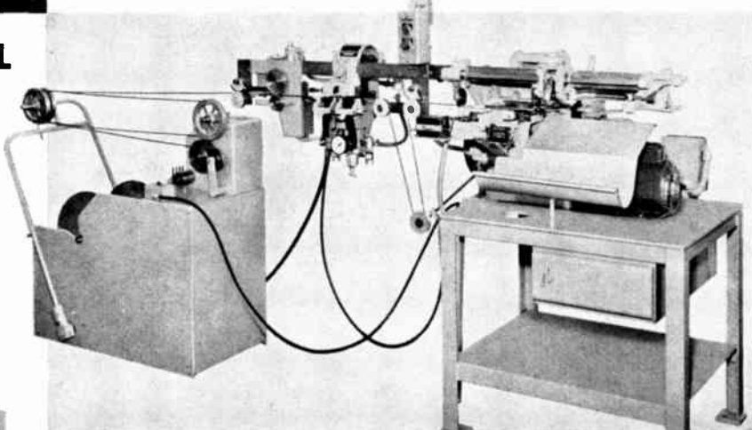
Model CS-6 Artos automatic machine produces leads from 2 to 194 in. long. Shown with self-regulating pre-feeder and automatic wire marking device.
