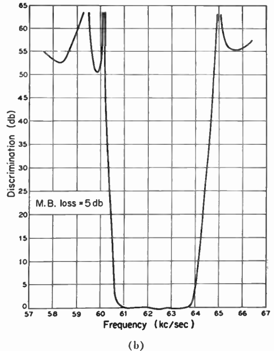
Fig. 11—Crystal channel filter. (a) Typical section showing use of divided plate crystals. (b) Attenuation characteristic for two sections of (a).
