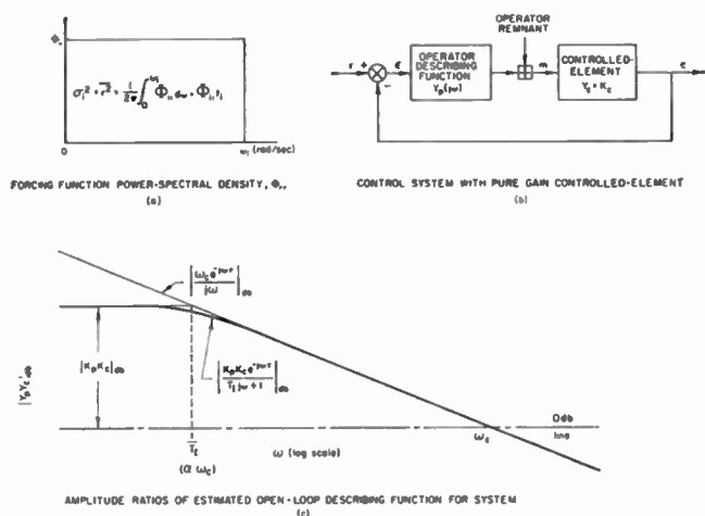
Fig. 5—Given and estimated characteristics for manual control system with Y_c = K_c .
