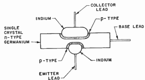
Fig. 4—A p-n-p alloyed germanium junction transistor. Two small dots of indium are alloyed into a single crystal n -type germanium wafer at a temperature of approximately 500^{\circ}\text{C} . At each indium-germanium interface the surface of the germanium wafer dissolves as indicated in the drawing and upon cooling the assembly, the indium becomes supersaturated with germanium, and a recrystallization layer of germanium heavily doped with indium is formed upon the wafer. These recrystallized layers then form the emitter and the collector sections of a p-n-p junction transistor with the original n -type wafer playing the part of the base. The leads to the three sections are connected to the indium dots and to the base as shown.
