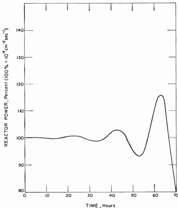
Fig. 8—Reactor power vs time. Average flux = 10^{14} cm -2 sec -1 . Actual gain = 1.1 \times "critical gain."
