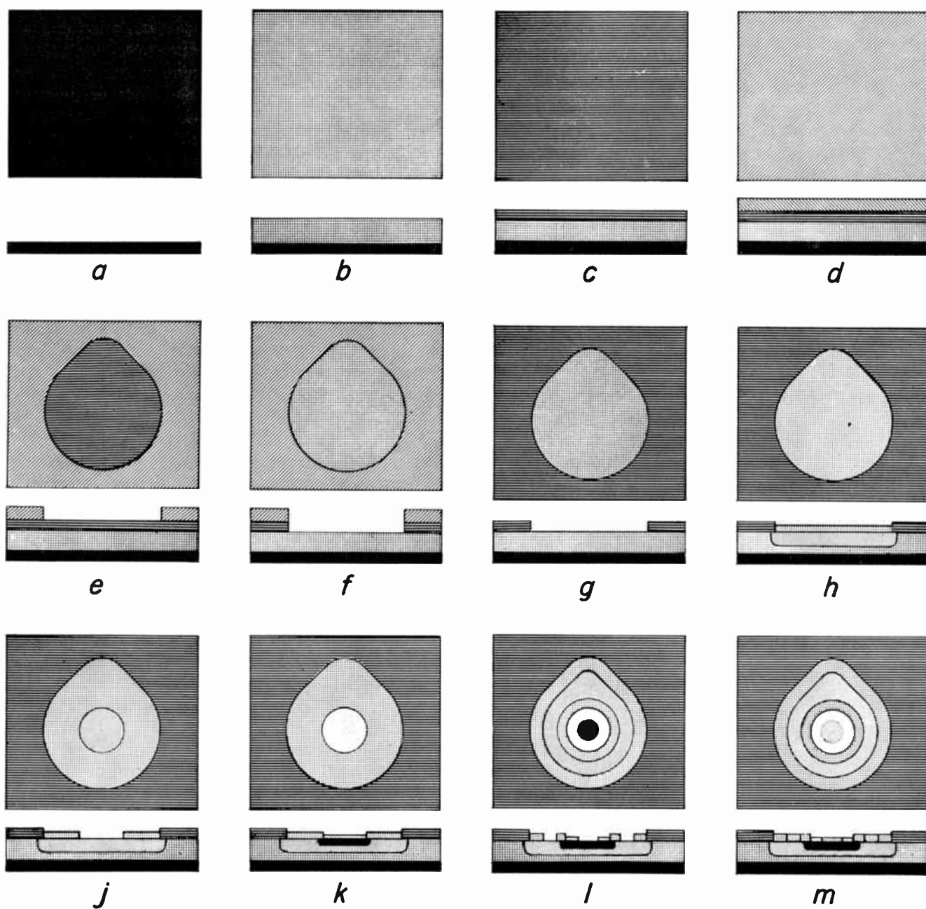
Fig. 13—Steps in fabricating a silicon epitaxial planar transistor. The operations are described in the text.
