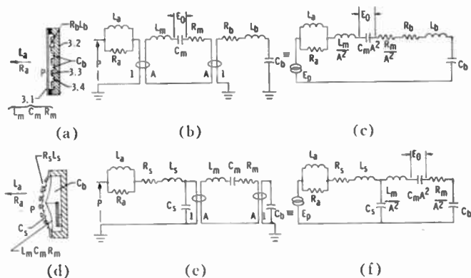
Fig. 3—Pressure microphone with displacement responsive transducer.
