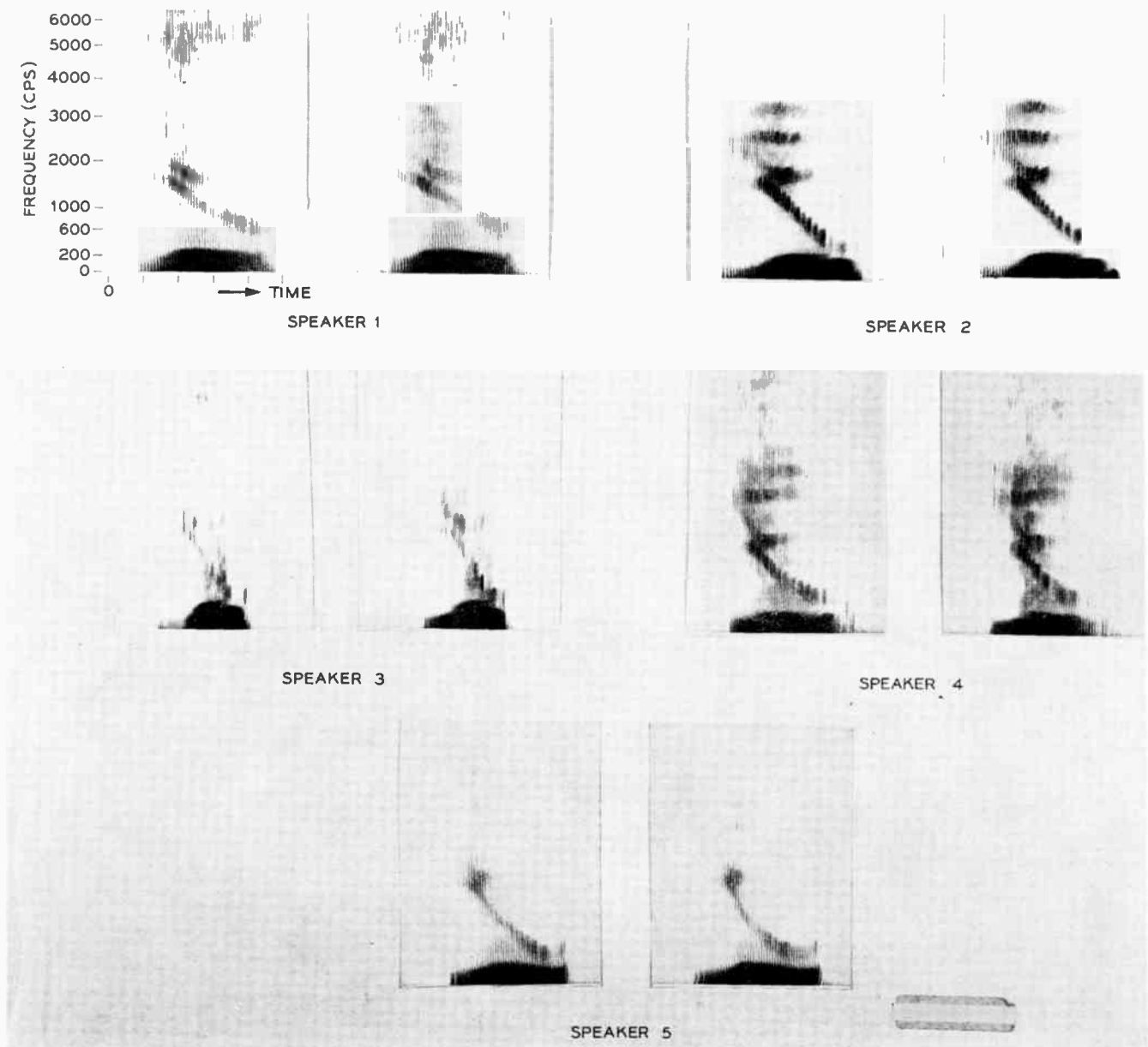
Fig. 4—Sound spectrograms of five talkers each pronouncing the word you twice, show that variations in spectral pattern from talker-to-talker are much greater than between successive utterances from the same talker.
