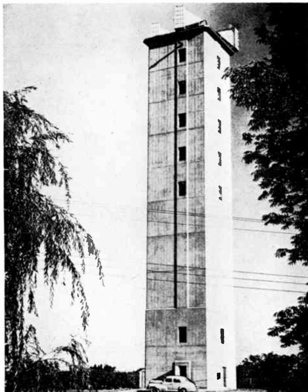
Fig. 1—Microwave radio relay circuits, exemplified by this Bell System TD-2 repeater tower, carry thousands of speech transmission channels on one radio circuit. The horn-lens antennas atop the tower, with a gain of 40 db and a beamwidth of 2 degrees [2], employ delay lenses [3] which were later found to be effective for directing the acoustic speech waves issuing from loudspeakers [4].
