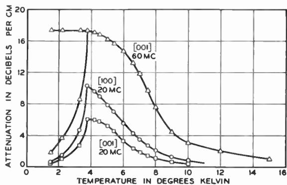
Fig. 1—Longitudinal wave attenuation for single crystal tin along the [001] and [100] axes.
