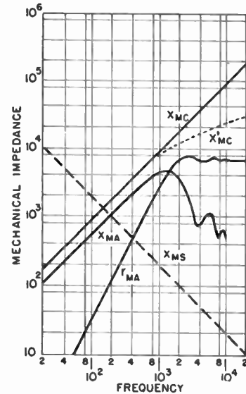
Fig. 3—Mechanical impedance-frequency characteristics of a direct-radiator dynamic loudspeaker with a cone 4 in in diameter. x_{MC} = the mechanical reactance of the cone and coil. x_{MA} = the mechanical reactance of the air load. r_{MA} = the mechanical resistance of the air load. x_{MS} = the mechanical reactance of the suspension system. x'_{MC} = the mechanical reactance of the cone and coil where wave motion occurs in the cone.
