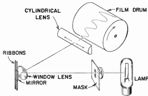
Fig. 3—Optical system of Duddell oscillograph.
