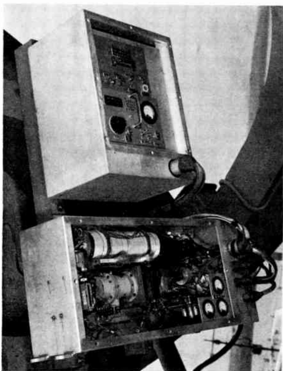
Fig. 6—35-kMc radio receiver for mounting on back of 10-foot radiotelescope at the USNRL. The waveguide from the focal point of the reflector can be seen entering the receiver on the left of the assembly. (Courtesy of USNRL.)
