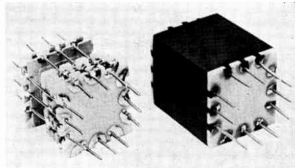
Fig. 19—Signal Corps-RCA micromodules—unencapsulated and encapsulated versions of about 1959. As you read this, there will have been 12 telephone-book size reports circulated to industry on this Signal Corps industry-wide program by RCA, the leading contractor.
