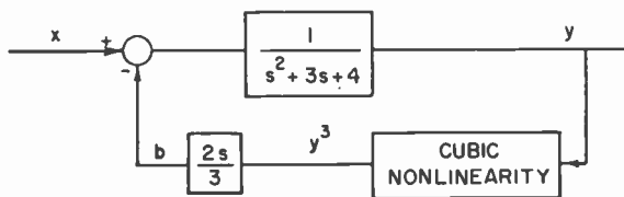
Fig. 4—Elementary nonlinear feedback system.
