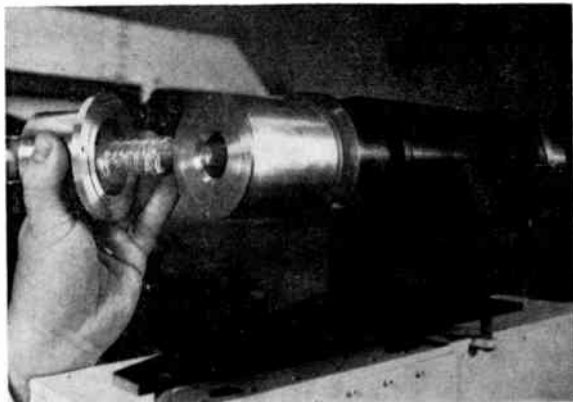
Fig. 6—Ruby laser showing flashtube and ruby.
