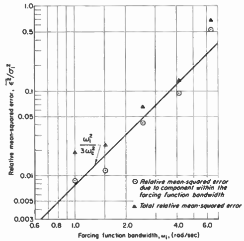
Fig. 7—Comparison of estimated and experimental mean-squared error.
