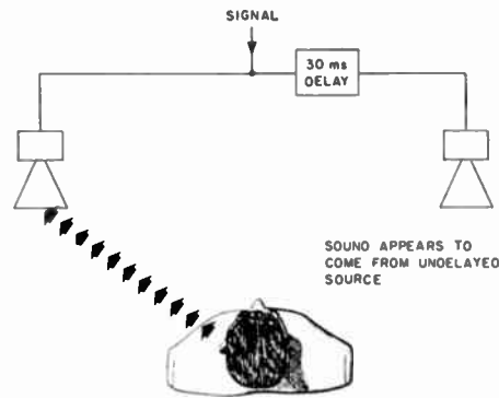
Fig. 3—Because of the precedence or Haas effect, the same sound issuing from two sources appears to come from the one with least delay.
