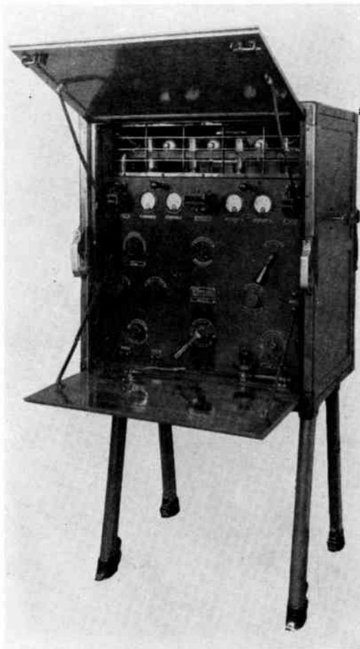
Fig. 4—Developed and designed, 1922-1923, by the General Electric Co., BC-127 400 watt, low frequency transmitter. It was transportable, and the first regular Signal Corps transmitter to use the MO-PA technique. Power-MG set. (Courtesy of RCA .)
