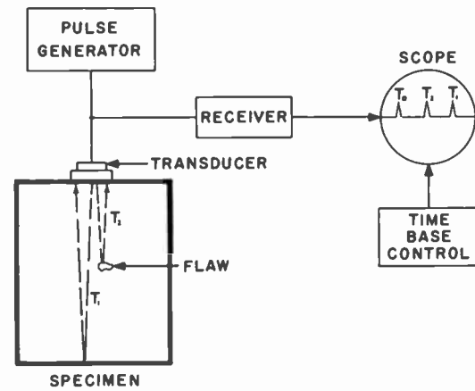
Fig. 3—Ultrasonic flaw detection by measuring reflected echo time.
