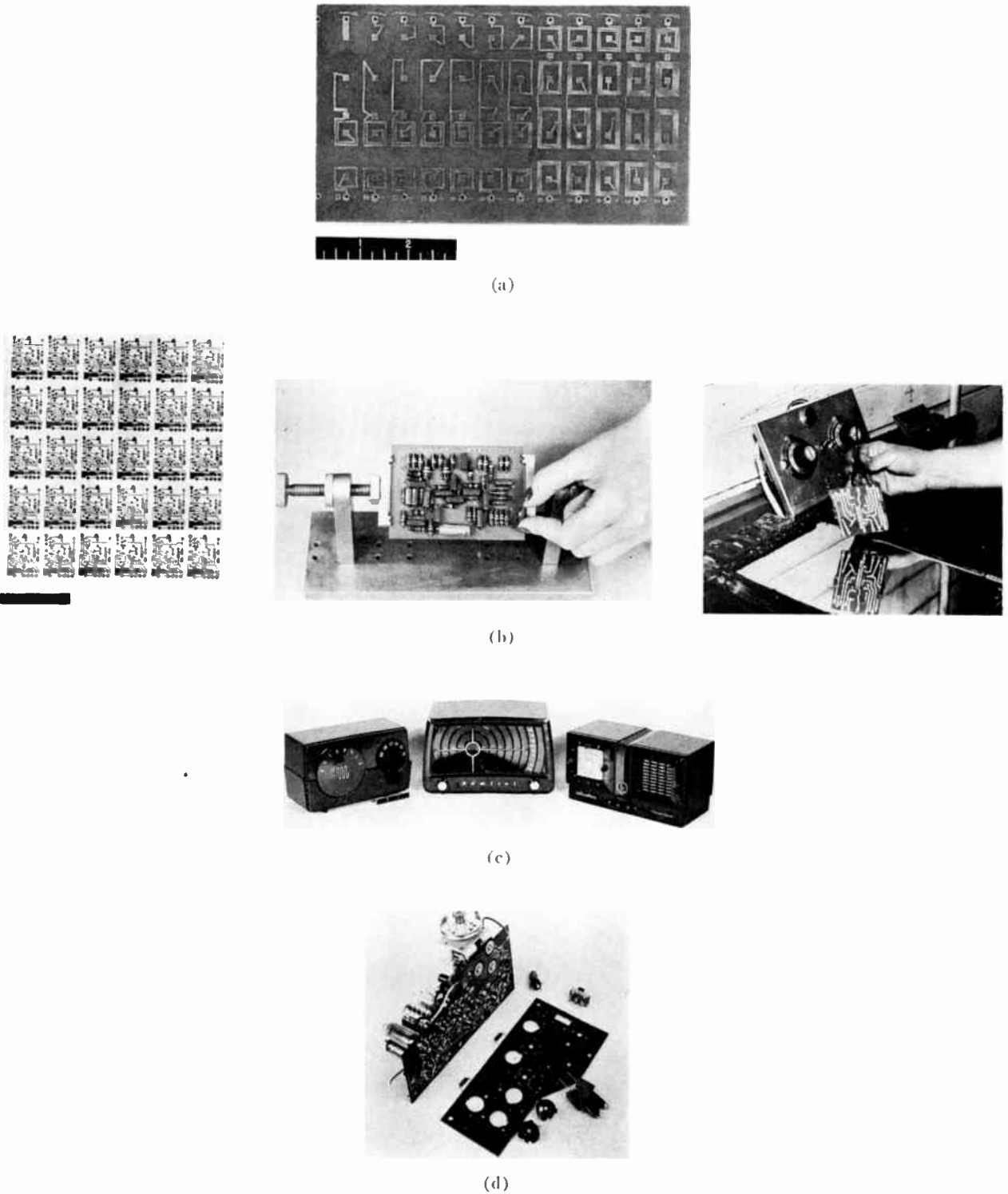
Fig. 5—Printed Wiring:
