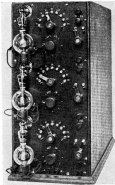
Fig. 3—Three-stage De Forest audion amplifier of the type first built by the Federal Telegraph Co. in 1912. This was the earliest known commercial cascade audio frequency amplifier, and was the type demonstrated to the U. S. Navy in September, 1912. (Courtesy of Electrical Communication .)
