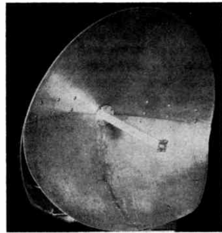
Fig. 6—Shaped-beam antenna employing a modified paraboloidal reflector.
