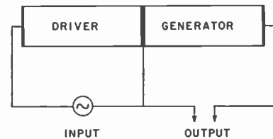
Fig. 4—Ferroelectric electromechanical voltage transformer. For maximum output voltage, the over-all length of the rod is made mechanically resonant at the electrical driving frequency.
