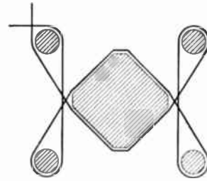
Fig. 3—Nylon thread mounting used on quartz bars of the Physikalisch Technische Bundesanstalt in Germany.
