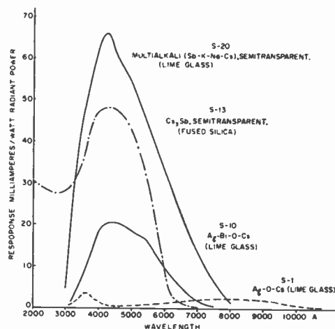
Fig. 15—Spectral response of typical commercial photocathodes. (After R. W. Engstrom, "Absolute spectral response characteristics of photosensitive devices," RCA Rev. , vol. 21, pp. 184–190; June, 1960.)
