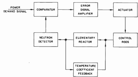
Fig. 4—Reactor control loop with temperature coefficient feedback.
