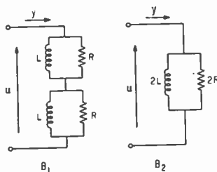
Fig. 2—Equivalent networks.
