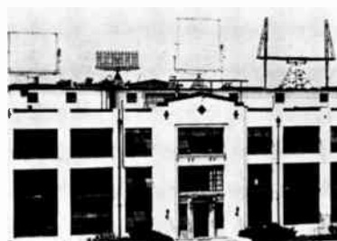
Fig. 9—Penthouse roof, Bldg. 12, showing (right to left), pre-XAF, XAF, 400-mc and CXAM antennas. Pre-XAF is hand driven; all others are motor driven with remote control. Summer, 1940.
