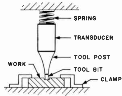
Fig. 6—Ultrasonic drill.
