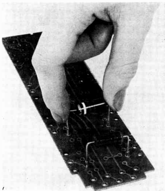
Fig. 15—IBM "Sage" computer board. This board was assembled in 1955 on the General Mills "Autofab" conveyerized automatic assembly machine. Note the wrap-around component tips on the ends of the resistor leads. The board had wiring patterns on both sides and plated-thru holes.
