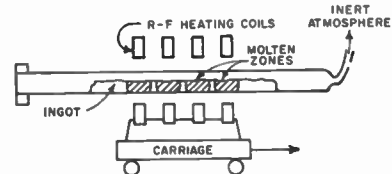
Fig. 5—Cross section of zone refining equipment. The RF heating coils cause melting to occur in the narrow zones. The zones are caused to move from one end of the semiconductor bar to the other by moving the carriage. Segregation at the liquid-solid interfaces causes impurities to move toward the ends of the bar. Several stages of recrystallization can be obtained without handling the material by using several zones and making repeated passes, so an extremely high degree of purification can be achieved.
