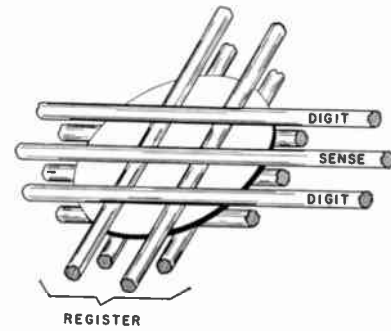
Fig. 8—Single magnetic film memory cell. The film which is supported on a glass substrate is about \frac{1}{4} inch in diameter and 1000 Å thick. For high-speed switching drive lines, simulate transmission lines. [After J. I. Raffel, M.I.T. Lincoln Laboratory, Lexington, Mass., private communication.]
