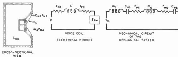
Fig. 7—Cross-sectional view, electrical and mechanical circuits of a direct-radiator dynamic loudspeaker mounted in a completely enclosed cabinet. In the electrical circuit: e = the internal voltage of the generator, r_{EG} = the electrical resistance of the generator, r_{EC} and L = the electrical resistance and the inductance of the voice coil, z_{EM} = the motional electrical impedance. In the mechanical circuit: f_M = the driving force, m_C = the mass of the cone, C_{MS} = the compliance of the suspension system, r_{MS} = mechanical resistance of the suspension system, m_A = the mass of the air load, r_{MA} = the mechanical resistance of the air load, C_{MB} = compliance of the air in the cabinet.
