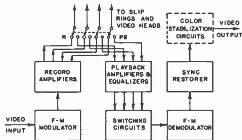
Fig. 8—Block diagram of video record and playback facilities.
