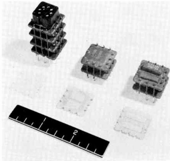
Fig. 2—Mechanize Production of Ceramic Wafer Assemblies
