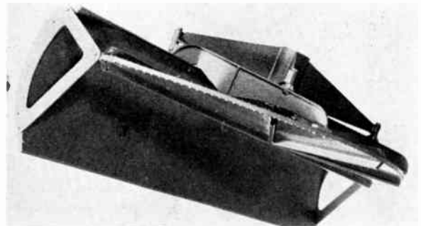
Fig. 4—Pillbox antenna feeding a cylindrical reflector.
