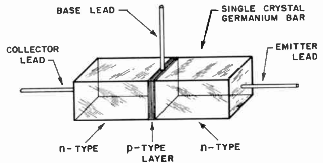
Fig. 3—The structure of an n-p-n germanium grown-junction transistor. Using the equipment of Fig. 2, a single crystal is drawn from an appropriately doped n -type melt (phosphorus or arsenic, typically), aided by a seed crystal, and the collector region is formed. At a suitable time, a p -type impurity such as boron or gallium is added to the melt to dope the base. Subsequently, an additional donor impurity is added to the melt to form the strongly doped n -type emitter. The crystal is then withdrawn, cut into bars, and leads attached. Several hundred transistors are obtained from a single crystal.
