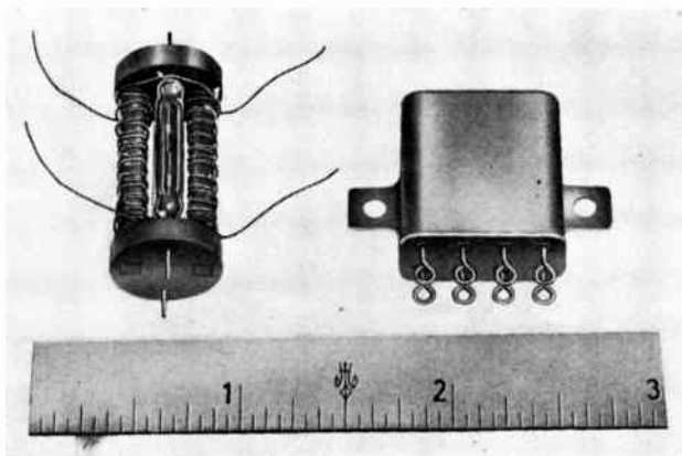
Fig. 3—Modern trends in relays. Left —ferreed with two contacts; right —D1D1T "crystal can" relay.
