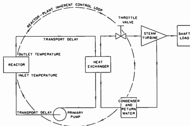
Fig. 5—Block diagram of reactor and associated plant showing inherent control loops.
