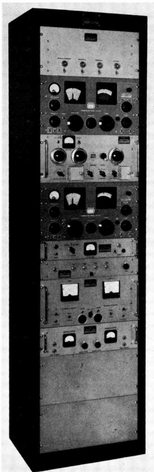
Fig. 8—Dual-diversity FSK Twinplex radio receiving terminal, as used in international point-to-point HF communications, features automatic frequency control and narrow-band Twinplex reception using 200-cps shift intervals. Eight 50-baud channels can be received with a total frequency-shift spread of 600 c through the combination of synchronized time-division multiplex and narrow-band twinplex techniques. (Courtesy of Mackay Radio and Telegraph Company.)
