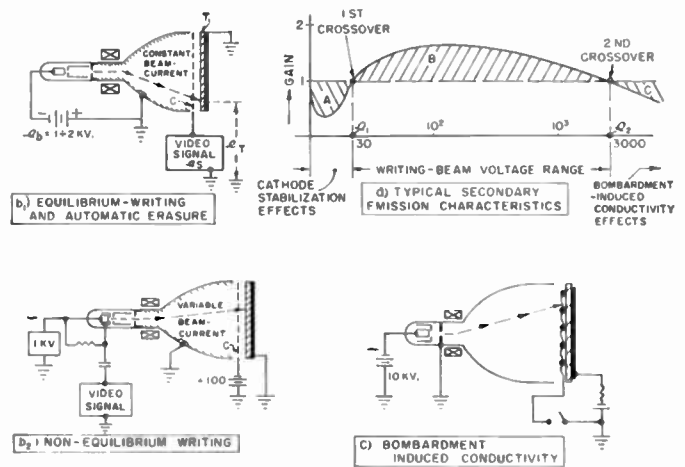
Fig. 9—Storage tube principles.
