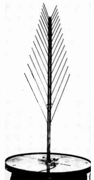
Fig. 9—Log-periodic resonant- V array.
