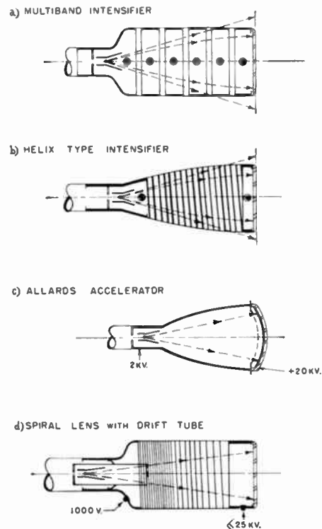
Fig. 6—Beam intensifiers for oscilloscopes.
