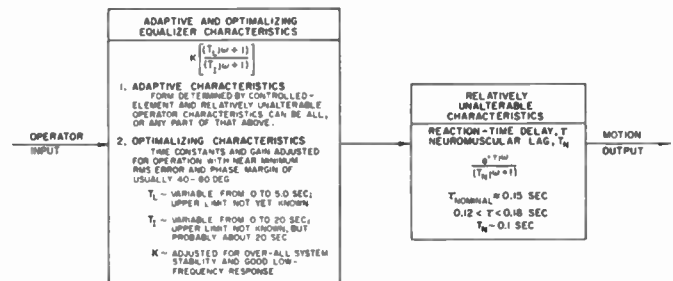
Fig. 4—Condensed version of human operator model for compensatory operation.
