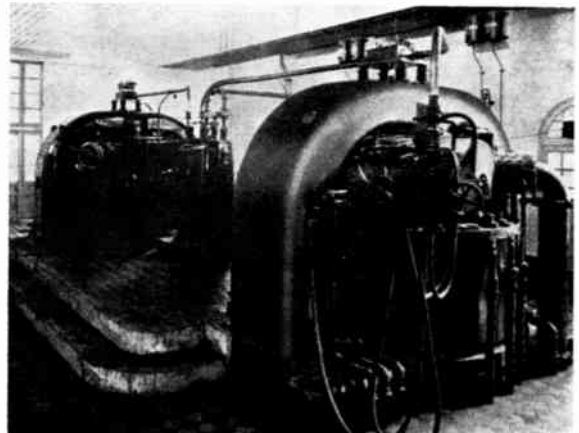
Fig. 2—Historic Lafayette radio transmitter station built by the Federal Telegraph Co. for the U. S. Navy near Bordeaux, France, during World War I. It was the largest transmitter ever built up to that time. (Courtesy of Electrical Communication .)
