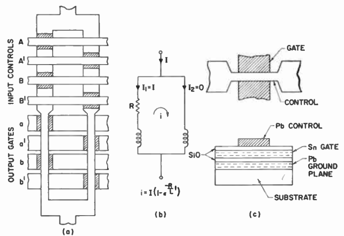
Fig. 1—Thin-film cryotron. (a) Basic cryotron logic circuit. (b) Switching time in terms of R/L time constant. (c) Cross-film cryotron structure.
