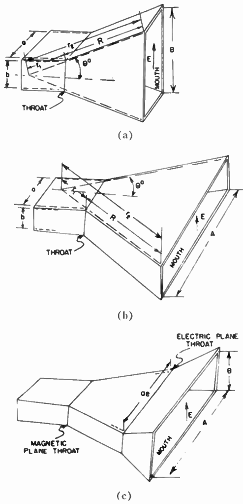
Fig. 1—Horn-feed types. (a) Electric-plane horn. (b) Magnetic-plane horn. (c) Compound horn.
