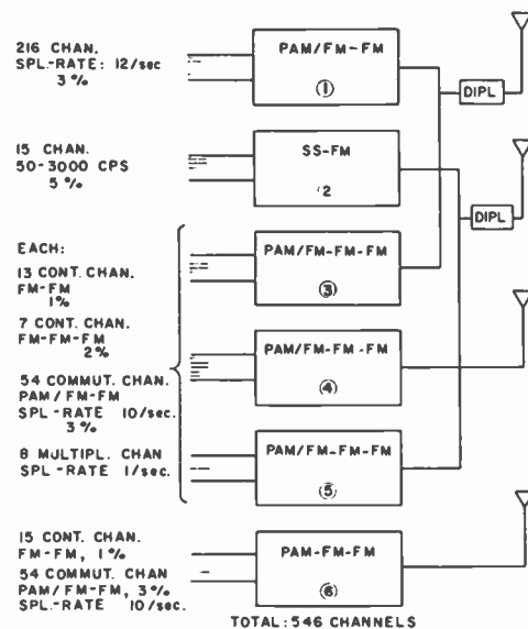
Fig. 6—Schematic diagram of Saturn booster telemetry system 13 (accuracy in per cent).
