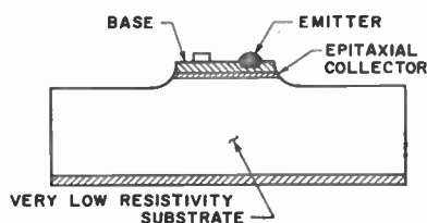
Fig. 12—Cross section of an epitaxial, diffused base, alloyed emitter mesa transistor. Typical fabrication steps for a p - n - p germanium transistor are similar to those described under Fig. 9, with the important difference being that the starting slice is one on which a high-resistivity p region has been epitaxially grown on a low-resistivity p+ slice. The fabrication steps of Fig. 9 then occur in the p region, the p+ region serving mainly as a mechanical support and a low-resistance electrical connection to the collector.
