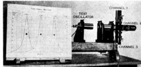
Fig. 7—An early form of three-channel multiplex and its measured frequency characteristic as of 1940.
