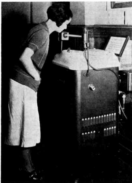
Fig. 4—Photoelectrically controlled drinking fountain (1931).
