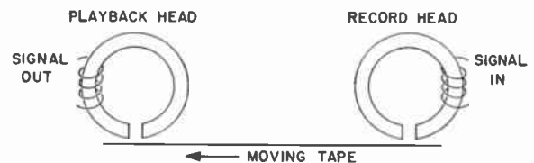
Fig. 3—Schematic representation of a magnetic recording and playback system.
