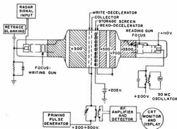
Fig. 11—Recording storage tube (Raytheon).
