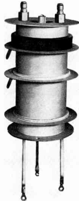
Fig. 5—Ceramic hydrogen thyatron GI-7890. Peak power=48 megawatts at 44 kw; peak current=2400 amperes; body length = 13½ inches; ceramic diameter = 4½ inches.
