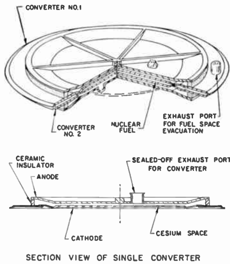
Fig. 3—Sandwich design of a thermionic converter.
