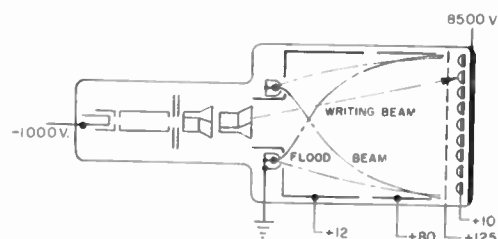
Fig. 12—Iatron storage display tube (ITT Labs.).
