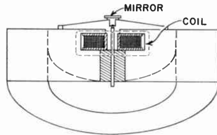
Fig. 5—Magnetic recording galvanometer.
