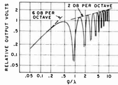
Fig. 3—Output of a long gap head. 2
