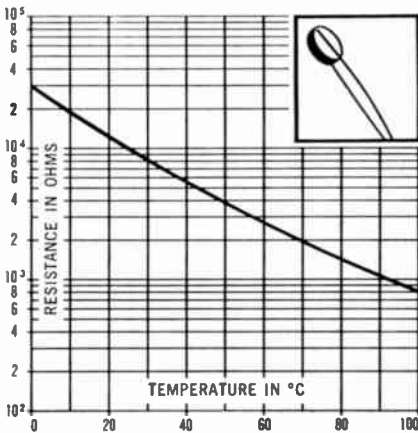
Resistance Temperature Characteristics - Partial Range—YSI #44006 Thermistors (10K).
