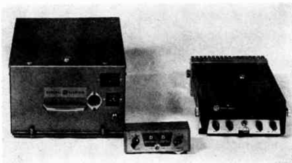
Fig. 4—General Electric Company mobile telephone equipments showing size reduction between 1950 and 1960.
