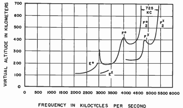
Fig. 1—Typical ionosonde record. Superscripts o and x correspond to the ordinary and extraordinary rays resulting from interaction of the wave with the earth's magnetic field. The sudden changes in height correspond to the critical frequencies of the layers.
