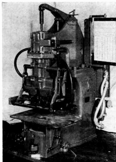
Fig. 16—United Shoe's "Dynasert," an individual component-part machine designed for bench installation. This was in fairly sizable production about 1955.
