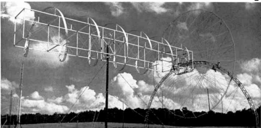
A Portion of a high gain broadband monopole, phased array, designed for electrical steering in azimuth and controlled elevation beamwidth.
