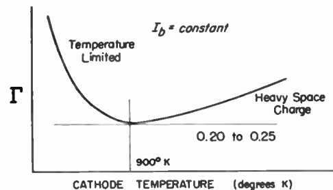
Fig. 3—Typical variation of \Gamma in a space-charge-limited diode with oxide-coated cathode.
