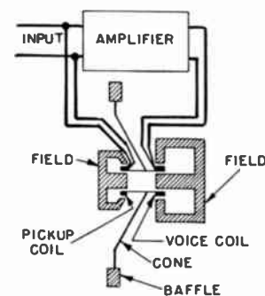
Fig. 15—Loudspeaker, amplifier and pickup-coil feedback system.
