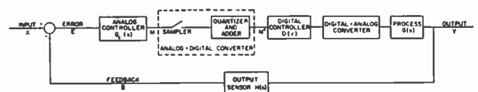
Fig. 3—Simplest computer-controlled feedback system.
