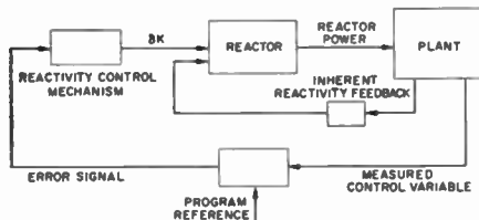
Fig. 10—Control system for a plant which is inherently stable.
