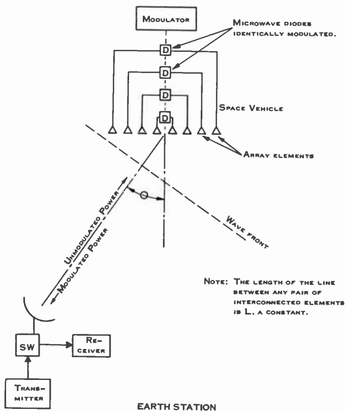
Fig. 8—TELARRAY data-transmission system.
