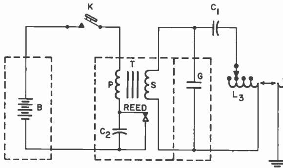
Fig. 1—Transmitter.
