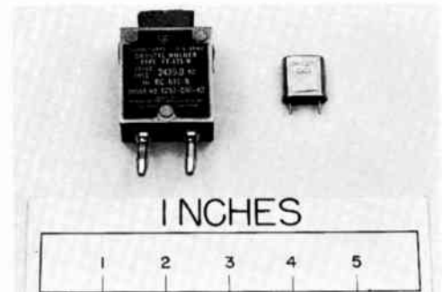
Fig. 2—Typical quartz crystal units of 1940 (left) and 1960 (right).
