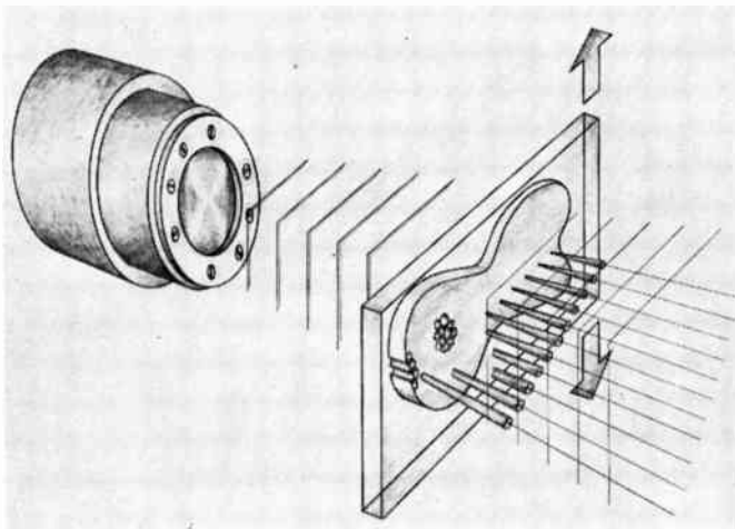
Fig. 3—Principle of operation of an ultrasonic microscope capable of resolving structure on an intracellular level. Plane pulsed waves of sound are generated by a piezoelectric plate element vibrating in thickness mode at any of a series of odd harmonics of the fundamental resonant frequency. After passing through the structure under examination, which is coupled in close proximity to the transducer element by a fluid medium, the acoustic energy passes into a medium imbedding an array of thermocouple junctions immediately adjacent to the specimen. Since differential absorption of the sound occurs in the specimen it is apparent that the temperature distribution defined by the different thermocouple outputs is a manifestation of structure in the specimen. By moving the specimen in its plane and in a direction at right angles to the direction determined by the linear array of junctions it is possible to obtain a two dimensional ultrasonic picture of microstructure of the specimen. The resolution of such a device is dependent on the size of the thermocouple junction, the thermal properties of the couple leads and of the imbedding medium, the ultrasonic pulse duration and intensity and the magnitude of differential absorption characteristic of the microstructural features.
