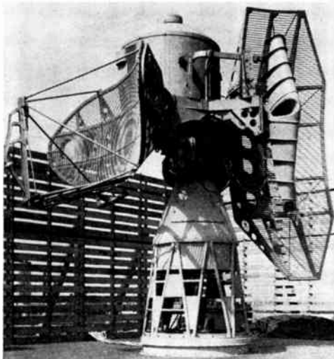
Fig. 7—Shaped-beam antenna (on the left) and Robinson Roll scanning antenna (on the right).
