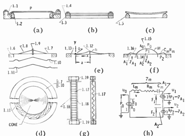
Fig. 1—Various types of diaphragms used in microphones.
