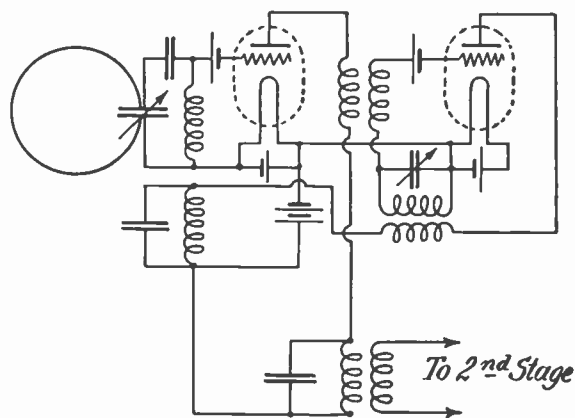
Fig. 3—Basic superheterodyne second harmonic circuit.
