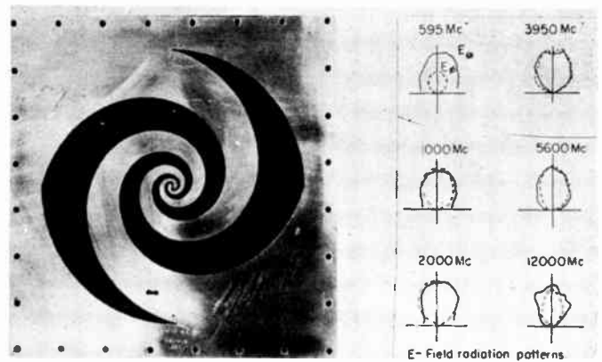
Fig. 7—Planar balanced equiangular spiral slot antenna.
