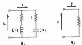
Fig. 3—Ground-state equivalent networks.
