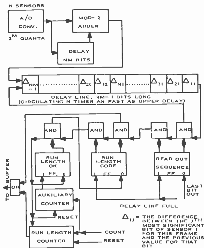
Fig. 2—A compactor for time-multiplexed sensors.
