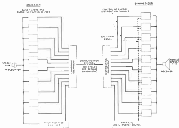
Fig. 8—The transmitting analyzer of the Dudley vocoder ends low-frequency signals over a narrow-band line to instruct the synthesizer on how to reconstruct the speech correctly.
