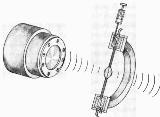
Fig. 2—Method of measuring the ultrasonic absorption coefficients of materials on samples as small as a few cubic millimeters. The material is supported in a tubular shaped container, formed of thin plastic sheet, in which a thermocouple is mounted in approximate coincidence with the long axis. The ultrasound pulses of rectangular envelope are focused in the volume of the medium surrounding the thermocouple junction and the voltage generated across the couple leads indicates the transient change in the temperature of the medium in the immediate neighborhood of the junction. From an analysis of the form of the temperature response, that part caused by absorption of the ultrasound in the body of the medium can be deduced, and from this and a knowledge of the heat capacity of the medium per unit volume and the absolute sound intensity, the acoustic absorption coefficient can be computed.
