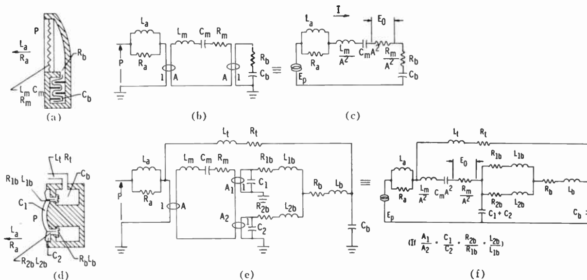
Fig. 4—Pressure microphone with velocity responsive transducer.
