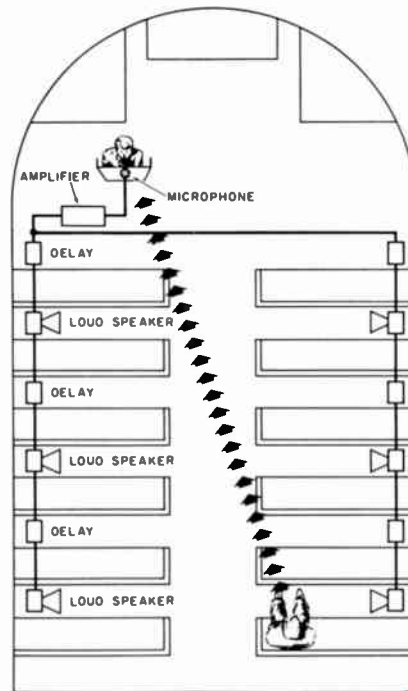
Fig. 4—An auditorium public-address system provides greater realism and intelligibility of delays as required by the Haas effect are introduced in the loudspeaker lines.
