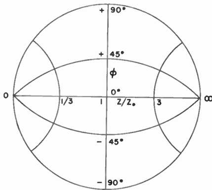
(b) Impedance, Z = |Z| \exp j\phi ; |Z| latitude, \phi longitude. (Carter chart)
