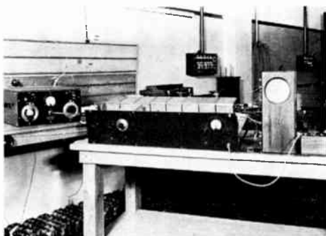
Fig. 4—Original 28-Mc receiver with indicator on test bench showing (left to right) standard signal generator, receiver, indicator, and audio output meter. 1936.
