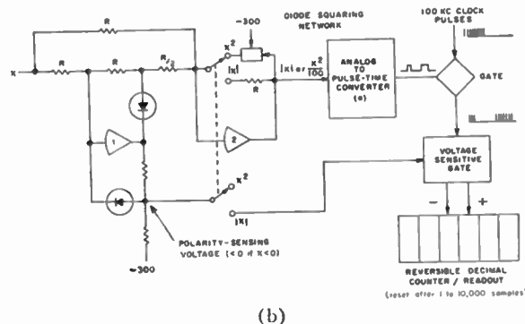
Fig. 11—(a) ASTRAC analog-to-pulse-time converter (b) Hybrid sample-averaging circuit. A precision absolute-value circuit (amplifiers 1 and 2) applies positive voltages |X| or X^2/100 to the converter and, if X is to be averaged, reverses the counter input when X changes sign. The decimal readout counter accumulates readings for between 1 and 10,000 samples of X or X^2/100 . Note that the average of a product XY/100 may be read out through alternate sampling of (X+Y)^2/4 and -(X-Y)^2/4 .
