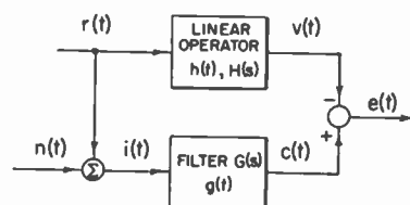
Fig. 6—Block diagram showing criterion for optimum filter.
