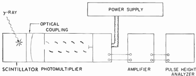
Fig. 1—Scintillation counter.
