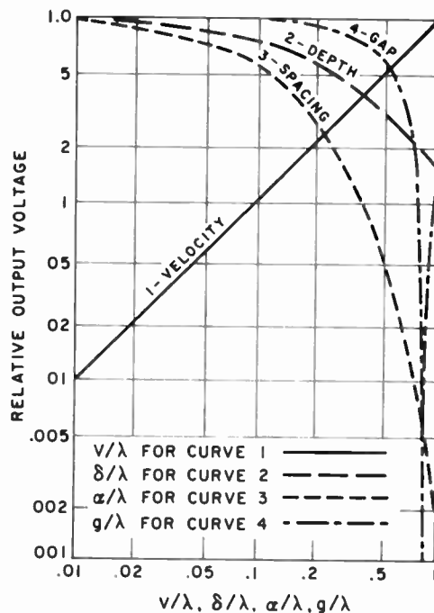
Fig. 4—Effect of tape velocity, thickness, spacing, and gap size on output.
