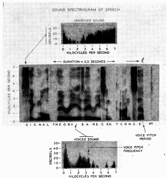
Fig. 3—Sound spectrograms of speech show spectral steady states and transitions which are intimately related to the phonetic content of the utterance.
