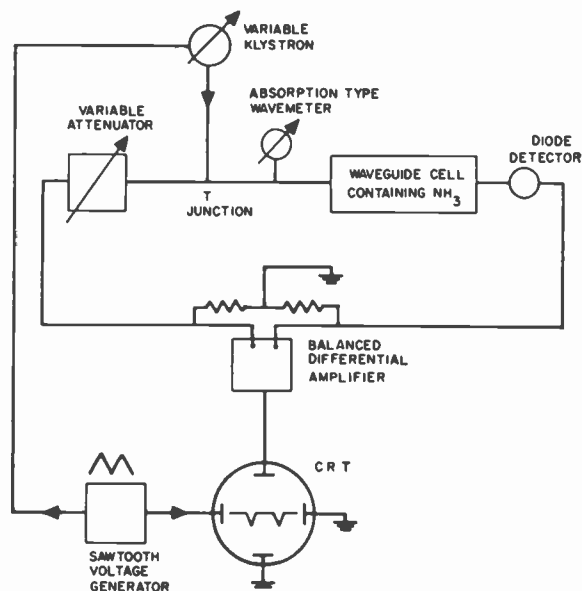
Fig. 1—Simplified block diagram of a microwave spectrometer of the type first used by W. Good.
