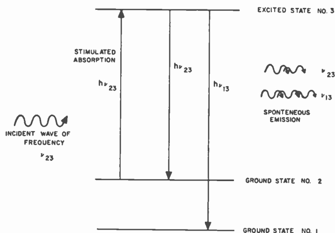
Fig. 3—Simplified optical pumping scheme (not drawn to scale, typically \nu_{13}/\nu_{12} \approx 10^6 ).
