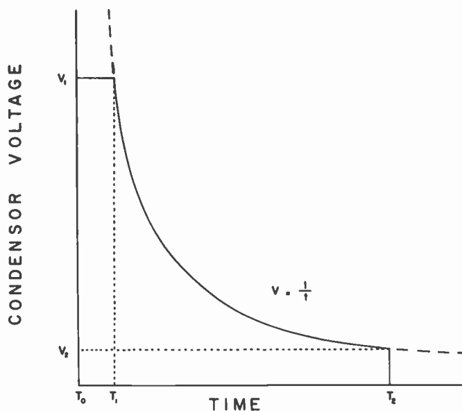
Fig. 6—If the time for one cycle of an event is T_2 and condenser discharge starts at T_1 from V_1 , through a square-law device, then frequency indication is linearly proportional to the final condenser voltage V_2 . The period T_0 to T_1 can be used for readout and resetting from the previous cycle.
