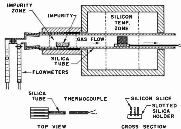
Fig. 8—Two-zone open-tube diffusion apparatus for silicon. The impurity zone temperature can be maintained independent of the silicon temperature to control the surface concentrations. An inert gas flow transfers the impurity to the silicon slices. Generally, the impurity sources are compounds—for example, P_2O_5 and BBr_3 . A chemical reaction occurs on the silicon surface resulting in the phosphorus or boron being deposited on the silicon. Diffusion then occurs into the silicon. Other diffusion techniques include the closed tube, and the semi-closed tube (box) systems.
