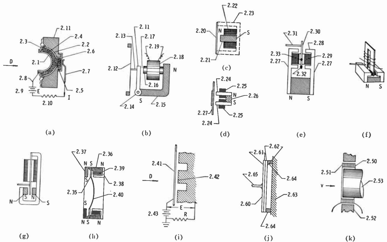
Fig. 2—Various types of transducers used in microphones.
