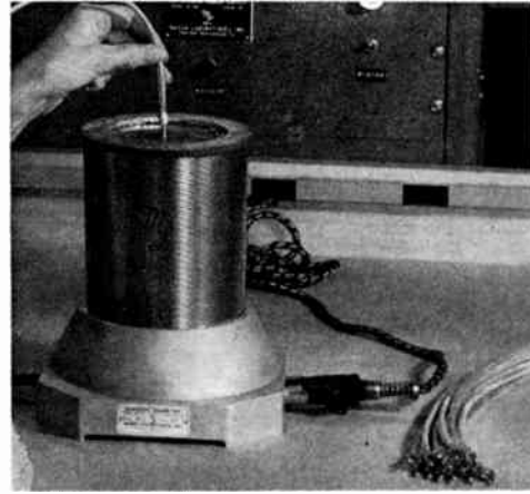
Fig. 11—Ultrasonic solder pot.
