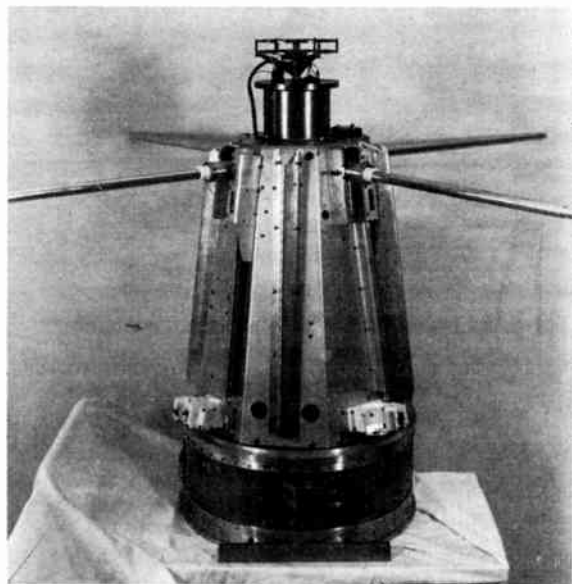
Fig. 2—P-21 Electron Density Profile Probe for upper ionospheric research.
