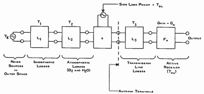
Fig. 5—Noise sources in a receiving antenna (after [12]).
