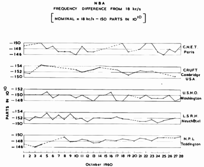
Fig. 9—The values of the frequency of the carrier wave of the station NBA as measured at a number of laboratories.
