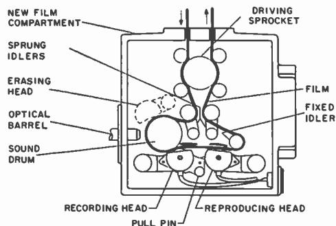
Fig. 11—RCA optical-magnetic recorder.
