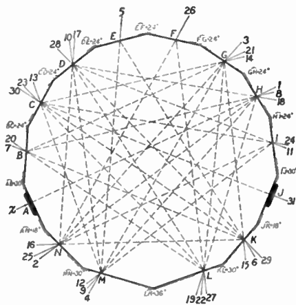
Fig. 5—Polygon shaped fused silica delay lines. Dashed lines show direction of wave propagation. Outside lines indicate damping regions to reduce spurious pulses (after Arenberg).
