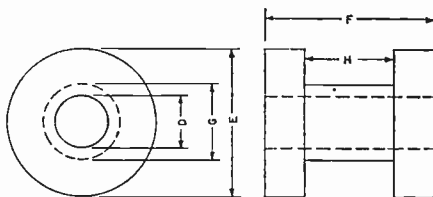
Dimensions of a bobbin.
