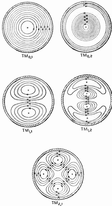
The H lines for the more elementary TM modes of transmission in circular Waveguides . The resonant wavelengths of cylindrical cavities are given by
