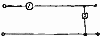
I network. The free ends are the left-hand terminal pair, and the junction point and one free end are the right-hand terminal pair.
