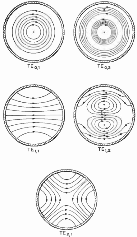
The E lines for some of the more elementary TE modes in circular Waveguides .
