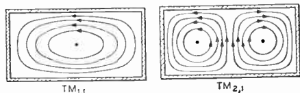
The H lines for the more elementary TM modes of transmission in rectangular Waveguides . The resonant wavelengths of cylindrical cavities are given by
