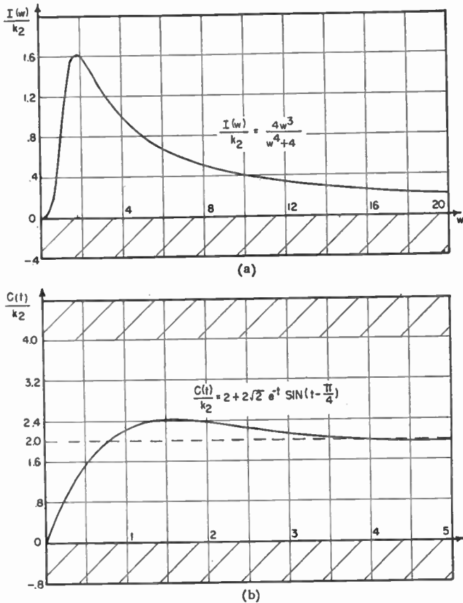
Fig. 5—Prohibited regions of Theorem 5. (a) The region from which I(\omega) is excluded by the hypothesis of Theorem 5. (b) The regions into which the corresponding C(t) cannot enter.
