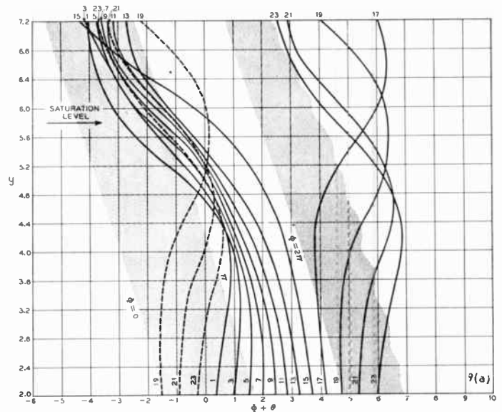
Fig. 9(a)— y versus (\Phi + \theta) curves for case (2).
