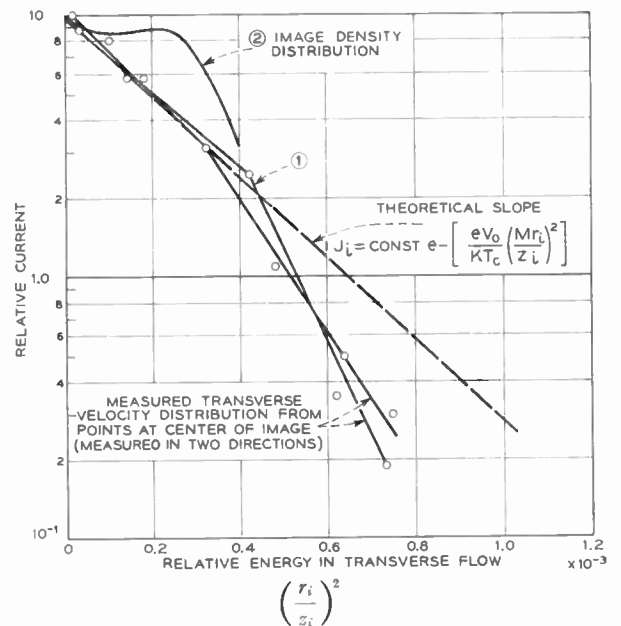
Fig. 5—Transverse velocity distribution. In Curve 1 is plotted the current arriving at the center of the image as a function of the aperture position (measured by laminar electron displacement in the image). Curve 2 is the distribution of image current density, and the dashed curve is the theoretical Maxwellian distribution which is predicted for either measurement for an ideal gun. Curve 2 reveals strong aberrations in the gun.
