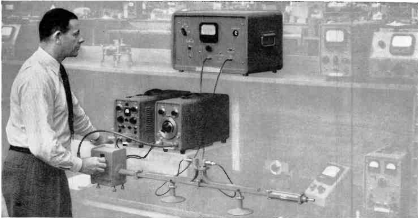
New -hp- reflectometer system comprises Klystron Power Supply, Swept Frequency Oscillator and Ratio Meter (rear) plus Variable Attenuator, Directional Couplers, Waveguide Crystal Detectors and Load (simulated by Shart).
