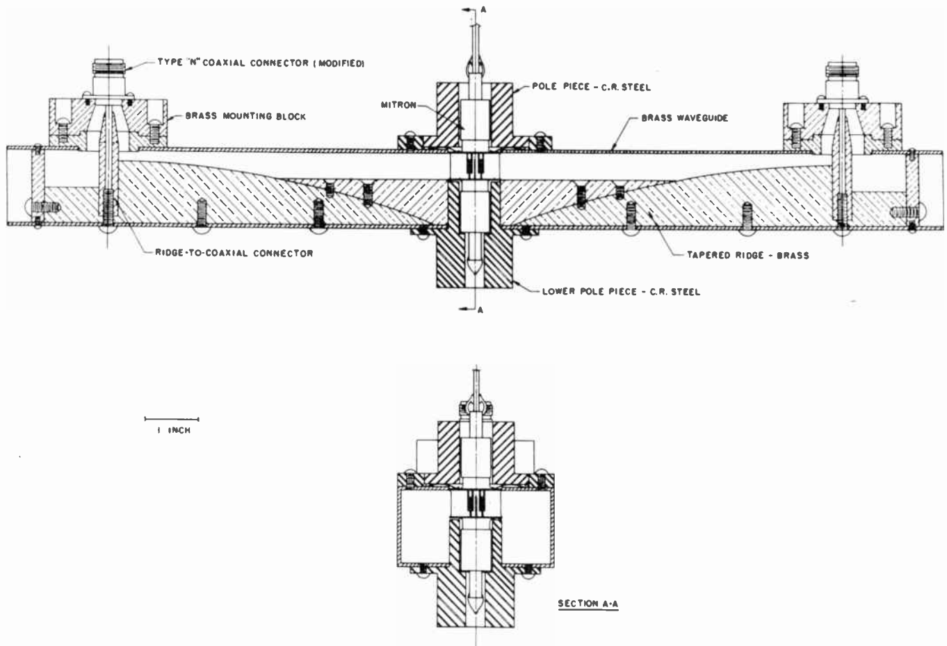
Fig. 1—Dual output cavity for mitron.
