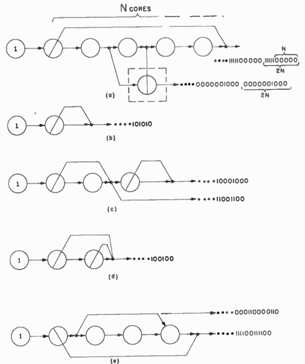
Fig. 6—Pattern generators.
