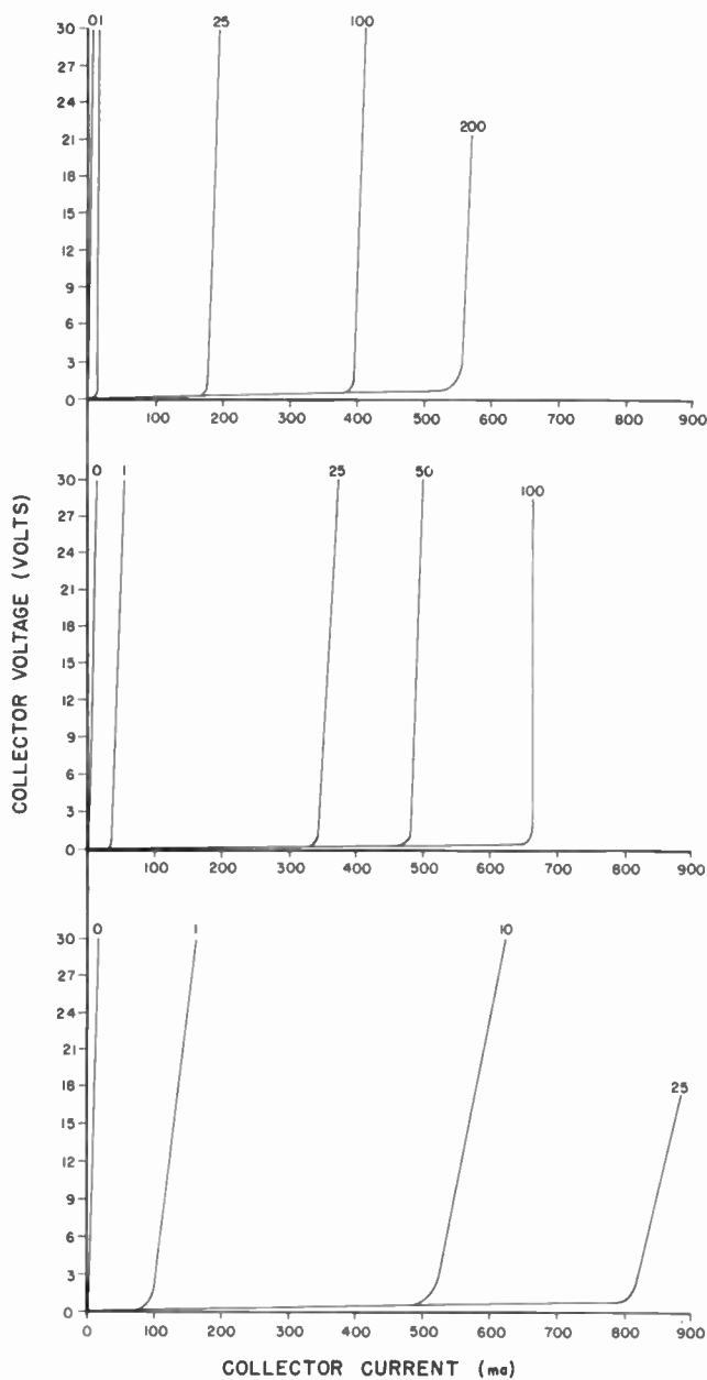
Fig. 2—Common-emitter characteristic curves of three representative power transistors.
