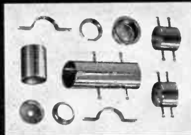
New Developmental \frac{3}{8} " Diameter Parts for "small neck" TV picture tubes
