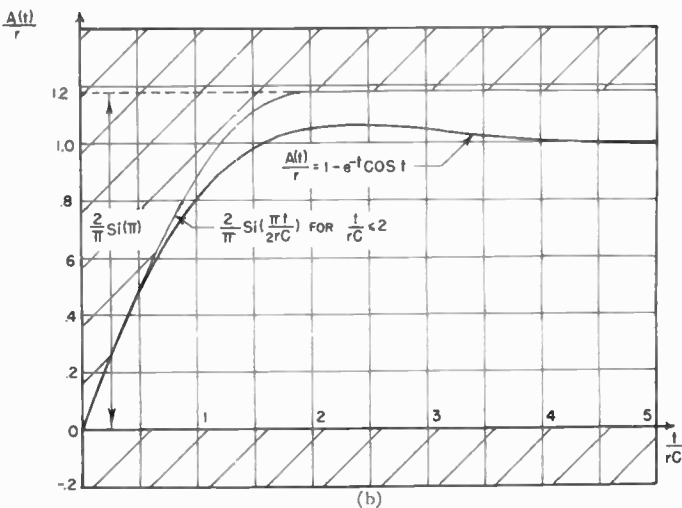
Fig. 1—Prohibited regions of Theorem 1 for the case K=0 . (a) The region from which dR/d\omega is excluded by the hypothesis of Theorem 1. (b) The regions into which the corresponding A(t) cannot enter.
