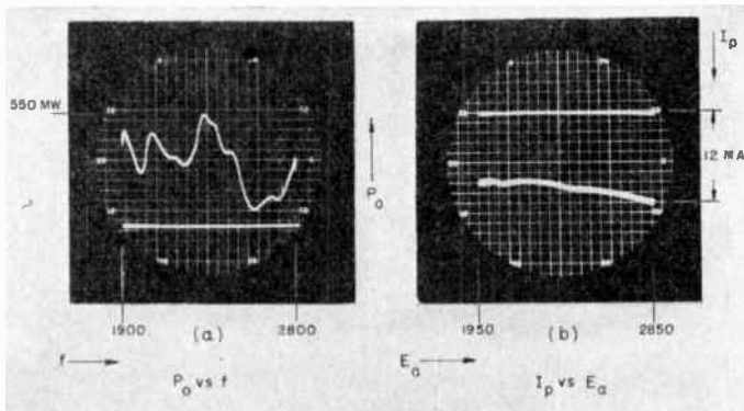
Fig. 4—Power and current characteristics. B = 4,510 gauss E_{dc} = 2,400 volts E_{ac} = 900 volts peak-to-peak I_p \approx 12 ma.
