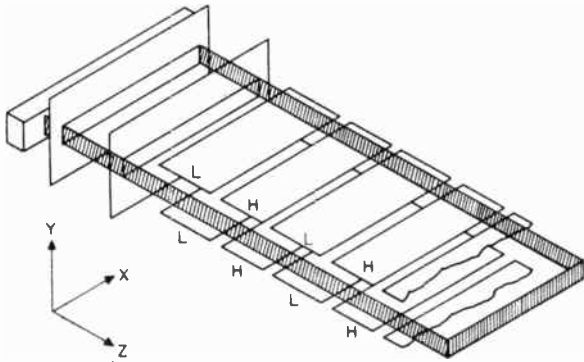
Fig. 1—Electrostatically focused ribbon-beam tube: beam from elongated cathode passes through collimating slots into space bounded by electrode pairs which are held at alternately high and low potentials.
