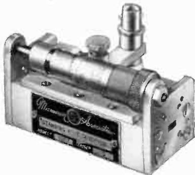
STANDING WAVE DETECTOR #1022
