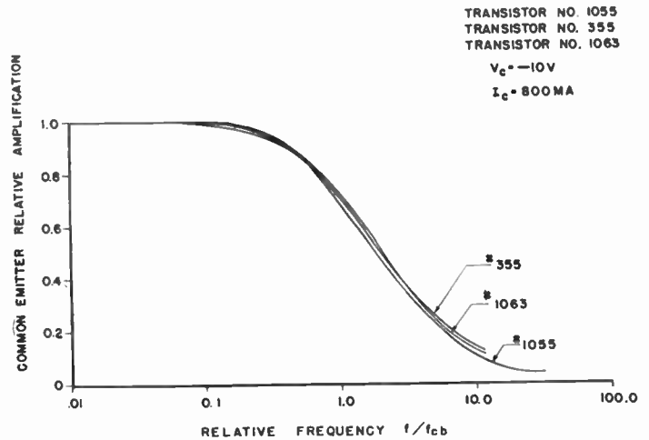
Fig. 10—Common-emitter relative frequency vs relative amplification.
