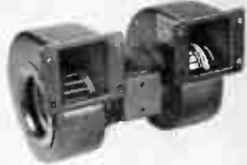
A15AD3—Axial blower unit for operation on 115 Volt 60 cycle single phase supply at 3300 RPM delivering 35 CFM at 0.2 S.P. This unit has special mounting bracket.
