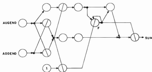
Fig. 16—Two-input adder.
