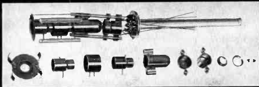
GUN ASSEMBLY FOR ELECTRO-STATIC TYPE TV PICTURE TUBES.
