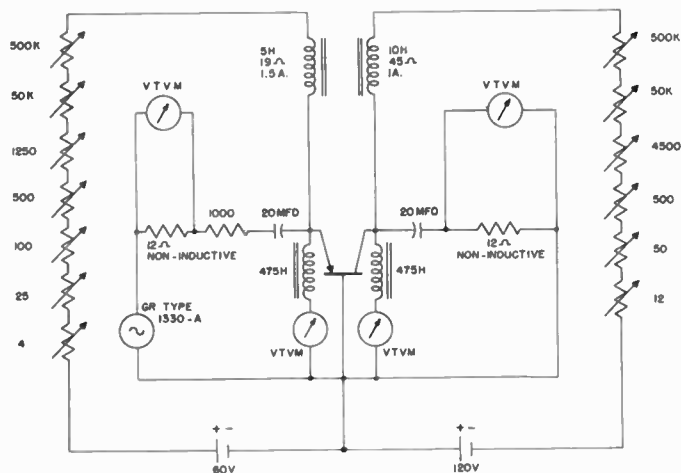
Fig. 3—Circuit diagram of current-amplification measuring apparatus.
