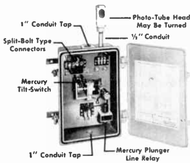
Model LC 2074 Tower Lighting Control Unit
