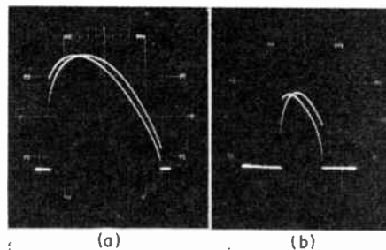
Fig. 3—Oscilloscope photographs of power vs beam voltage (sinusoidal sweep) for two-cavity klystron oscillator. (The two traces are displaced slightly in phase to show the hysteresis breaks.) (a) Moderate load. (b) Heavy load (large load conductance).
