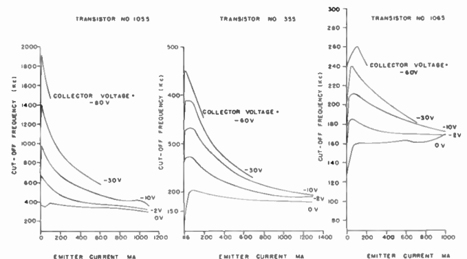
Fig. 6—Common-base cutoff frequency as a function of emitter current and collector voltage.
