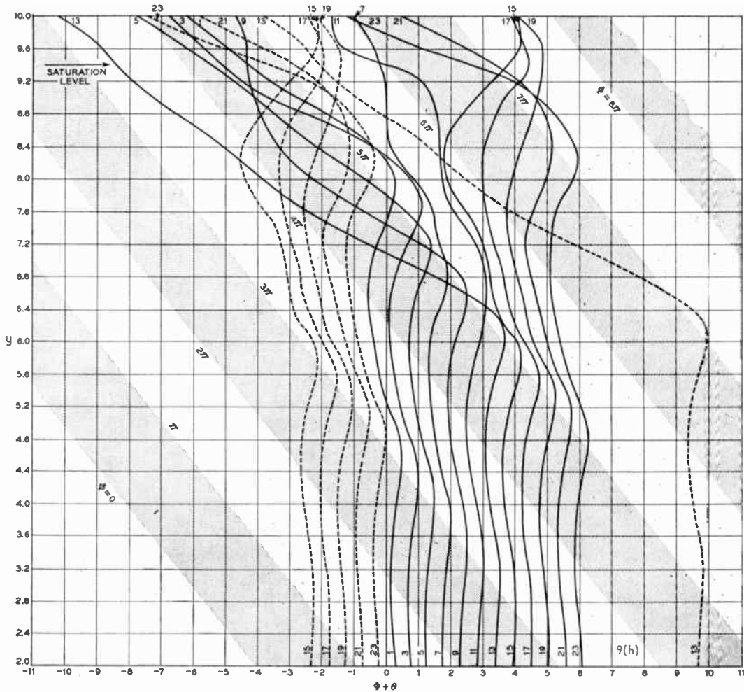
Fig. 9(h)—y versus (\Phi + \theta) curves for case (17).
