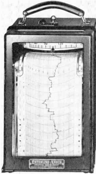
TYPICAL EXAMPLE OF SOLA VOLTAGE REGULATING ACTION. The recording on the left represents a fairly common condition of voltage fluctuation on a 115v line. The chart on the right
