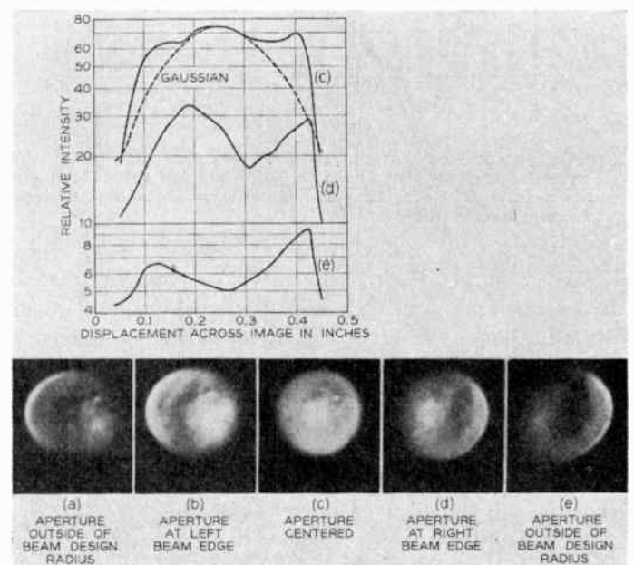
Fig. 3—Fluorescent screen images obtained from gun No. 1 in a pin-hole camera tube. The curves give the measured illumination of the corresponding image. Compare this with Fig. 7.
