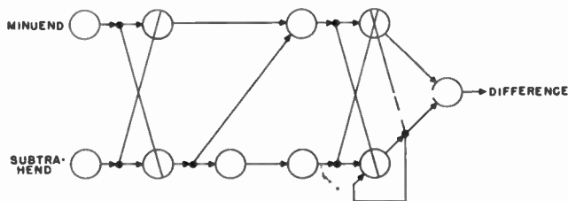
Fig. 15—Two-input subtracter.
