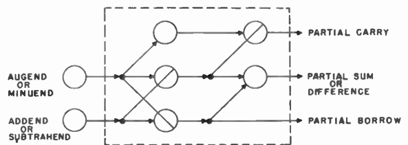
Fig. 10—Half-adder-subtractor.
