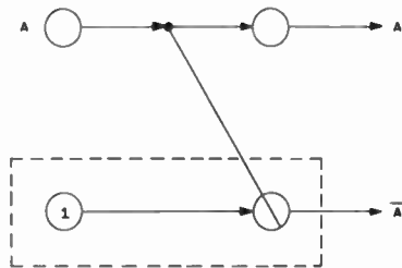
Fig. 7—Complementing circuit.
