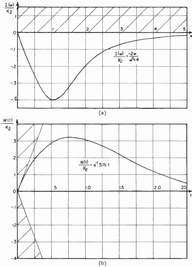
Fig. 3—Prohibited regions of Theorem 3. (a) The region from which I(\omega) is excluded by the hypothesis of Theorem 3. (b) The regions into which the corresponding W(t) cannot enter.
