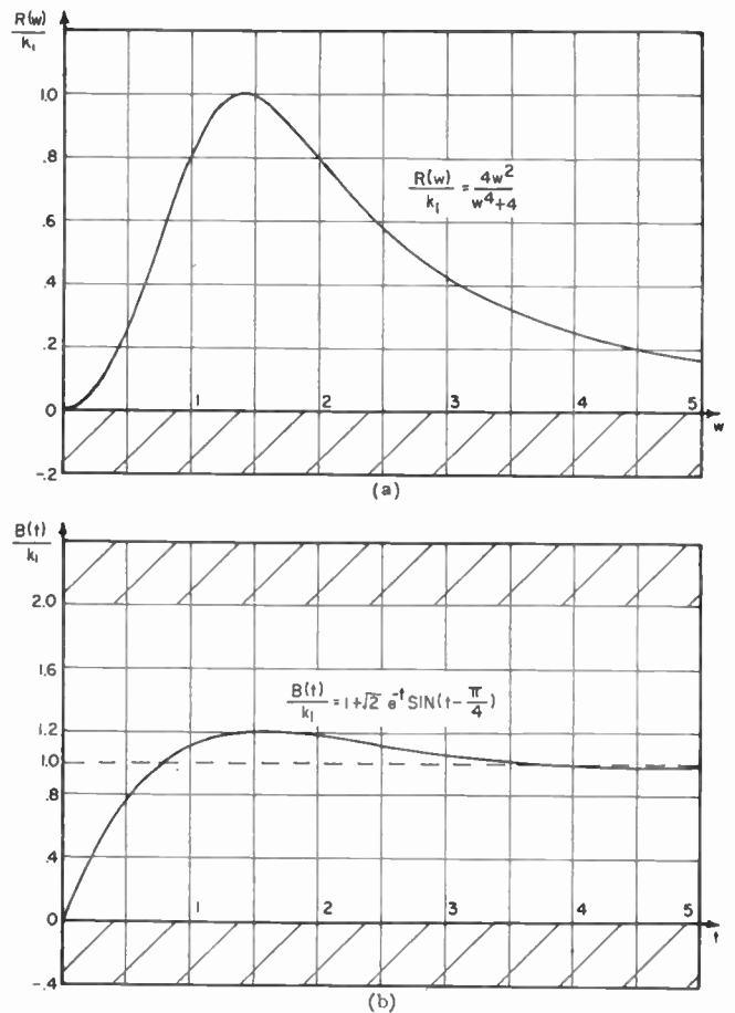
Fig. 4—Prohibited regions of Theorem 4. (a) The region from which R(\omega) is excluded by the hypothesis of Theorem 4. (b) The regions into which the corresponding B(t) cannot enter.
