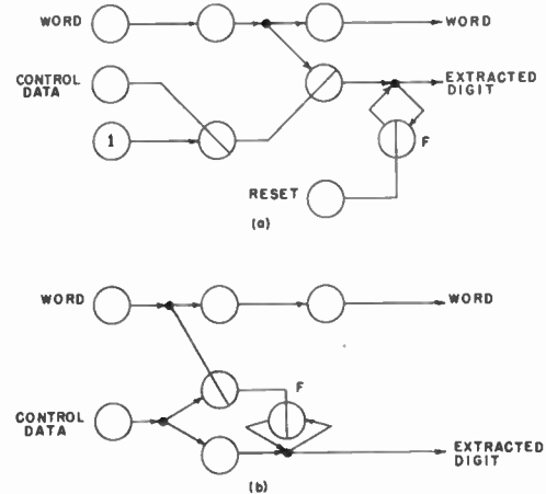
Fig. 13—Extracting and storing.
