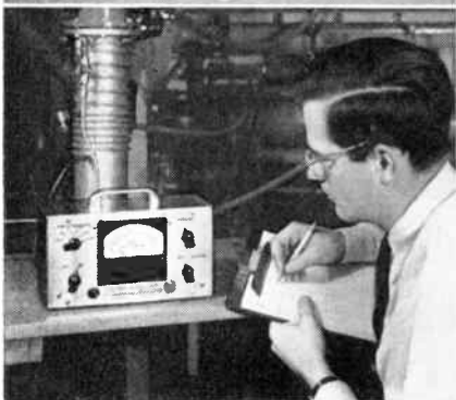
The AC-operated Model 517, newest of the Alphanon® Vacuum Gauges, with 6 ranges covering pressures from 1000 to .0001 mm. Hg. Price: $425.
