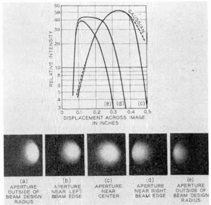
Fig. 7—Photographs of images from a gun having the same electrical design as gun No. 1, but using the negative beam-forming electrode design of Fig. 6(c). These pictures reveal no significant departure from the ideal.
