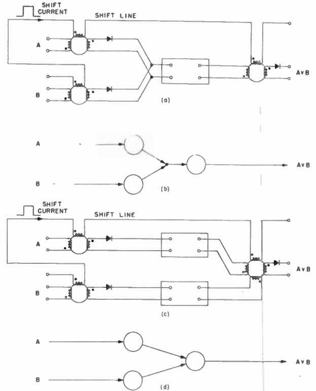
Fig. 3—Mixing or buffer circuits.
