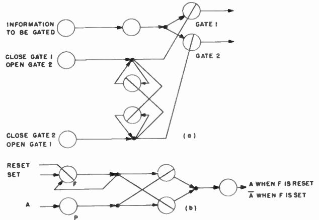
Fig. 12—Gating.
