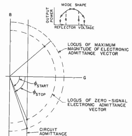
Fig. 4—Admittance diagram of klystron oscillator, with admittance first increasing with rf voltage and then decreasing.
