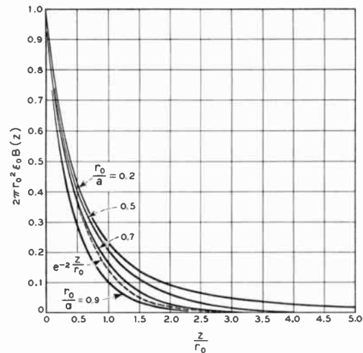
Fig. 1—The solid curves show 2\pi r_0^2 \epsilon_0 B(z) versus z/r_0 , calculated for the force between two electron-discs inside a conducting cylinder, and the dotted curve indicates that computed from the universal function e^{-2z/r_0} .
