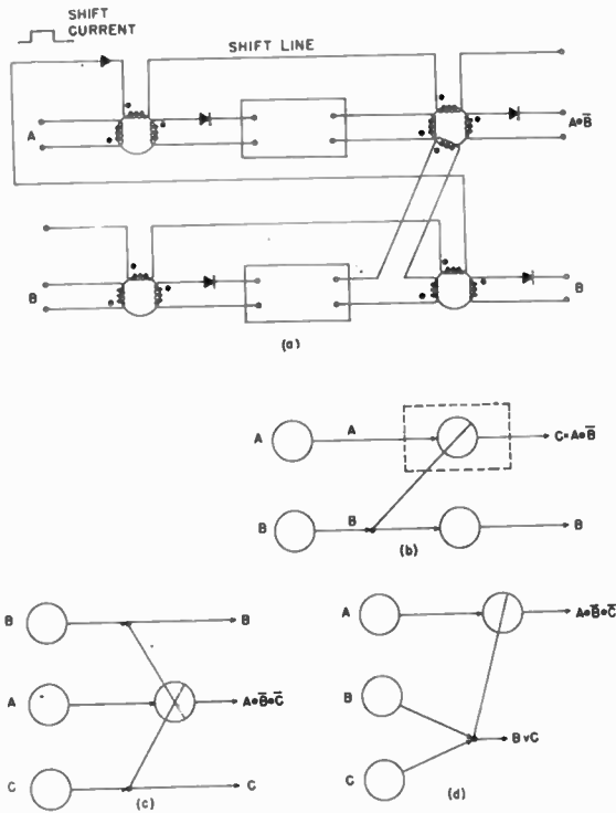
Fig. 4—Inhibit circuits.
