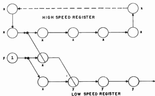
Fig. 14—Information transfer in arbitrary order from higher-to-lower-speed register.
