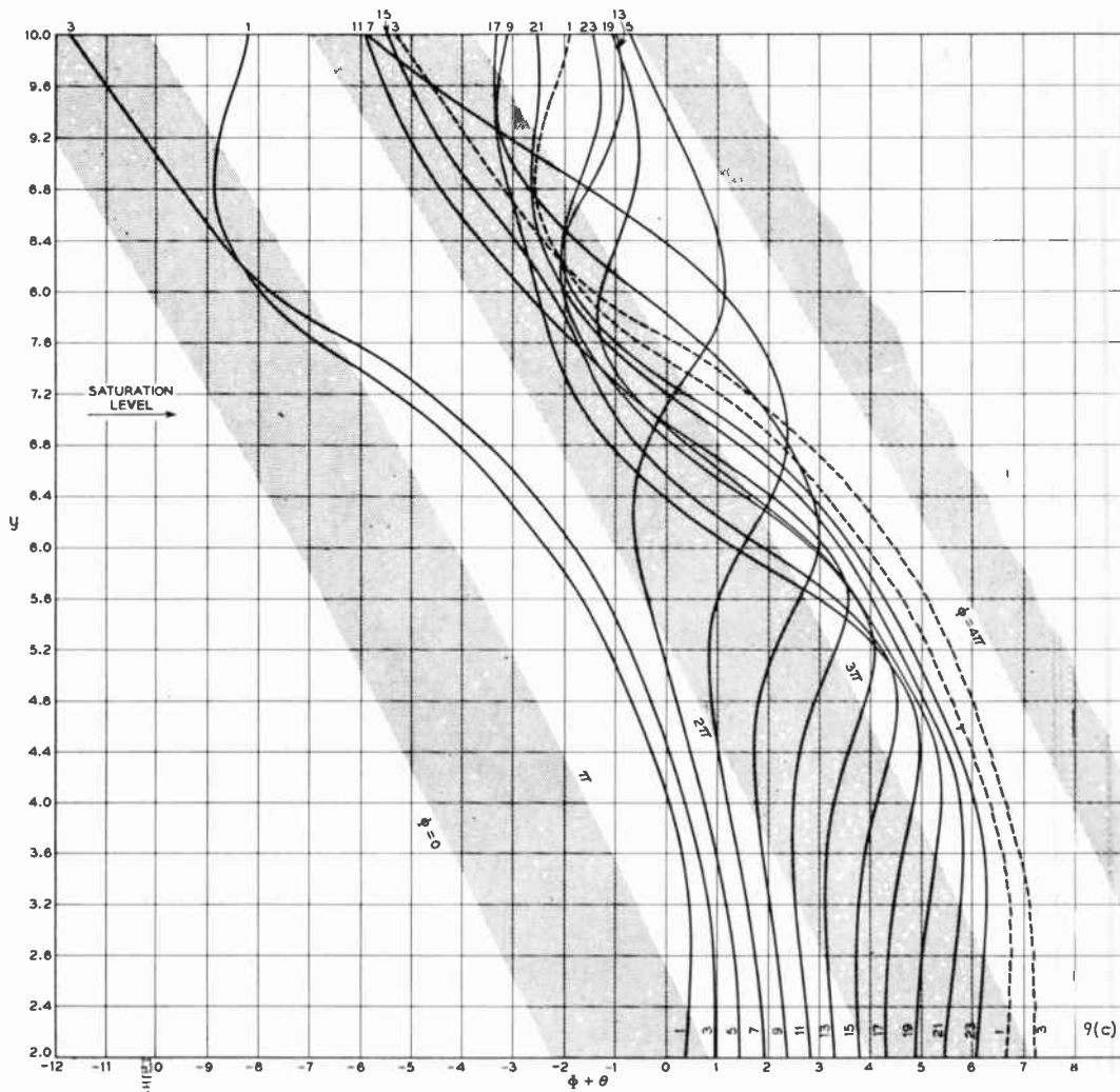
Fig. 9(c)— y versus (\Phi + \theta) curves for case (8).
