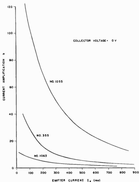
Fig. 5—Emitter current vs current amplification for common-emitter operation.
