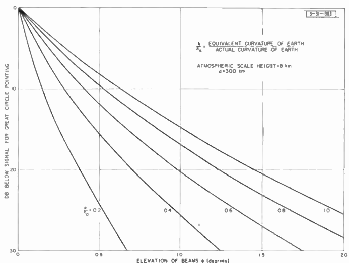
Fig. 7—Decrease in field due to elevating T and R beams equal angles, for several effective earth's curvatures. Indefinitely narrow beams are assumed, and a correction is required for beams of finite width (see Fig. 12).
