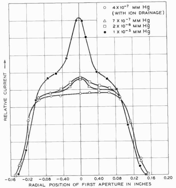
Fig. 12—Current-density distribution from gun No. 2 at various gas pressures, showing the effect of space-charge neutralization by positive ions.
