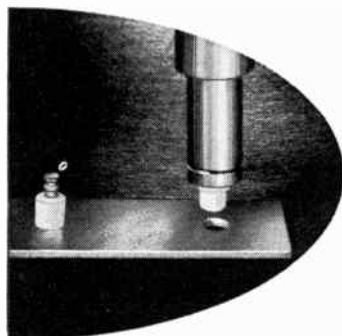
"Press-Fit" Teflon terminals press-fit into chassis holes by means of inexpensive insertion tool. Teflon seals terminal firmly and permanently in place.
