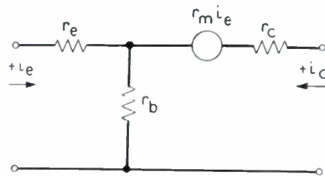
Fig. 3—Equivalent circuit representation of the transistor.
