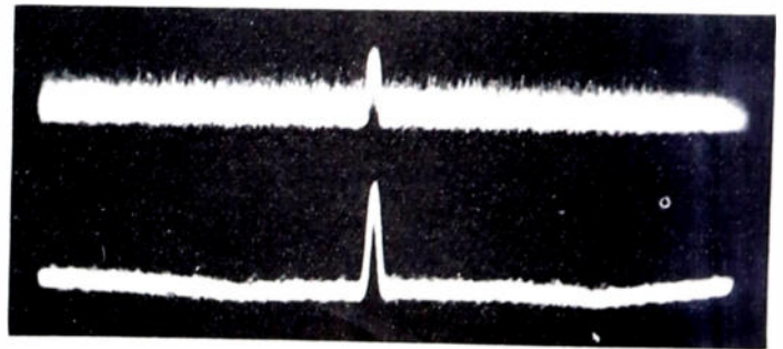
Fig. 7—Pictures of actual signal-to-noise improvement for a 1-microsecond pulse, \gamma=0.1 and n=9 additions.
