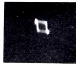
Fig. 13—Photograph of ultradynamic Lissajous figure of distorted wave involving the third harmonic.
