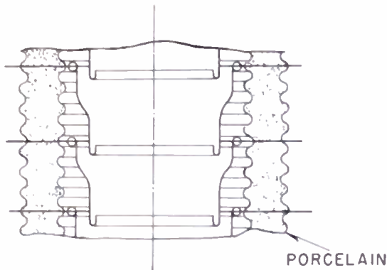
Fig. 3—Re-entrant tube design.
