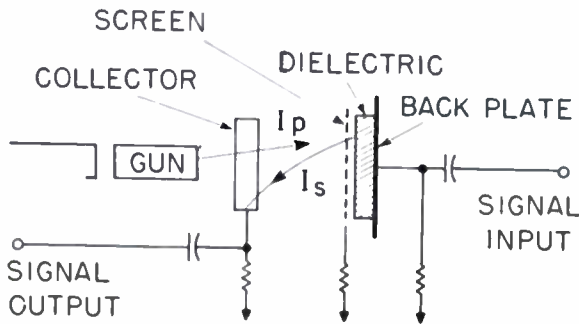
Fig. 2—Simplified schematic of barrier-grid storage tube.
