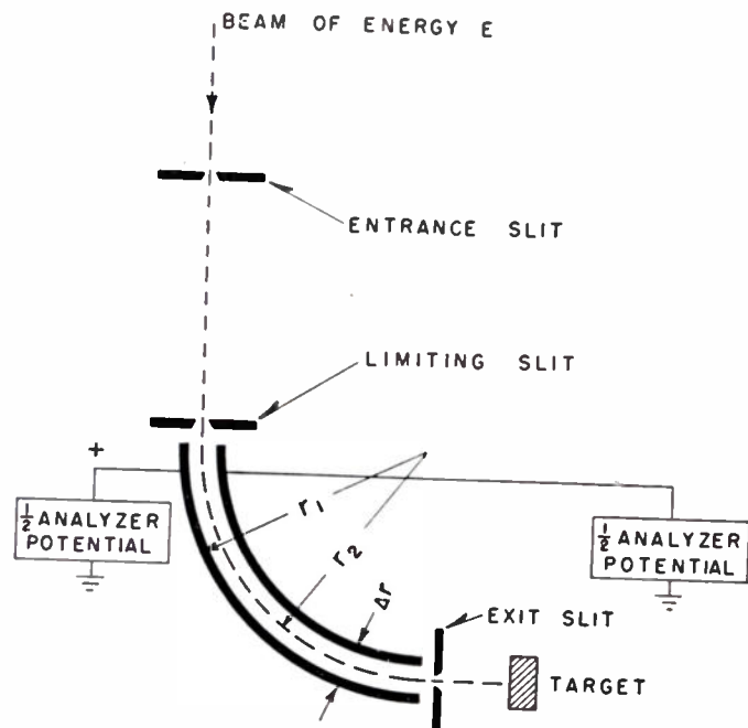
Fig. 10—A curved plate electrostatic analyzer.
