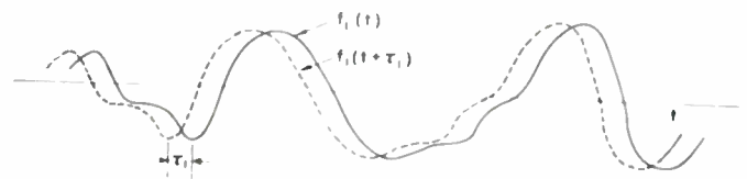
Fig. 2—Graphical method of obtaining an autocorrelation function. Integrate the product over a long duration; and (4) to take the average value of the integral over the duration thus obtaining the points \phi_{11}(\tau_1) on the autocorrelation curve as illustrated in Fig. 3. Repetition of this procedure for
