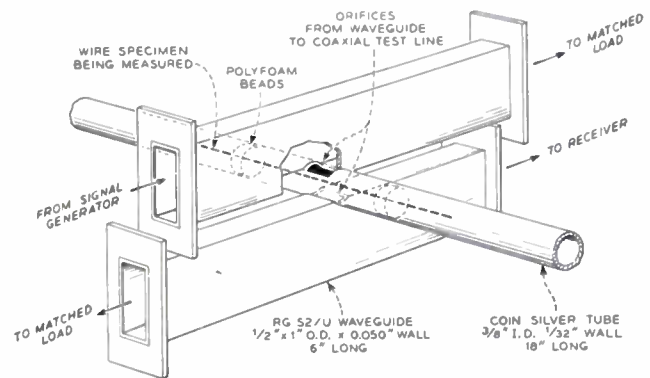
Fig. 1—Specimen holder for wire conductivity measurements.
