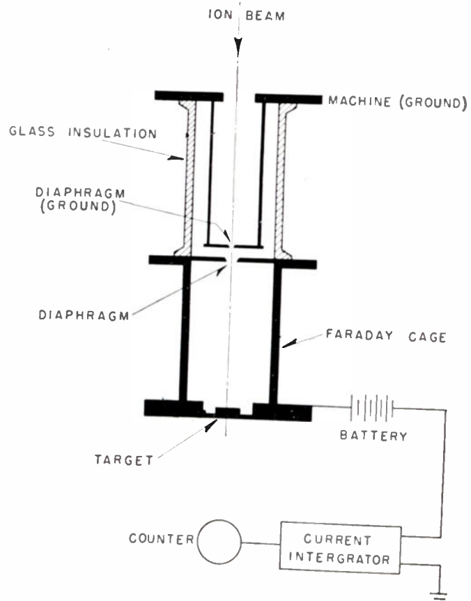
Fig. 8—A beam current collection and measurement.
