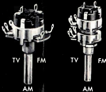
New Centralab Model 2 Radiohm Controls. At left single unit switch type, tapped with single shaft. Right — twin unit switch type, untapped with single shaft.
