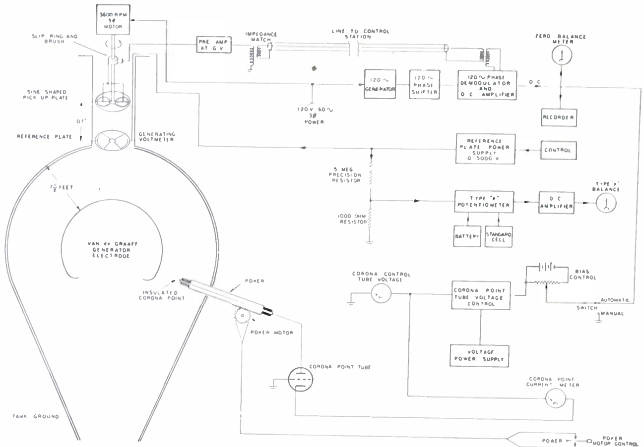
Fig. 13—A Westinghouse Van de Graaff generator generating voltmeter comparison and control circuits.
