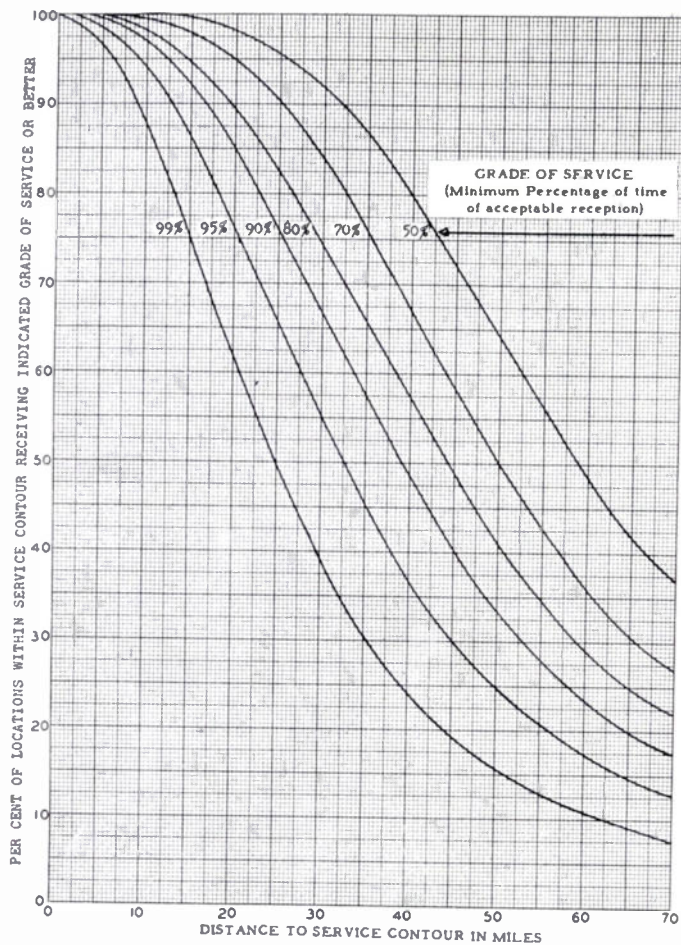
Fig. 3—Cochannel interference. Distance to service contour along radial between desired station and interfering station versus percentage of locations within service contour for various minimum grades of service. Frequency, 82 Mc; transmitting antenna heights, 500 feet; receiving antenna heights, 30 feet; equal power for both stations; station spacing, 150 miles; interference ratio, 40 db; type of area, rural.
