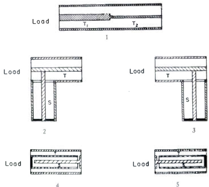
Fig. 1—Two element frequency-compensating matching sections.
