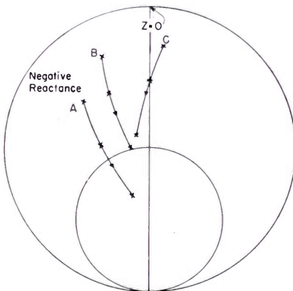
Fig. 4—Transformation of initial curve A to real axis. (Frequency increases in direction of arrow.)
