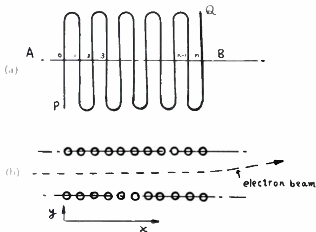
Fig. 2—Diagrammatic illustration of deflecting system. (a) View of the folded parallel transmission lines from above. (b) Side view.
