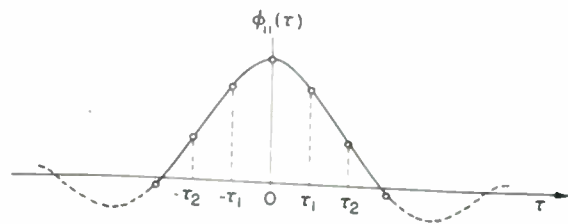
Fig. 3—Autocorrelation function obtained by graphical method.
