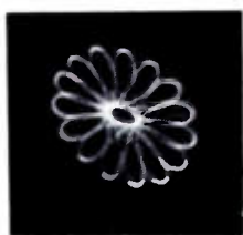
Fig. 15—Lissajous figure involving fractional harmonic.
