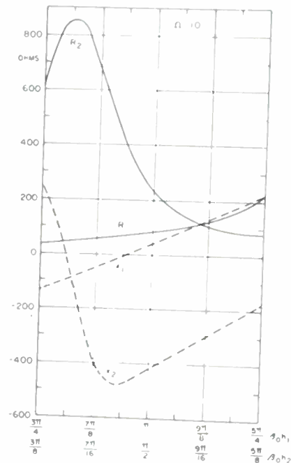
Fig. 12 Impedance behavior of the symmetrical center-driven antenna.
