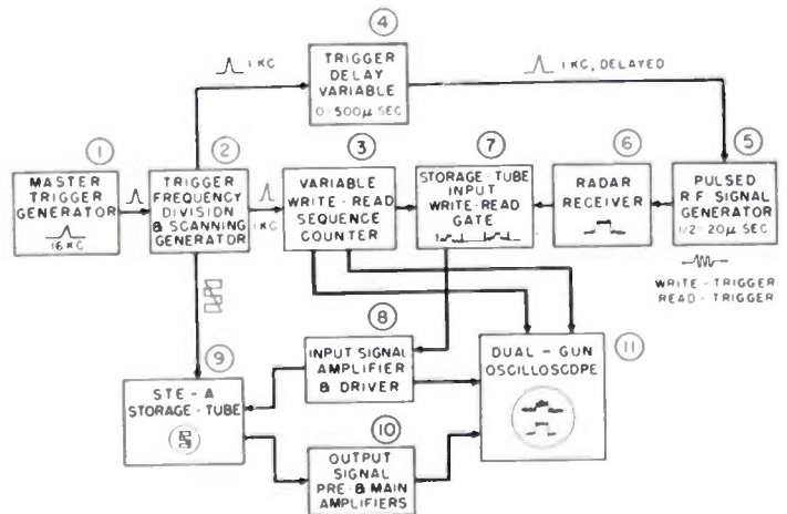
Fig. 5—Block diagram of storage-tube-integrator experimental equipment arrangement.
