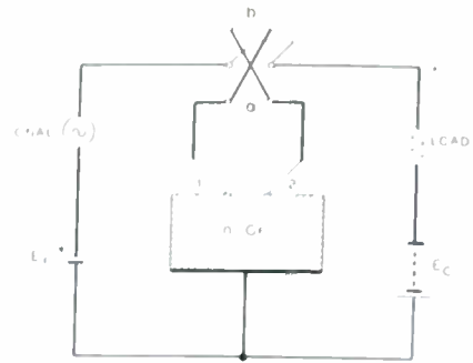
Fig. 1.—Circuit demonstrating reversible properties of an n germanium transistor amplifier. When switch is in position a , electrode 1 is emitter, 2 is collector. When switch is in position b , 2 is emitter, 1 is collector.
