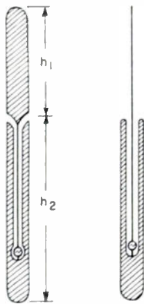
Fig. 2—Asymmetrical antenna internally driven.
