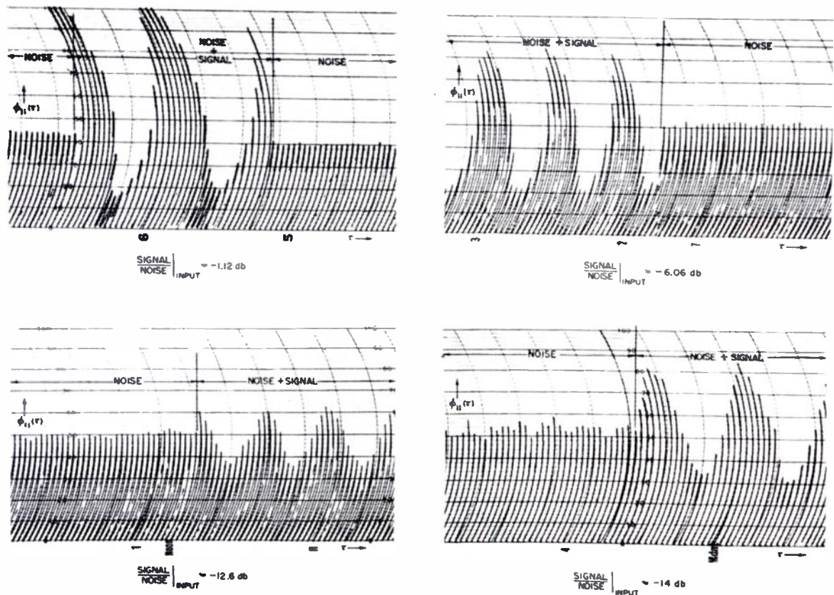
Fig. 10—Experimental results from electronic correlator showing gain in output signal-to-noise ratio for input of sinusoid plus random noise at several ratios.
