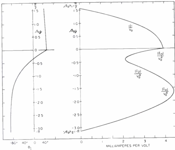
Fig. 5—Current distribution on asymmetrical antenna.
