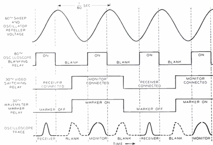
Fig. 6—Wave-form timing and phasing diagram.
