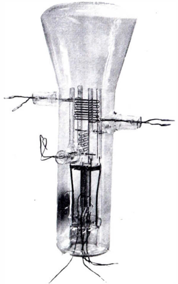
Fig. 1—Construction of the traveling-wave cathode-ray tube.
