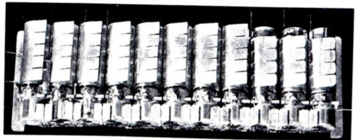
Fig. 5—Front view of the complete assembly of the printed, miniature intermediate-frequency amplifier, Model PC-IV.
