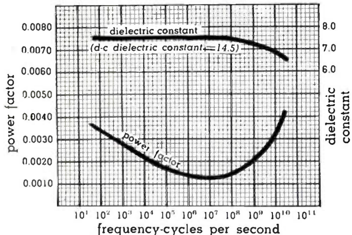
Mycalex 400 - variation of power factor and dielectric constant with frequency
