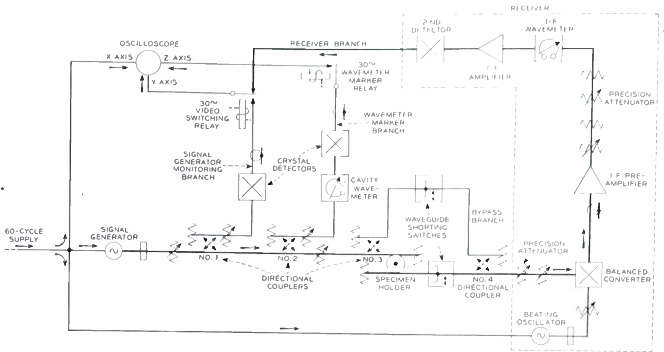
Fig. 2—Block diagram of wire-conductivity measuring equipment.
