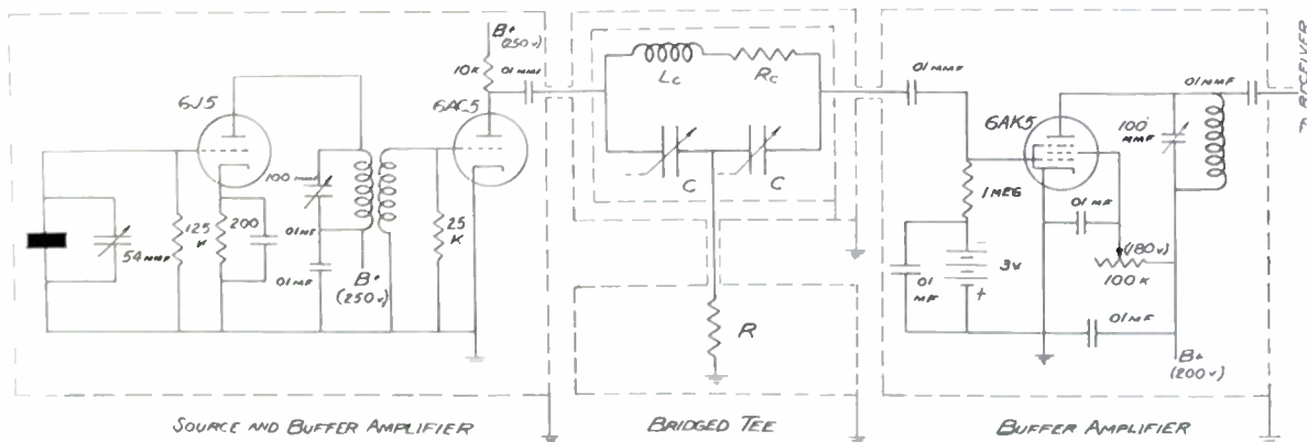
Fig. 2—Schematic diagram of measuring circuit.
