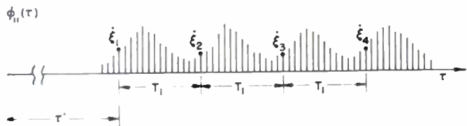
Fig. 8—Output graph of electronic correlator for large values of \tau .
