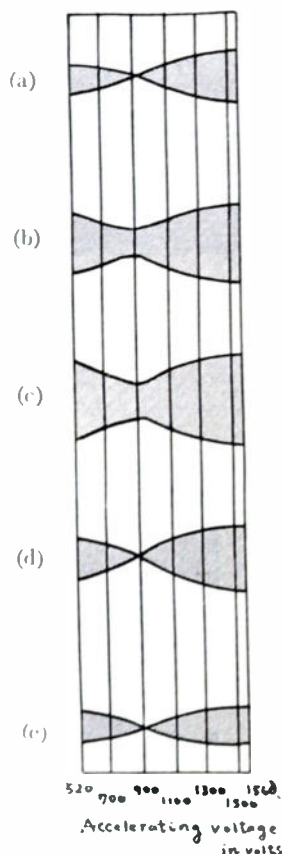
Fig. 8—Inversion spectrum for various terminated conditions. Sections (a) and (e) are cases when the waves are very small. Sections (b), (c), and (d) are cases when reflection occurred.
