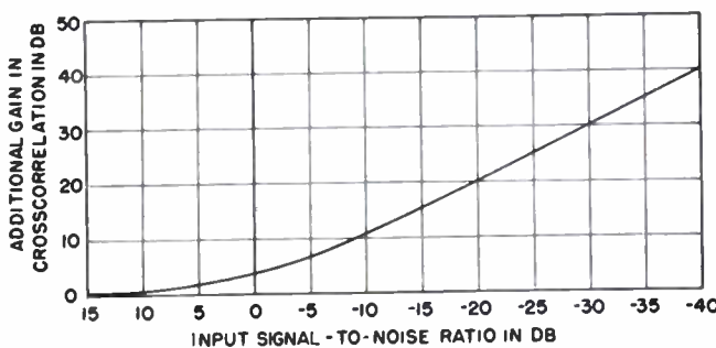
Fig. 11—Additional gain in signal-to-noise ratio through crosscorrelation as compared with autocorrelation (difference of the two curves in Fig. 9.)
