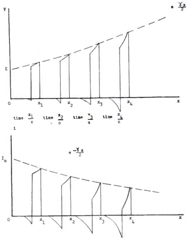
Fig. 3—Sketches of voltage and current distribution on an infinite line, excited by a short rectangular voltage pulse, for several instants of time at which the leading edge of the pulse has reached the positions x_1, x_2, x_3, and x_4 . The distortion is exaggerated and corresponds to that occurring with very great taper.
