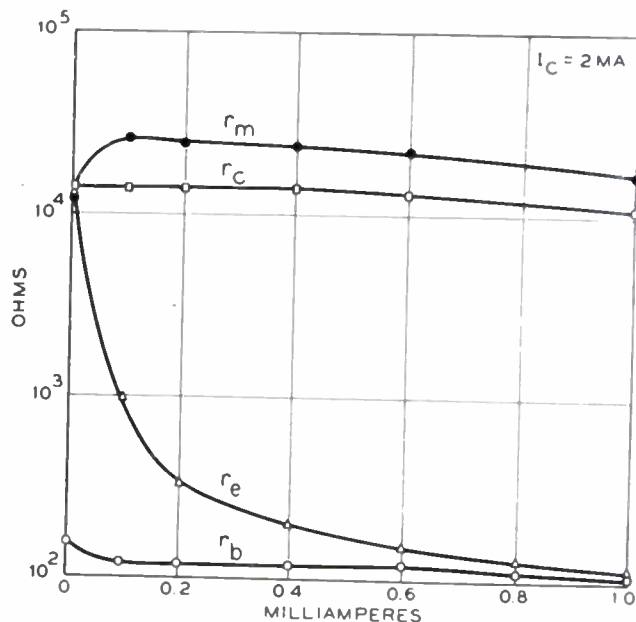
Fig. 4—Small-signal self- and transfer-impedances of a representative p -germanium transistor.
