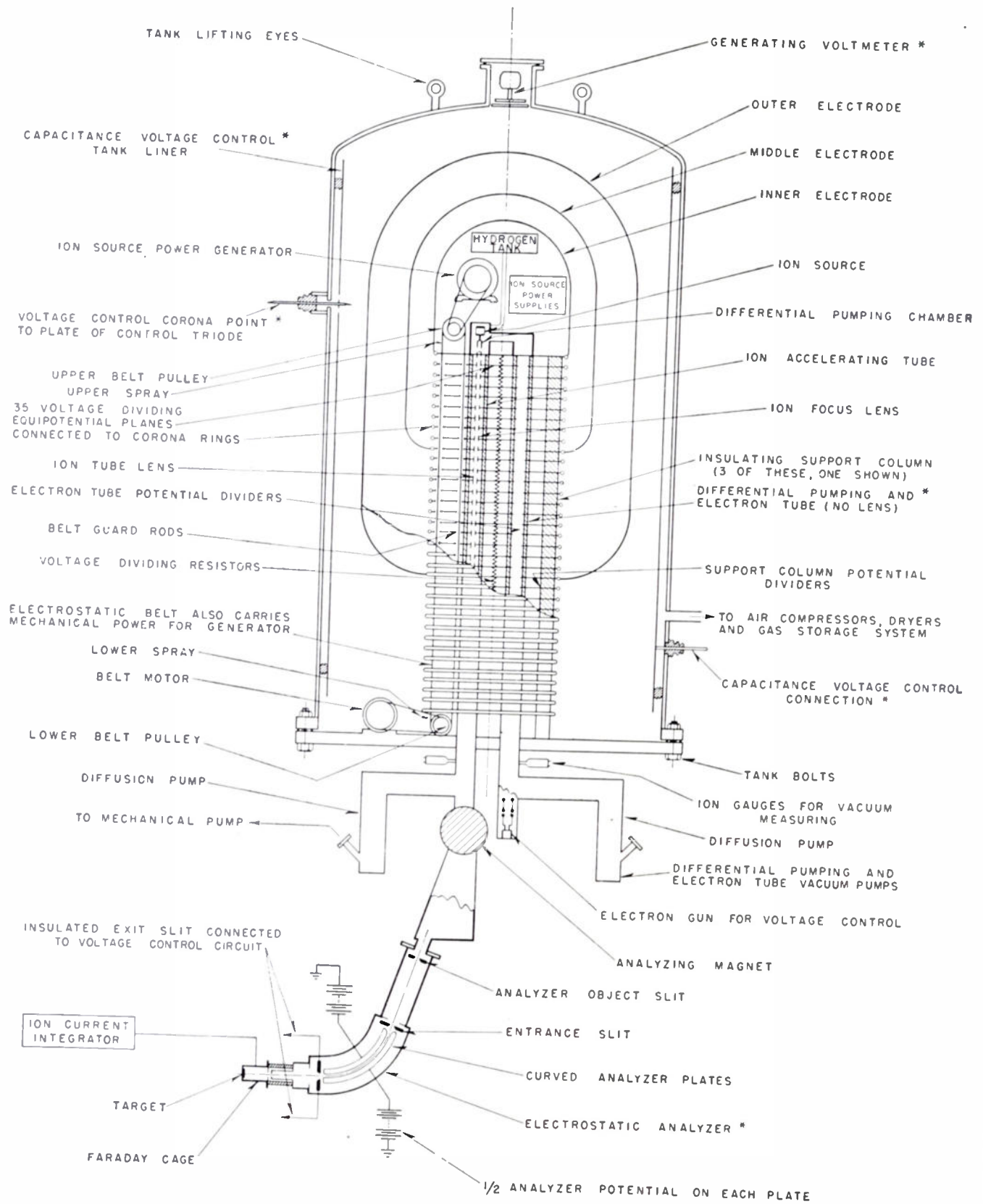
Fig. 1—Schematic of an electrostatic generator.
