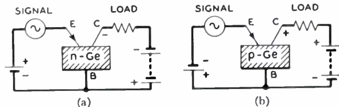
Fig. 1—Schematics showing operation of (a) n -germanium transistor, and (b) p -germanium transistor.
