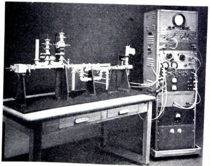
Fig. 4—The complete conductivity-measuring apparatus.
