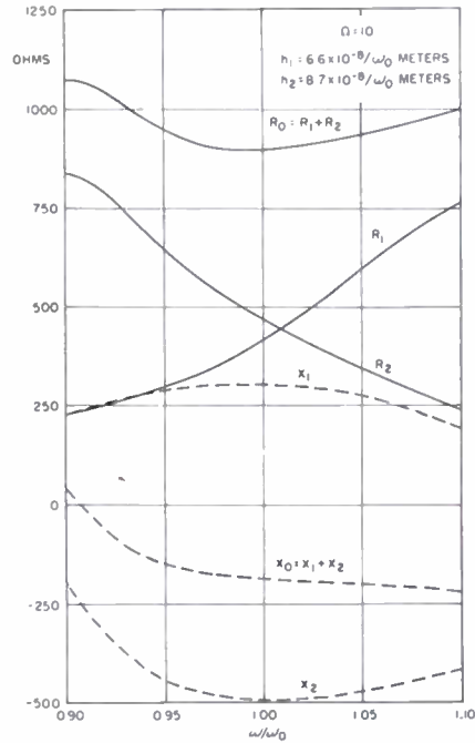
Fig. 6—Broad-band characteristics of asymmetrical antenna.
