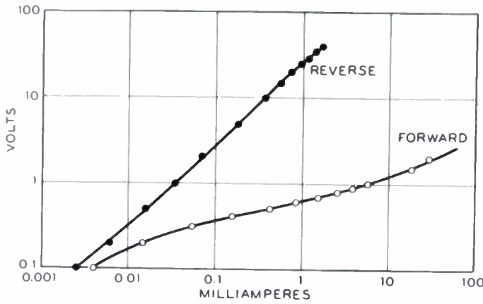
Fig. 7—Current-voltage characteristic of collector junction in a representative p -germanium transistor.
