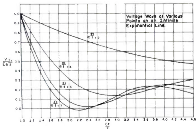
Fig. 1—Voltages at the end of step-up sections of exponential transmission line of length x (terminated in an indefinite continuation of the same line) as functions of a time parameter ct/x when the lines are excited with a step input voltage E at time t=0 . Curves are drawn for sections with voltage ratios of one to two, four, six, and seven, and voltage is expressed as a ratio of actual voltage to the input voltage multiplied by the voltage ratio in each case.
