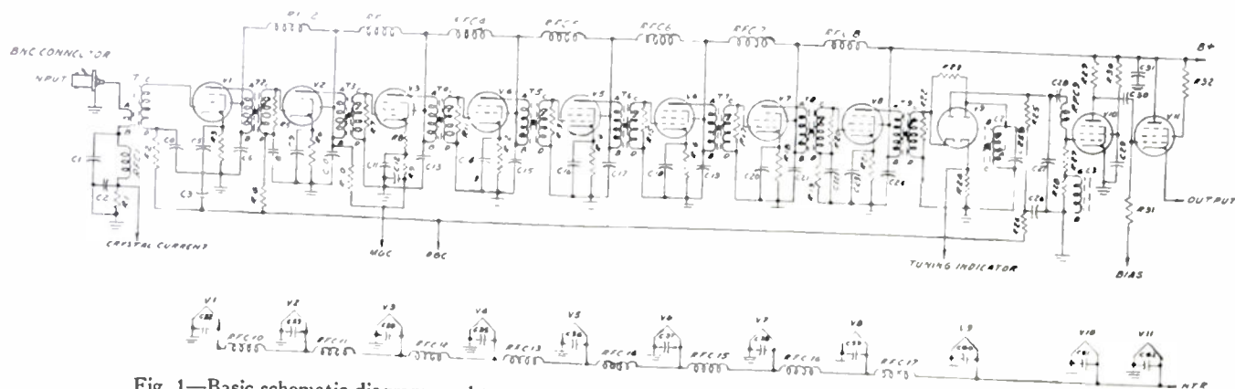
Fig. 1—Basic schematic diagram used to construct miniature wide-band amplifiers. Note—All transformers except T1 are bifilar wound. C25 is temperature compensating.
