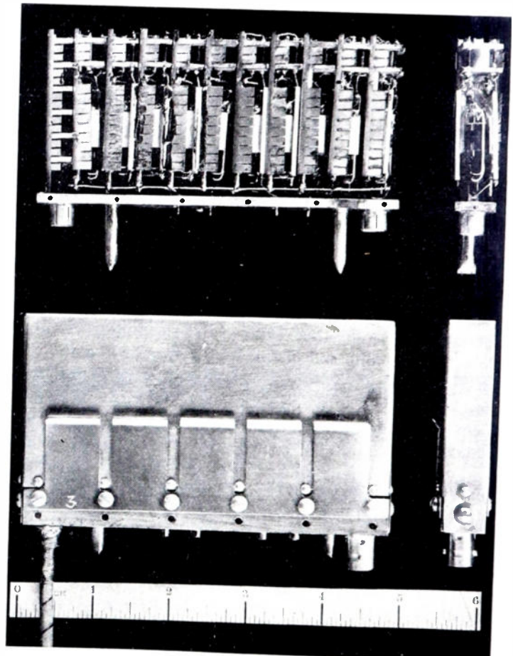
Fig. 8—Model V miniature intermediate-frequency amplifier. (Top) Side and end views of final assembly. (Bottom) Side and end views of encased amplifier in socket.
