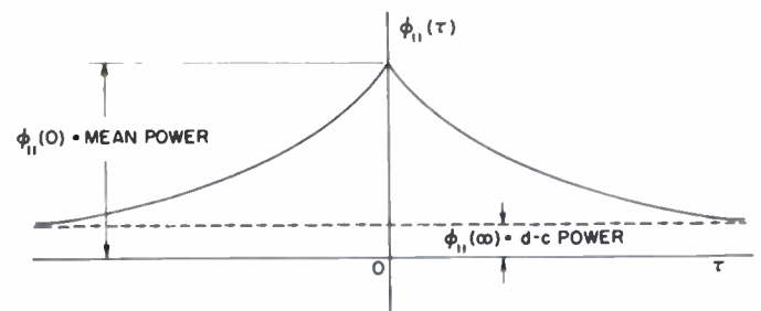
Fig. 1—Sketch of an autocorrelation function.
