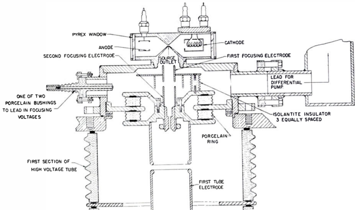
Fig. 6—A capillary-type ion source.
