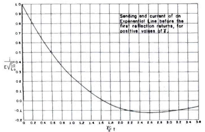
Fig. 4—Current at the sending end of an exponential transmission line when the line is excited at this point by a step voltage function. This current is applicable not only in the case of the line of infinite extent but also to any line section prior to the arrival of reflections from the receiving (load) end.
