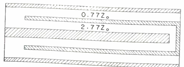
Fig. 7—Transformations due to frequency-compensating matching section.
