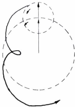
Fig. 10—Lissajous figure when vectors incidental to fundamental and harmonic wave are rotating in the same direction.
