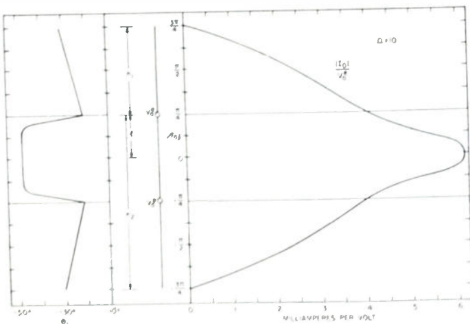
Fig. 10—Current distribution on the sleeve dipole.
