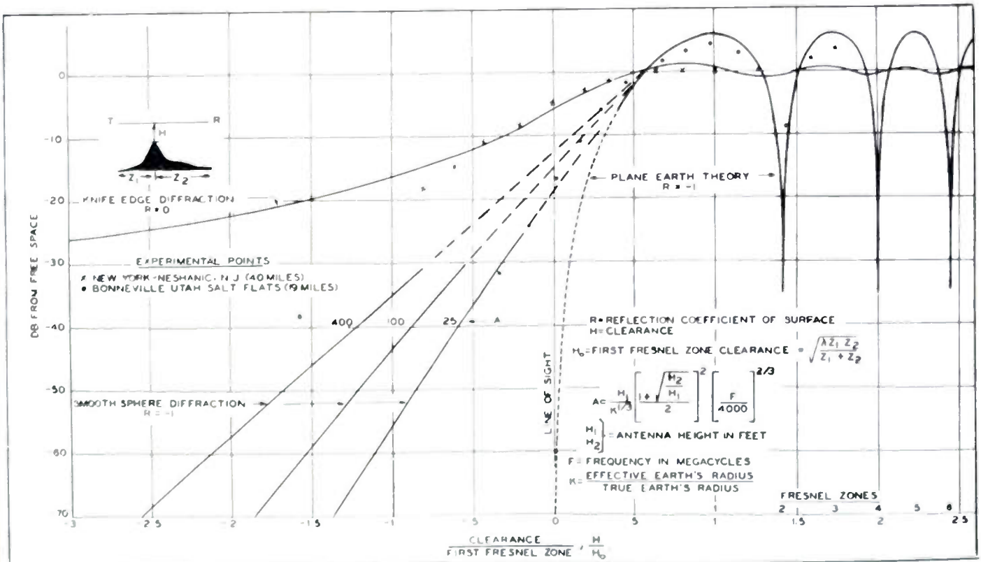
Fig. 1—Effect of clearance on radio transmission.
