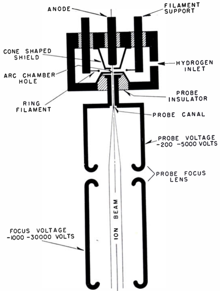
Fig. 5—A Zinn-type ion source.
