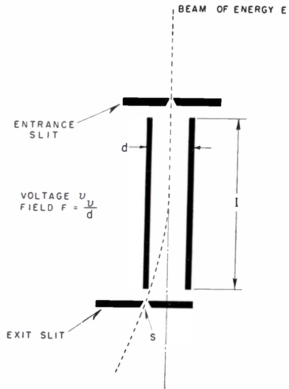
Fig. 9—A parallel plate electrostatic analyzer.
