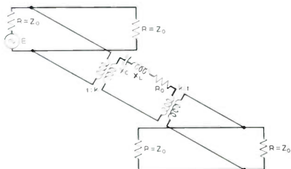
Fig. 8—A representation of the equivalent circuit of the specimen holder shown in Fig. 1.
