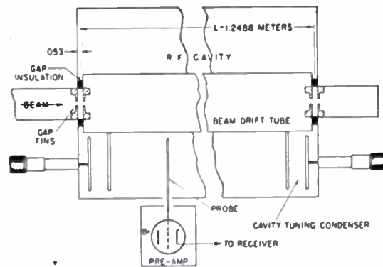
Fig. 12—An schematic section of the speed gauge cavity, giving essential dimensions.
