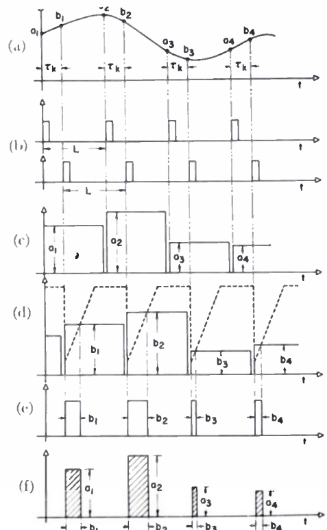
Fig. 5—Characteristic wave forms of electronic correlator.
