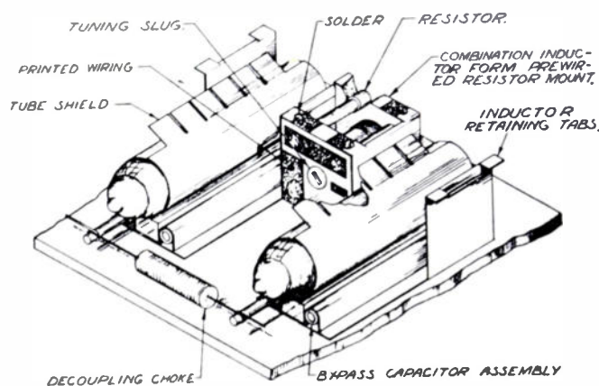
Fig. 3—Stage assembly of the Model II intermediate-frequency amplifier.
