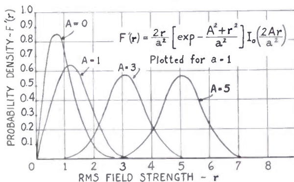
Fig. 1—Probability-density curves for various ratios of direct-path to reflected rms signal strength.
