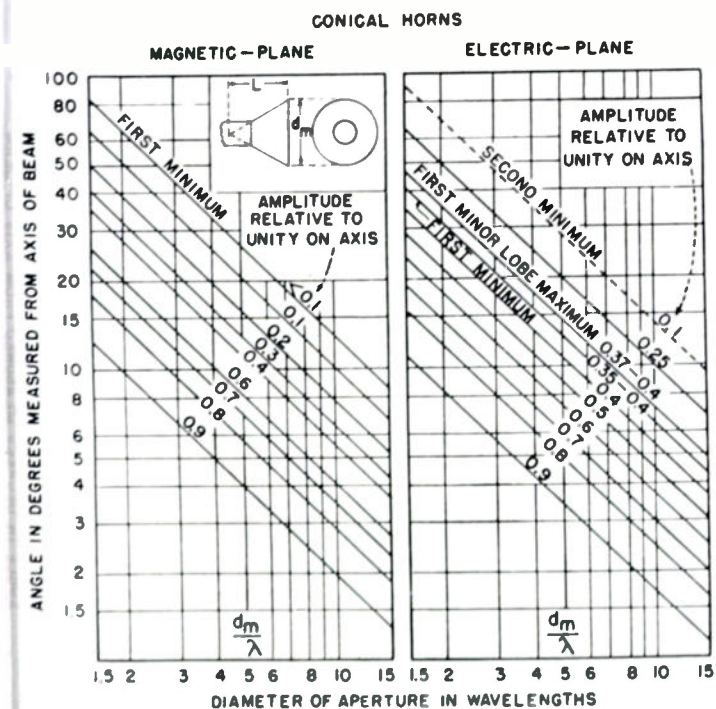
Fig. 6—Nomogram for plotting the radiation characteristic for conical horns of optimum design.
