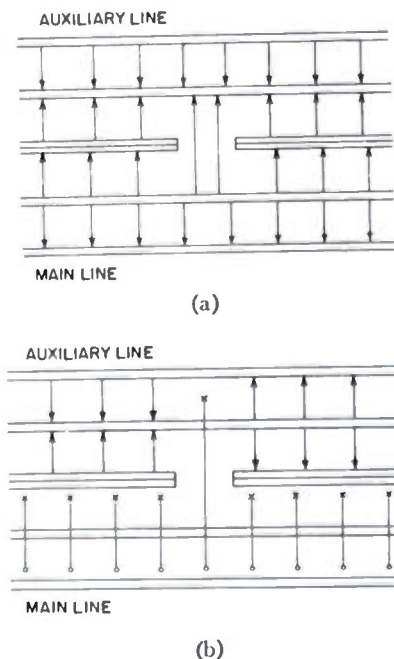
Fig. 2—(a) A schematic drawing showing the electric field in the auxiliary line produced by electric field component of a traveling wave in the main line. (b) A schematic drawing showing the electric field in the auxiliary line produced by the magnetic field component of the traveling wave in the main line.
