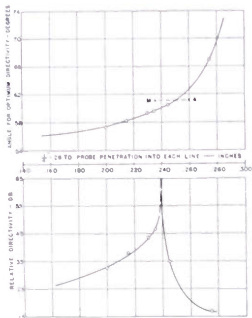
Fig. 5—The effect of capacity compensation upon the directivity and the optimum angle of a Bethe-hole coupler. The compensating capacity is introduced by means of a \frac{1}{4} -inch screw. The abscissa in this graph is the depth of penetration of the screws into the coaxial lines. The diameter of the hole = 1.098 inch. Inside diameter of the coaxial line = 0.875 inch.
