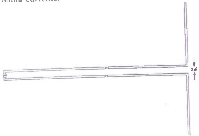
Fig. 1—Cylindrical antenna driven by two-wire open transmission line.
