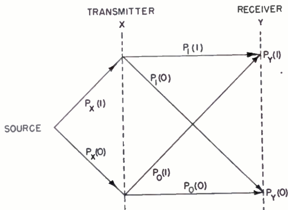
Fig. 1—Effect of noise on signal transmission.
