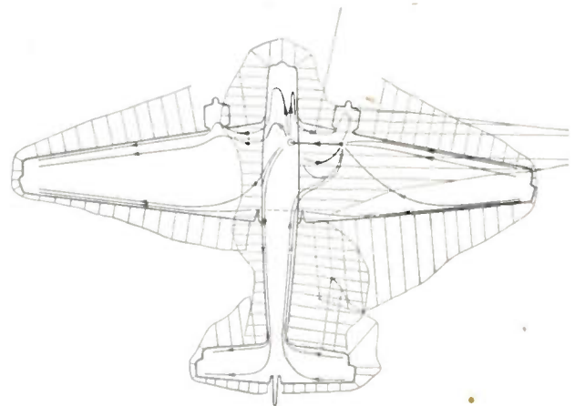
Fig. 2—Current distribution measured on a JU-52 aircraft with shunt-feed excitation of the wing. The length of the lines drawn perpendicular to the air frame is proportional to the amplitude of the current density at that point. The direction of the current at one instant of the rf cycle is shown by the arrows.
