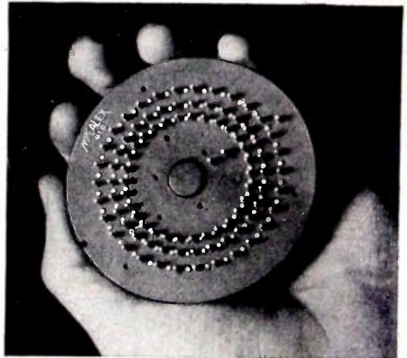
Illustrated are top and bottom views of the MYCALEX 410 molded insulation commutators manufactured to the specifications of Raymond Rosen Engineering Products, Inc., for Air Material Command, Navy telemetering projects, and other government agencies. These commutators are precision injection molded with 108 or 180 contacts and 3 slip rings all of coin silver.
