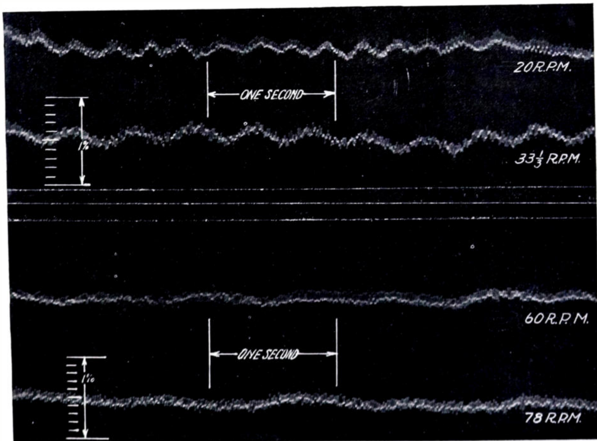
Fig. 7—Flutter oscillograms of variable-speed turntable.
