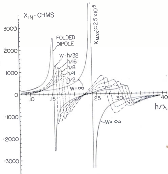
Fig. 8—Input reactance of the corresponding structures of Fig. 7.
