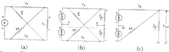
Fig. 1—The steps in the degeneration of the symmetrical lattice.
