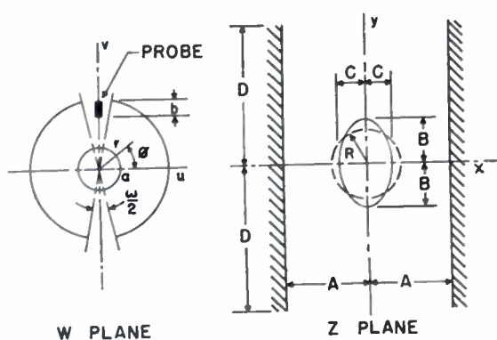
Fig. 5—Transformation of coaxial line to slab line.
