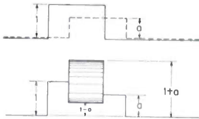
Fig. 3—Possible resultants of overlapping pulses. The resultant may fall below the slicing level for s = a + but will always exceed the slicing level for s < 1 - a .
