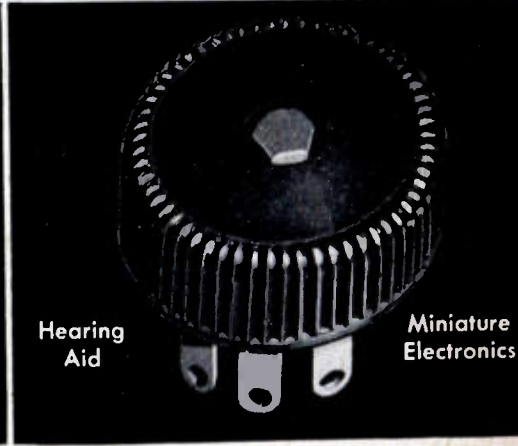
Centralab's Model 1 Radiohm Control — Model 1 Radiohm control available in plain or switch types. No larger than a dime! Rated 1/10 watt. Ideal for miniature uses.
