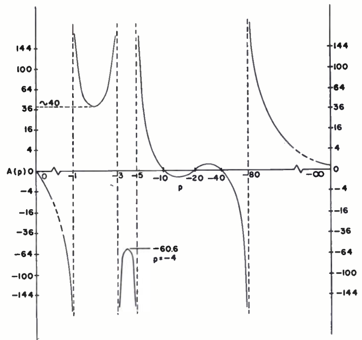
Fig. 2— A(p) for example of unloaded lattice.
