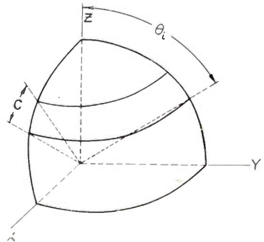
Fig. 1—Zonal type of scan.
