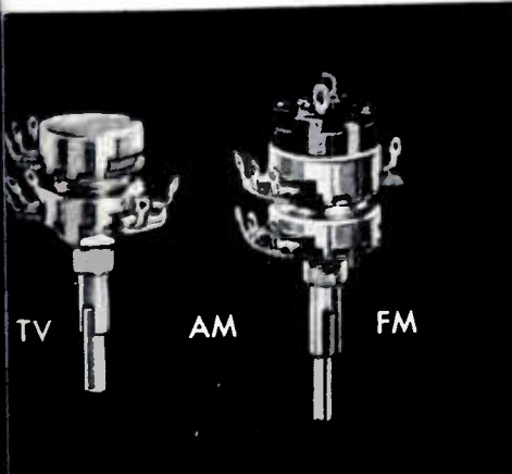
New Centralab Model 2 Radiohm Control — Left, twin unit plain type, front section tapped; right, twin unit switch type, rear section tapped. Both units have concentric shafts.
