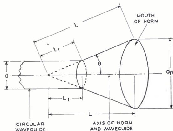
Fig. 1—Conical horn.
