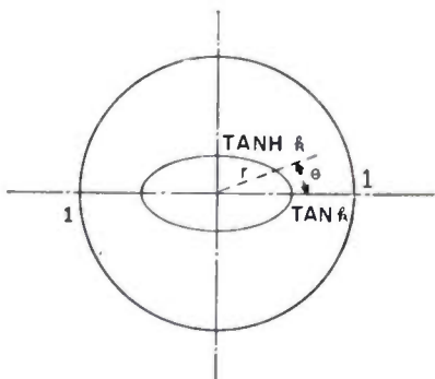
Fig. 6—Transformed slab line with circular center conductor.
