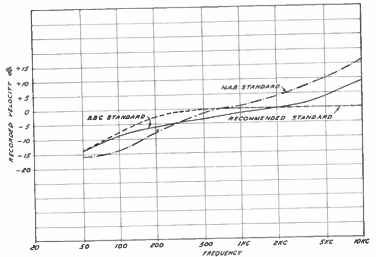
Fig. 6—Recording characteristics: BBC recording characteristic compared with the NAB and recommended standard.
