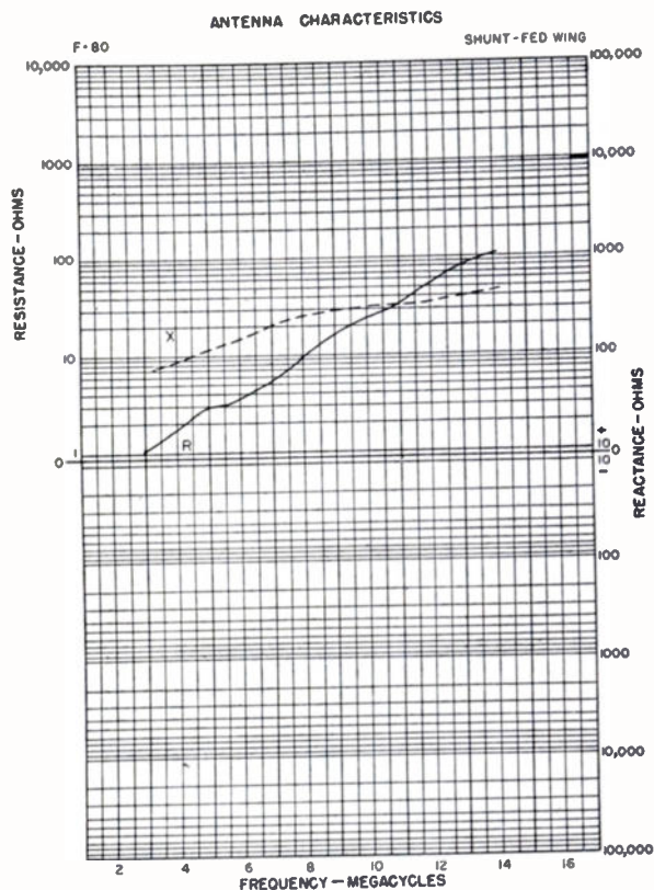
Fig. 10—Measured input impedance characteristic of the antenna structure shown in Fig. 5.
