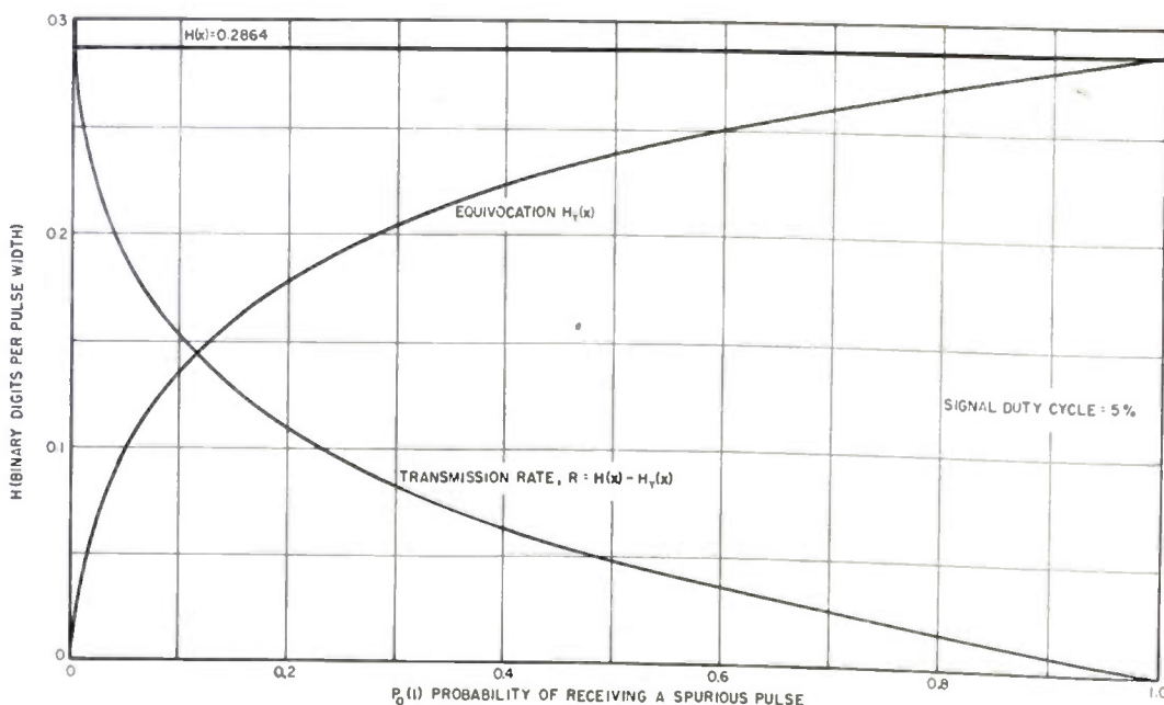
Fig 3—Effects of spurious pulses on transmission rate.
