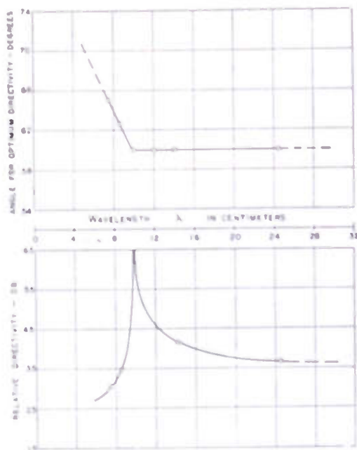
Fig. 6—The directivity and optimum angle for a properly compensated large hole coupler as a function of wavelength. The diameter of the hole = 1.098 inch; inside diameter of coaxial line = 0.875 inch.
