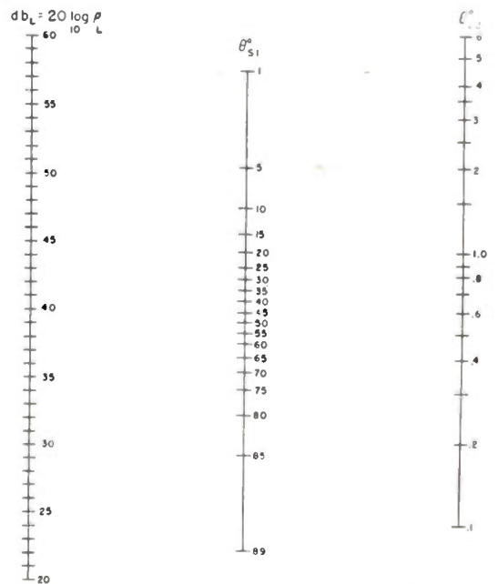
Fig. 2—Nomograph for method B of Table I.
