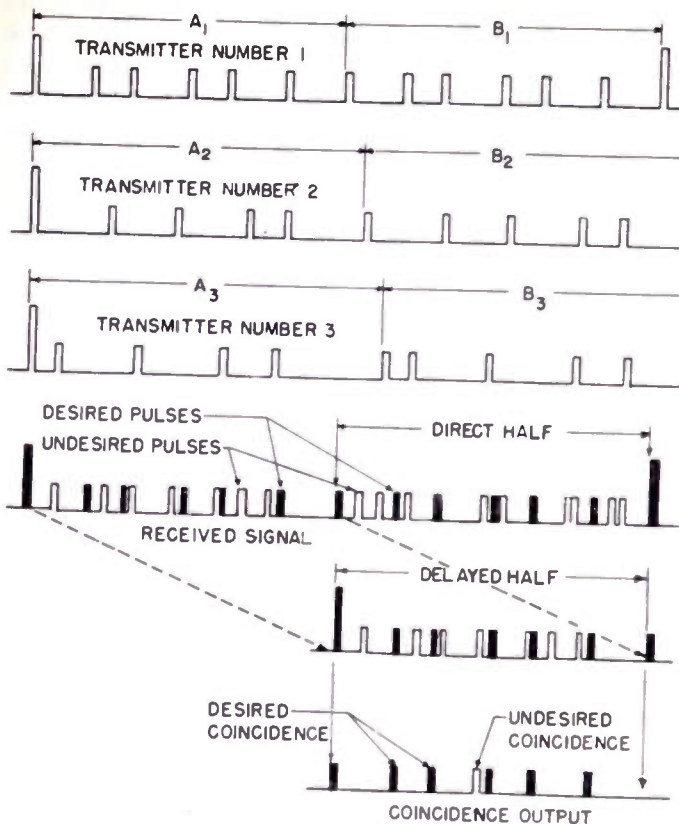
Fig. 6—Coincidence multiplex signal.
