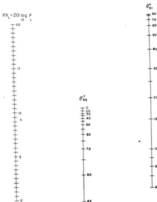
Fig. 9—Nomograph for method of Fig. 8.
