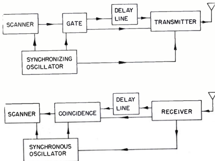
Fig. 5—Coincidence multiplex system.
