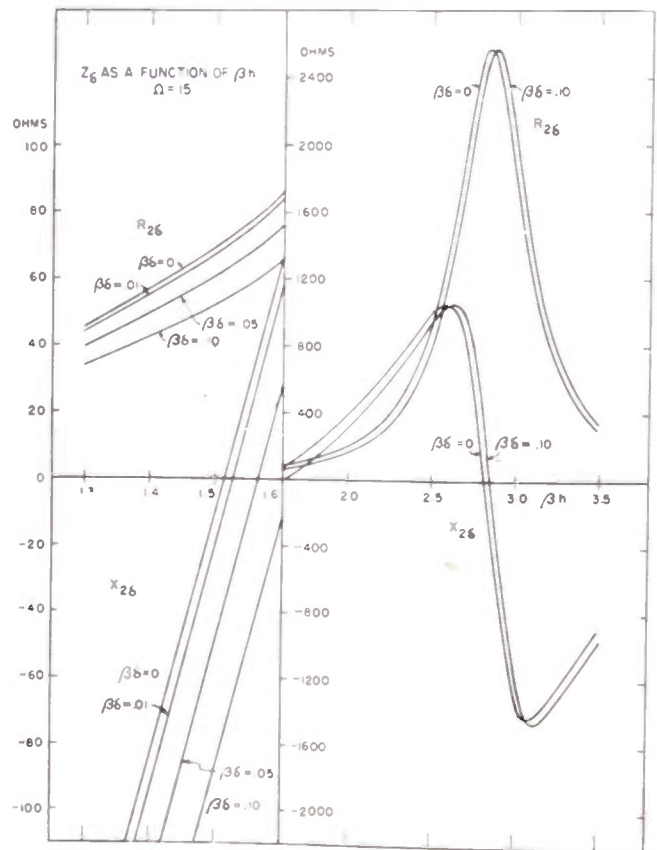
Fig. 3— Z_i as a function of \beta h ; \Omega = 15 .
