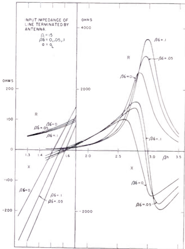
Fig. 2—Input impedance of line terminated by antenna.
