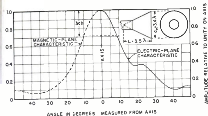
Fig. 5—Radiation pattern of a 17.7-db gain conical horn of optimum design.
