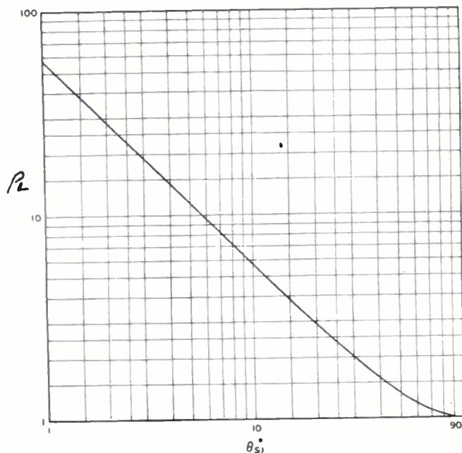
Fig. 3—Graph for method D of Table I.
