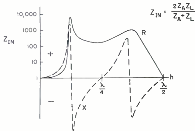
Fig. 6—Sketch of the input impedance of a symmetrical folded dipole of half-length h .
