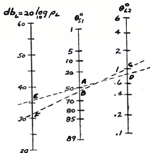
Fig. 10—Method for evaluating the range of VSWR values obtainable with method B of Table I.
