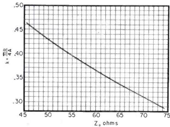
Fig. 3—Design curve for computing characteristic impedance.
