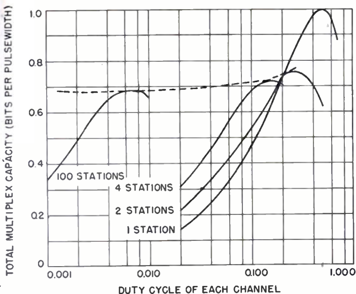
Fig. 4—Information capacity, simple asynchronous system.
