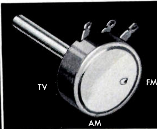
Centralab's Model "R" Radiohm Control — This control is wire-wound, 3 watts. Linear taper. Resistance: 2 to 10,000 ohms.
