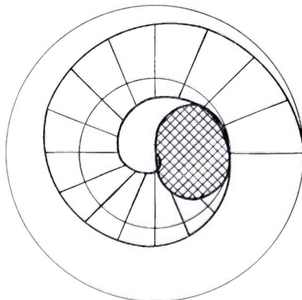
Fig. 2—Starting at its outer edge at an angle 2C from the pole (the outer circle), the radar beam touches the pole after one complete revolution. The region searched is indicated by radial lines.
