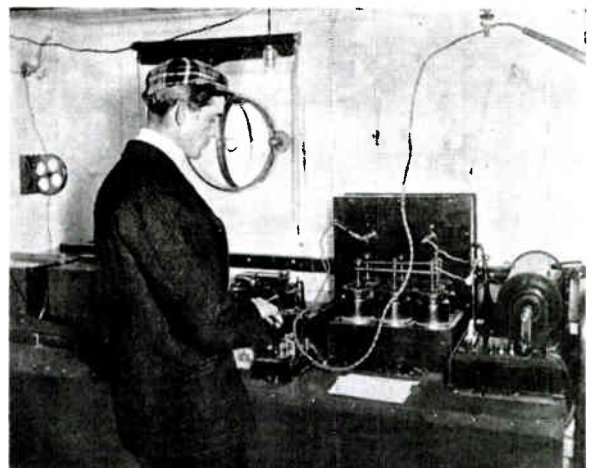
First experimental ship radio installation in U. S., on the S.S. St. Paul , 1899.
