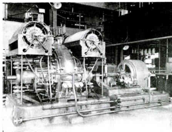
Alexanderson r.f. alternator, as installed at the RCA station in New Brunswick, November 1919.
