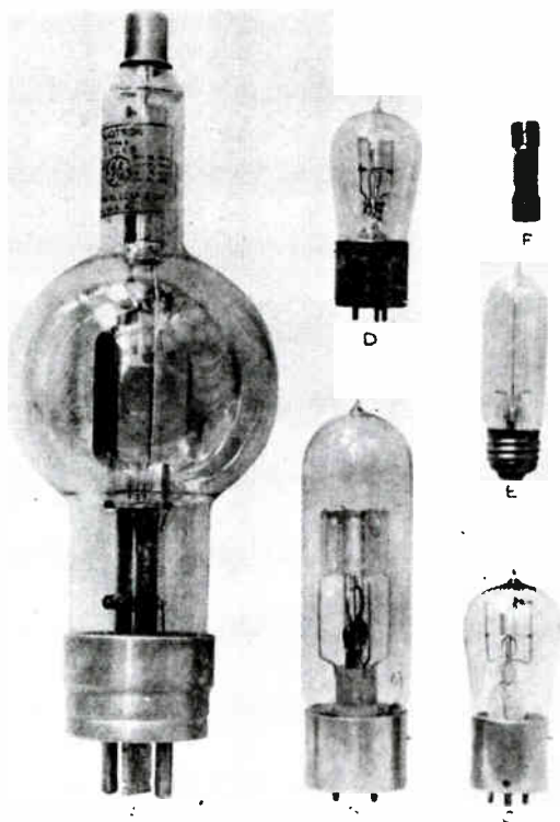
Receiving and transmitting tubes up to 5 watts, 1918.
