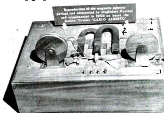
Early model of Marconi magnetic detector.
