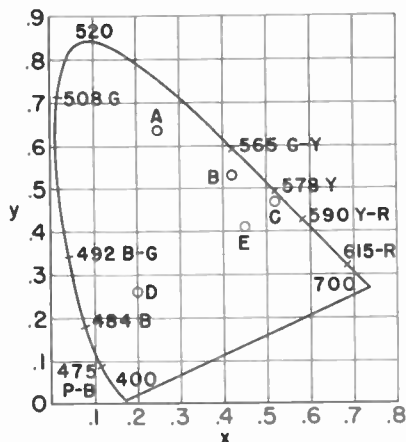
Fig. 5—ICI spectrum locus. Willemite = A ; Zn-Bc silicate = B ; blue sulfide = D ; illuminant A = E ; orange sulfide = C .
