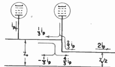
Fig. 14—Current distribution in tapered line.
