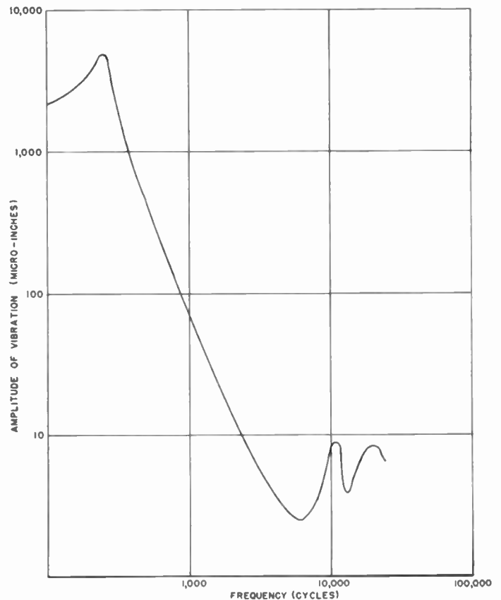
Fig. 9—Response of the vibrator with \frac{1}{4} ampere flowing through the driving coil.
