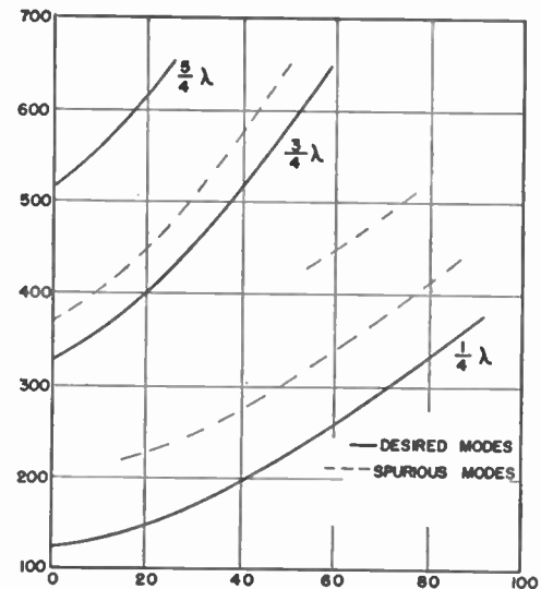
Fig. 4—Spurious modes in a split-stator line.
