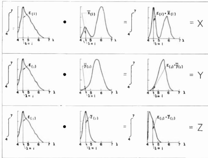
Fig. 4—Graphic representation of method of obtaining ICI tristimulus values.
