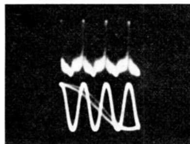
Fig. 13—Oscillogram illustrating hash type of microphonism.
