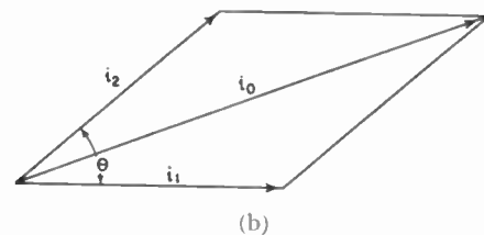
Fig. 4—(a) Paired-plate type of distributed amplifier; (b) current phase relations in paired plate amplifier.
