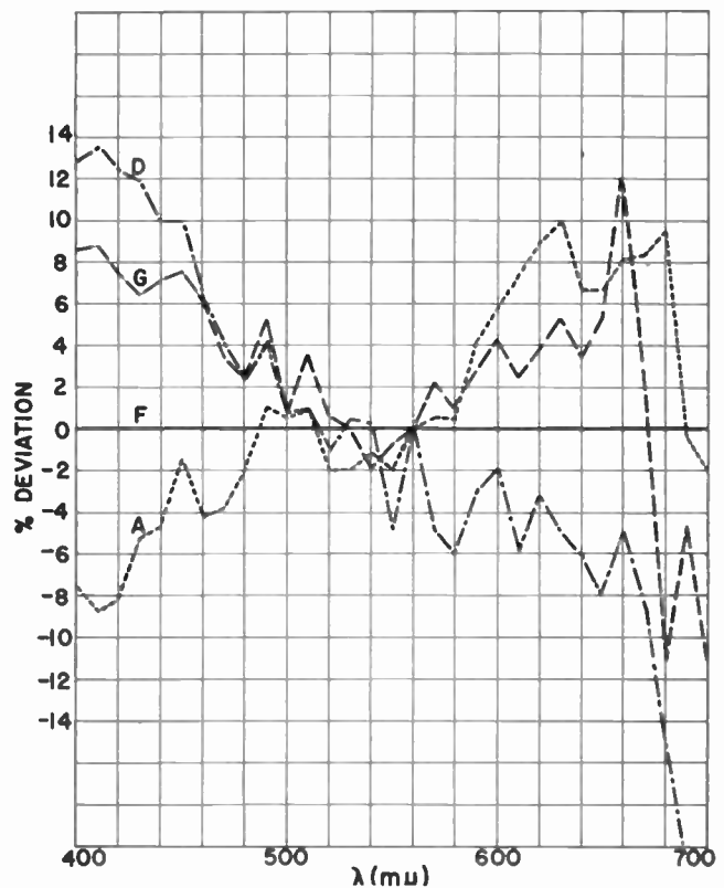
Fig. 11—Deviation of response curves from that of photocell F .
