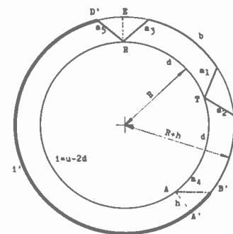
Fig. 16—Sliding-wave propagation around the earth; direct path, a_1 + b + a_3 , indirect path, a_2 + b + i' + a_4 .
