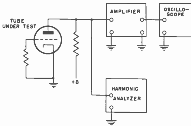
Fig. 10—Electrical test circuit block diagram.
