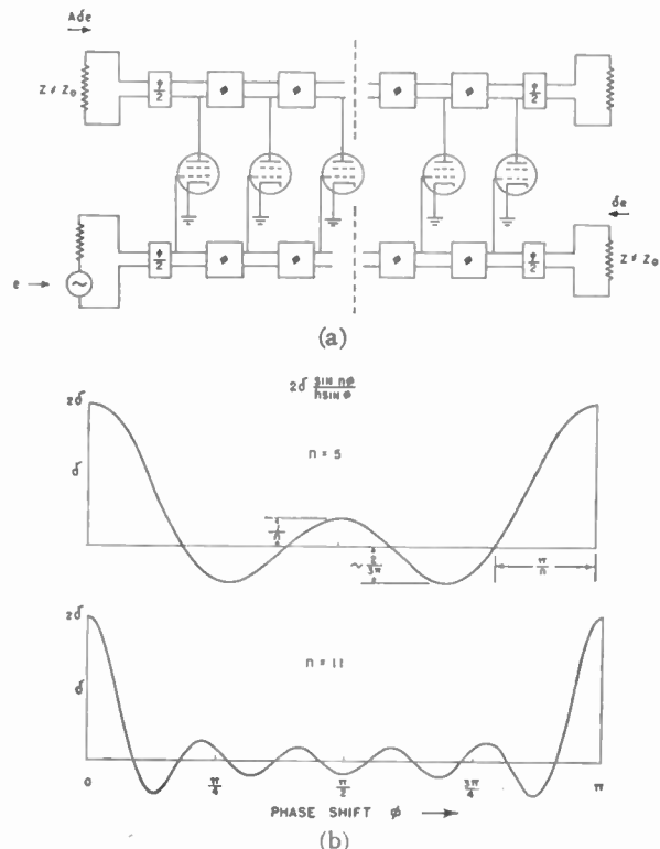
Fig. 12—(a) Diagram of distributed amplifier showing phase shift and reflection from terminations; (b) ratio of signal to reflected voltages.
