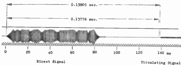
Fig. 15—Explanation of the errors in the measurements.
