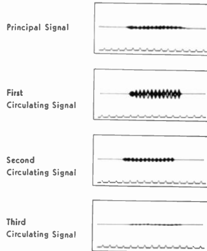
Fig. 10—Amplitudes on repeated circulating signals.
