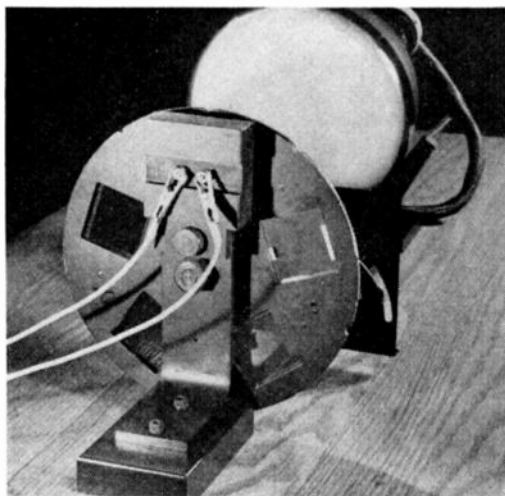
Fig. 7—Photoelectric tristimulus colorimeter.
