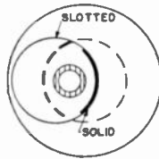
Fig. 12—Cross section of the distributed-capacitance line.
