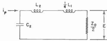
Fig. 21—Equivalent plate circuit of the bridged-tee connection.
