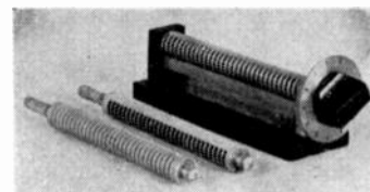
Fig. 8—A distributed-inductance line.
