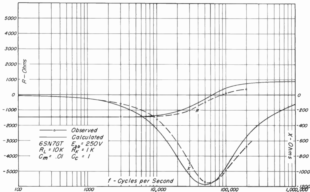
Fig. 6—High-frequency case considering C_M . Series components of impedance versus frequency.
