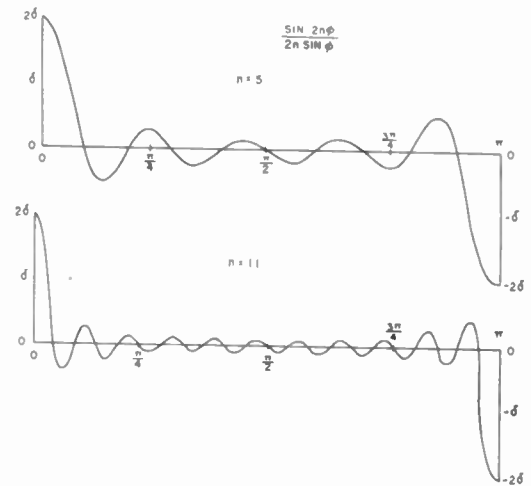
Fig. 13—Variations in output voltage.
