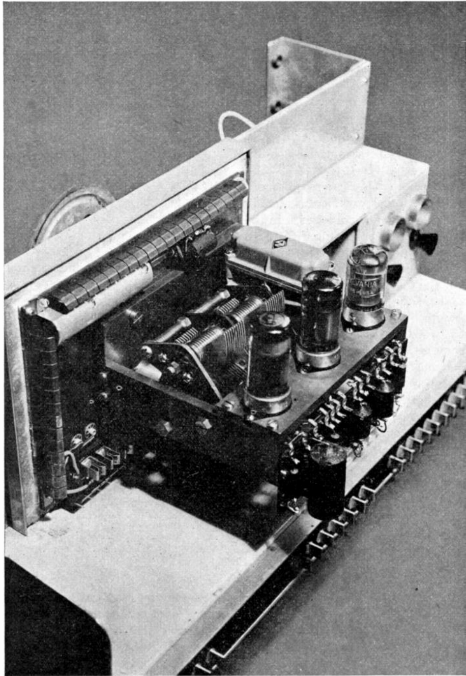
Fig. 11—Rear view of the first oscillator with thermostat and double screening removed.
