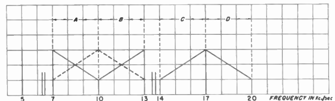
Fig. 1—Arrangement of channels in former equipment.
