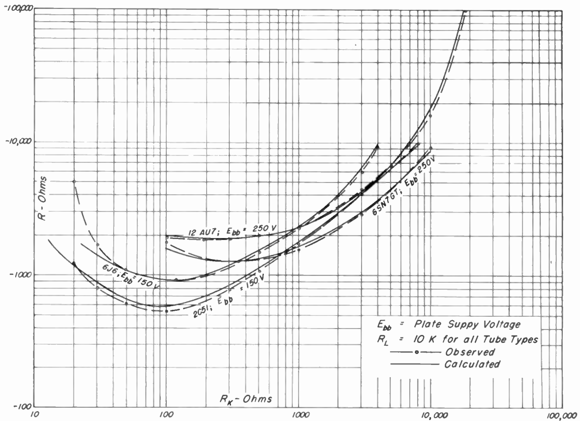
Fig. 2—Negative resistance as a function of cathode resistance; tube types 6SN7GT, 6J6, 12AU7, and 2C51.
