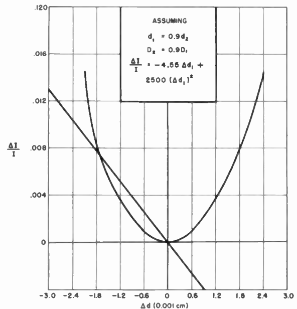
Fig. 3—First- and second-order output variation resulting from filament shift on the triode.
