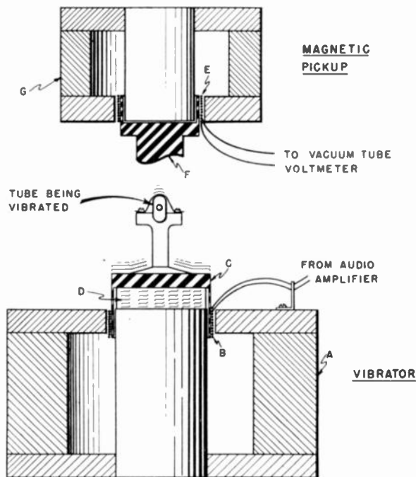
Fig. 8—Electromagnetic vibrator.
