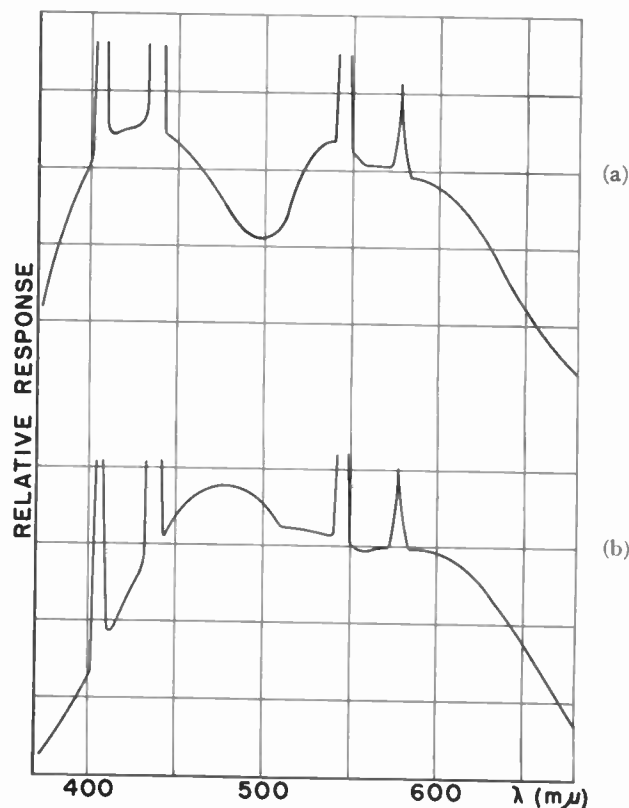
Fig. 8—Spectroradiometric comparison of two fluorescent lamps. (a) x=0.314 , y=0.323 (b) x=0.313 , y=0.324 .
