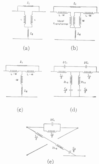
Fig. 10—Equivalent circuits for bridged-tee connection.
