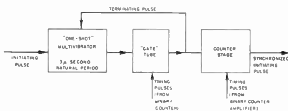
Fig. 3—Block diagram of the pulse synchronizer.
