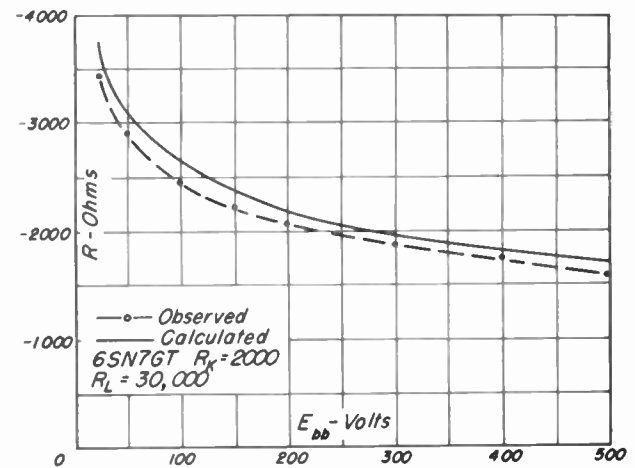
Fig. 7—Negative resistance versus plate-supply voltage.
