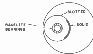
Fig. 11—Cross section of the distributed-inductance line.
