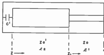
Fig. 13—Diagram of the discontinuity line.
