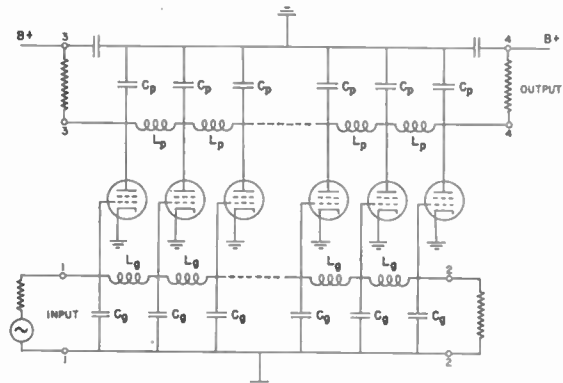
Fig. 1—Basic distributed amplifier.
