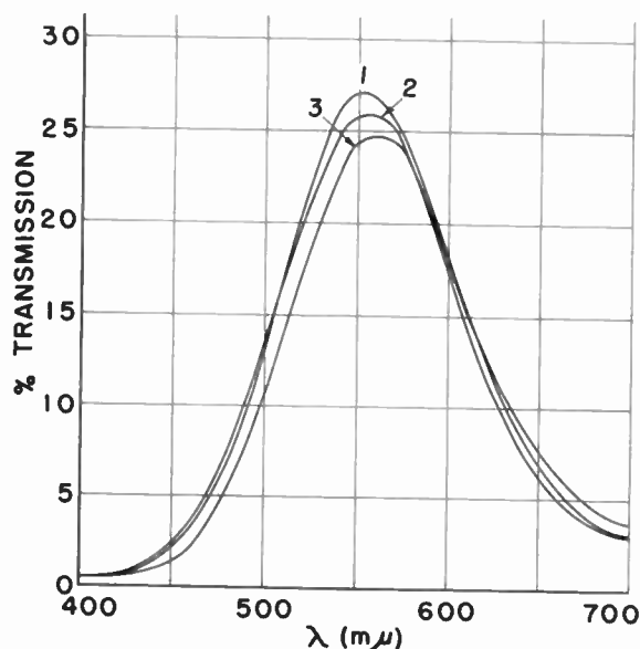
Fig. 12—Transmission curves— B filters for Barnes colorimeter.
