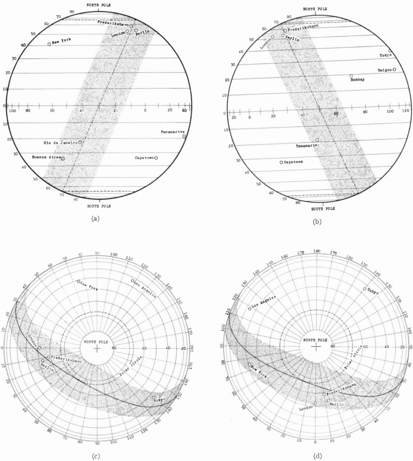
Fig. 3—Direction of the echo zone; (a) in winter at 09 h 00 m and in summer at 21 h 00 m CET; (b) in winter at 15 h 40 m and in summer at 03 h 40 m CET; (c) in winter at 09 h 00 m and in summer at 21 h 00 m CET; (d) in winter at 14 h 20 m and in summer at 02 h 20 m CET.
