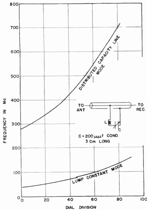
Fig. 5—Wavetrap modes of operation.
