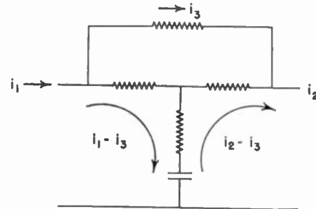
Fig. 20—Bridged-tee current connection.
