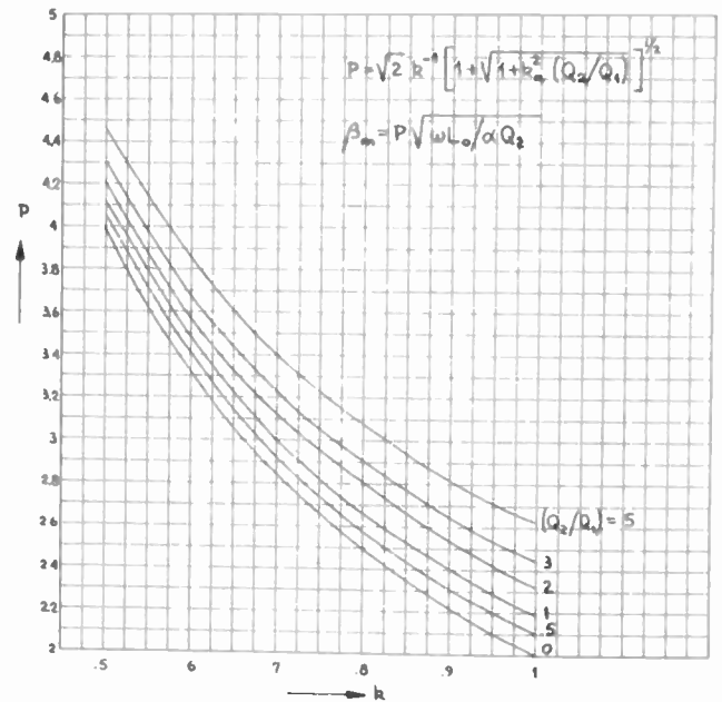
Fig. 2—Chart which permits the calculation of the function \beta_m and from this the optimum LNSI and sensitivity, according to equations (3) and (4).
