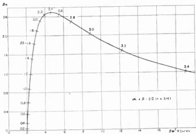
Fig. 6—Conversion-efficiency characteristic curve.
