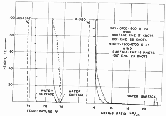
Fig. 14—Day and night temperature and mixing-ratio curves from mean soundings of March 9, and 10, 1945.
