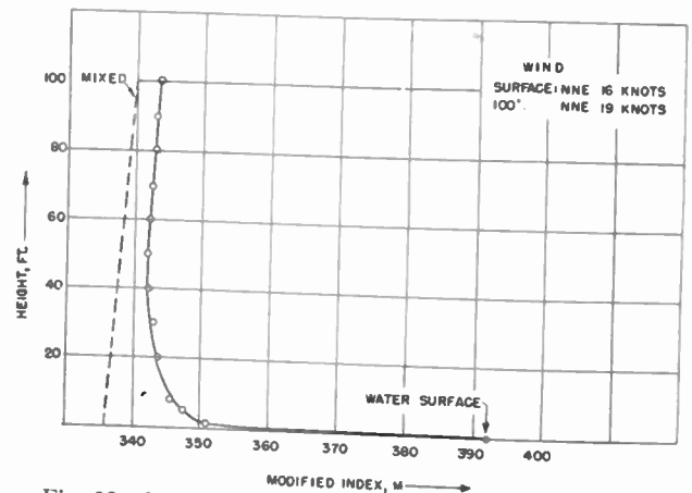
Fig. 22—Modified index curve, average for 1900-0700, March 27 to 29, 1945.
