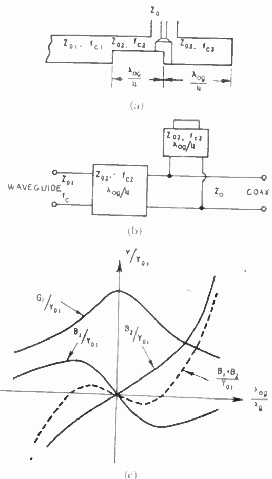
Fig. 4—Transforming-type junction. (a) Schematic. (b) Approximate equivalent circuit. (c) Admittance curves for f_c = f_{c1} = f_{c2} .
