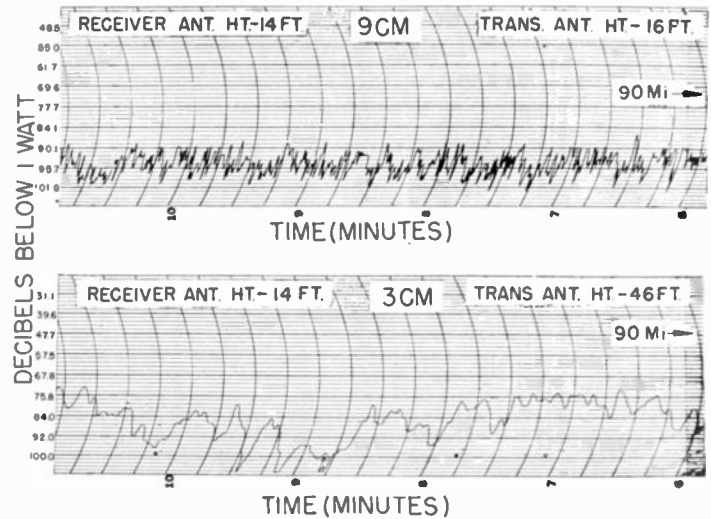
Fig. 6—High-speed records of March 20, 1945, range of 90 miles.
