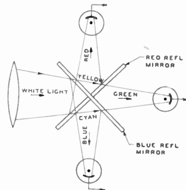
Fig. 5—Crossed dichroic beam-splitter.
