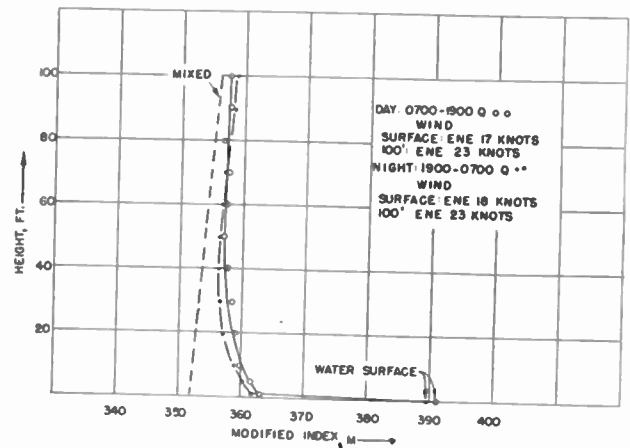
Fig. 15—Day and night M curves of March 9 and 10, 1945, sounding.
