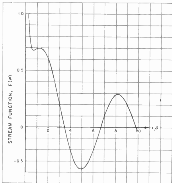
Fig. 1—Radial variations of typical stream function.
