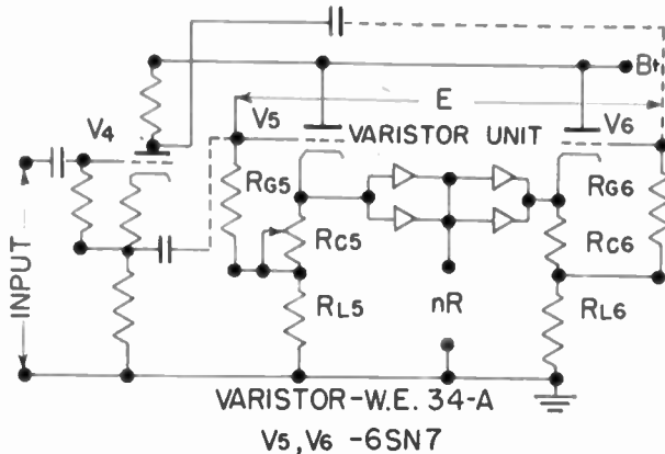
Fig. 6—Frequency-control circuit. R_{g5} = R_{g6} = 1.0 megohm R_{c5} = R_{c6} = 2000 ohms R_{L5} = R_{L6} = 20,000 ohms B+ = 250 volts
