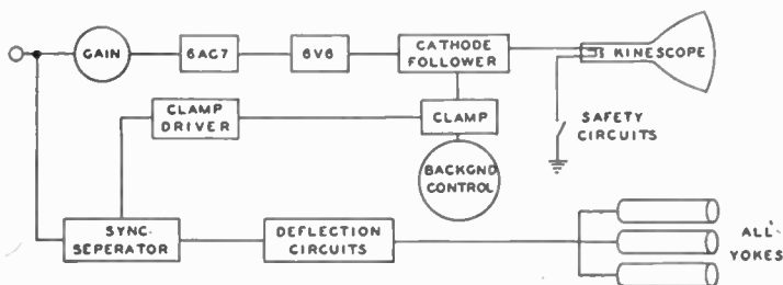
Fig. 11—Video block diagram of green channel.
