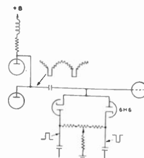
Fig. 11—Detail of the clamp circuit.
