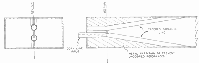
Fig. 11—A wave-guide-to-coaxial-line junction having a length of tapered loaded wave guide as matching element.
