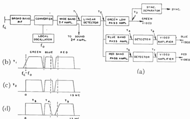
Fig. 3—Simultaneous color receiver for subcarrier reception.
