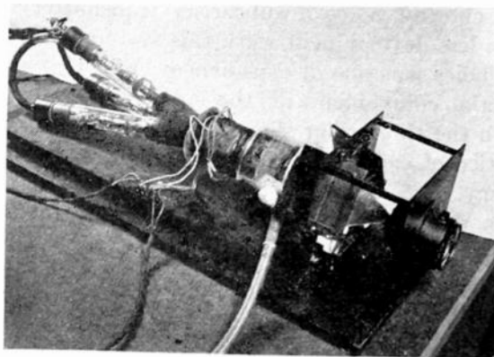
Fig. 5—Three-gun single-yoke tube.
