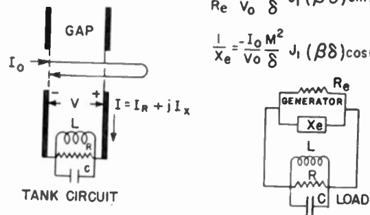
Fig. 3—Equivalent circuit for a reflex oscillator.
