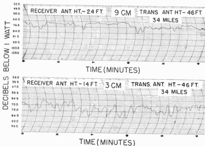
Fig. 5—High-speed records of March 20, 1945, range of 34 miles.
