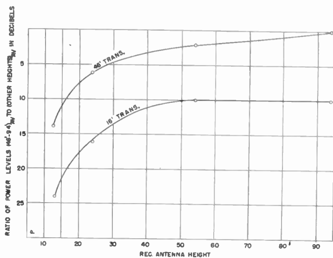
Fig. 12—Average height gain, 9 centimeters.
