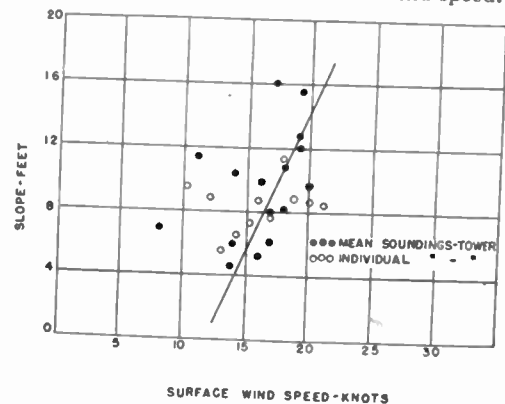
Fig. 25—Effective M slope versus wind speed.
