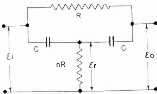
Fig. 2—Negative-feedback network.
