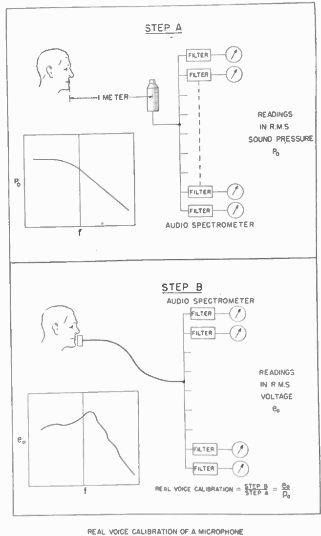
Fig. 7—Procedure for obtaining the real-voice calibration of a microphone. Upper step shows measurement of speech spectrum; lower shows measurement of voltage output of microphone.
