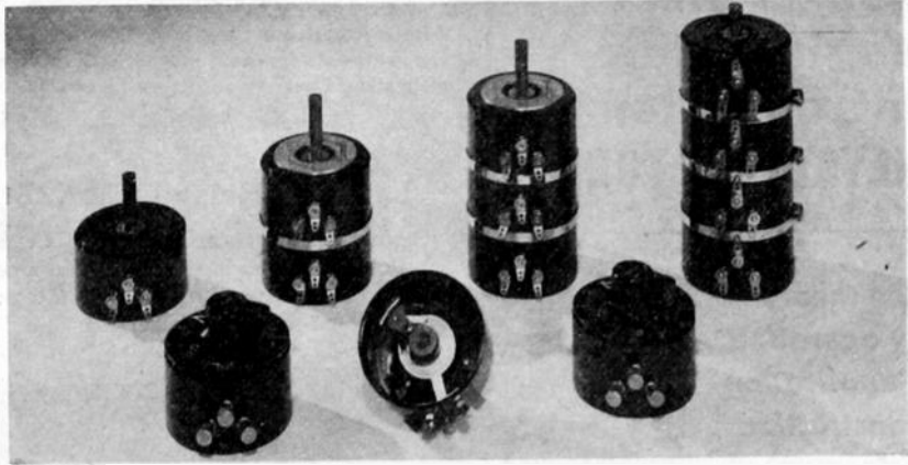
TOP: Type RVS Resistor . . . note clean design, simplicity of ganged assemblies. No need for mounting plates or spacers. Easily adjusted. BOTTOM CENTER: View of interior of resistor. BOTTOM LEFT AND RIGHT: Type RVL3 for experimental laboratories . . . direct reading.
