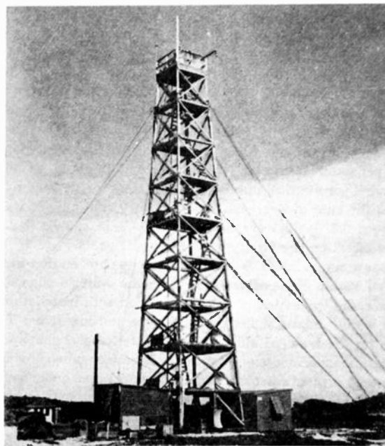
Fig. 2—90-foot tower with 9- and 3-centimeter receiving antennas.
