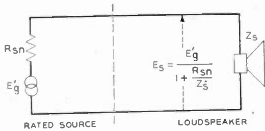
Fig. 4—Loudspeaker and associated rated source.
