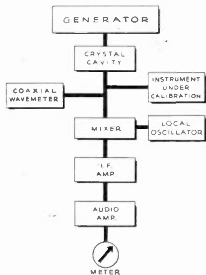
Fig. 5—Typical measuring setup.
