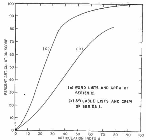
Fig. 11—Experimentally determined relations between word or syllable articulation and articulation index A .
