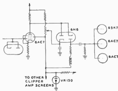
Fig. 13—Detail of the clipper circuit.
