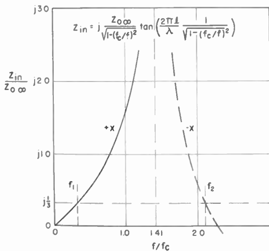
Fig. 10—Input impedance of a shorted wave-guide line. ( l = \frac{1}{2}\lambda_g at f = 1.41 f_c .)
