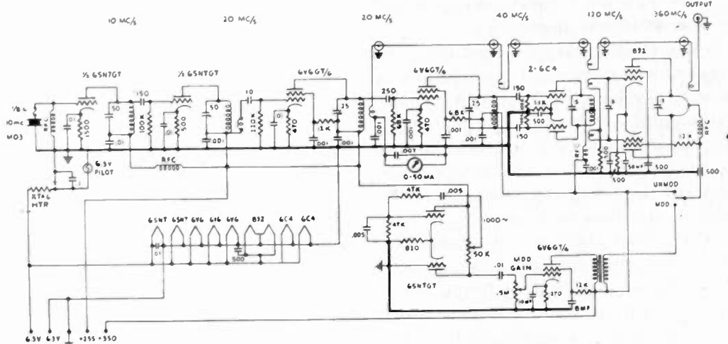
Fig. 2—Silicon crystal multiplier, secondary frequency standard.
