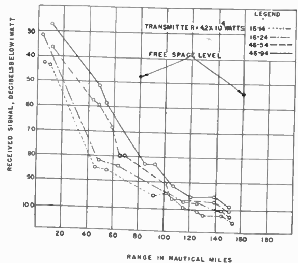
Fig. 7—Received power versus range at 9 centimeters, March 15, 1945.
