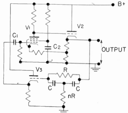
Fig. 5—Practical oscillator circuit.
