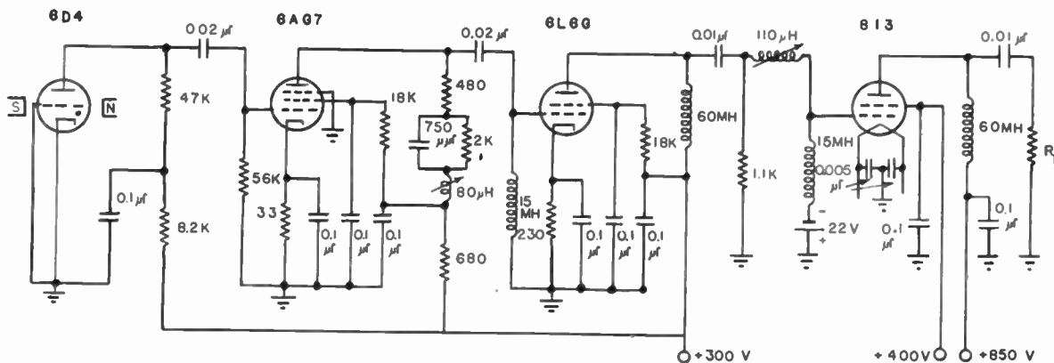
Fig. 5—High-level wide-band (0.1 to 2.5 megacycles) noise generator. R_L either 2000 or 4000 ohms.
