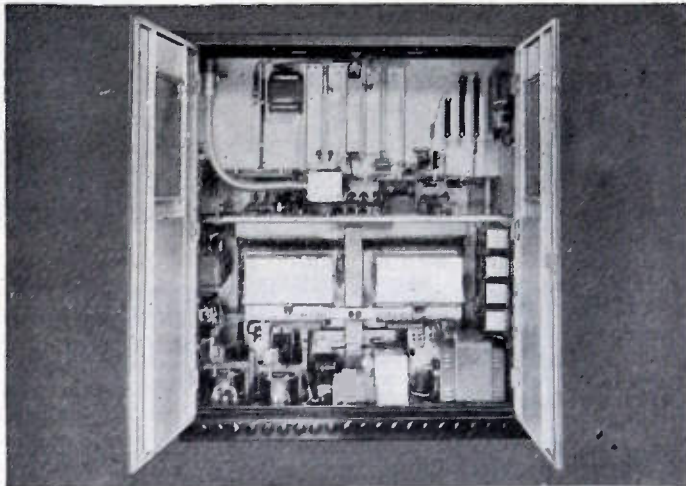
EASY TO MAINTAIN... full-opening doors, open vertical arrangement of components and power outlets, facilitate inspection and maintenance. All access doors are electrically and mechanically interlocked for safety of service personnel.
