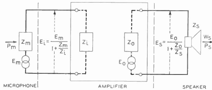
Fig. 2—Schematic of simplified sound-system circuit.
