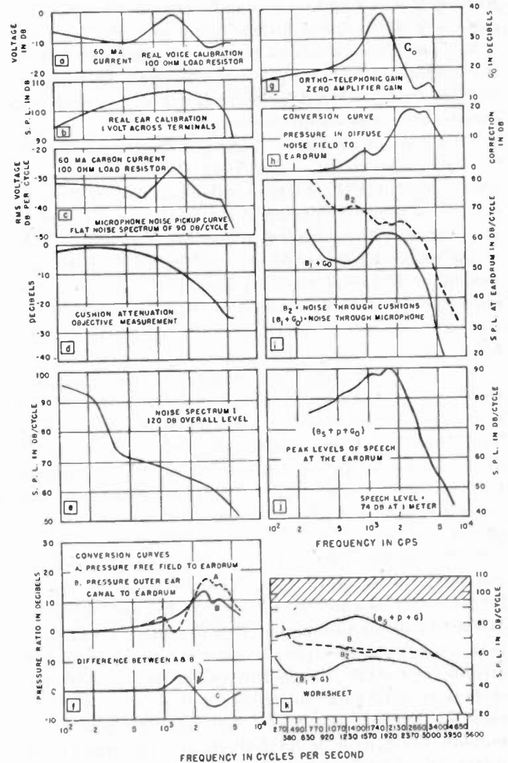
Fig. 16—Detailed steps in calculation of articulation index. The procedure is outlined in the text.
