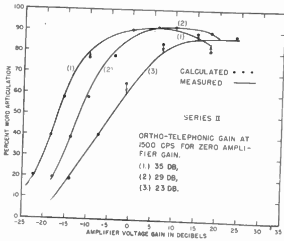
Fig. 14—Comparison of experimentally determined and calculated articulation scores for three types of interphone systems in an untreated bomber.
