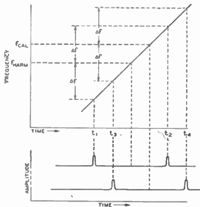
Fig. 4—This diagram shows how the pips are presented on the oscilloscope screen at the same times that the frequency of the frequency-modulated oscillator differs from that of the two fixed frequencies by \Delta f , the frequency of the receiver.
