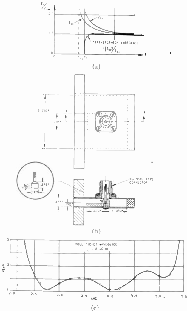
Fig. 7—Ridge-block transforming junction. (a) "Transformed" impedance. (b) Construction. (c) Frequency response.
