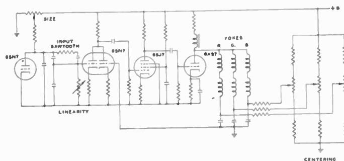
Fig. 7—Vertical-deflection circuit.
