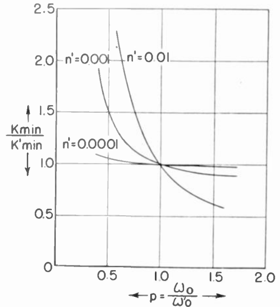
Fig. 4—Positive-feedback ratio versus \omega_0/\omega_0' .
