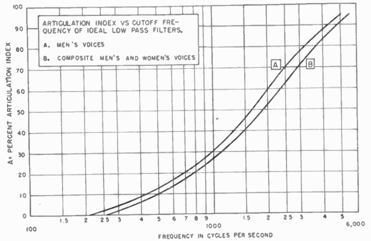
Fig. 9—Articulation index versus cutoff frequency of ideal low-pass filters as determined by French and Steinberg.
