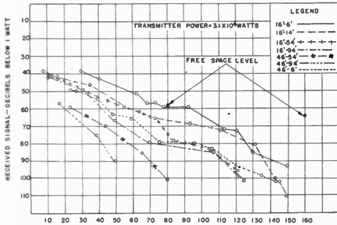
Fig. 8—Received power versus range at 3 centimeters, March 15, 1945.
