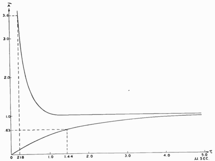
Fig. 8—Unit-function responses of the flying-spot scanner.
