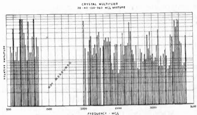
Fig. 3—Radio-frequency spectrum.
