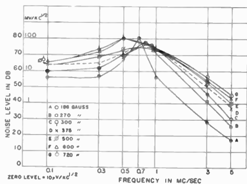
Fig. 2—Effect of magnetic field strength on the 6D4 noise spectrum. Electromagnet used. Load resistance = 20,000 ohms. Anode current = 5 milliamperes.
