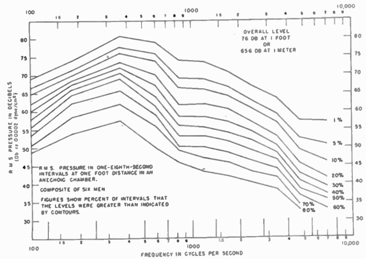
Fig. 2—Root-mean-square sound-pressure levels measured in successive \frac{1}{8} -second-long intervals at one-foot distance in an anechoic chamber (from French and Steinberg). Contours show percentage of intervals in which the level exceeded the values shown on the ordinate at different frequencies.
