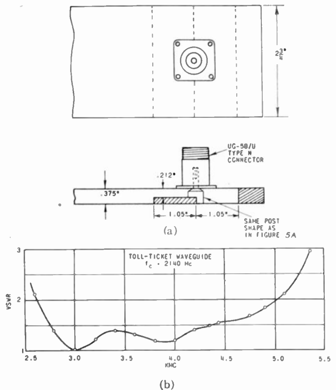
Fig. 6—Transforming junction designed to have voltage-standing-wave ratio = 1.5 at center frequency of 3550 megacycles. (a) Construction. (b) Frequency response.
