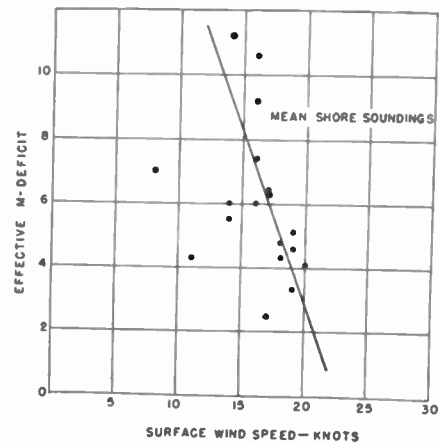
Fig. 24—Effective M deficit versus wind speed.
