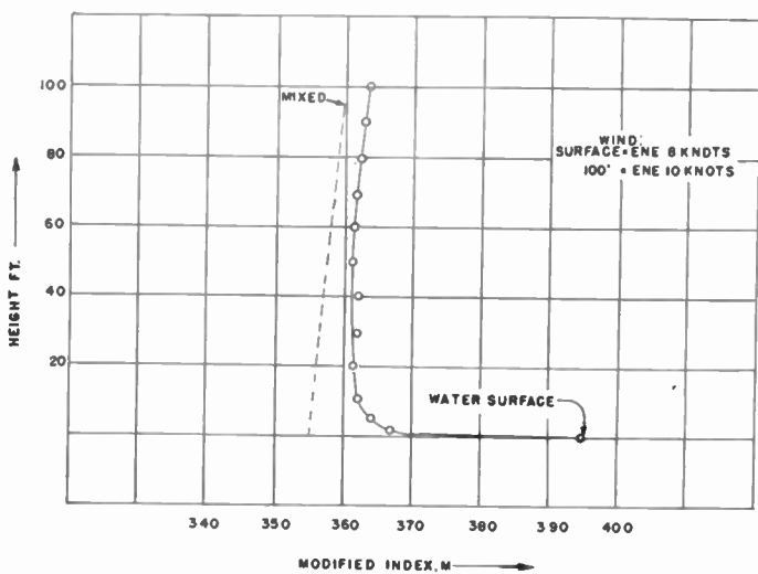
Fig. 20—Modified index curve for 0700-1900, March 24 and 25, 1945.
