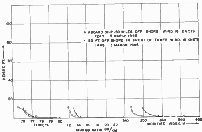
Fig. 19—Very-low-level soundings of March 3 and 5, 1945.
