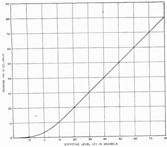
Fig. 6—Relation between masking and the effective level of a critical band width. M is the change in the threshold of a pure tone due to the noise. Z is the number of decibels that the total energy in a critical band is above its threshold level.
