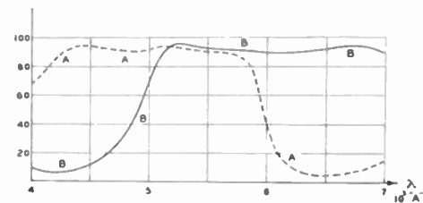
Fig. 4—Spectral characteristic of two dichroic mirrors.
