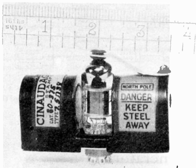
Fig. 1—6D4 permanent-magnet noise source.
