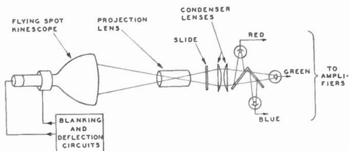
Fig. 1—Diagram of the color-slide scanner.
