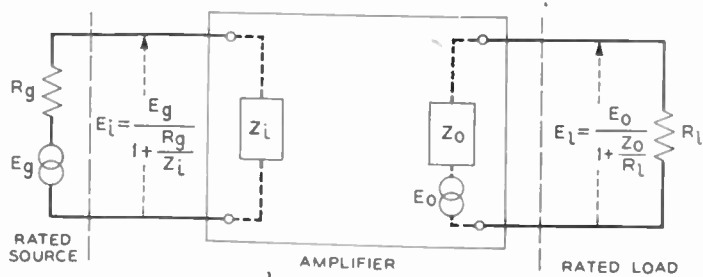
Fig. 3—Amplifier terminated in rated source and rated load for gain measurements.
