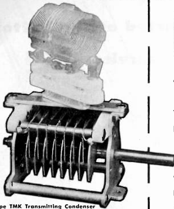
Type TMK Transmitting Condenser
