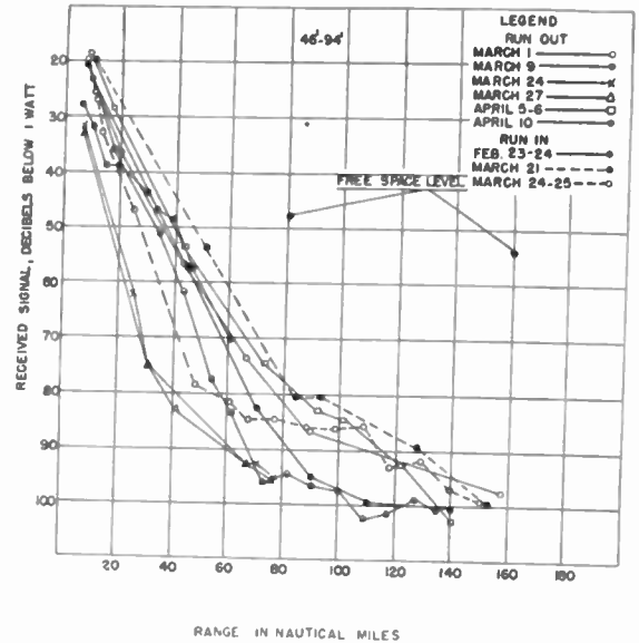
Fig. 10—Received power level versus range at 9 centimeters. Composite of all runs with 46- to 96-foot antennas.
