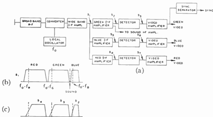
Fig. 4—Simultaneous color receiver for three-carrier or subcarrier reception.
