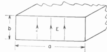
Fig. 1—Cross section of rectangular wave guide.
