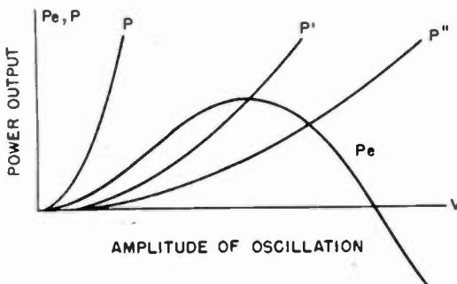
Fig. 4—Power output as a function of oscillation amplitude.
