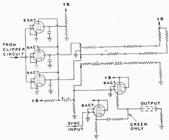
Fig. 14—Detail of the gamma-control circuit.
