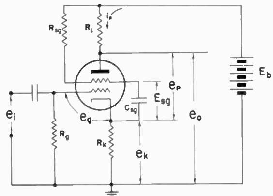
Fig. 3—Circuit diagram of a tetrode tube used in a cathode-degenerated stage.
