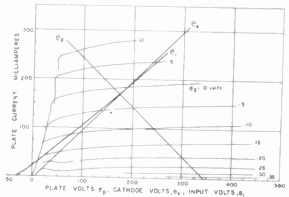
Fig. 6—Plate-characteristic curves for a 6L6 tetrode with the addition of the lines needed for analysis of the circuit of Fig. 5.
