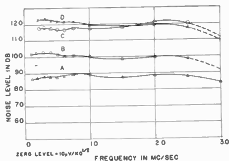
Fig. 7—Noise spectrum for circuit of Fig. 5.
