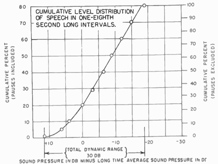
Fig. 3—Curve showing cumulative level distribution of speech in an octave band in \frac{1}{8} -second-long intervals versus the sound-pressure level in decibels minus long-time average sound-pressure level in decibels. The right-hand ordinate has been added to the original graph of French and Steinberg.
