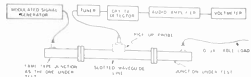
Fig. 15—Test setup.
