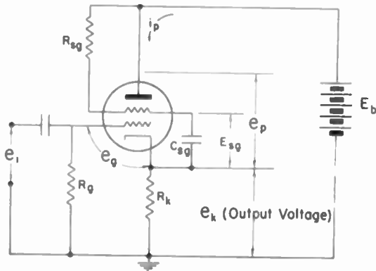
Fig. 5—Circuit diagram for a tetrode-connected cathode-follower stage.
