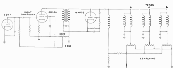
Fig. 6—Horizontal-deflection circuit.
