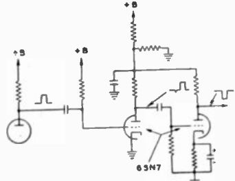
Fig. 12—Detail of the nonlinear differentiating circuit for making clamping pulses of RMA synchronizing signals.
