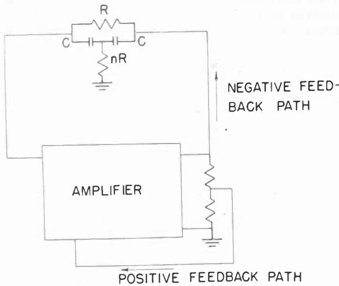
Fig. 1—Basic oscillator circuit.
