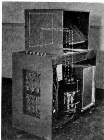
Fig. 8—Receiver showing trinoscope assembly.
