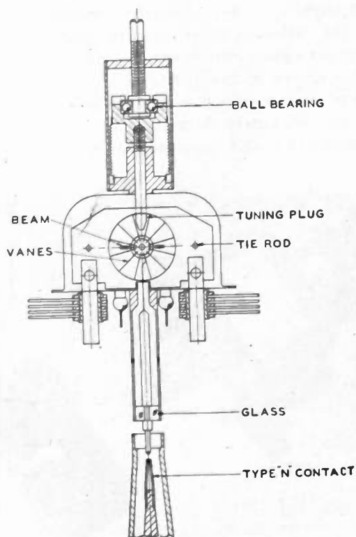
Fig. 1—Longitudinal cross section.
