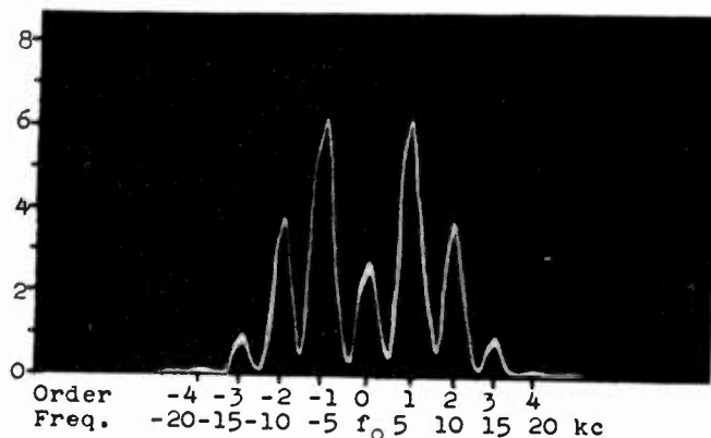
Fig. 3—Oscilloscope picture of single-tone frequency-modulated signal (5-kilocycle modulation—10-kilocycle deviation).
