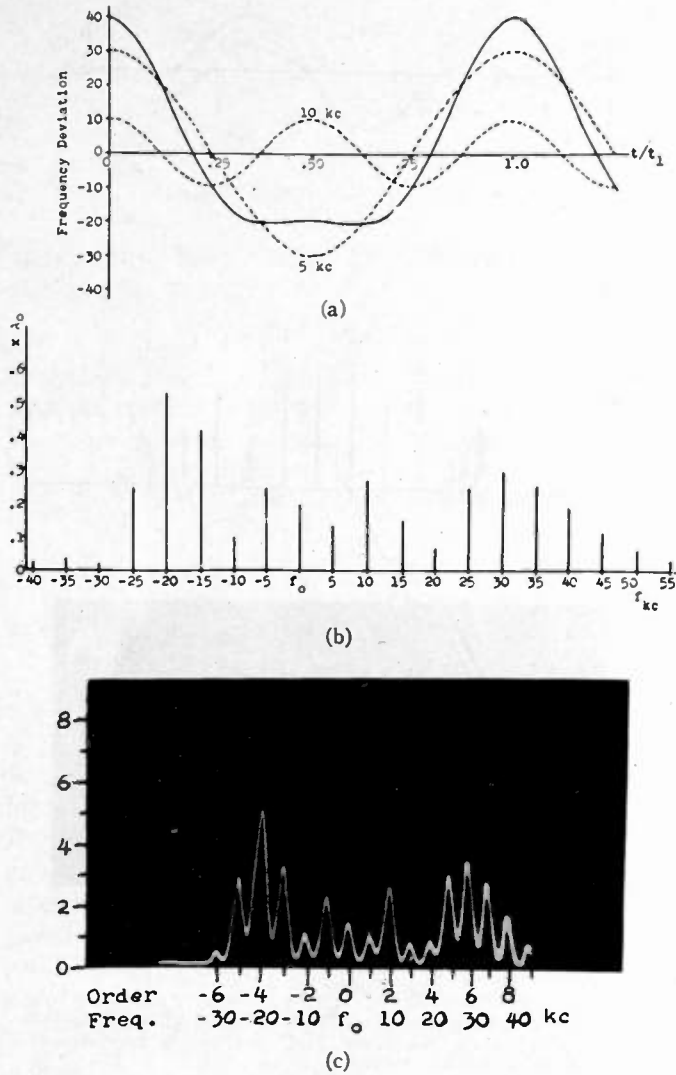
Fig. 10—Two-tone frequency-modulated signal (5-kilocycle modulation—30-kilocycle deviation, and 10-kilocycle modulation—10-kilocycle deviation).
