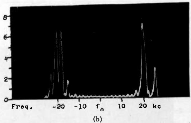
Fig. 16—Multitone frequency-modulated signal (500-cycle square-wave modulation—20-kilocycle deviation.)
