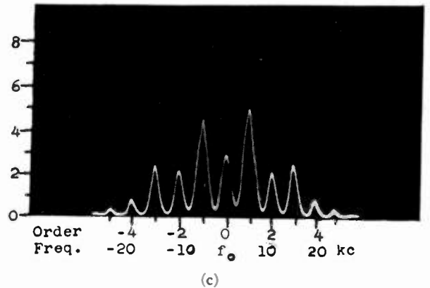
Fig. 7—Two-tone frequency-modulated signal (5-kilocycle modulation—10-kilocycle deviation, and 10-kilocycle modulation—10-kilocycle deviation.)
