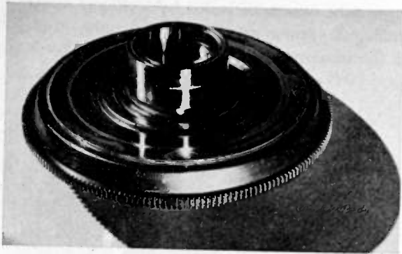
Fig. 2—Triple-cylinder tuning element mounted on a diaphragm forming a portion of the tube lid.
