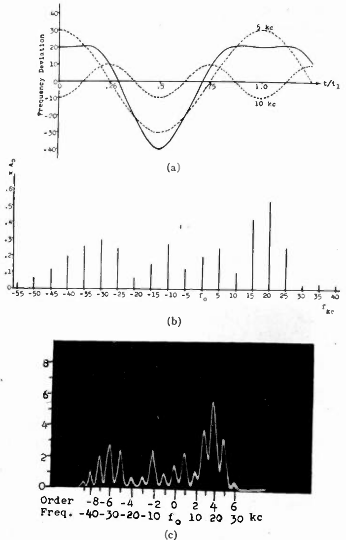
Fig. 11—Two-tone frequency-modulated signal (5-kilocycle modulation—30-kilocycle deviation, and 10-kilocycle modulation—10-kilocycle deviation).
