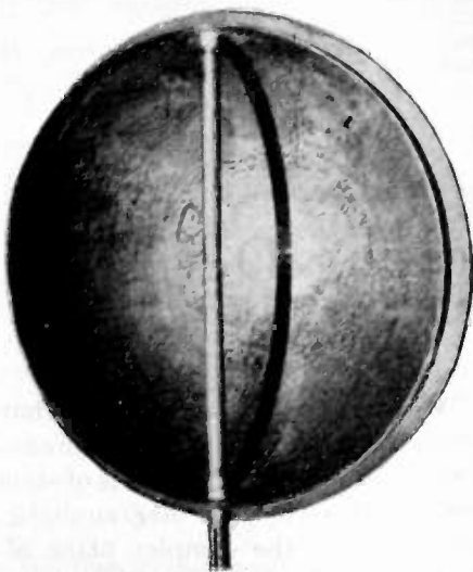
Fig. 8—View of cylinder antennas of 1 1/8-inch diameter in a hemisphere of 13-inch radius.
