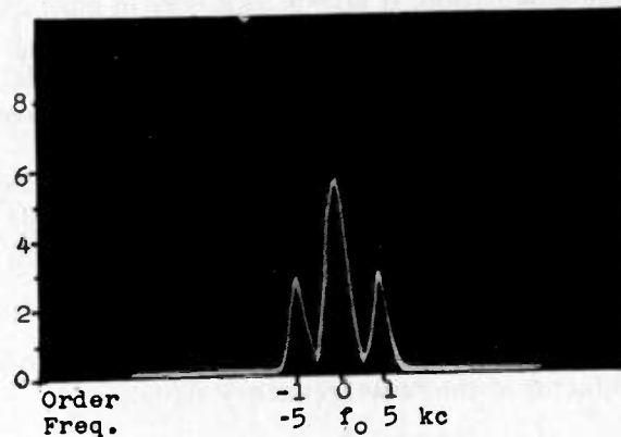
Fig. 1—Oscillogram picture of single-tone amplitude-modulated signal.
