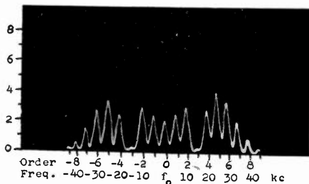
Fig. 4—Oscilloscope picture of single-tone frequency-modulated signal (5-kilocycle modulation—30-kilocycle deviation).
