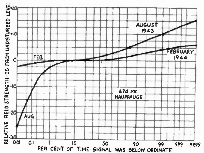
Fig. 9—Same as Fig. 8, but for frequency of 474 megacycles. Note that field here is compared to undisturbed level, rather than free space.
