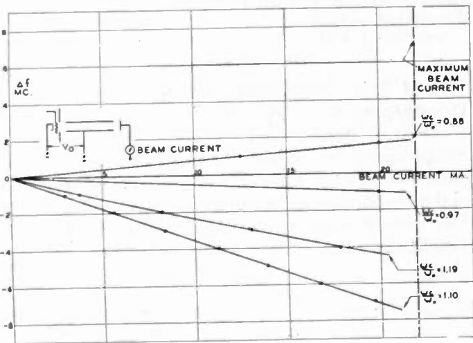
Fig. 8—Frequency shift versus beam current for various values of \omega_c/\omega_0 = He/m\omega_0 . Beam current is varied by grid voltage.
