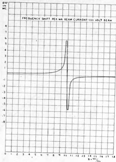
Fig. 13—Frequency shift versus magnetic field for the rectangular cavity structure.
