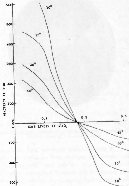
Fig. 2—Computed values of reactance for cones in free space versus cone length. Cone revolution angles, 10 to 45 degrees.
