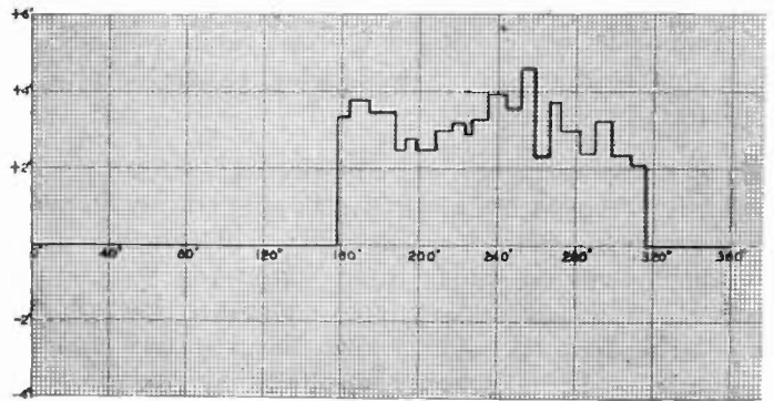
Fig. 5—Skyline survey for beacon with antenna height of 20 feet.
