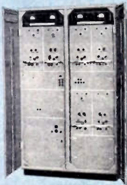
RADIO TRANSMITTER 185-A. Provides maximum operation on 1 phone channel and 1 CW channel simultaneously, or 2 CW channels simultaneously with choice of up to 6 different frequencies.
