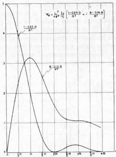
Fig. 2—Electronic admittance as a function of \theta .
