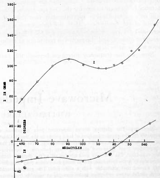
Fig. 10—Electrical characteristic of cylinders of 9/16-inch diameter in a hemisphere of 13-inch radius.
