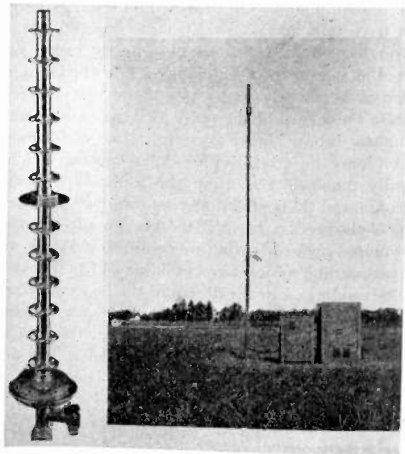
Fig. 2—3000-megacycle beacon and antenna in operating position with inset showing details of antenna assembly.
