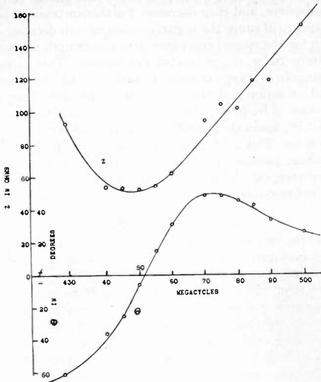
Fig. 7—Electrical characteristic of cones having a 5-degree revolution angle in a hemisphere of 13-inch radius.
