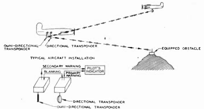
Fig. 11—Typical "ring-around" system.
