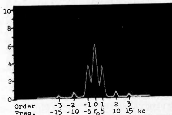
Fig. 2—Oscillogram picture of multitone amplitude-modulated signal.
