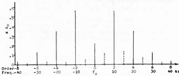
Fig. 20—Single-tone combined amplitude- and frequency-modulated signal. Frequency spectrum after combined modulation:
