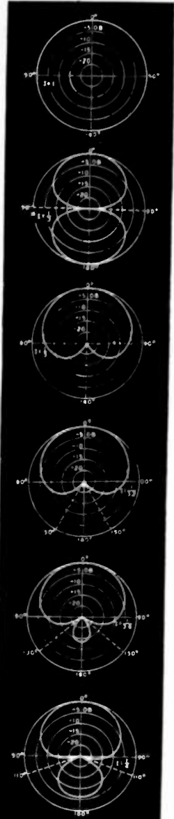
These six pick-up patterns are available with the 639B Microphone.
