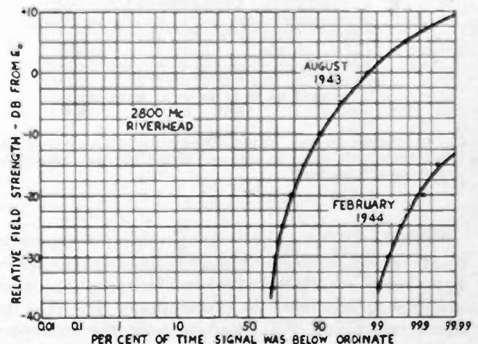
Fig. 13—Same as Fig. 11, but for 2800 megacycles.
