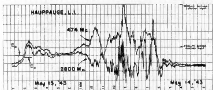
Fig. 6—Example of synchronous fading of opposite phase over an optical path, transcribed from record taken at Hauppauge.
