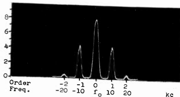
Fig. 5—Oscilloscope picture of single-tone frequency-modulated signal (10-kilocycle modulation—10-kilocycle deviation).
