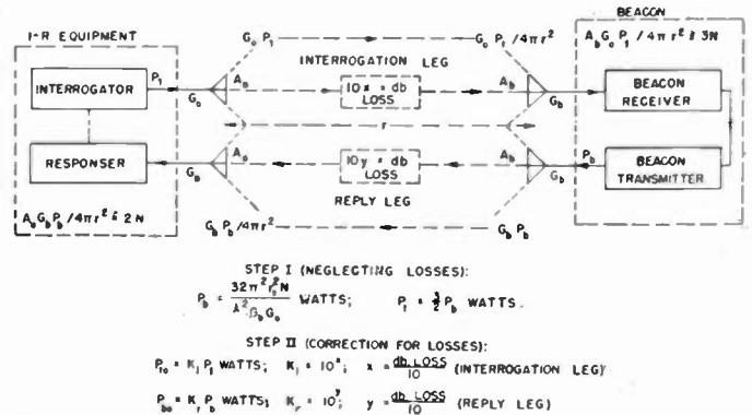
Fig. 4—Summary of secondary-system design considerations.
