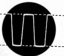
Adjust amplitude of this calibrating signal to match desired peaks of unknown signal. Read voltage from dial settings of calibrator.
