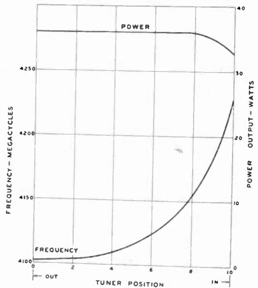
Fig. 7—Tuning curves taken at matched load. “Out” and “in” refer to position of tuning plug in the cavity.
