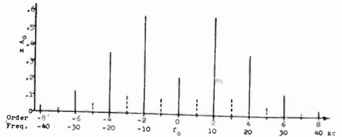
Fig. 21—Single-tone combined amplitude- and frequency-modulated signal. Frequency spectrum after combined modulation:
