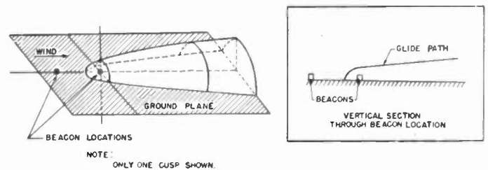
Fig. 12—Hyperbolic glide path.
