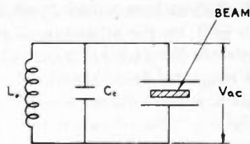
Fig. 4—Equivalent lumped circuit of resonant system.
