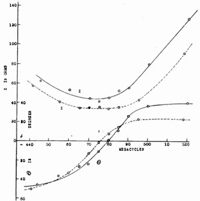
Fig. 5—Electrical characteristic of cones having a 15-degree revolution angle in hemisphere of 13½-inch radius. Solid line: fine tips; dotted line: blunt tips (see text).
