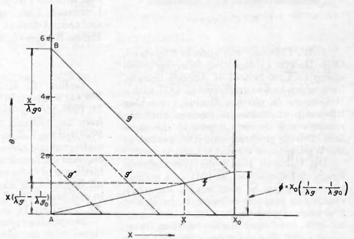
Fig. 4—This auxiliary sketch shows the relation of probe position ( x ), angular position of the standing-wave ratio scale ( \theta ), and guide wavelength ( \lambda_{g0} ). The lines g', g'' \dots supplement g in order to reduce the range of \theta values.
