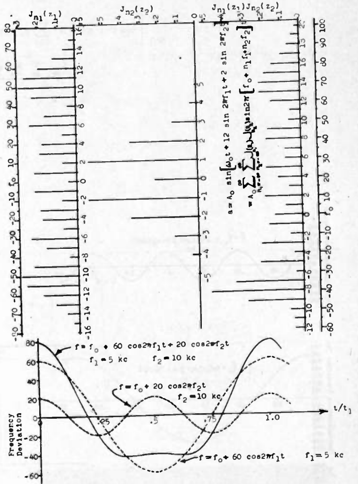
Fig. 13—Single- and two-tone frequency-modulated signal (5-kilocycle modulation—60-kilocycle deviation, and 10-kilocycle modulation—20-kilocycle deviation).
