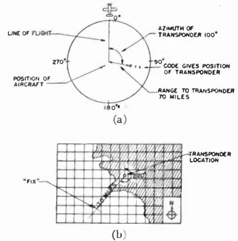
Fig. 9.—Obtaining a "fix."
