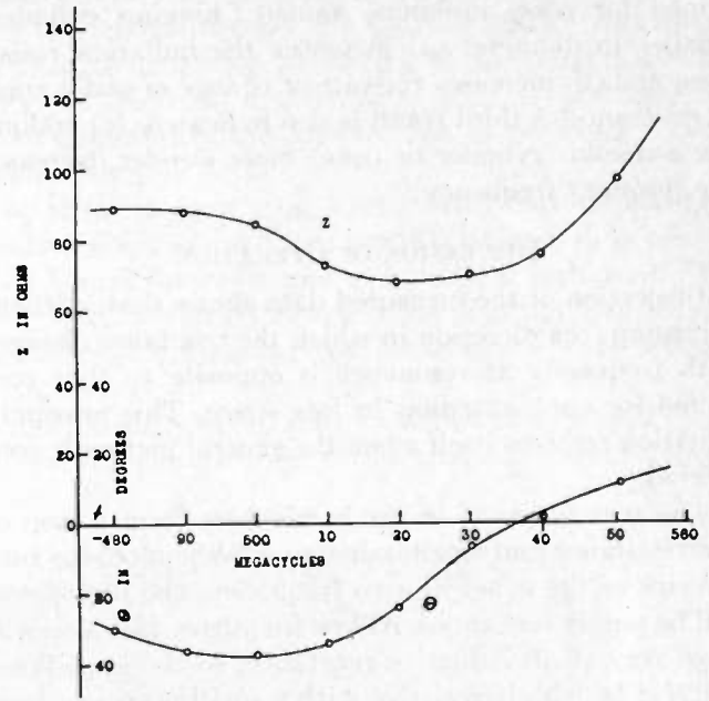
Fig. 9—Electrical characteristic of cylinders 1 1/8-inch diameter in a hemisphere of 13-inch radius.
