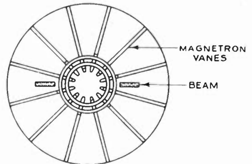
Fig. 7—Cross-sectional view of multivane magnetron with auxiliary beams.
