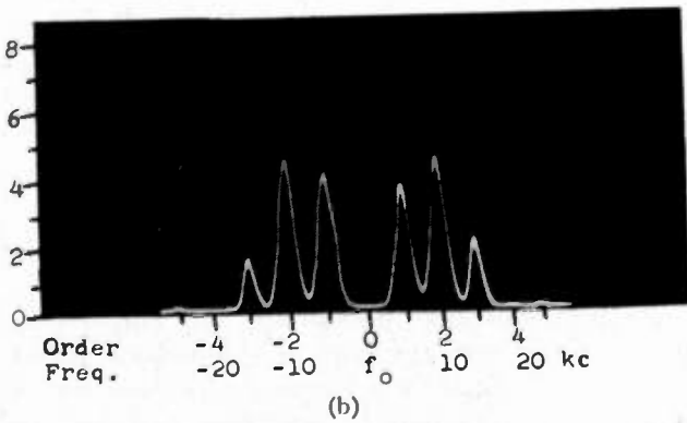
Fig. 15—Multitone frequency-modulated signal (5-kilocycle square-wave modulation—10-kilocycle deviation.)
