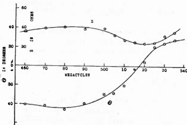
Fig. 4—Electrical characteristic of cones having a 45-degree revolution angle in hemisphere of 12½-inch radius.
