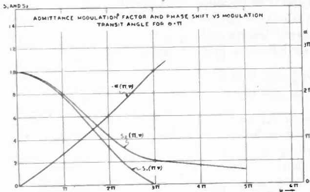
Fig. 8—Admittance modulation factor and phase shift versus modulation transit angle for \theta = \pi .
