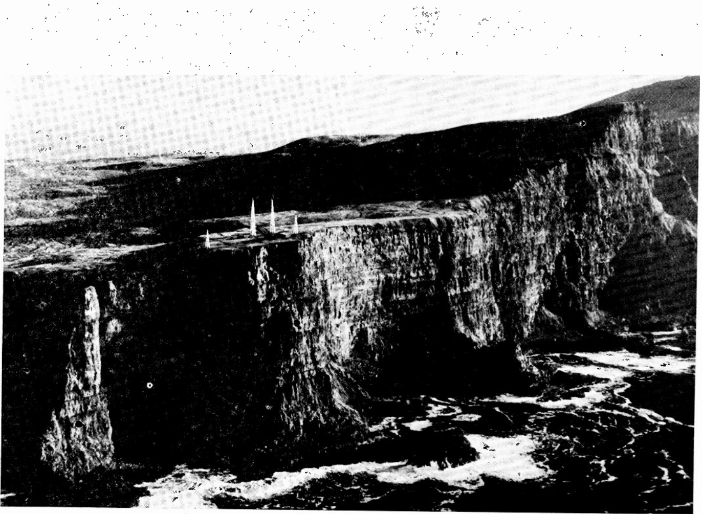
Fig. 13—An aerial view of a loran transmitting station in the Faeroes Islands. The wooden antenna towers are about 120 feet high. The height of the cliff is not an advantage.
