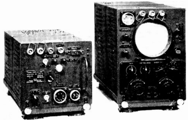
Fig. 7—An air-borne loran receiver-indicator, shown without the interconnecting cables. The smaller unit contains the receiver and the main power supply for both units, and need not be immediately accessible. 45,000 of these sets had been delivered by August 1, 1945.
