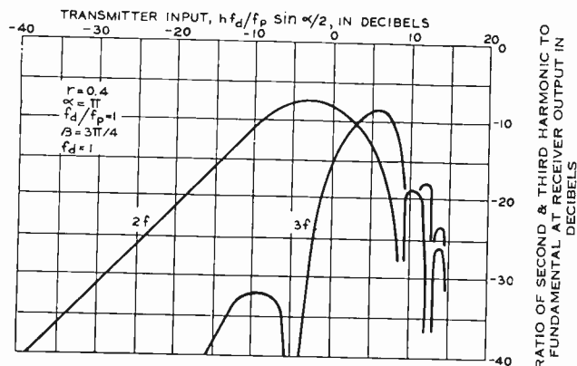
Fig. 6—Single-frequency harmonic output as a function of fundamental input to transmitter.
