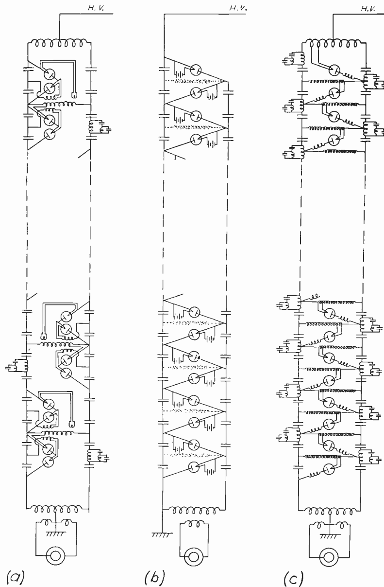
Fig. 9—Various forms of capacitor-coupled rectifier cascades.
