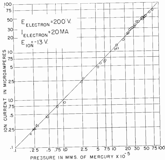
Fig. 2—Ion current versus pressure. \circ and \square represent readings taken one week apart on the same gauge (#1). \times and \Delta represent readings taken on the same gauge (#2), with the latter readings being taken after the tube had been burned in air three times, being partially evacuated after each time.
