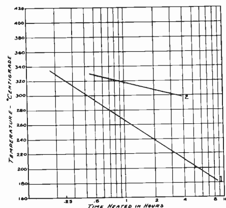
Fig. 2—Optimum baking conditions for 774 Pyrex-brand glass rods, treated with a DC 200 fluid; the times of baking should not be less than those given by curve 1 or greater than those given by curve 2.
