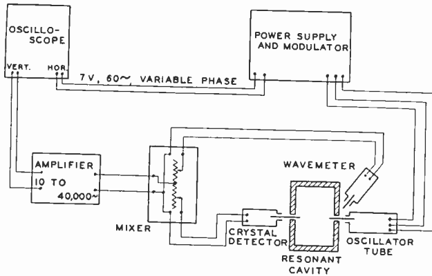
Fig. 1—Diagram of measuring equipment.
