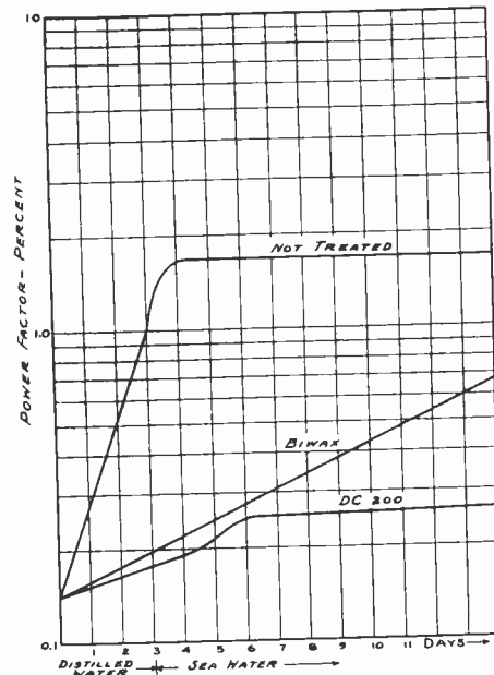
Fig. 6—Power factors of coil forms as affected by immersion in water.
