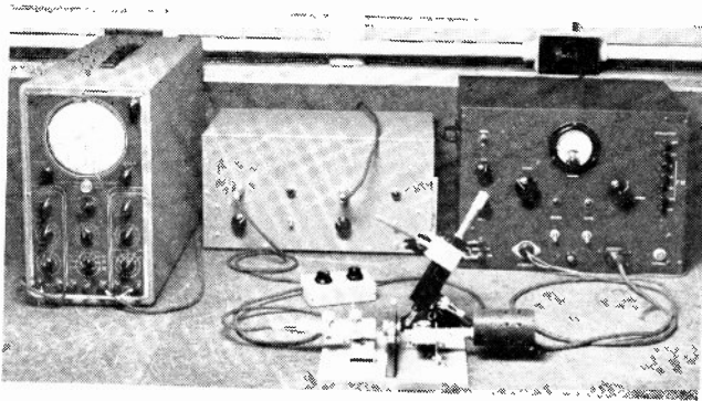
Fig. 2—Photograph of measuring equipment. The oscilloscope, audio amplifier, and power-supply modulator are in the background. The mixer box is in the center. In the foreground are the detector, cavity mounting, wavemeter, and oscillator.
