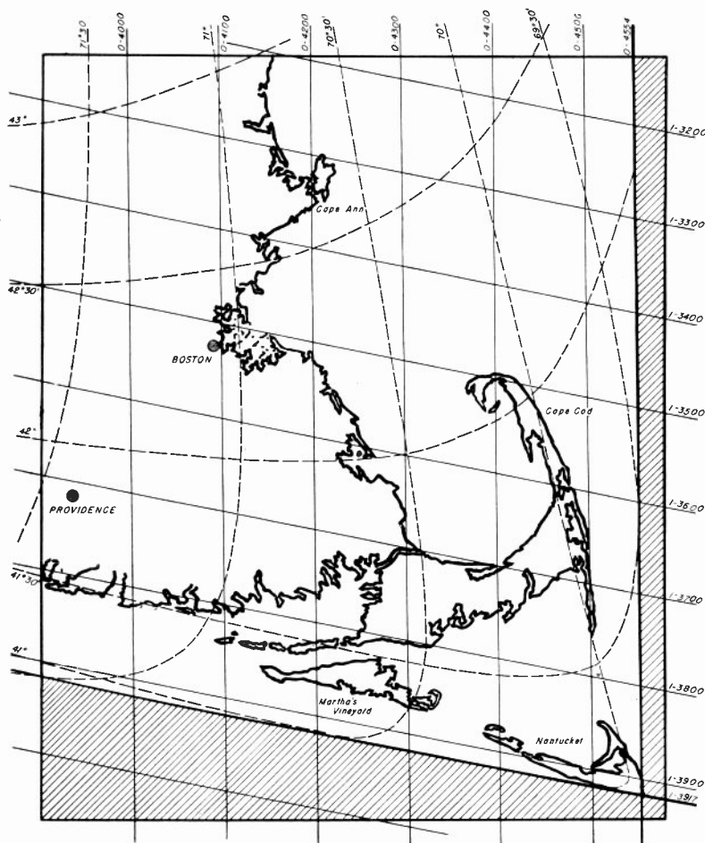
Fig. 14—A map drawn by assuming that loran lines of position are straight and parallel. By use of this sort of map the construction of devices for automatically plotting position becomes easy. The example shown exhibits almost the worst possible distortion.
