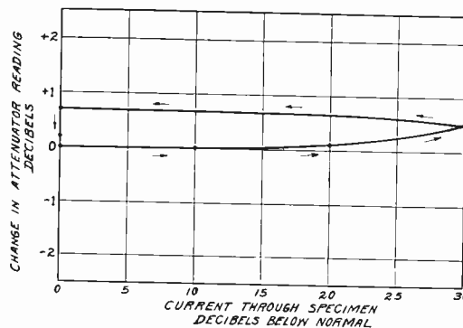
Fig. 8—Observed changes in attenuator readings for changes in current through specimen. 0.0106-inch-wall copper tube at 3 megacycles. Normal current 3 amperes.
