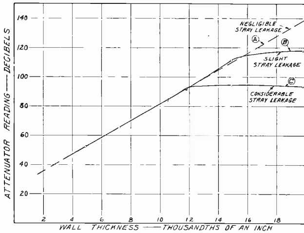
Fig. 12—Measured effects of stray leakage at 3 megacycles. Pure-copper tubes of different wall thicknesses.
