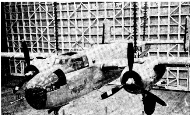
Fig. 5—B25 airplane supported and ready for study.
