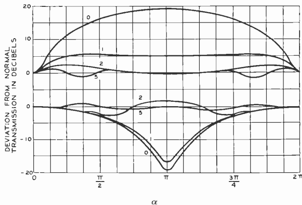
Fig. 9—Frequency distortion; \alpha = linear variable with frequency. The number on each curve is the value of hf_a/f_p used in computation. \beta = \pi in the upper group; \beta = 0 in the lower group. r = 0.8 .
