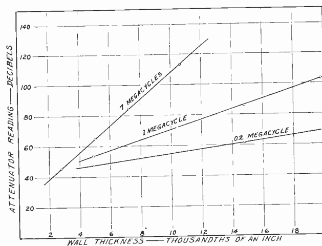
Fig. 7—Test results at three frequencies on 2-foot 5/16-inch-inside-diameter pure-copper tubes of different wall thicknesses.
