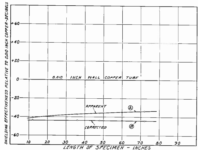
Fig. 13—(A) Measured apparent shielding effectiveness at 3 megacycles of a shield having exceptionally high resistance. Tests on specimens of different lengths. (B) True shielding effectiveness of the high-resistance shield obtained by correcting values shown in (A).
