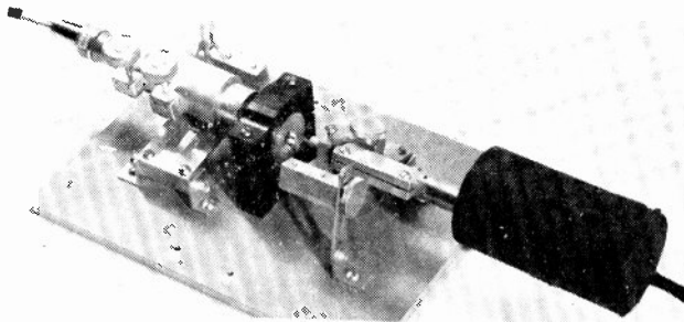
Fig. 3—Detector, cavity mounting, and oscillator. The low- Q crystal detector circuit is a coaxial line, tunable by a rack-and-pinion control. Another rack and pinion controls the insertion of the detector probe into the resonator. The tunable transmission line from the oscillator is terminated by the small wire probe which projects into the cylindrical cavity being tested.
