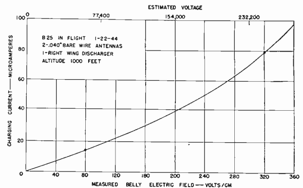
Fig. 3—Observed charging current versus belly electric field in flight
