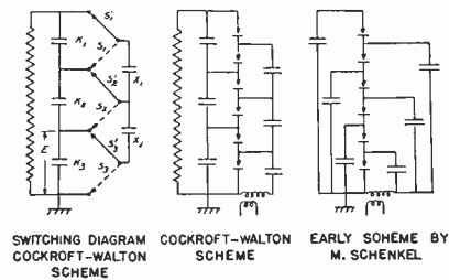
Fig. 8—Fundamental diagram of the Cockcroft-Walton scheme.
