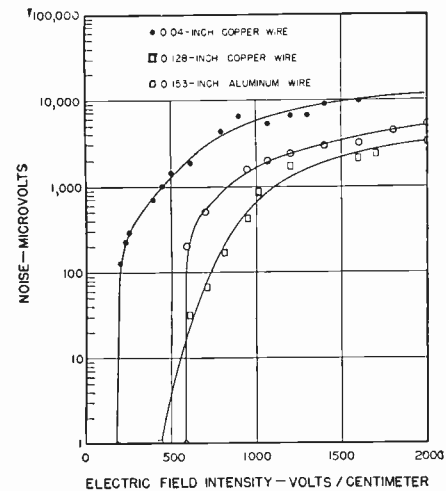
Fig. 6—Noise characteristics for three bare-wire antennas measured at 900 kilocycles on RB-37 suspended in the hangar. Airplane charged negative.
