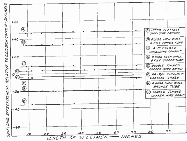
Fig. 11—Measured shielding effectiveness of various types of shields at 3 megacycles. Tests on specimens of different lengths.
