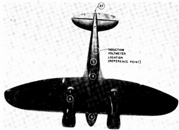
Fig. 2—Bottom view of model plane showing the field measurements relative to the reference base of 10.
