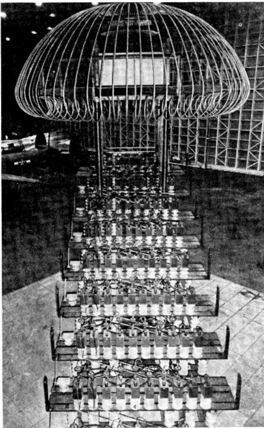
Fig. 3—Close-up view of the high-voltage generator showing the rectifier cascade.
