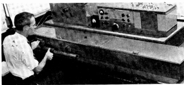
Fig. 2—Production-test equipment for comparative measurement of cylindrical shields at 3 megacycles.
