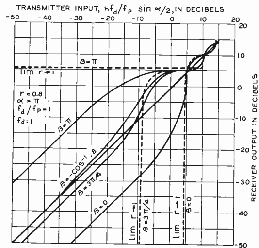
Fig. 2—Single-frequency amplitude characteristics of an over-all frequency-modulation radio system.
