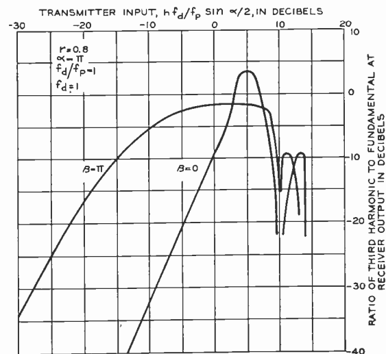
Fig. 5—Single-frequency harmonic output as a function of fundamental input to transmitter.
