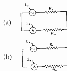
Fig. 14—Equivalent circuits. (a) With standard under test (attenuator reads A_1 ). (b) With unknown under test (attenuator reads A_2 ).
