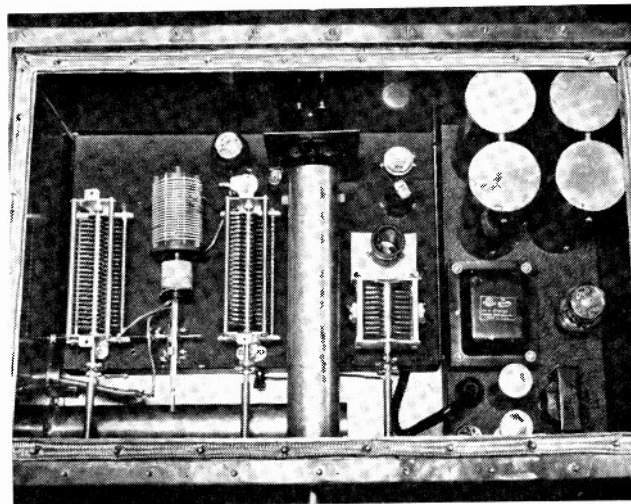
Fig. 3—Inside view of signal-source unit.
