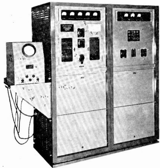
Fig. 11—A loran transmitter, capable of about 100-kilowatt pulse output. The high-voltage power supply is at the right, with the modulator and radio-frequency unit in the center. On the shelf at the left is a monitor oscilloscope used to check the output frequency and pulse shape.
