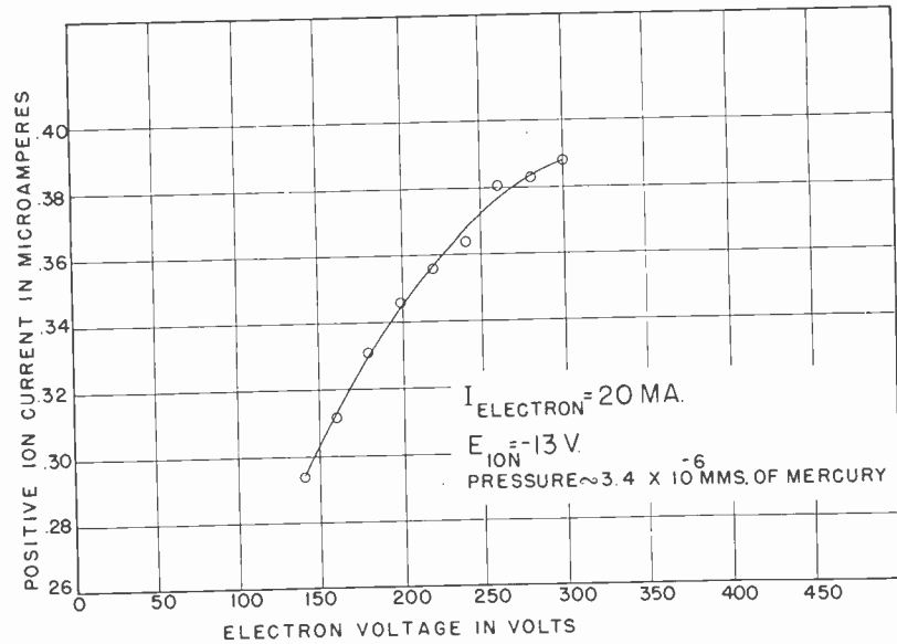
Fig. 3—Positive-ion current versus electron-collector voltage.
