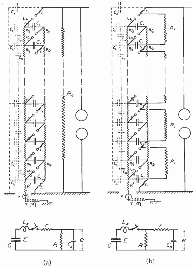
Fig. 11—Impulse generator connections and equivalent circuits for standard surge waves; (a) 1.5- to 40-microsecond surge wave, (b) 1- to 5-microsecond surge-wave connection.
