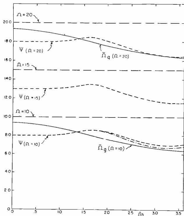
Fig. 1—Expansion parameters \Omega (Hallén and Bouwkamp); \bar{\Omega}_g (Gray and modified Gray) for \Omega = 10, 20 ; and \psi (King and Middleton), for \Omega = 10, 15, 20 . The curve for \psi ( \Omega = 10 ) is shown divided into two parts. The lower part was calculated using the zeroth-order sinusoidal distribution of current (10). The upper part was calculated using a function approximating the first-order distribution of current.
