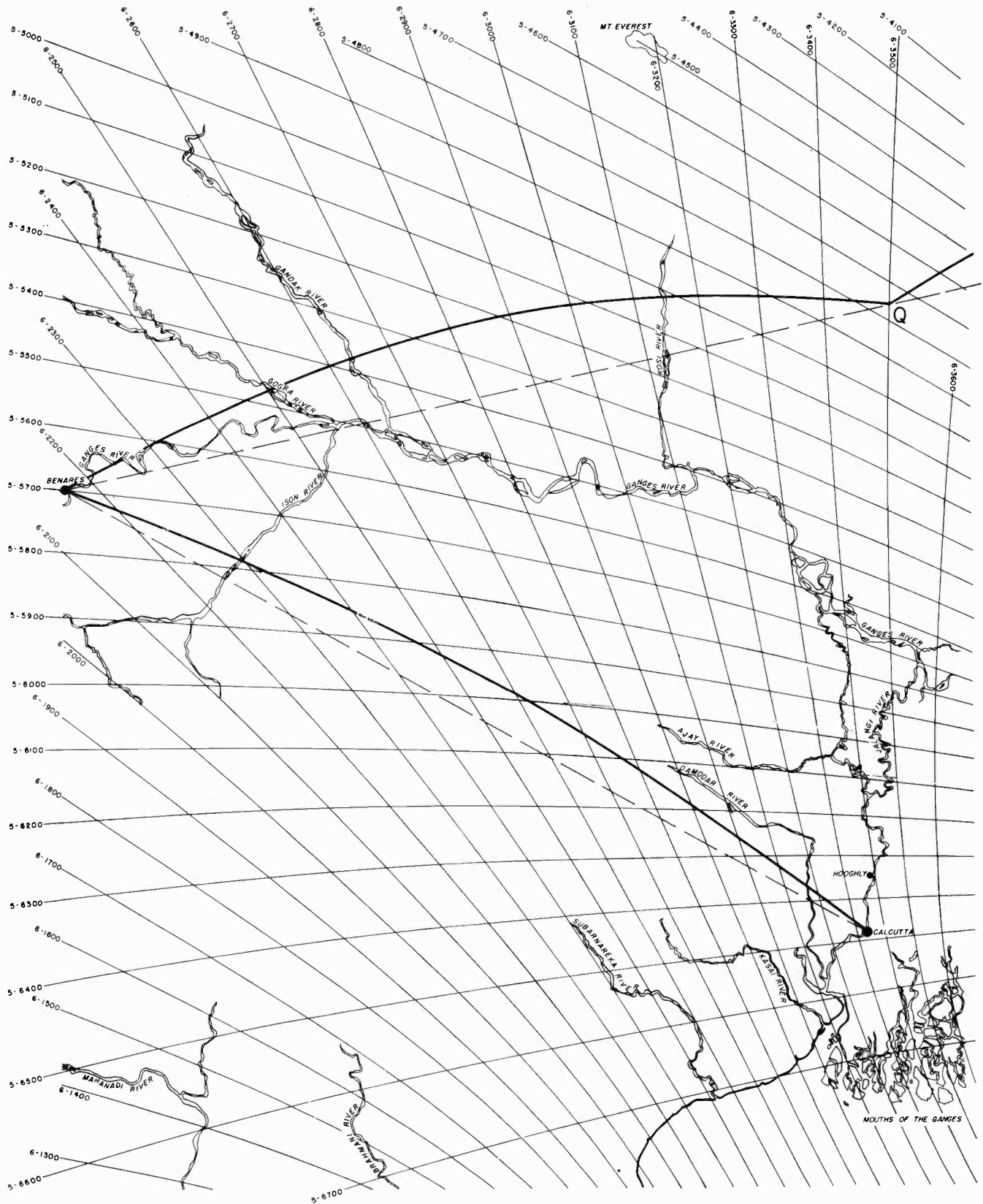
Fig. 15—Two examples of the loximuth line, or curve which intersects two families of loran hyperbolas at a constant ratio. These lines can be followed automatically by the use of relatively simple equipment.
