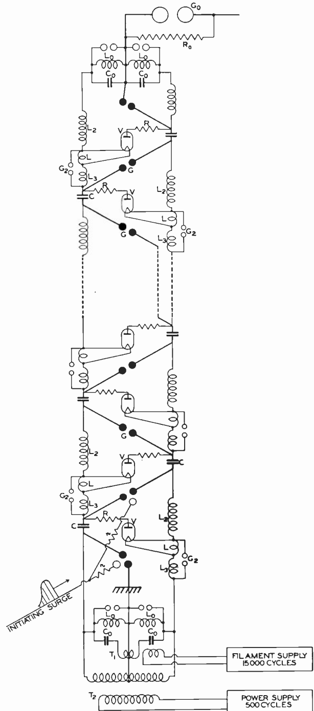
Fig. 4—Schematic diagram of the high-voltage generator.
