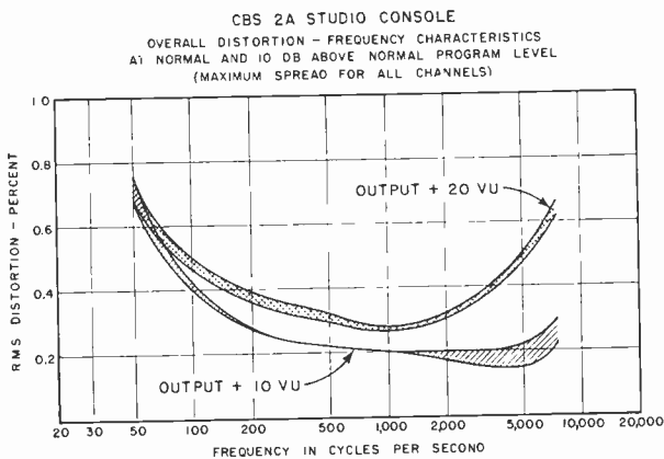
Fig. 11—The harmonic distortion, as a function of frequency, of the complete program channel of the Columbia Broadcasting System 2A studio console is shown above. The measurements are full single-frequency test tones at output levels corresponding to normal program level (+10 vu) and at levels 10 decibels above normal (+20 vu). The absolute magnitude of the harmonic distortion and the spread for a number of channels are seen to be quite small.
