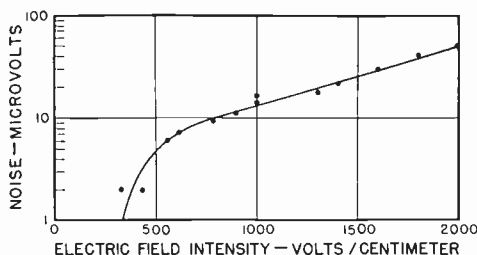
Fig. 5—Base noise characteristic of 0.128-inch bare copper wire protected by a high-resistance cord and installed on RB-37 suspended in the hangar. Noise measured at 900 kilocycles, airplane charged negatively.
