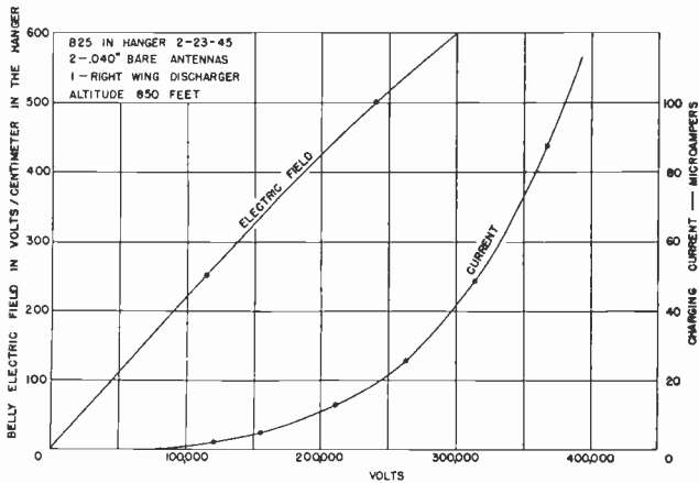
Fig. 4—Voltage-belly electric field-charging current characteristics for B25 supported in hangar.
