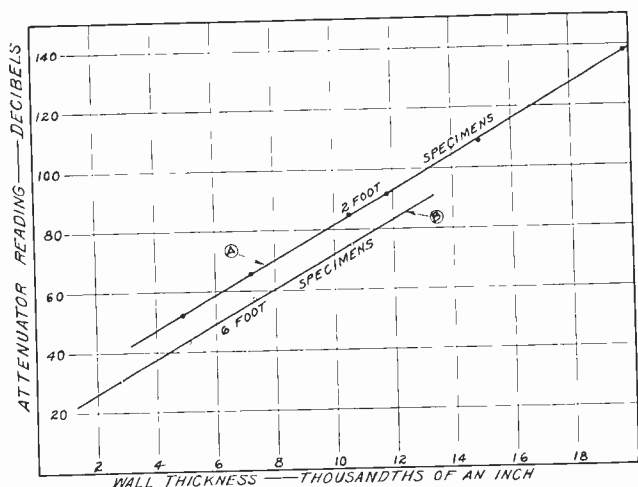
Fig. 6—Test results at 3 megacycles on 5/16-inch-inside-diameter pure-copper tubes of different wall thicknesses.
