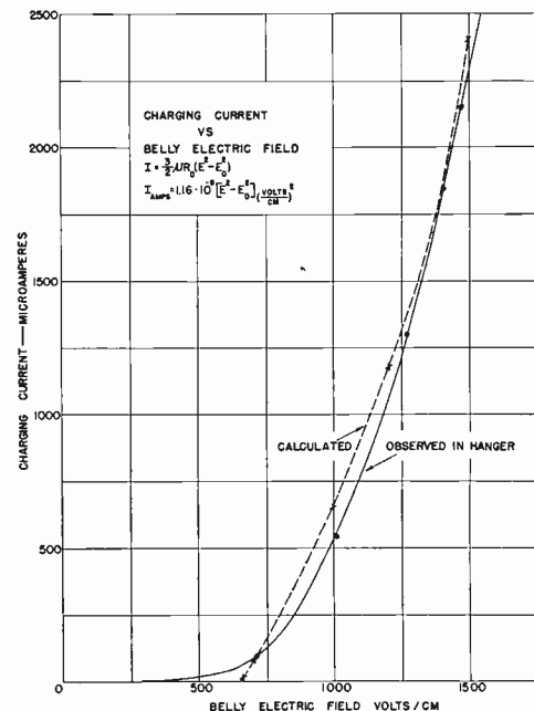
Fig. 8—Charging current to B25 in hangar compared with the calculated values.
